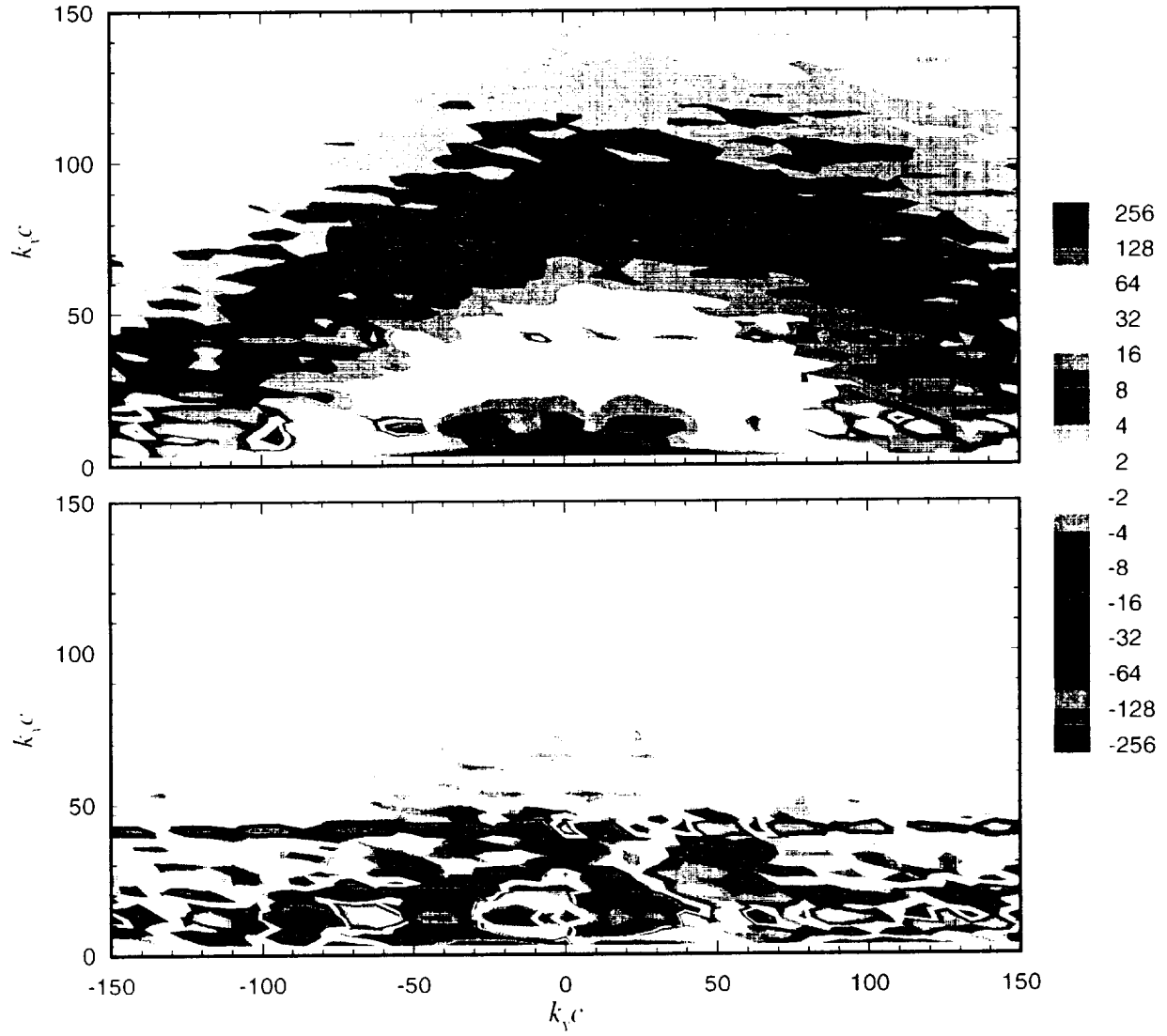
Figure 3.48: Wave-number frequency spectrum of the spanwise ( v ) velocity component measured along the line T4 about point D shown in Figure 3.4. Contours of the real component of \phi_{vr} U_\infty / (4\pi^2 c^2 \overline{v^2}) \times 10^6 are shown at top; imaginary component on bottom.
