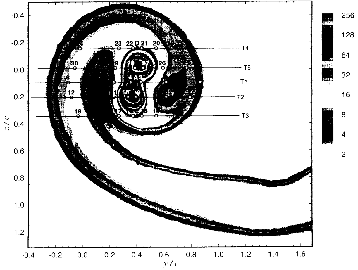
Figure 3.4: Contours of axial normal turbulence stress, \overline{u^2}/U_\infty^2 \times 10^5
