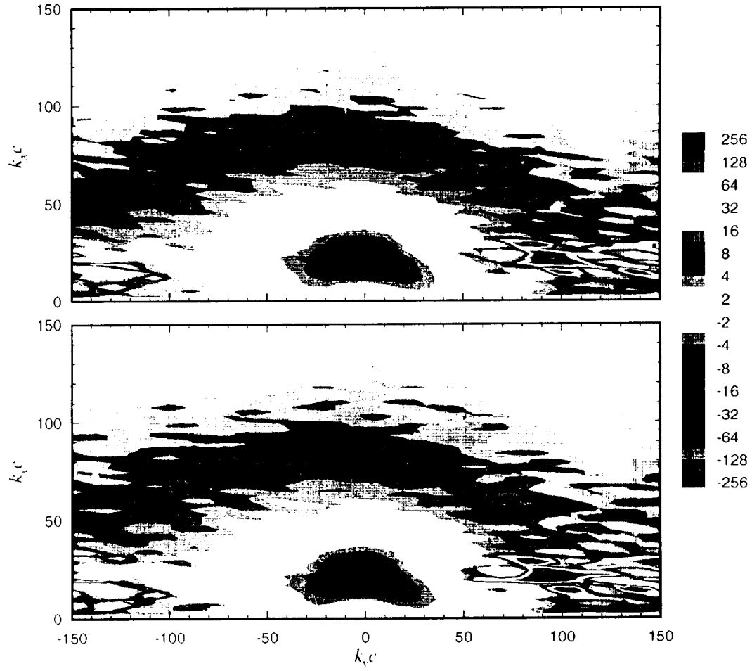
Figure 3.37: Comparison of the wave-number frequency spectrum of the upwash ( w ) velocity component measured by Miranda and Devenport [25] in the 3-D wake of an airfoil calculated with (top) and without (bottom) the use of the Liepman model. Contours are \phi_{uw} U_{\infty} / (4\pi^2 c^2 \overline{w^2}) \times 10^6 .
