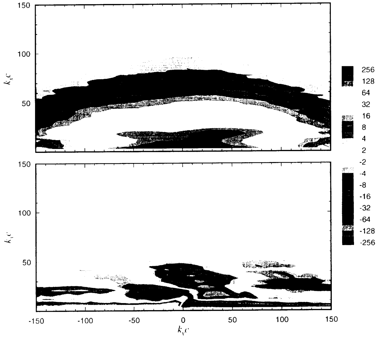
Figure 3.42: Wave-number frequency spectrum of the spanwise ( v ) velocity component measured along the line T2 about point B shown in Figure 3.4. Contours of the real component of \phi_{vv} U_\infty / (4\pi^2 c^2 \overline{v^2}) \times 10^6 are shown at top; imaginary component on bottom.
