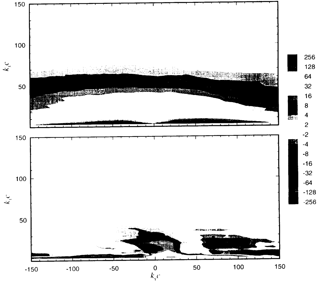
Figure 3.43: Wave-number frequency spectrum of the upwash ( w ) velocity component measured along the line T2 about point B shown in Figure 3.4. Contours of the real component of \phi_{w\omega} U_\infty / (4\pi^2 c^2 \overline{w^2}) \times 10^6 are shown at top; imaginary component on bottom.
