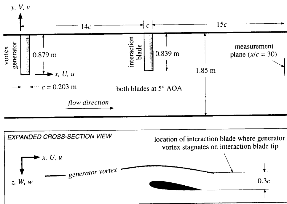
Figure 2.2: Wind tunnel schematic and coordinate system
