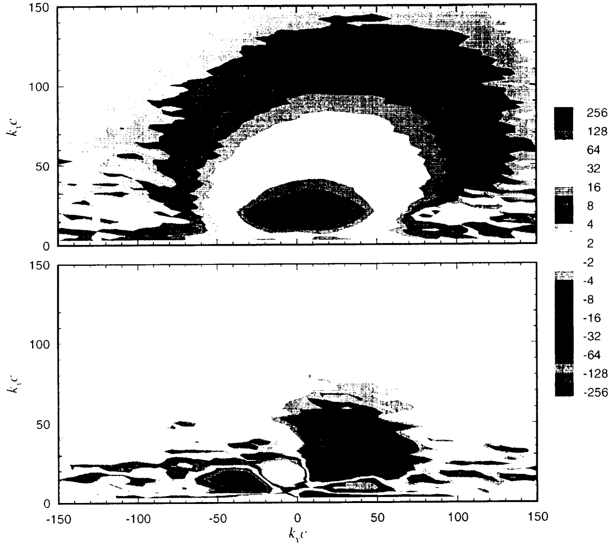
Figure 3.49: Wave-number frequency spectrum of the upwash ( w ) velocity component measured along the line T4 about point D shown in Figure 3.4. Contours of the real component of \phi_{ww} U_\infty / (4\pi^2 c^2 \overline{w^2}) \times 10^6 are shown at top; imaginary component on bottom.
