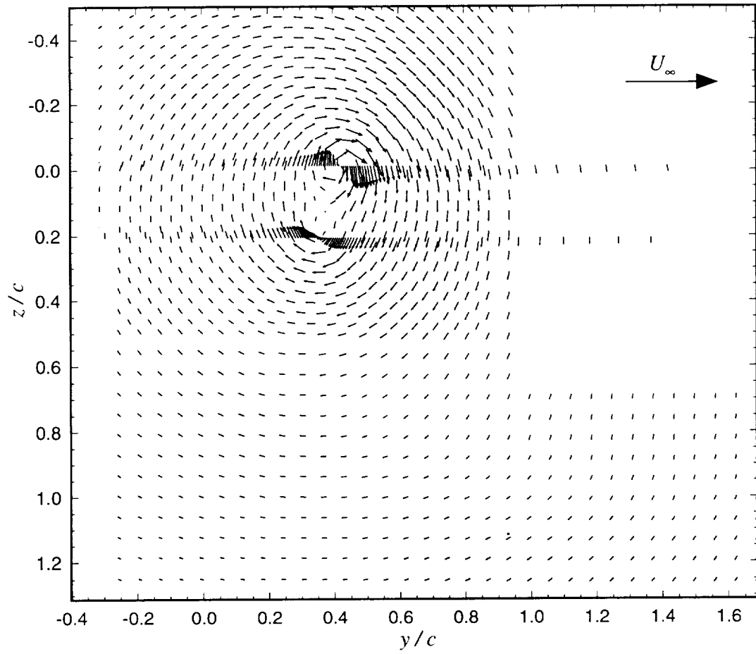
Figure 3.1: Mean cross flow velocity vectors
