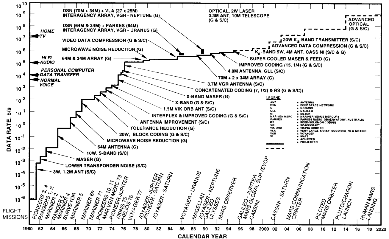
Figure 16. Stair-Step Chart of Telecommunications Performance.
