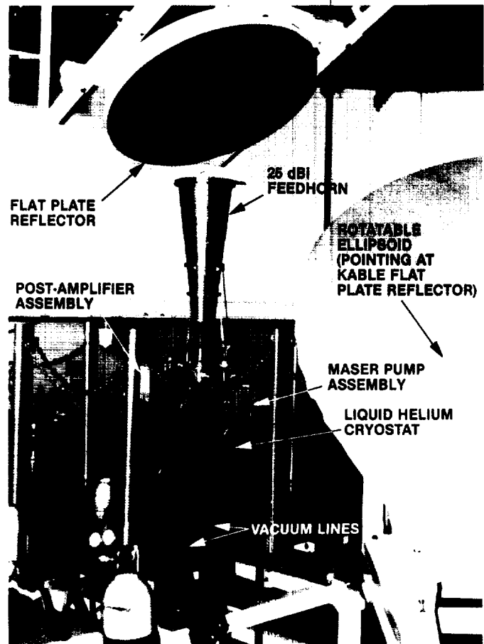
Figure 8. Ultra-Low-Noise Amplifier (ULNA) at DSS 13.
