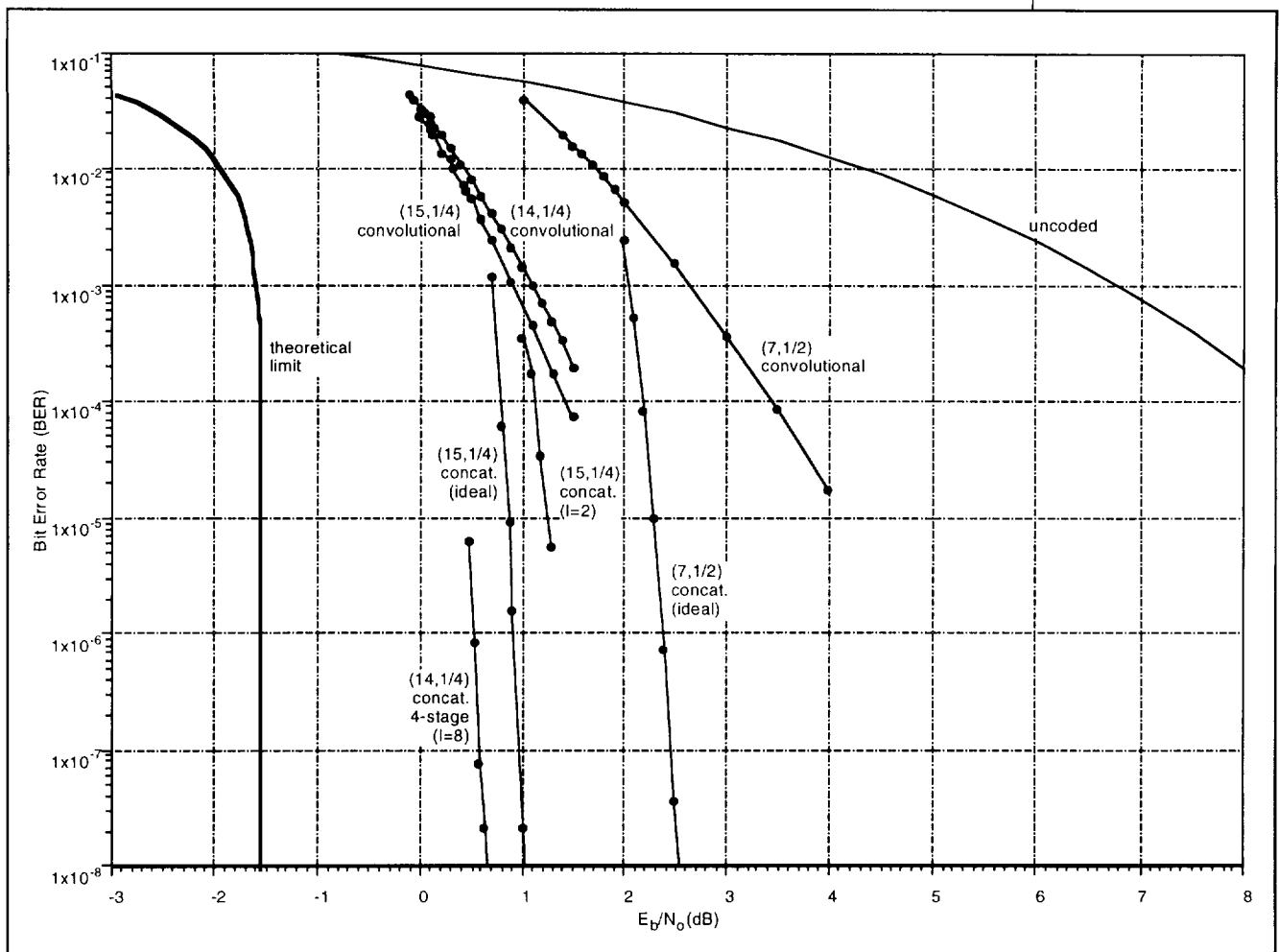
Figure 11. The Probability of Erroneous Data Bits.
