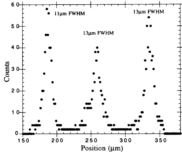
Figure 2 Histogram of the pinhole images in Figure 1 showing the point spread functions, & structure of one peak due to discrete pore locations.
