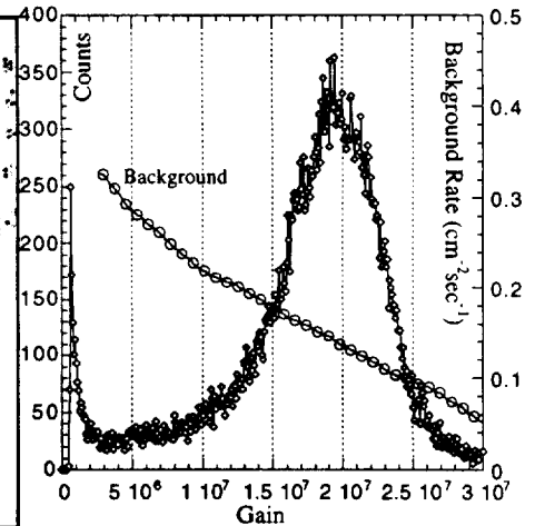
Figure 5. PHD for Philips 7\mu\text{m} pore MCP 4 \times 50:1 L/D stack & background rate vs threshold
