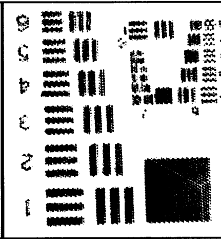
Figure 4. Galileo 5\mu\text{m} pore MCP illuminated with an Air Force test mask pattern.
