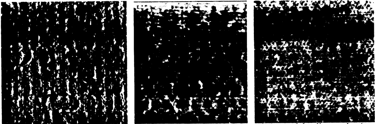
Figure 6. High resolution flat field images of 12.5 \mu\text{m} pore MCP Z stack (cross delay line readout). a) Multifibers aligned b) Multifibers rotated 7.3° c) Multifibers rotated 20°
