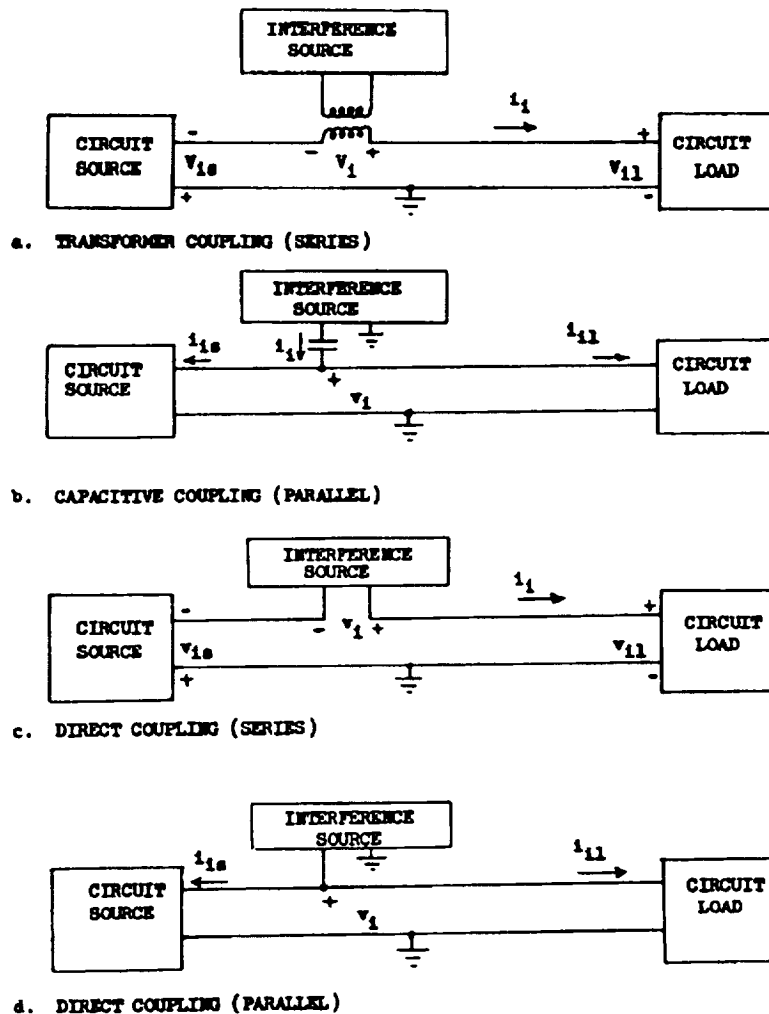
Figure B.2-1. Susceptibility Test Methods.
