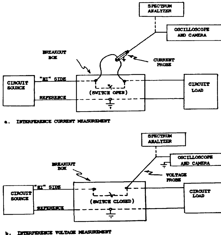
Figure B.2-2. Interference Measurement Methods.
