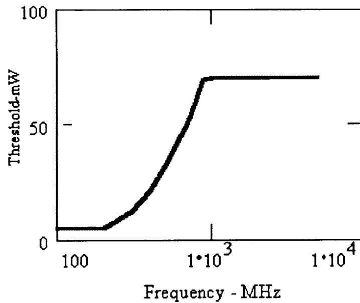
Figure 3-7. Line Receiver Susceptibility.
