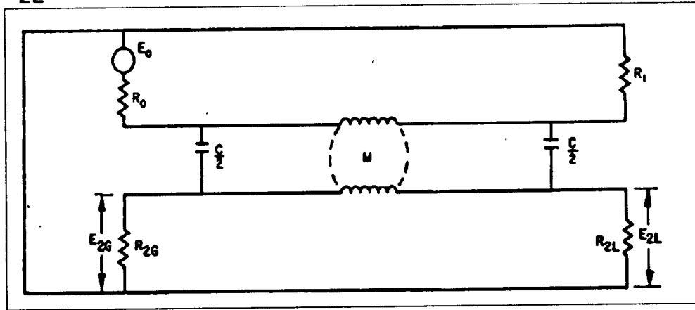
Model of wire-to-wire noise coupling
