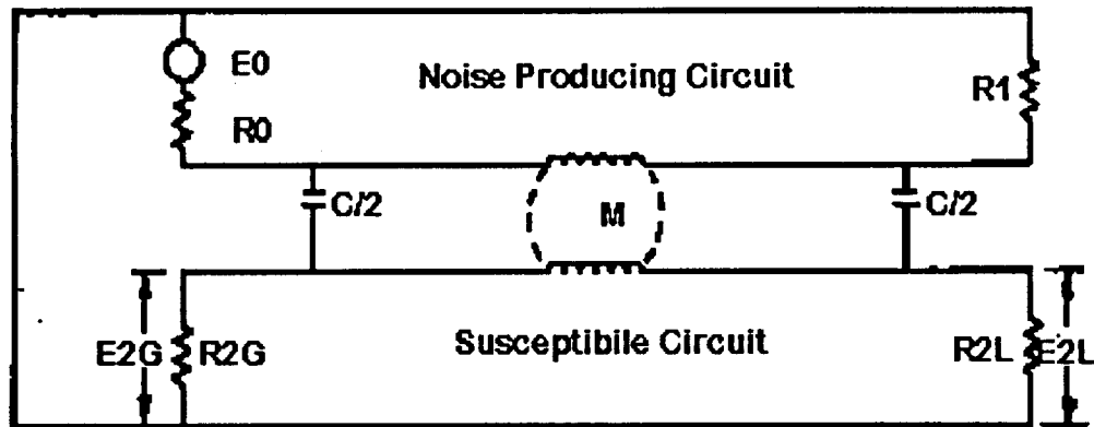
Figure 3-1. Wire to Wire Coupling.
