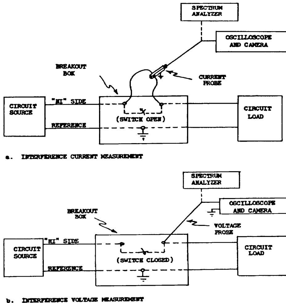
Figure 4-2. Interference Measurement Methods.
