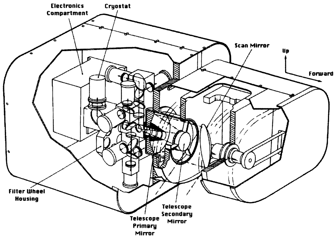
Figure 1. Cutaway drawing of CAR. The dimension of the instrument housing is 72\ \text{cm} \times 41\ \text{cm} \times 39\ \text{cm} .
