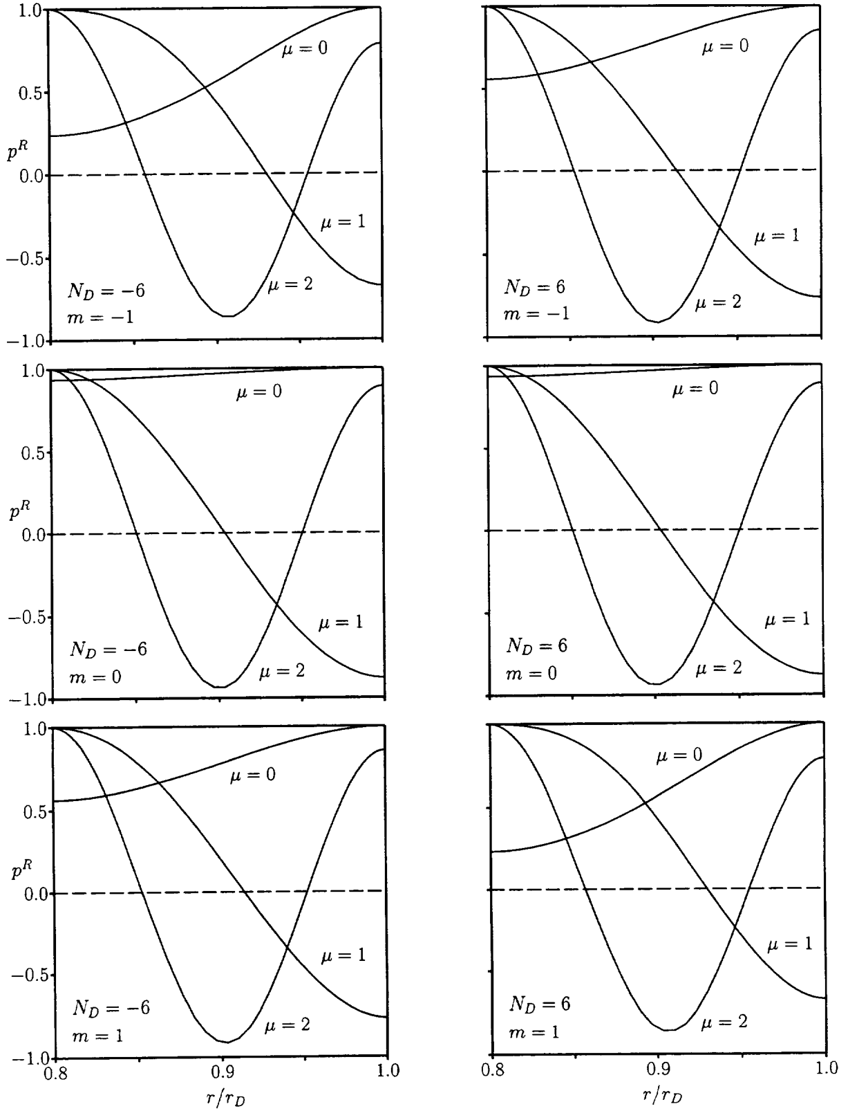
Figure 6: Radial pressure modes, p_{m\mu}^R(\tau) , m = -1, 0, 1 , \mu = 0, 1, 2 , for acoustic disturbances at N_D = \mp 6 in the far field of the helical fan.
