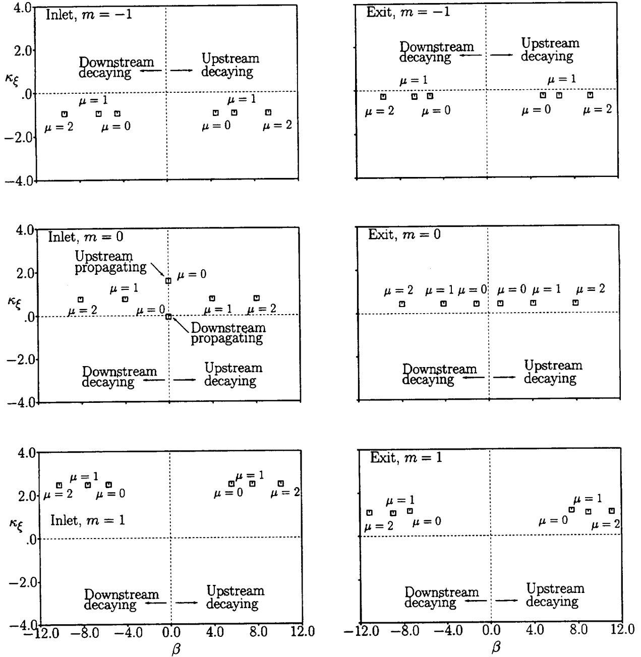
Figure 25: Axial eigenvalues, \chi = \beta + i\kappa_\xi , for three circumferential ( m = -1, 0, 1 ) and three radial ( \mu = 0, 1, 2 ) modes of acoustic disturbance far upstream and far downstream of the 3D 10th Standard Cascade, for an unsteady flow at \omega = 1.0 and N_D = 6 .
