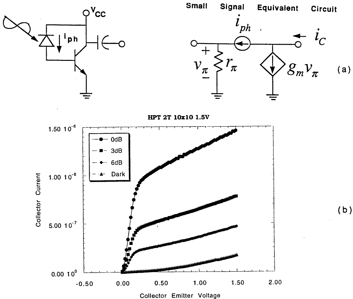
Figure 3 Equivalent circuit (a) and optical response characteristics (b) for an HPT with 10\text{ }\mu\text{m} \times 10\text{ }\mu\text{m} emitter operated in two terminal configuration (base floating).
