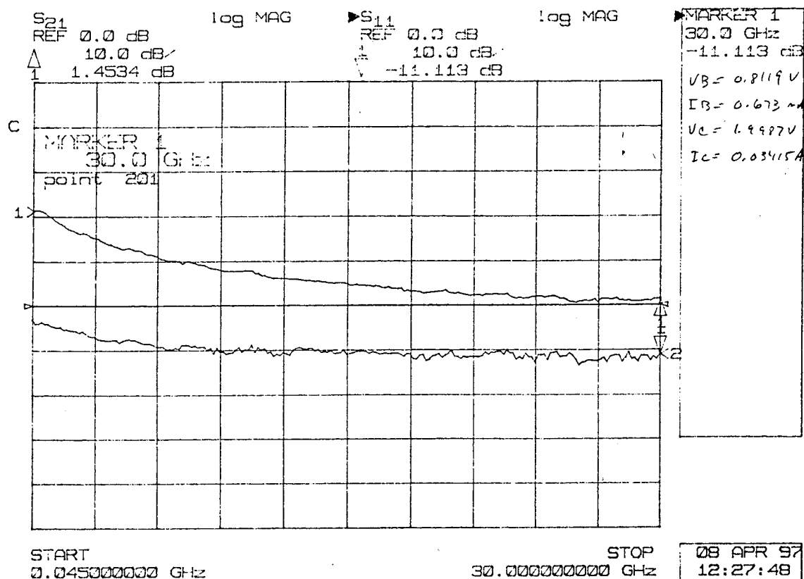
Figure 9 Microwave results for a large 100 \mu\text{m} x 100 \mu\text{m} emitter HBT showing a cutoff frequency of 30 GHz.
