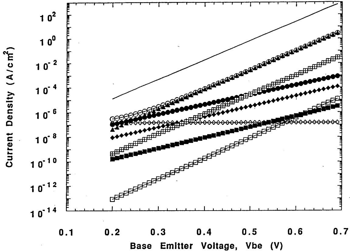
Figure 20 Gummel plot of total collector J_c (no symbol) and base J_b (O) current density and base recombination current components (nonradiative J_{br} ( \blacktriangle ), radiative J_r ( \square ), surface J_{sr} ( \bullet ), interface J_{ir} ( \blacklozenge ), space charge region J_{scr} ( \blacksquare ), hole back injection J_{ep} ( \square ), and collector hole J_{cp} ( \diamond )) versus emitter-base bias for the device of Chandrasekhar et al. [21] for no optical illumination ( F_o=0 ).
