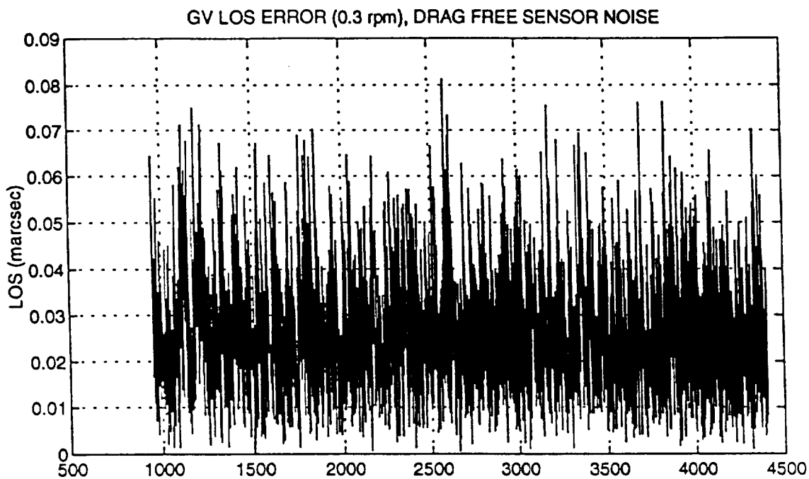
Figure 3-15 LOS Error (.3 rpm, GSV and GSI, Drag Free Sensor Noise)
