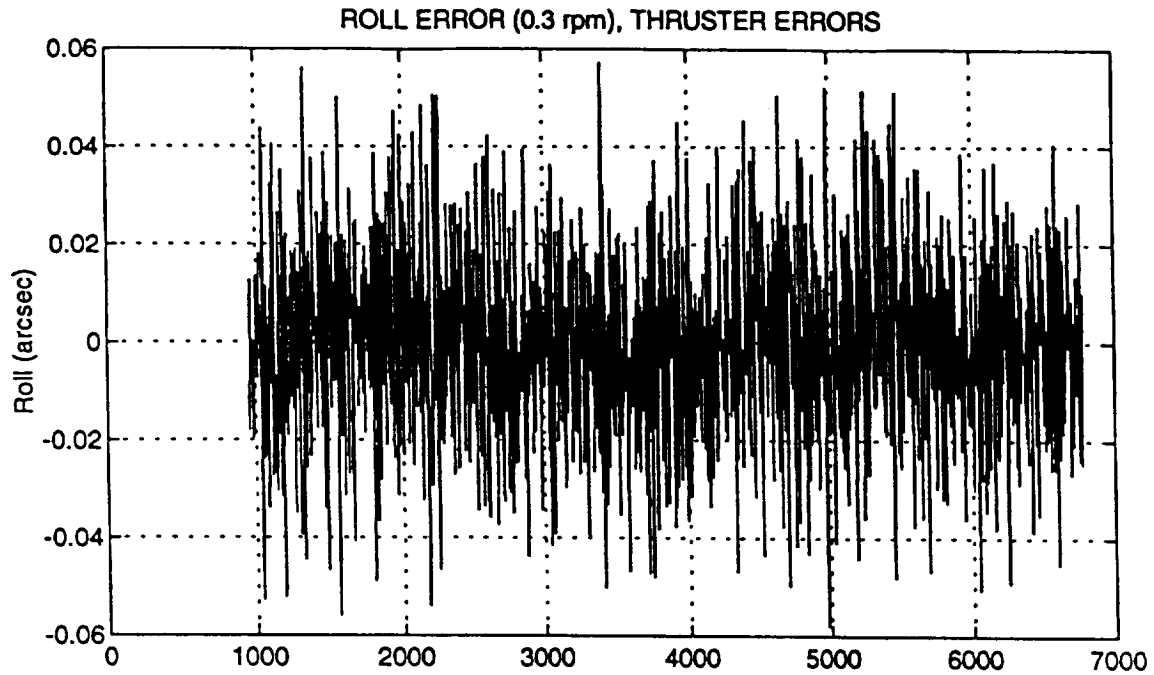
Figure 3-4 Roll and Translational Error (.3 rpm, Thruster Errors)
