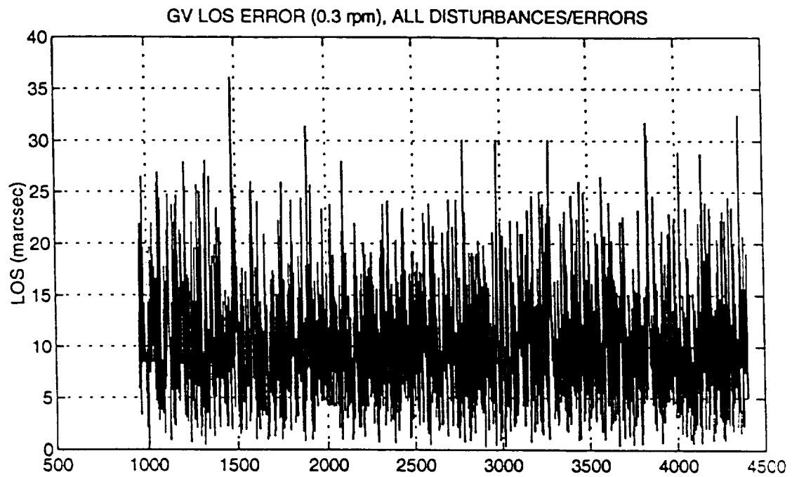
Figure 3-19 LOS Error (.3 rpm, GSV and GSI, All Disturbances and Errors)
