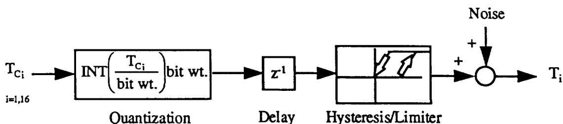
Figure 2.1.2-1 Thruster Model
