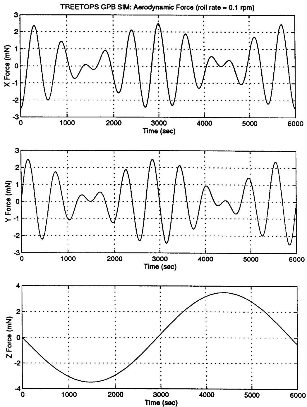
Figure 2.2-2 Aerodynamic Disturbance Force
