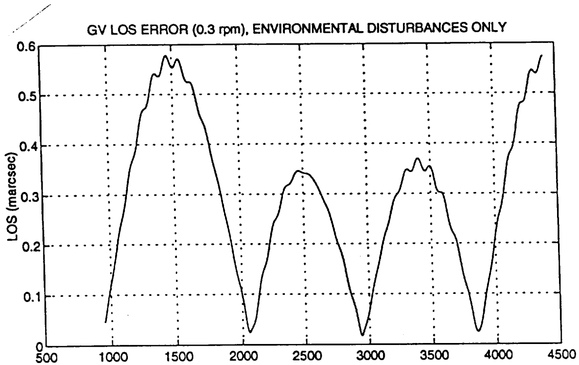
Figure 3-1 LOS Error (.3 rpm, GSV and GSI, Environmental Dist Only)
