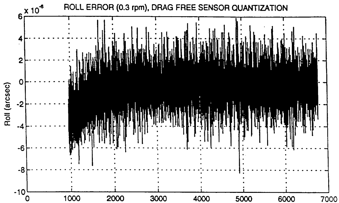
Figure 3-18 Roll and Translational Error (.3 rpm, Drag Free Sensor Quantization)
