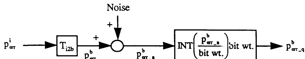
Figure 2.1.1-4 Drag Free Sensor Model
