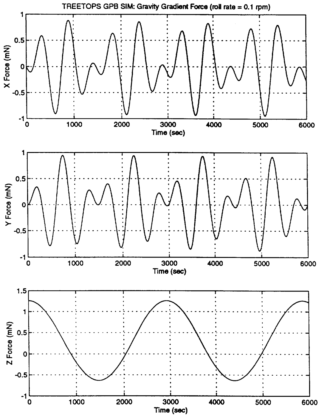
Figure 2.2-4 Gravity Gradient Disturbance Force
