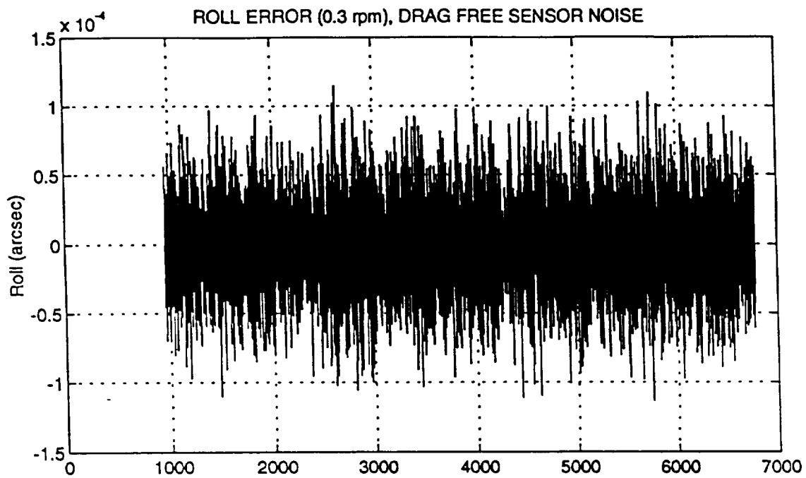
Figure 3-16 Roll and Translational Error (.3 rpm, Drag Free Sensor Noise)
