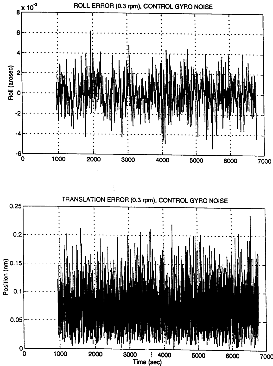
Figure 3-12 Roll and Translational Error (.3 rpm, Control Gyro Noise)
