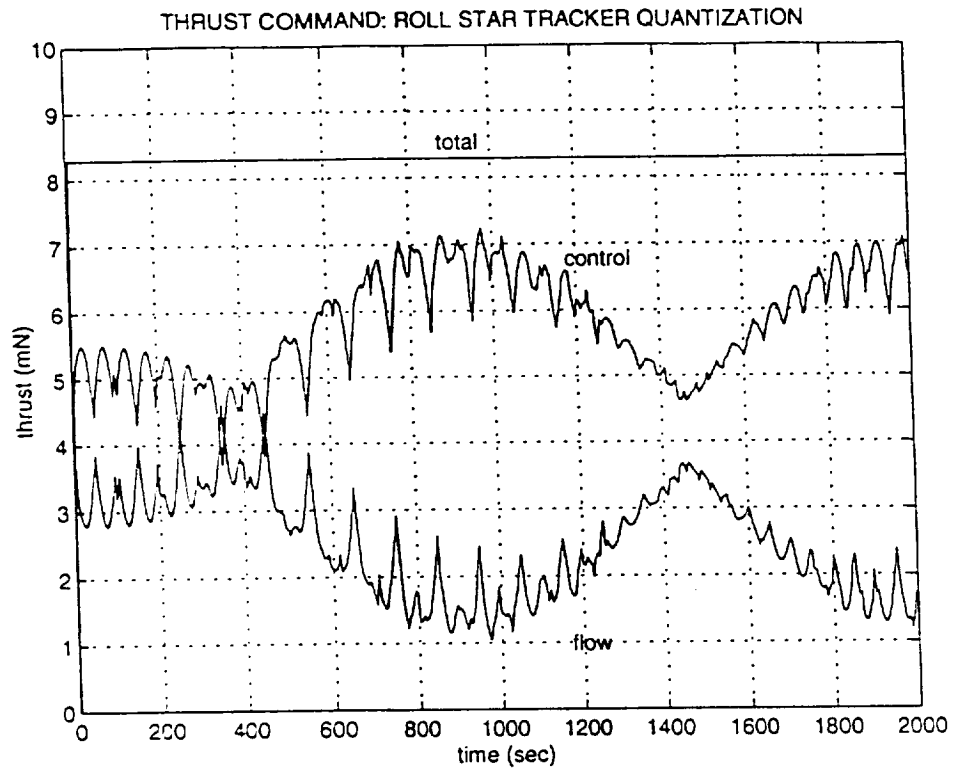
Figure 3.1-7 Thrust Command For Roll Star Tracker Quantization
