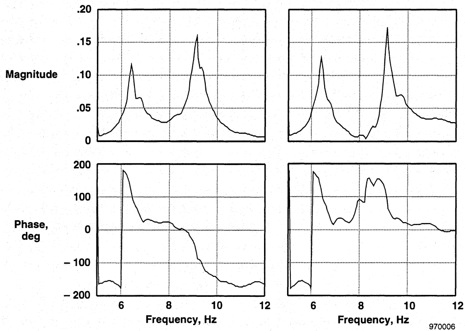
(b) Corresponding time-frequency generated transfer function.
