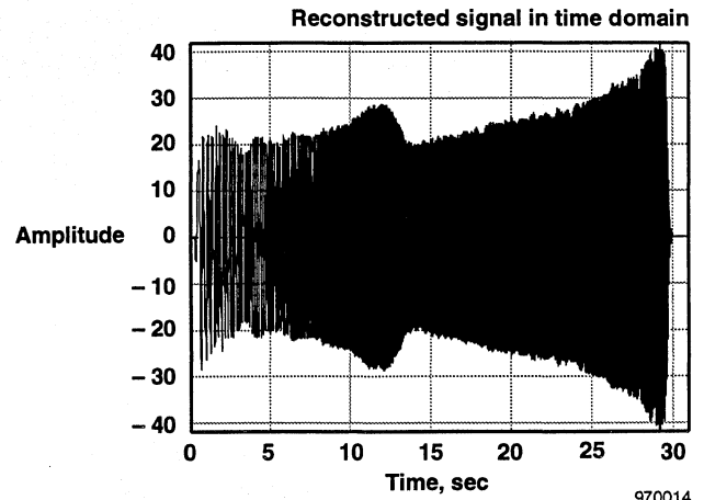
(b) Reconstructed signal of cleaned accelerometer response.
