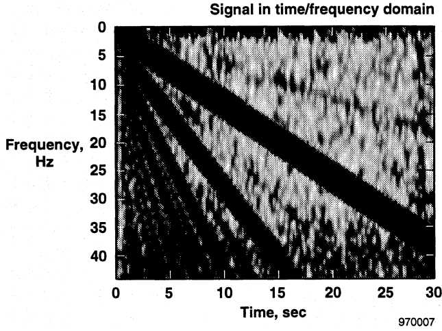
(a) Morlet continuous wavelet transform.
