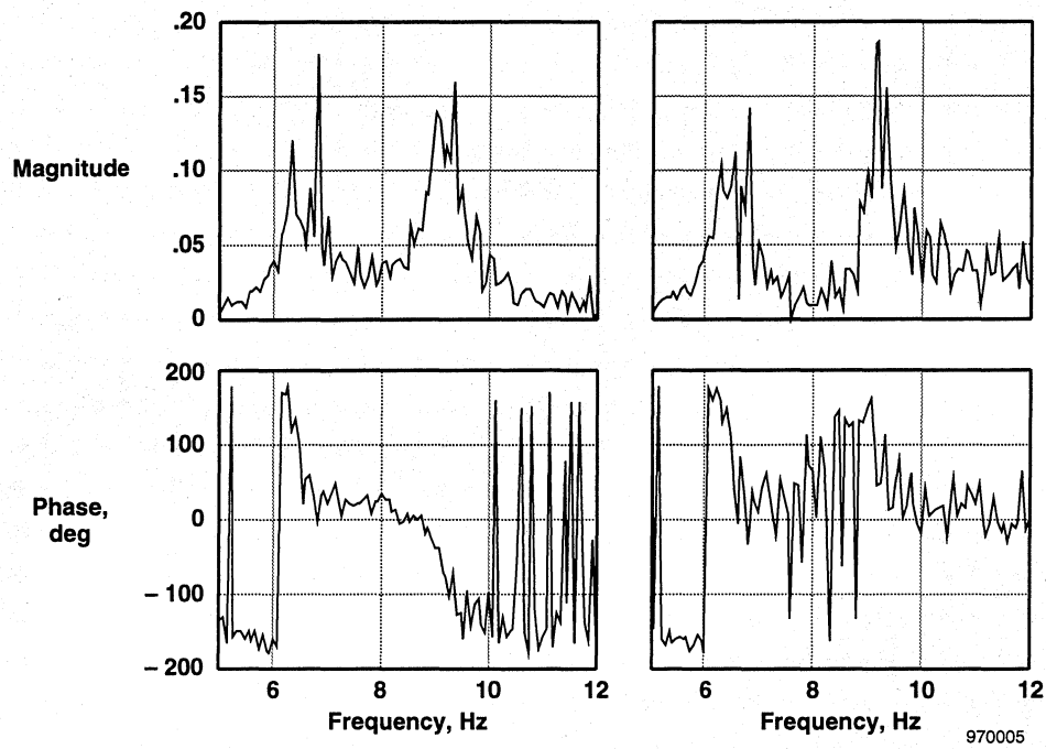
(a) Classical Fourier transfer functions.
