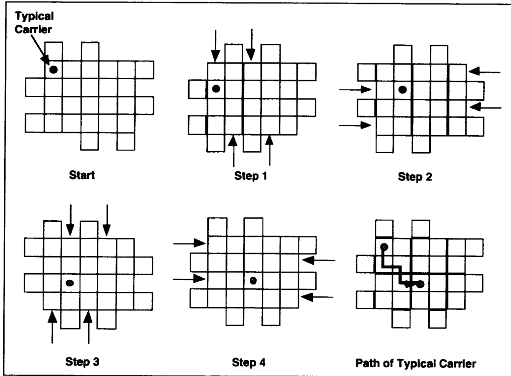
Figure 2-5. Four-step braiding process.
