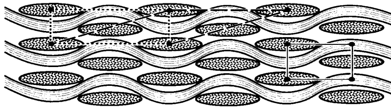
Figure 5-3. Alternative unit cells (short and long dash lines at upper left) in a plane woven laminate. The smaller, solid-lined rectangle (lower right) shows a reduced cell that takes advantage of reflection symmetry about a vertical plane.
