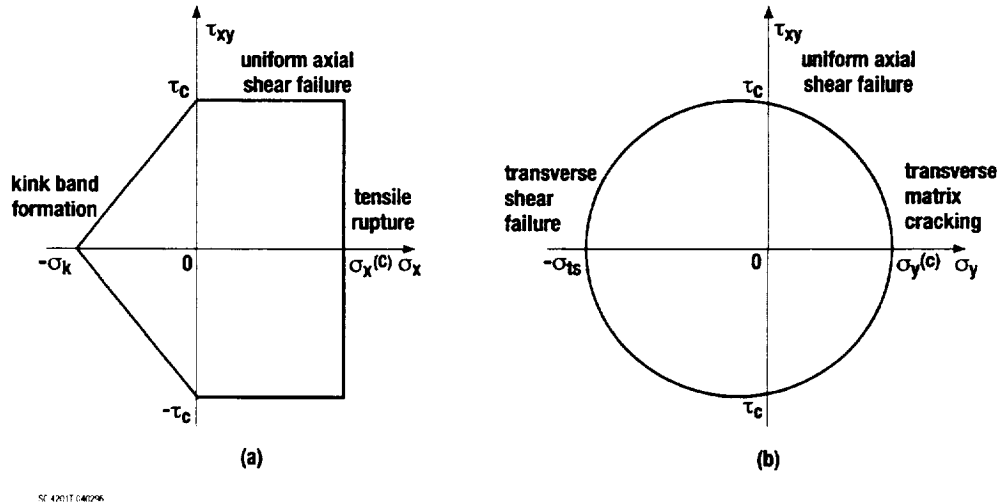
Figure 6-2. Failure loci for individual tows or plies in terms of the local stress state. (a) Combined aligned and axial shear loads. (b) Combined transverse and axial shear loads. The x -axis is aligned with local fiber direction. The axes are not to scale.
