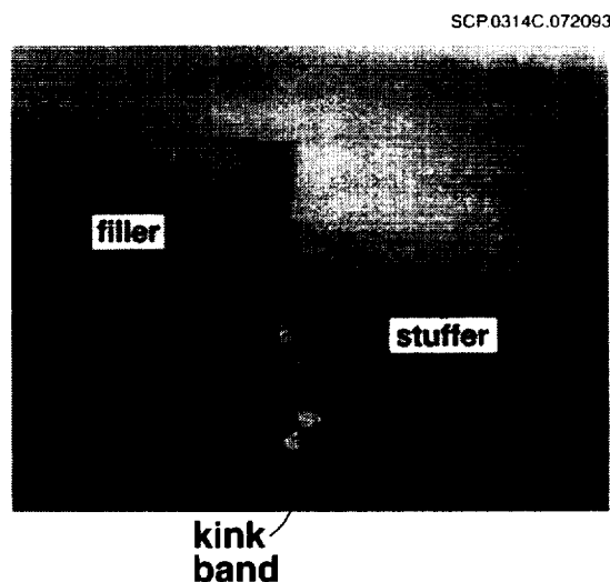
Figure 4-11. A kink band formed in fatigue in a misaligned segment of a stuffer in an AS4/1895 layer-to-layer interlock weave (from [4.37]).
