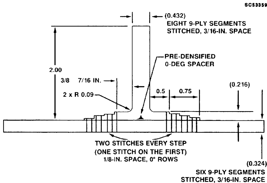
Figure 2-26. A stitched skin/stiffener assembly. (From Ref. [2.30])
