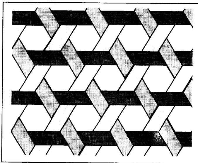
Figure 2-12. Triaxial weave.
