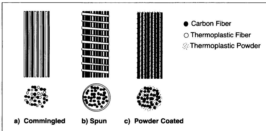
Figure 2-9. Techniques for using thermoplastics in textiles.
