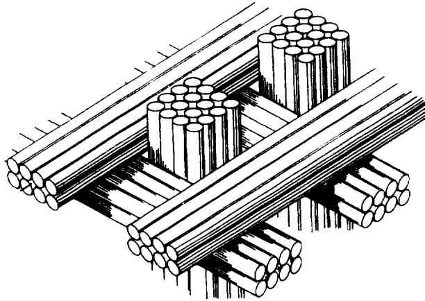
Figure 2-15. 3D orthogonal composite.
