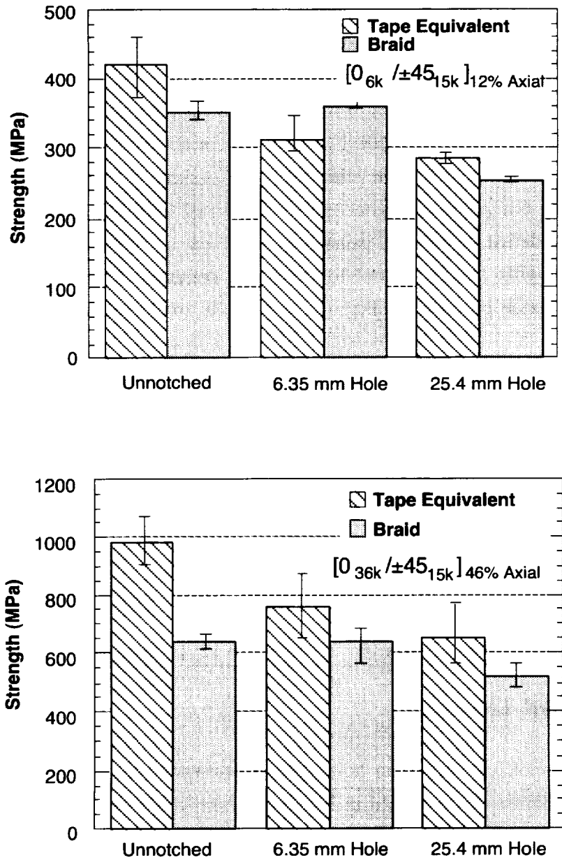
Figure 3-4. Comparison of unnotched and open hole tensile strengths for two triaxial braids and equivalent tape laminates (from [3.7]).
