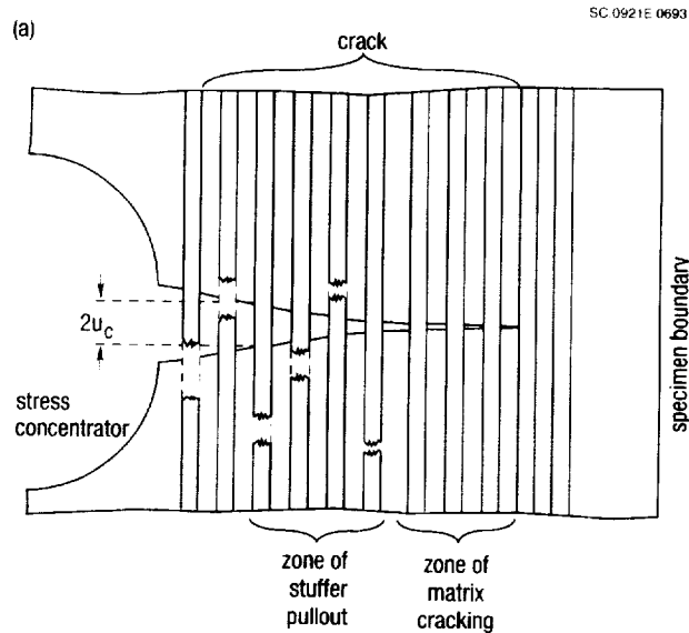
Figure 4-10. Schematic of a nonlinear damage band growing from a stress concentrator in a textile composite.
