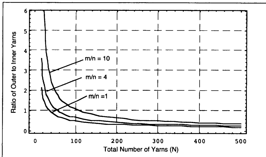
Figure 2-20. Ratio of outer (surface) yarns to inner yarns.
