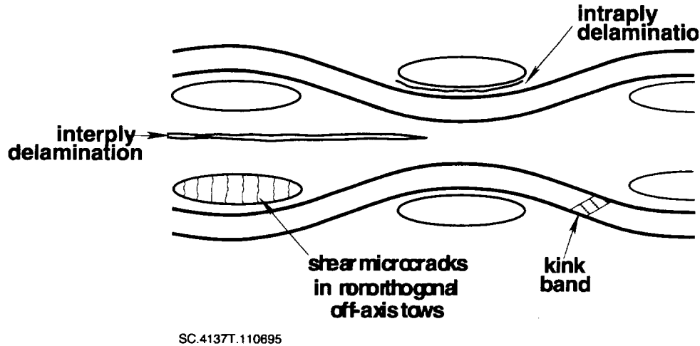
Figure 4-5. Schematic of delamination and shear failure events in a typical 2D weave.
