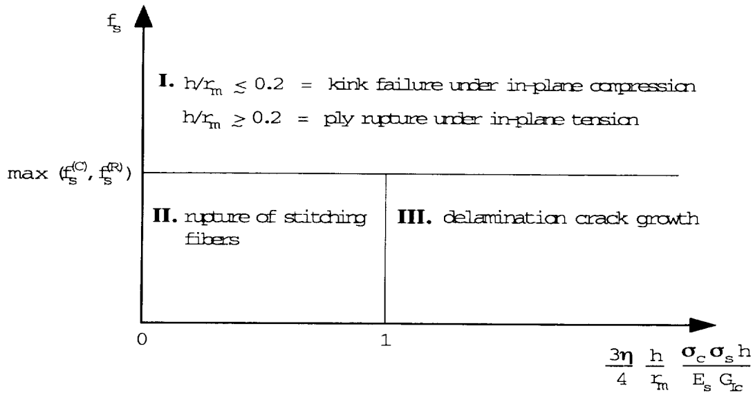
Figure 4-9. Map of failure modes for a curved panel. The transition from failure on the compressive side to failure on the tensile side in Domain I depends on the relative values of the critical stresses for tensile rupture and kinking. The critical value of h/r_m shown corresponds to a tensile rupture stress that is 50% higher in magnitude than the kinking stress.
