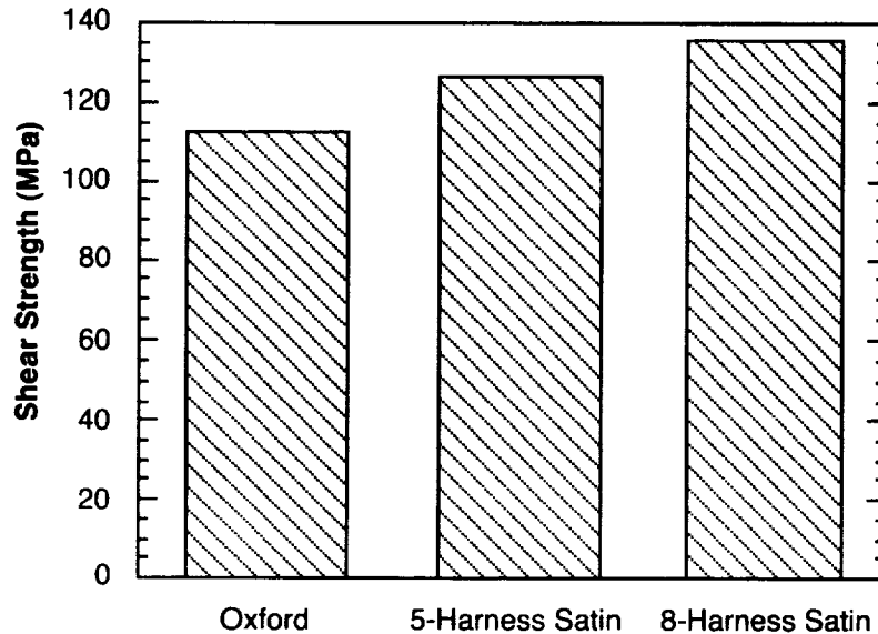
Figure 3-3. Comparison of in-plane shear strengths of various T300/934 weaves, showing effect of crimp. (From [3.6].)
