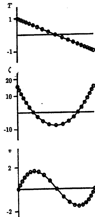
(d) Natural convection; V_0 = 0, \frac{g\beta h^2 T_w}{\nu} = 100
