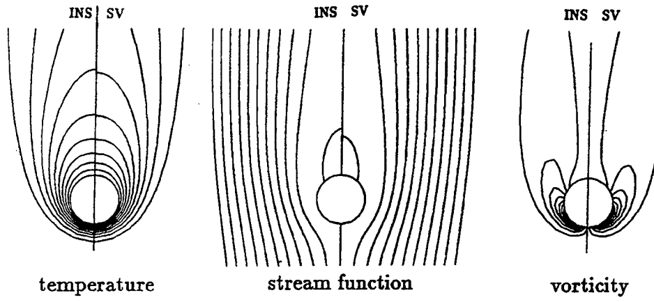
(a) Forced convection ( Re = 20 , Gr = 0 )
