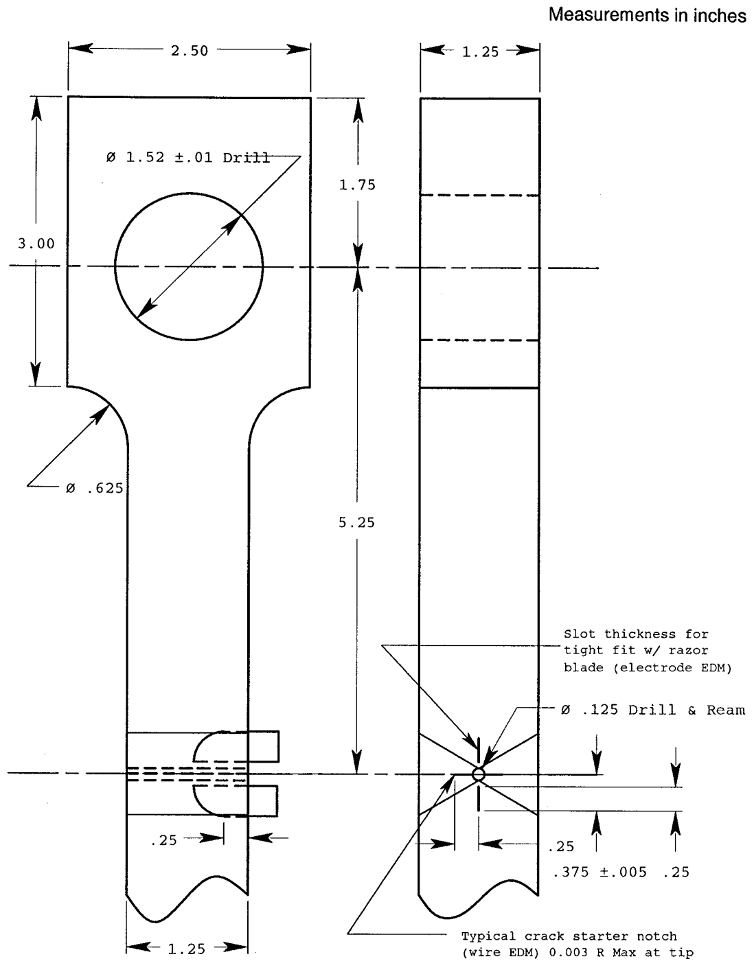
Figure A-5: Center cracked panel tension specimen.
