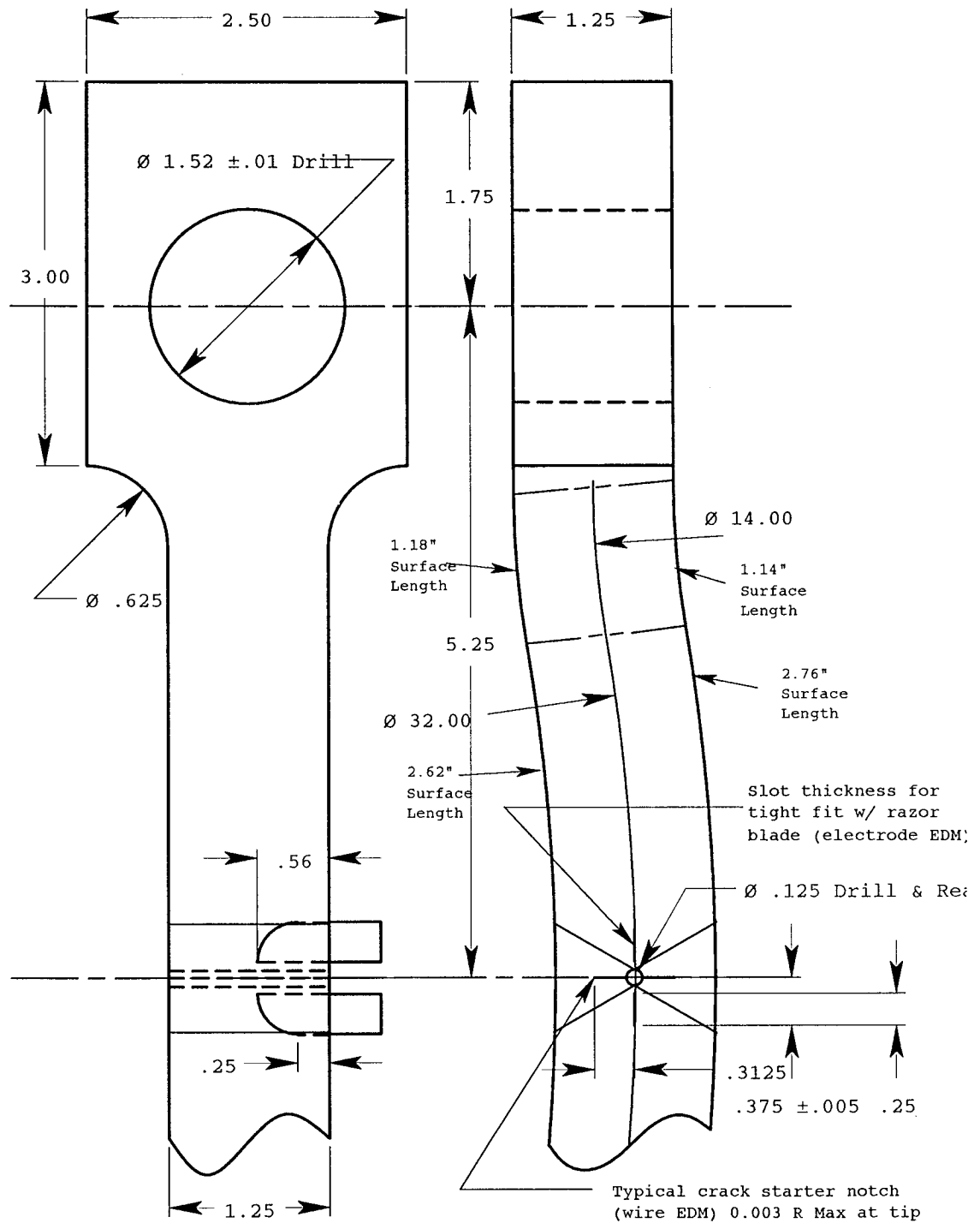
Figure B-2: Center cracked panel tension plus bending specimen.
