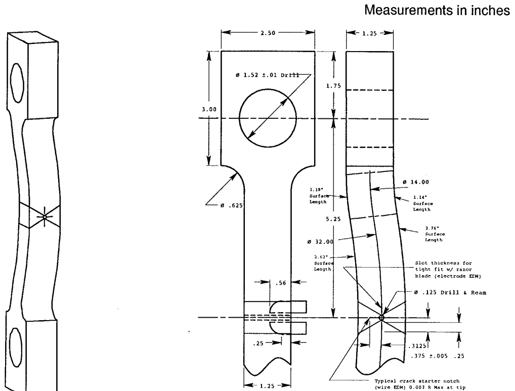
Figure 37: Center cracked panel specimen for tension plus bending loading. (Figures appear larger in Appendix A for clarity.)
