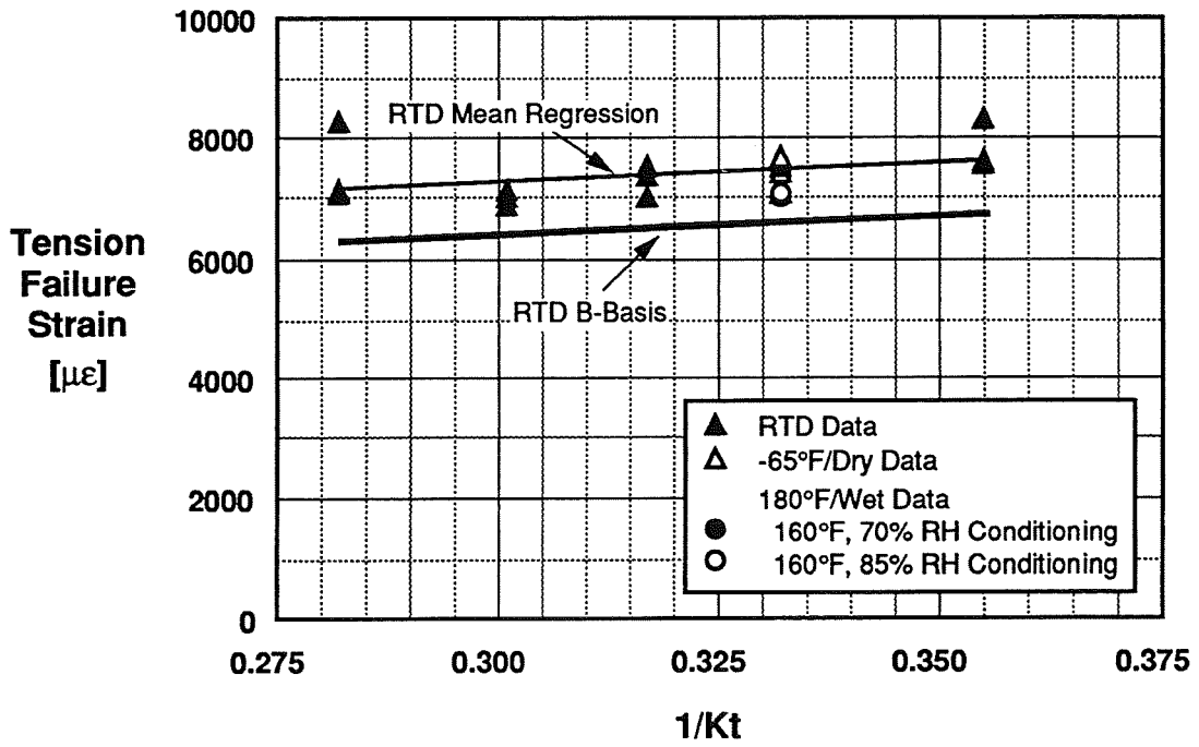
Figure D-9: Open hole tension failure strains vs. inverse of stress concentration factor.
