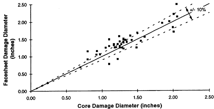
Figure 6-3. Comparison of Planar Extent of Impact Damage in Sandwich Facesheet and Core Materials. The Line Represents Equal Damage in Facesheet and Core.
