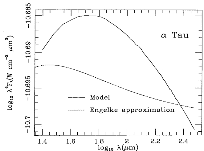
FIG. 6. Far-infrared model continuum extrapolation (solid line) of our \alpha Tau composite, compared with the extrapolated Engelke approximation (short dashed line) for this star. The maximum difference between these two spectra occurs near 65 \mu\text{m} , where it attains almost 2%.
