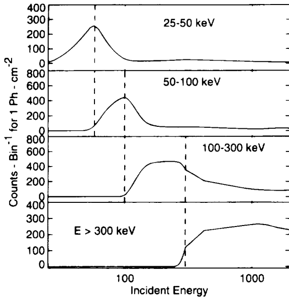
FIG. 5.—Plot of the DRM for LAD 2. The response is displayed in the four LAD discriminator channels as a function of incident photon energy. The vertical dashed lines indicate the energy boundaries of each output channel.
