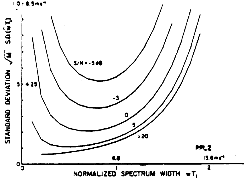
Figure 20. A plot of the normalized standard deviation associated with the width estimator derived assuming a Gaussian shape and using autocorrelation lags one and two. (Source: ©1979 IEEE, Zrnic, "Spectrum Width Estimates for Weather Echos", IEEE Trans. on AES, September 1979.)
