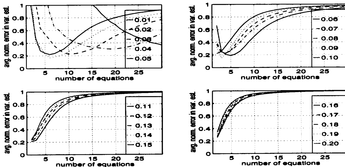
Figure C-8. The averaged normalized error in the variance estimate for the 5 dB SNR case using the [1 \ 2] estimator in an overdetermined system.
