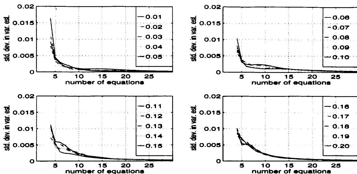
Figure D-11. The standard deviation in the variance estimate for the 5 dB SNR case using the [0 \ 1 \ 2 \ 3] estimator in an overdetermined system.
