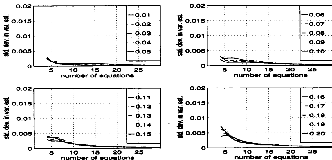
Figure D-6. The standard deviation in the variance estimate for the 10 dB SNR case using the [1 \ 2 \ 3 \ 4] estimator in an overdetermined system.
