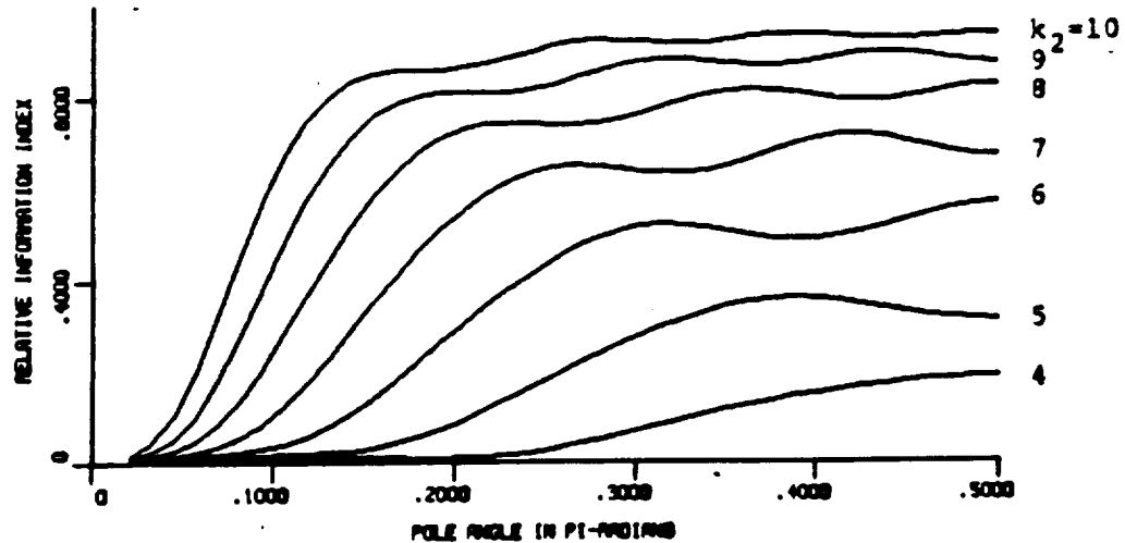
Figure 10. A plot of the RII for the AR(2) model with a pole magnitude of 0.95 (narrowband) as a function of the number of lags used in the estimate and the pole angle in radians. (Source: ©1984 IEEE, Bruzzone and Kaveh, "Informaiton Tradeoffs in Using the Sample Autocorrelation Function in ARMA Parameter Estimation", IEEE Trans. on ASSP, August 1984.)
