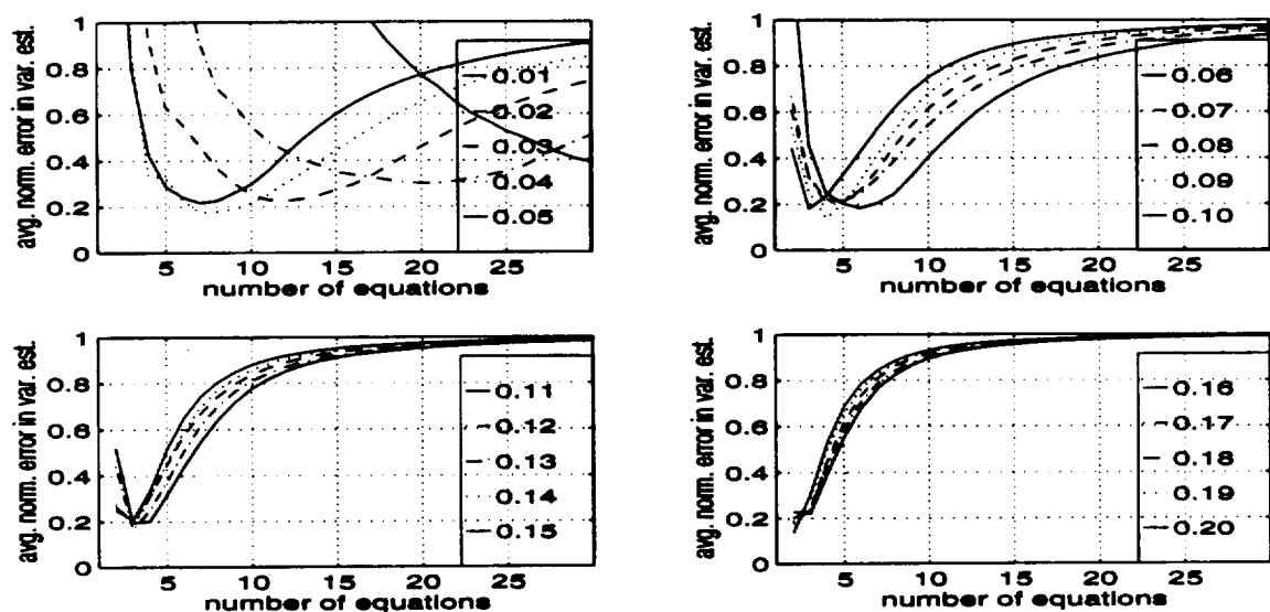
Figure 31. The averaged normalized error in the variance estimate for the 5 dB SNR case using two terms in the overdetermined system.
