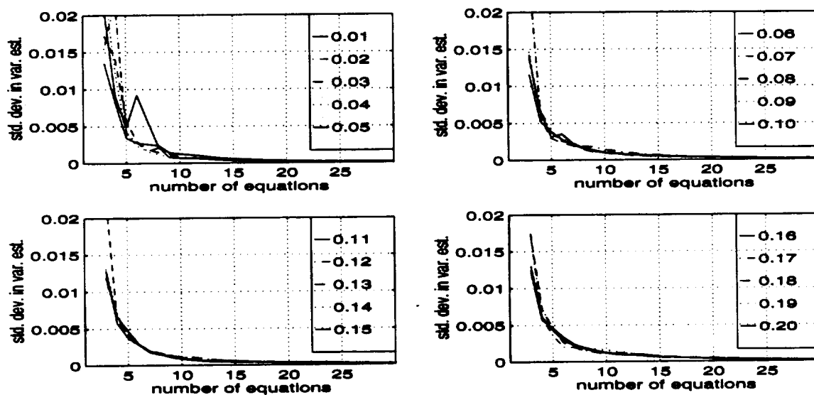
Figure D-16. The standard deviation in the variance estimate for the 0 dB SNR case using the [1 \ 2 \ 3] estimator in an overdetermined system.
