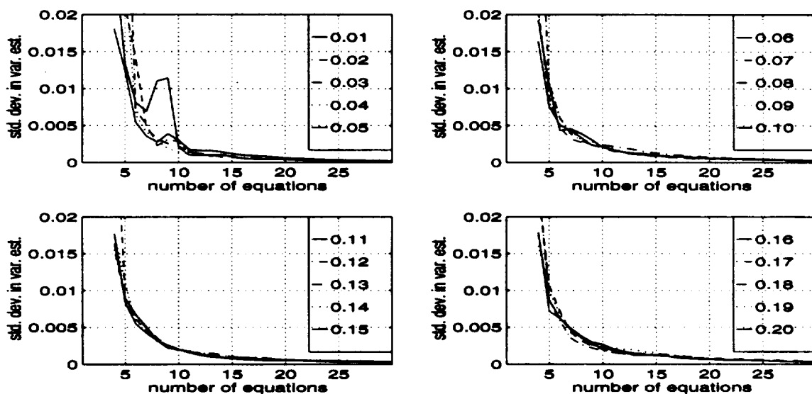
Figure D-18. The standard deviation in the variance estimate for the 0 dB SNR case using the [1 \ 2 \ 3 \ 4] estimator in an overdetermined system.
