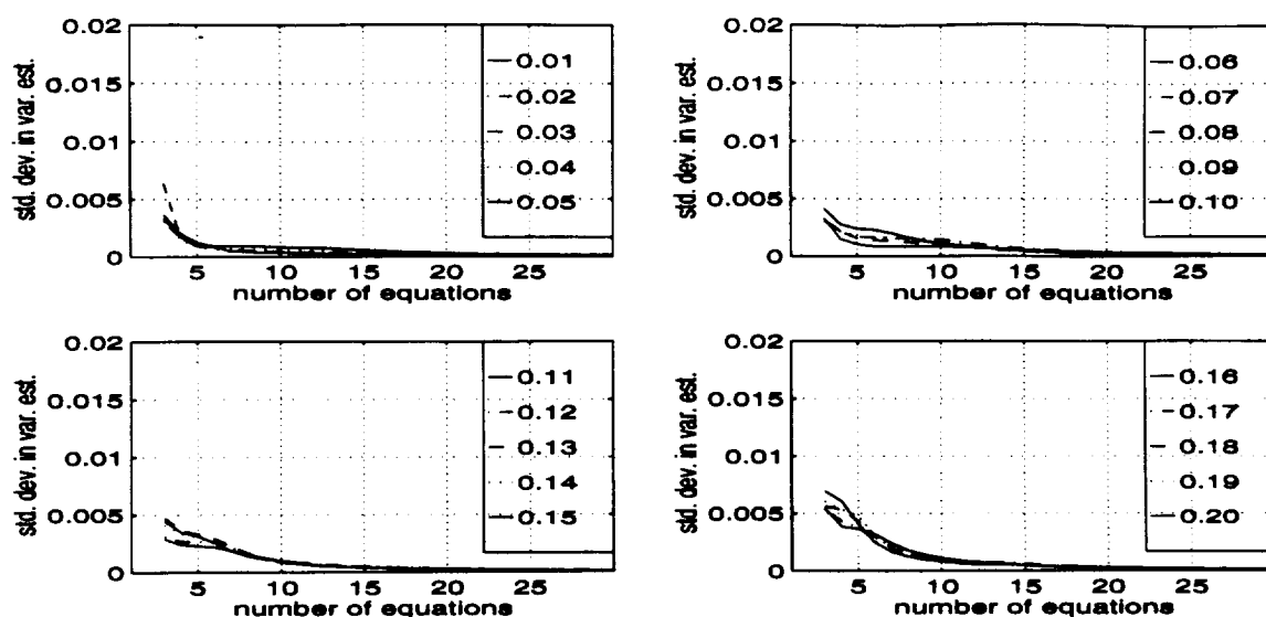
Figure D-3. The standard deviation in the variance estimate for the 10 dB SNR case using the [0 \ 1 \ 2] estimator in an overdetermined system.
