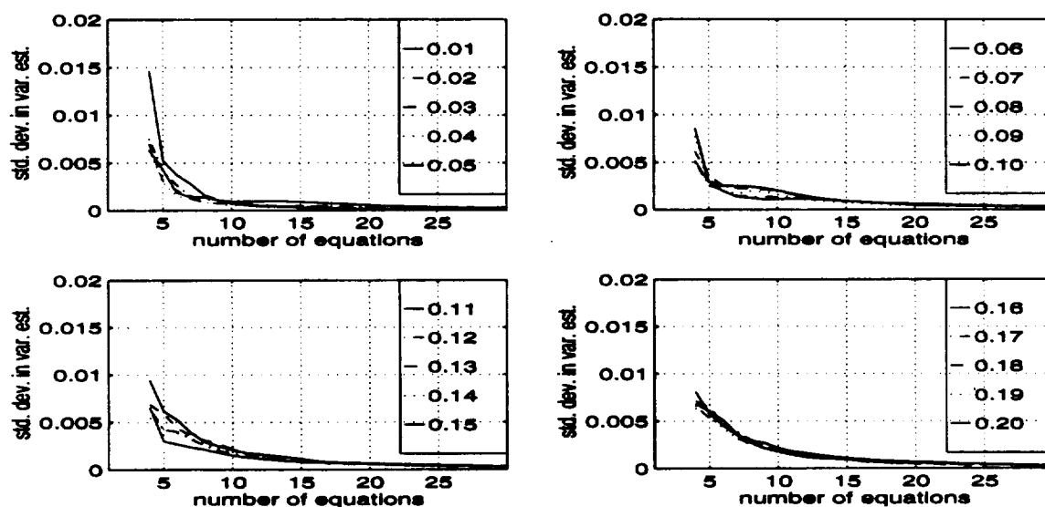
Figure D-12. The standard deviation in the variance estimate for the 5 dB SNR case using the [1 \ 2 \ 3 \ 4] estimator in an overdetermined system.
