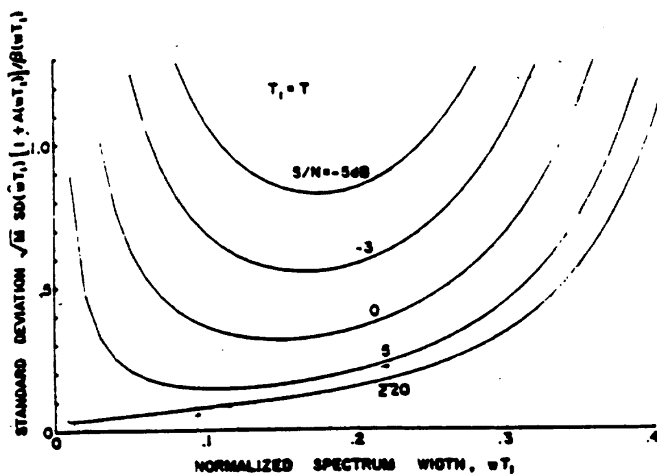
Figure 16. A plot of the normalized standard deviation associated with the pulse-pair width estimator. (Source: ©1977 IEEE, Zrnic, "Spectral Moment Estimates from Correlated Pulse Pairs", IEEE Trans. on AES, July 1977.)
