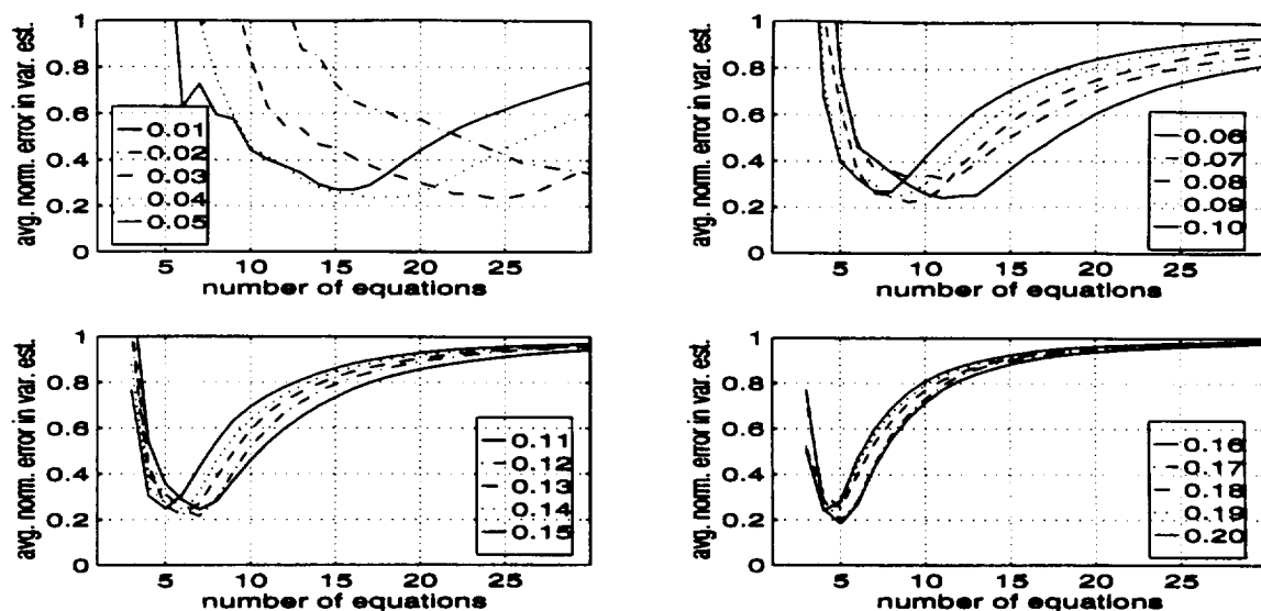
Figure C-15. The averaged normalized error in the variance estimate for the 0 dB SNR case using the [0 \ 1 \ 2] estimator in an overdetermined system.
