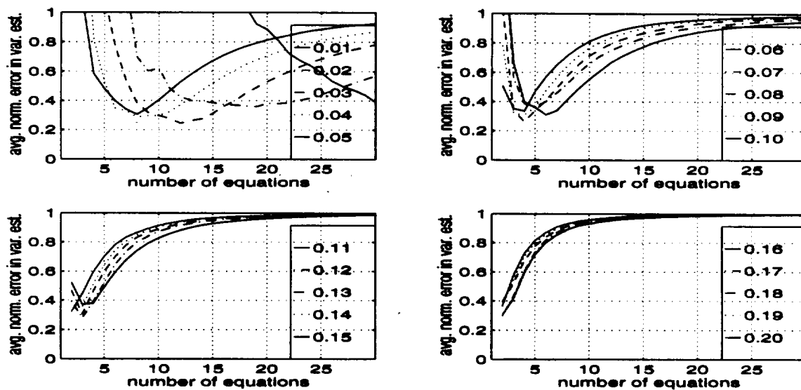
Figure C-14. The averaged normalized error in the variance estimate for the 0 dB SNR case using the [1 \ 2] estimator in an overdetermined system.
