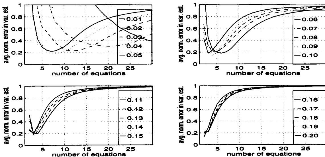
Figure C-7. The averaged normalized error in the variance estimate for the 5 dB SNR case using the [0 \ 1] estimator in an overdetermined system.
