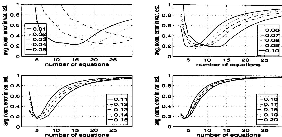
Figure C-9. The averaged normalized error in the variance estimate for the 5 dB SNR case using the [0 \ 1 \ 2] estimator in an overdetermined system.
