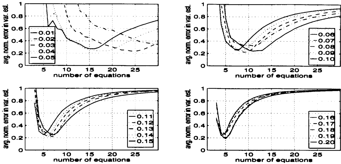
Figure 34. The averaged normalized error in the variance estimate for the 0 dB SNR case using three terms in the overdetermined system.
