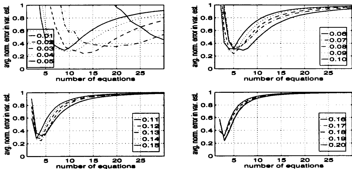
Figure 33. The averaged normalized error in the variance estimate for the 0 dB SNR case using two terms in the overdetermined system.
