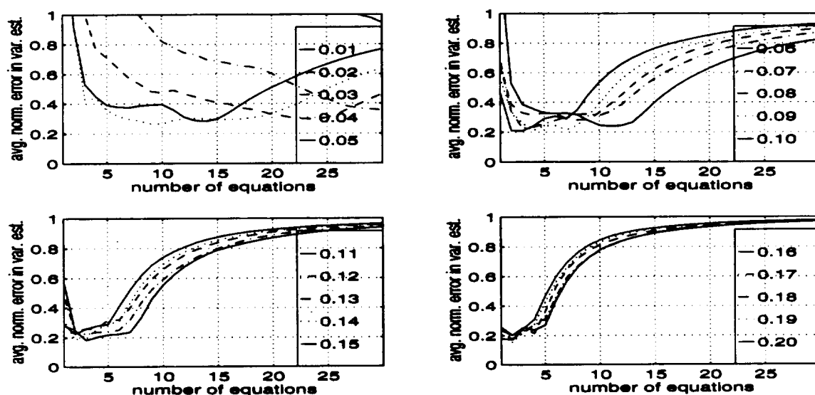
Figure 35. The averaged normalized error in the variance estimate for the 5 dB SNR Gaussian case.
