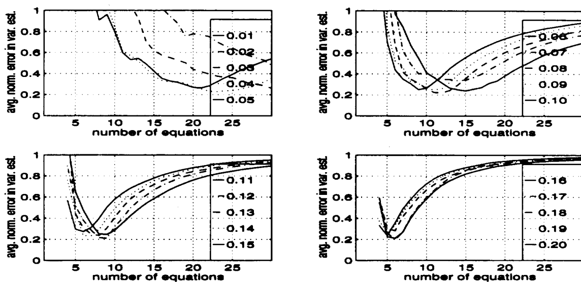
Figure C-18. The averaged normalized error in the variance estimate for the 0 dB SNR case using the [1 \ 2 \ 3 \ 4] estimator in an overdetermined system.
