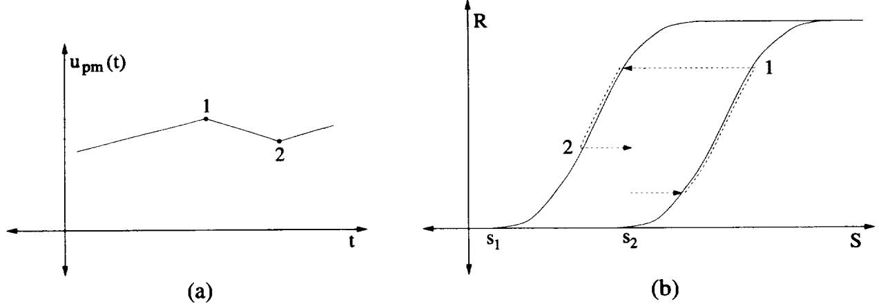
Figure 7. (a) Piecewise monotone input; (b) Output from the Krasnoselskii-Pokrovskii kernel in response to a piecewise monotone input.
