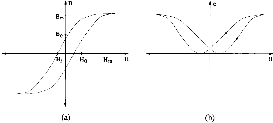
Figure 4. (a) Relationship between the magnetic field strength H and the magnetic flux density B ; (b) Applied magnetic field H and resulting strain distribution \epsilon .
