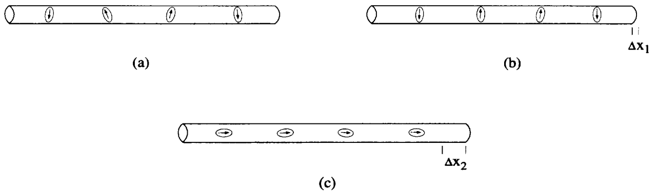
Figure 2. Magnetic domains in the Terfenol-D rod; (a) Orientation of moments within domains in unstressed rod with no applied field; (b) Orientation of moments in prestressed rod with no applied field; (c) Orientation of moments in prestressed rod when field is applied in direction of longitudinal rod axis.
