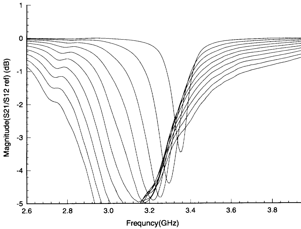
Figure 10(a). x-, y-, and z-offset cases, offsets from .05" to .25", every .025"
