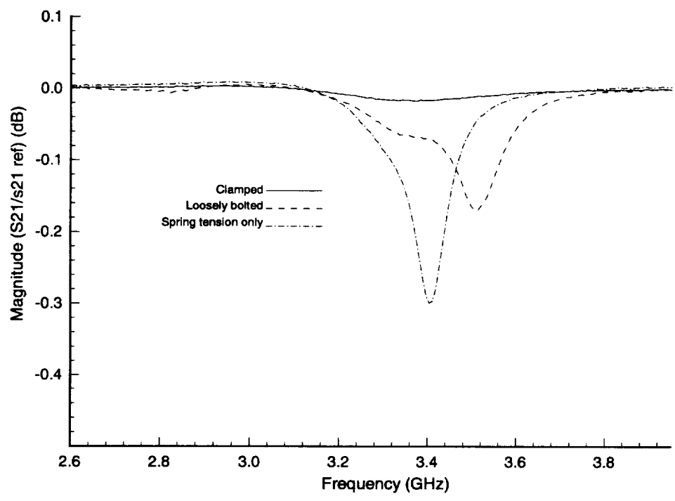
Figure 5. Aligned case
