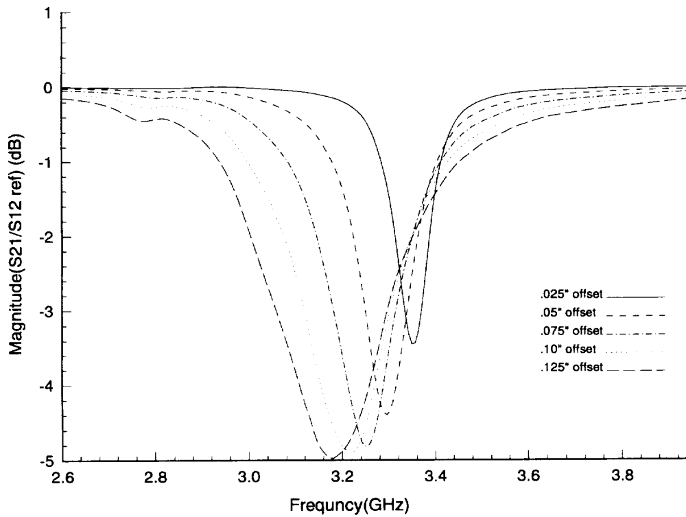
Figure 10(b). x-, y-, and z-offset cases, offsets from .05" to .125", every .025"
