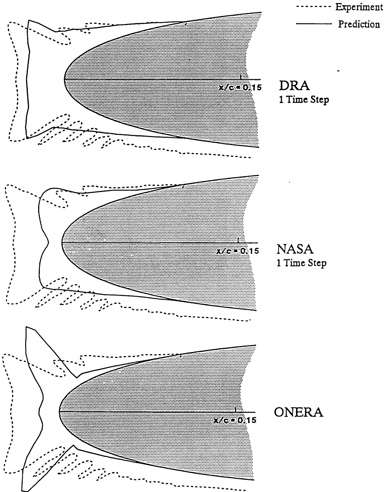
Figure 37 - Comparison of ice shape predictions for DRA cases. NACA0012, Chord = 0.53, \alpha = 0.0 , V_\infty = 130.5 , T_s = -12.3^\circ\text{C} , LWC = 0.5 , MVD = 20.0\mu , \tau = 480.0
