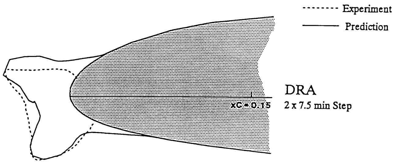
Figure 40B - Comparison of ice shape predictions for ONERA cases.
