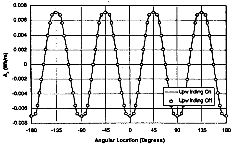
Figure 3.4. Magnetic Vector Potential, A_z , At Rotor Surface For 0 rpm
