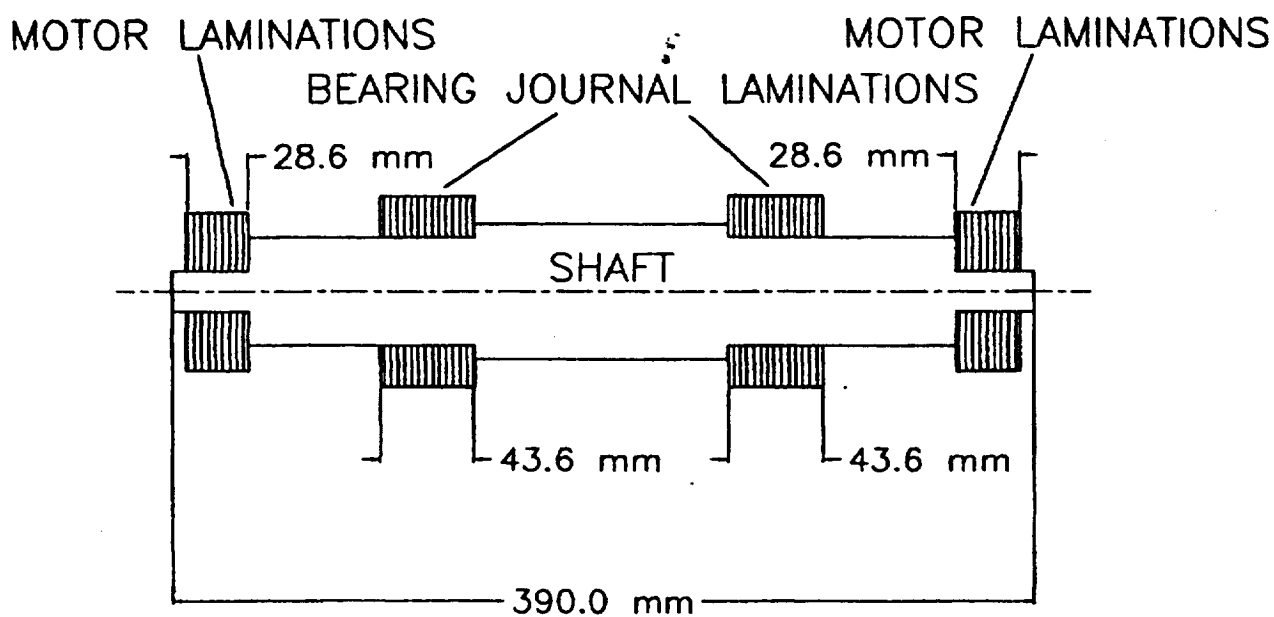
Figure 2.2. Rotor Assembly Drawing
