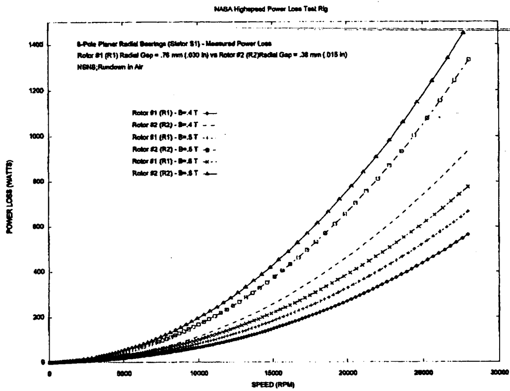
Figure 2.5. Measured Bearing Power Loss Values
