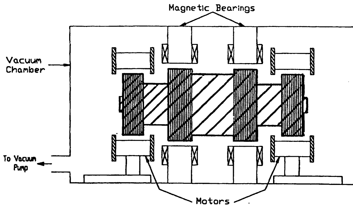
Figure 2.1. Diagram of Magnetic Bearing Loss Test Rig
