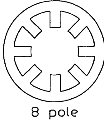
Figure 1.1 Heteropolar Magnetic Bearing Configuration
