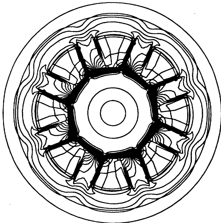
d) 9550 rpm
