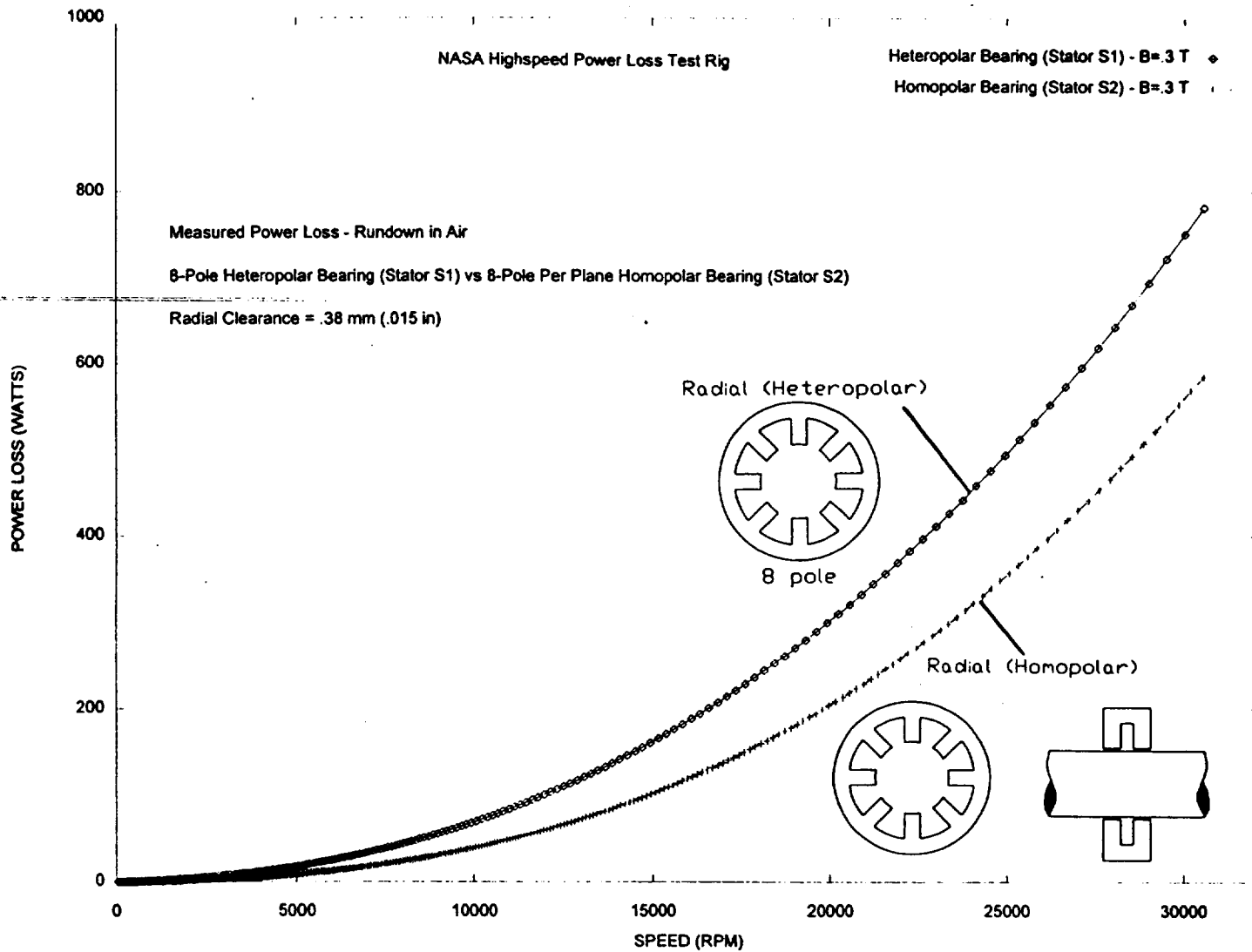
Figure 2.7 Power Loss Data for Homopolar vs. Heteropolar Bearing
