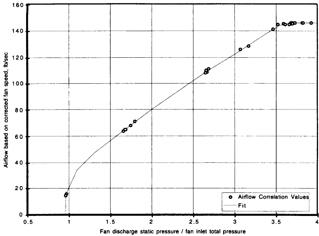
Figure 19. Method 4 flow correlation.
