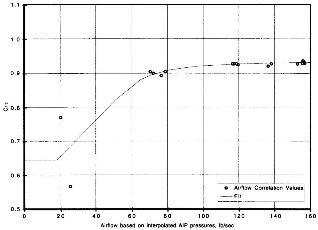
Figure 18. Method 3 flow coefficient relationship.
