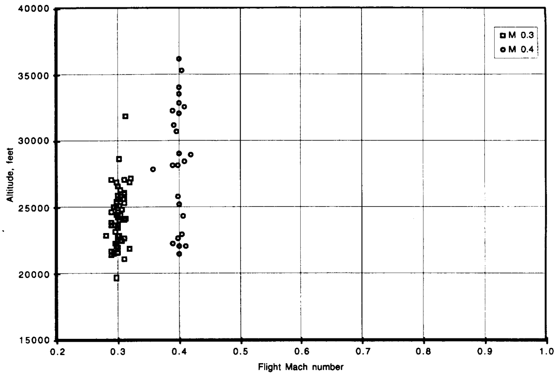
Figure 24. Test range of Mach numbers and altitudes.
