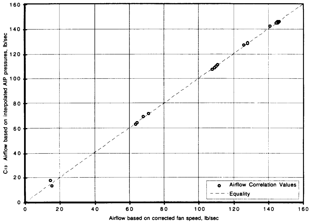
Figure 22. Method 3 calculated airflow as a function of reference method airflow.
