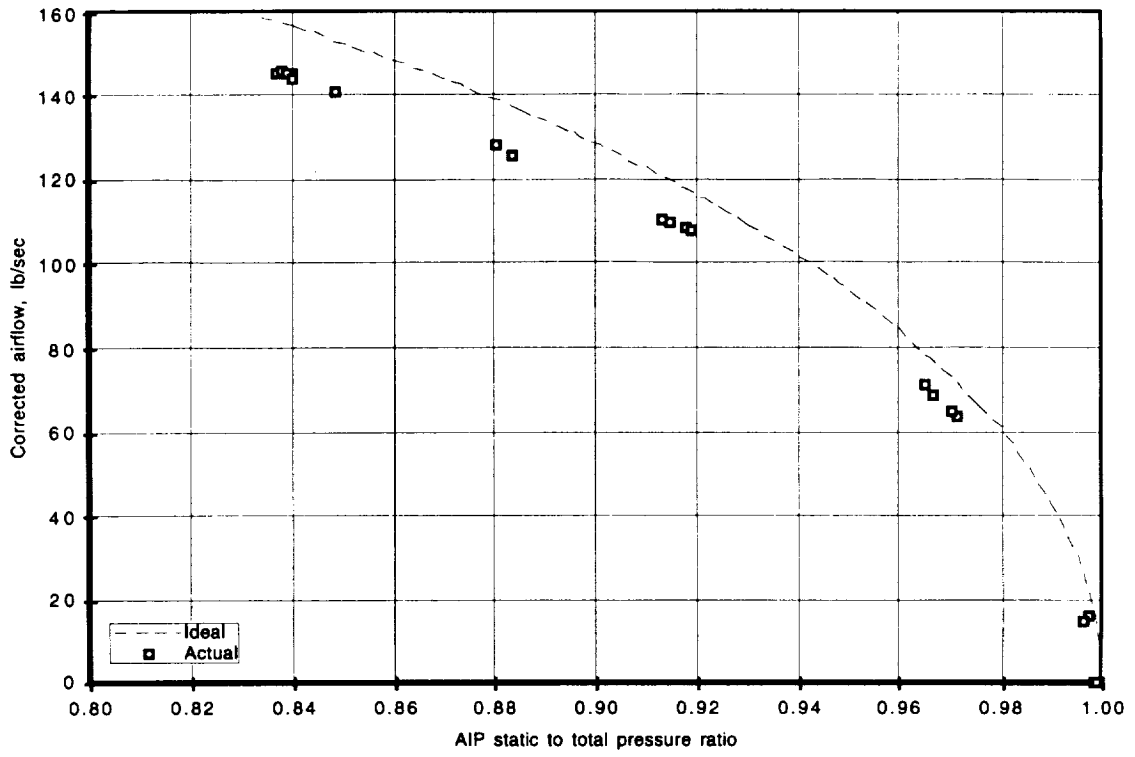
Figure 12. Airflow as a function of AIP static to total pressure ratio.
