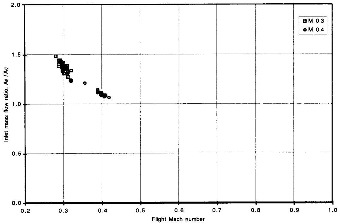
Figure 25. Test range of inlet capture area ratios.
