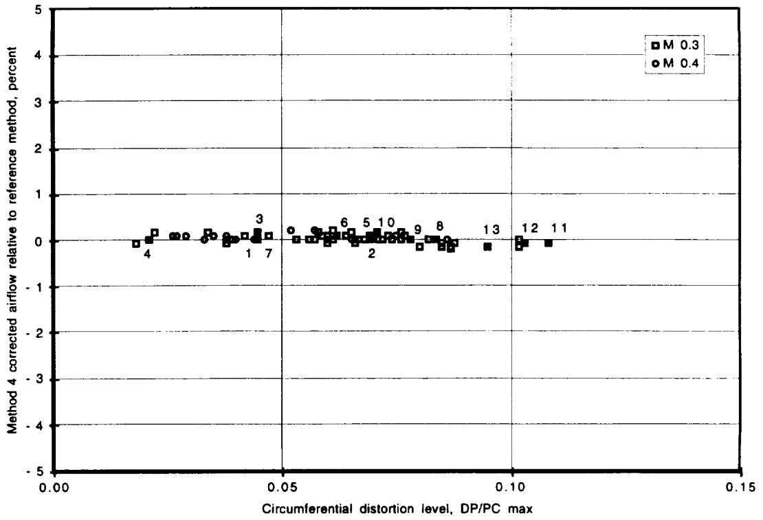
Figure 35. Method 4 corrected airflow relative to reference method as a function of circumferential distortion level.
