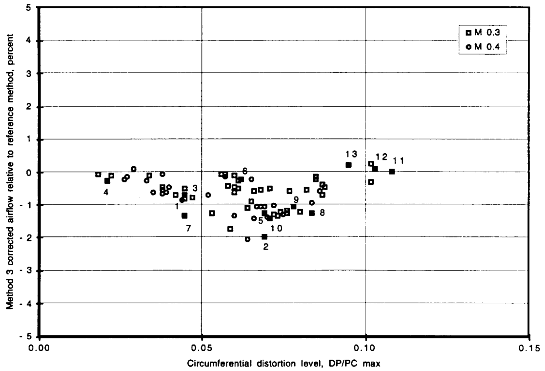
Figure 34. Method 3 corrected airflow relative to reference method as a function of circumferential distortion level.
