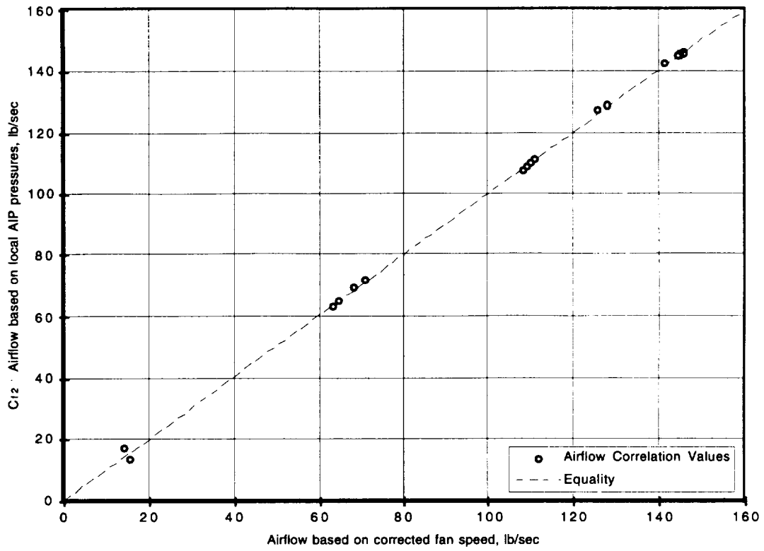
Figure 21. Method 2 calculated airflow as a function of reference method airflow.
