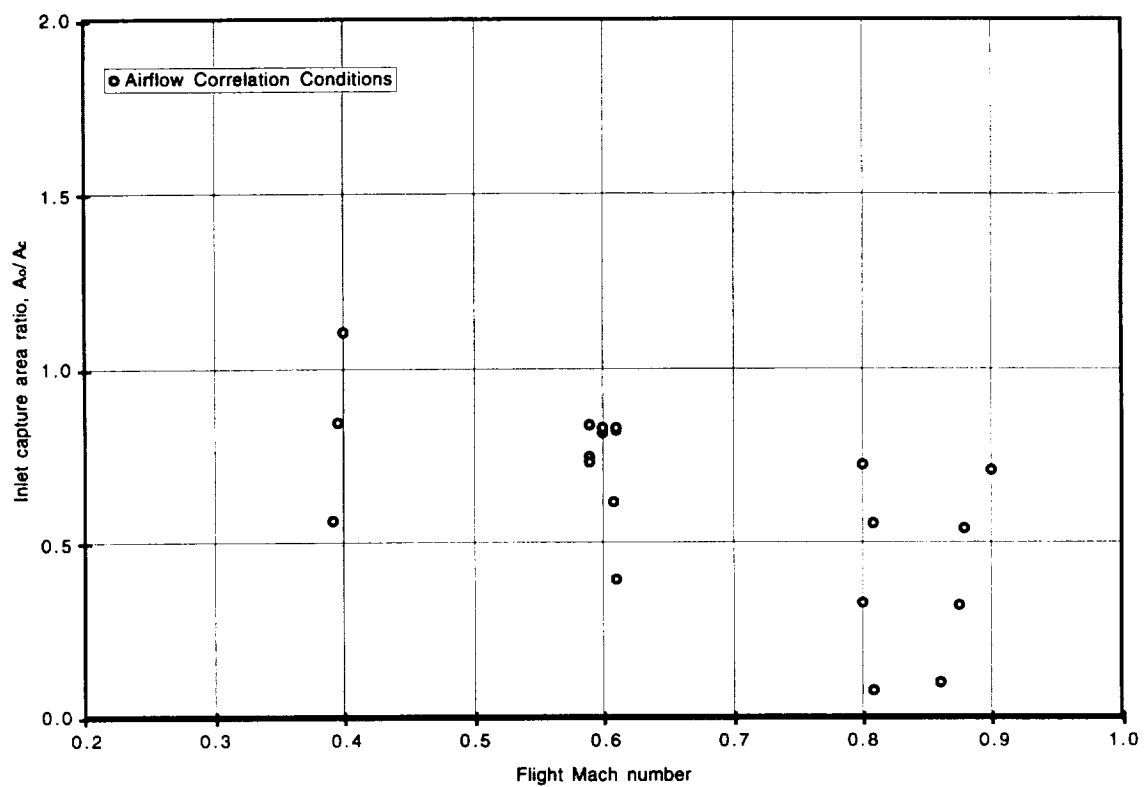
Figure 7. Inlet capture area ratios for airflow correlation conditions.
