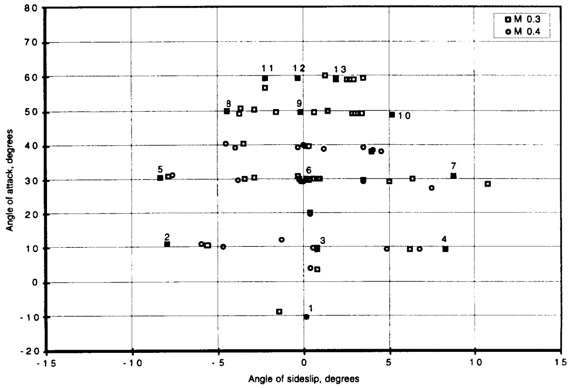
Figure 26. Test range of inlet data maneuver conditions.
