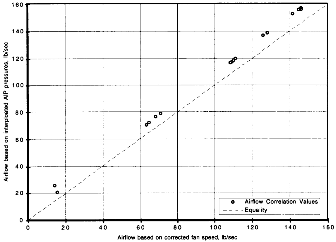
Figure 17. Corrected airflow based on AIP estimated static pressures and local total pressures as a function of airflow based on fan corrected speed.
