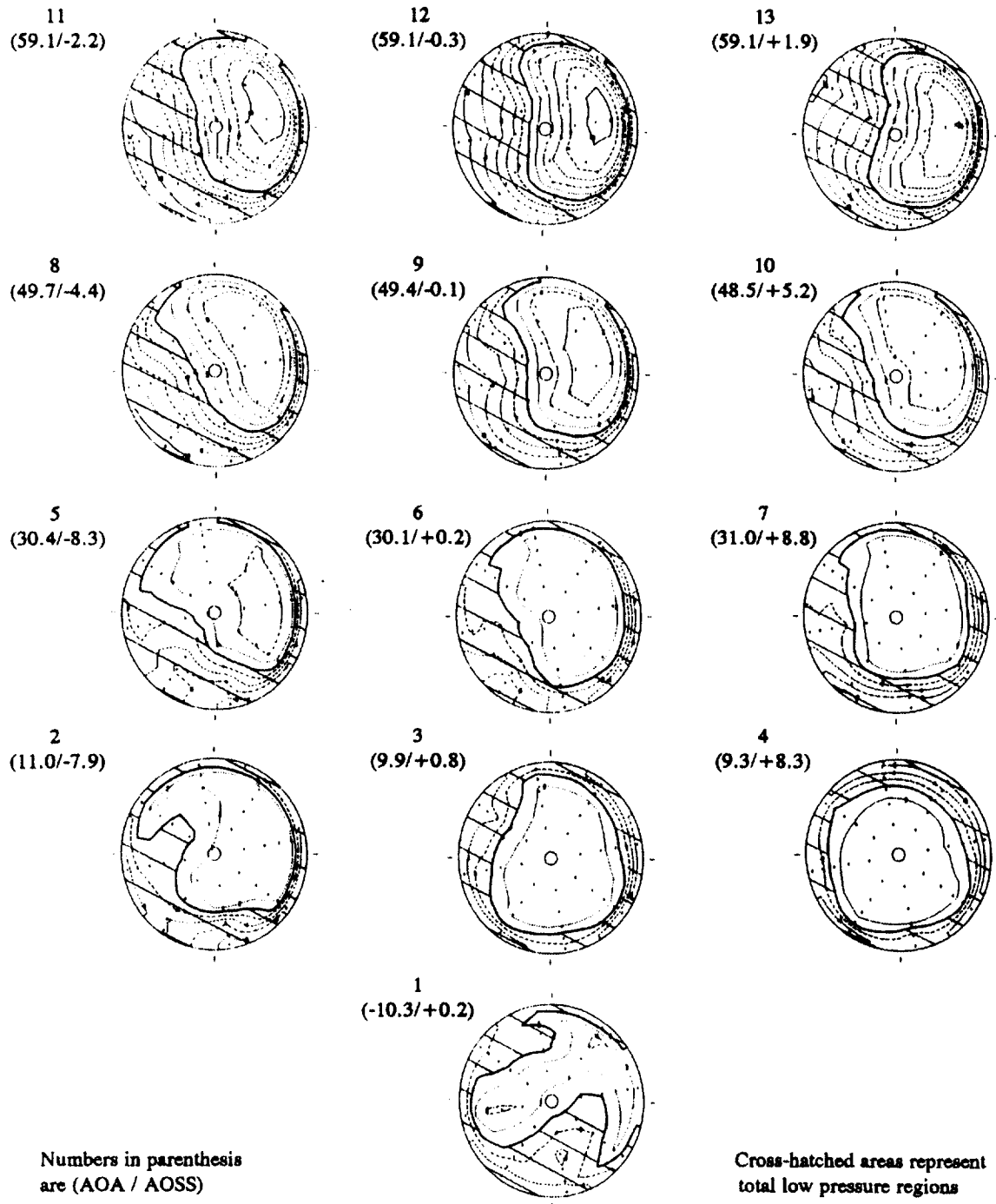
Figure 30. Right inlet (ALF) steady-state AIP total-pressure patterns for a range of fixed aerodynamic attitude conditions.
