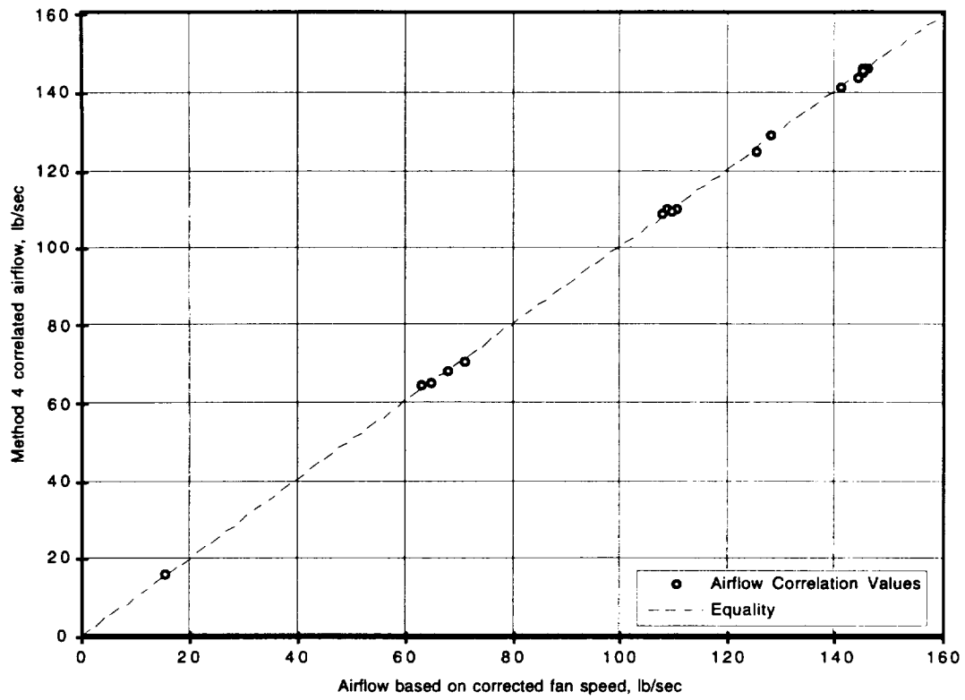
Figure 23. Method 4 calculated airflow as a function of reference method airflow.
