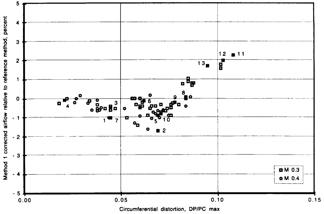
Figure 32. Method 1 corrected airflow relative to reference method as a function of circumferential distortion level.
