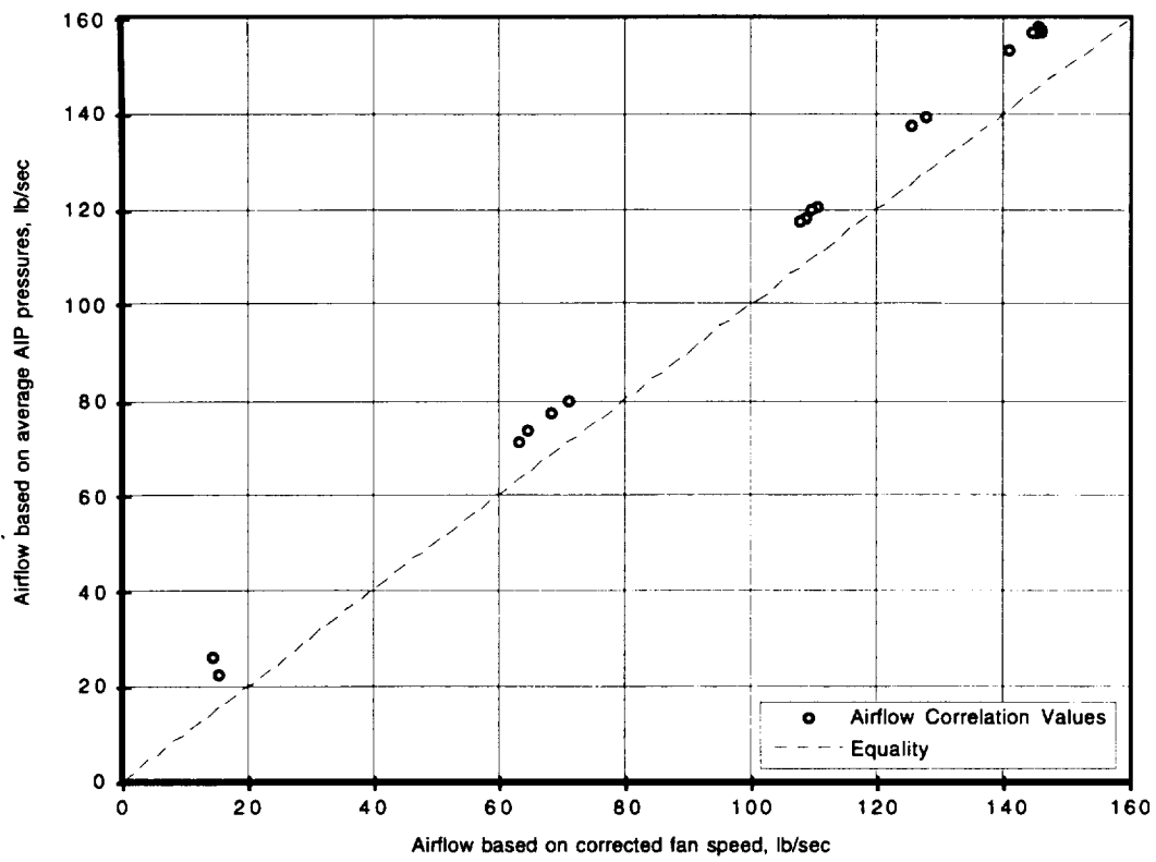
Figure 13. Corrected airflow based on AIP average pressures as a function of airflow based on corrected fan speed.
