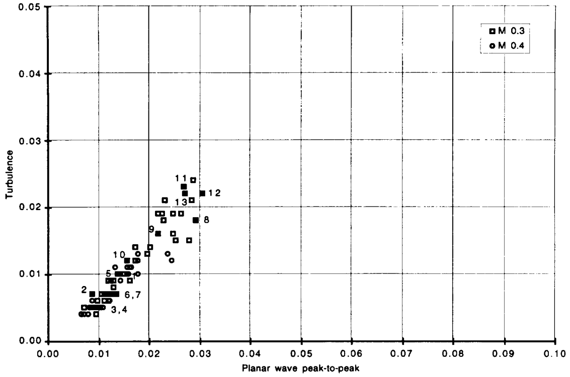
Figure 29. Test range of turbulence and planar wave levels.
