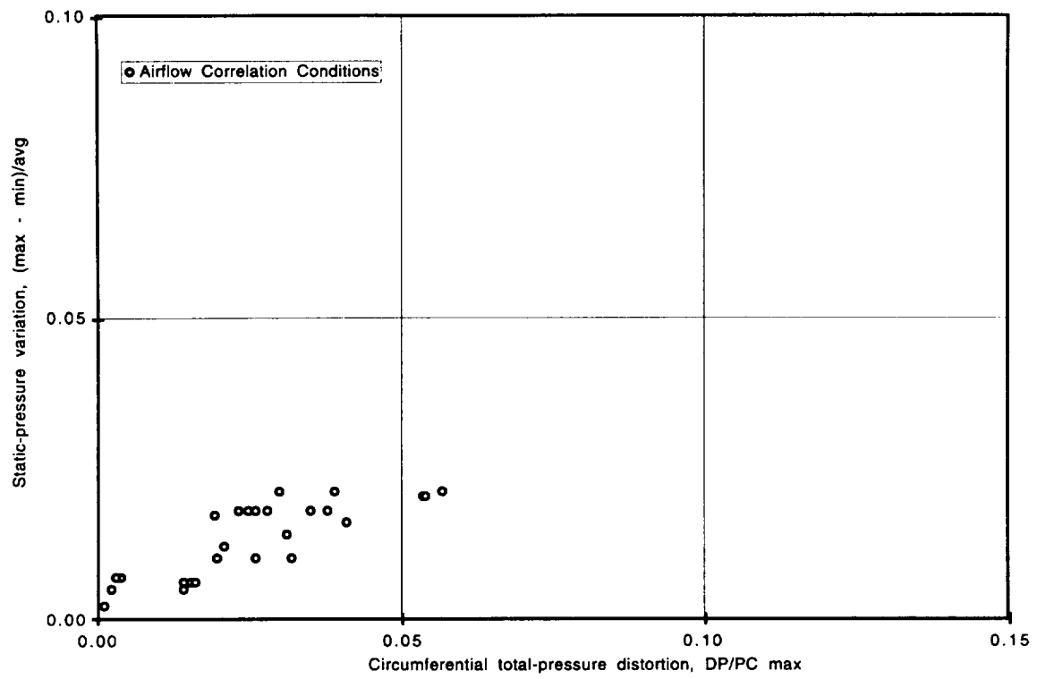
Figure 10. AIP static-pressure variations and steady-state circumferential distortion levels for airflow correlation conditions.
