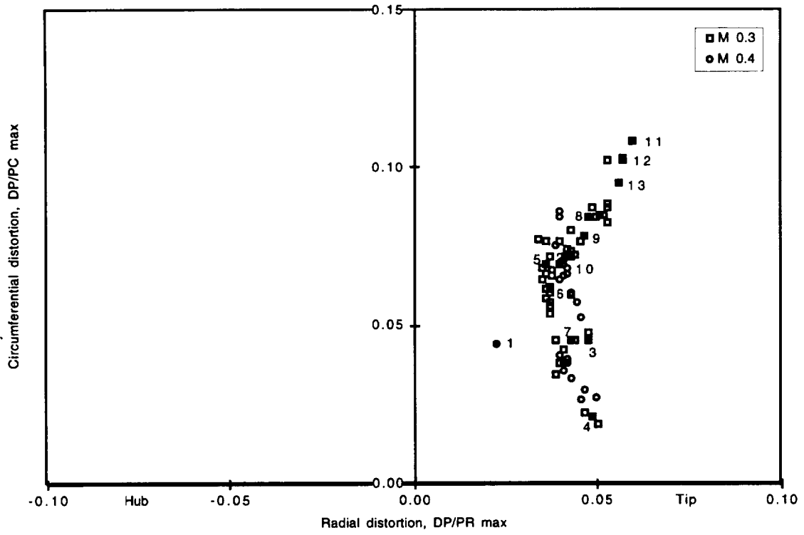
Figure 27. Test range of steady-state circumferential and radial distortions.
