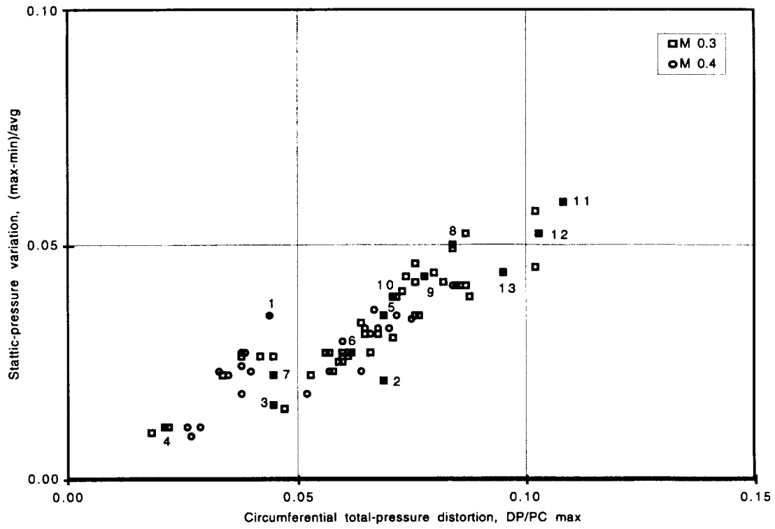
Figure 28. Test range of AIP static-pressure variations and steady-state circumferential distortions.
