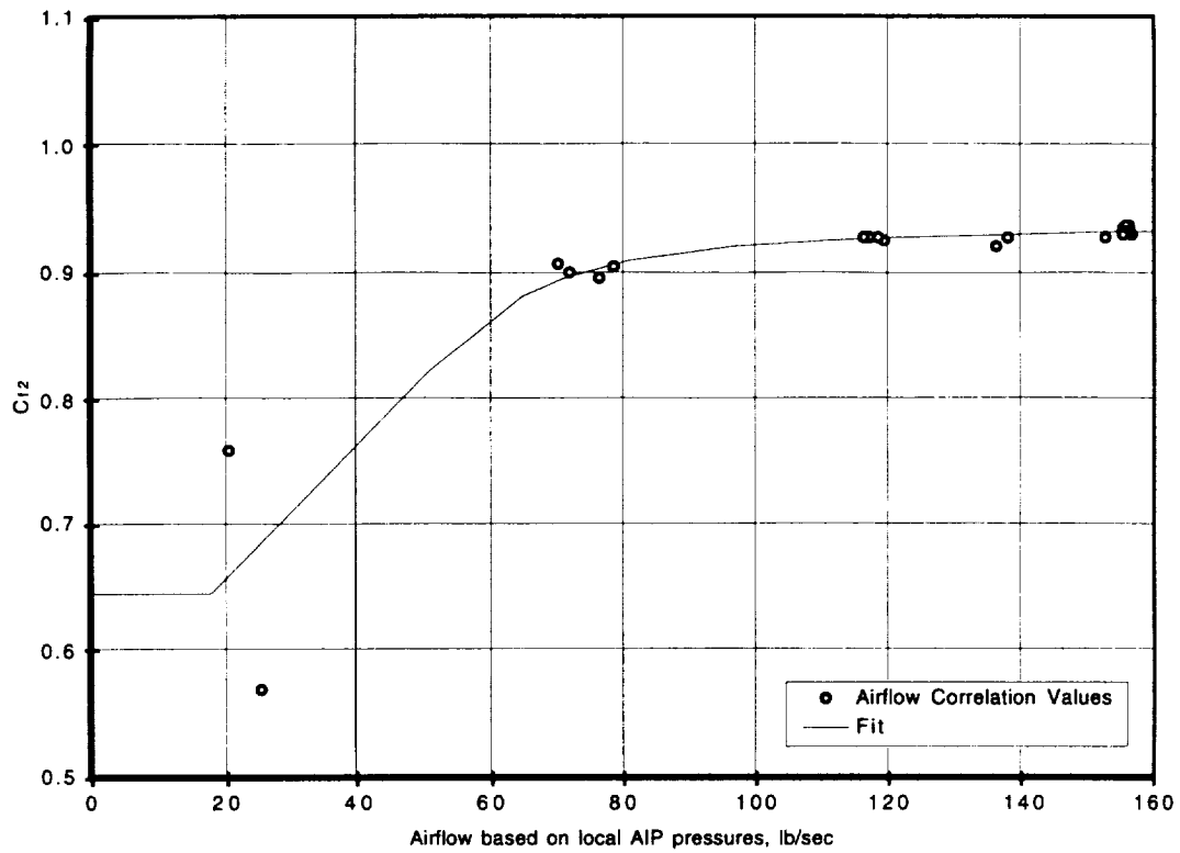
Figure 16. Method 2 flow coefficient relationship.
