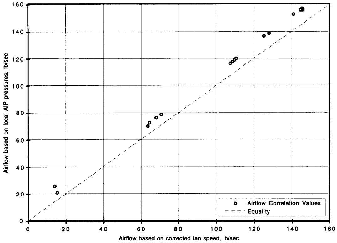
Figure 15. Corrected airflow based on AIP rake average static pressure and local total pressures as a function of airflow based on corrected fan speed.
