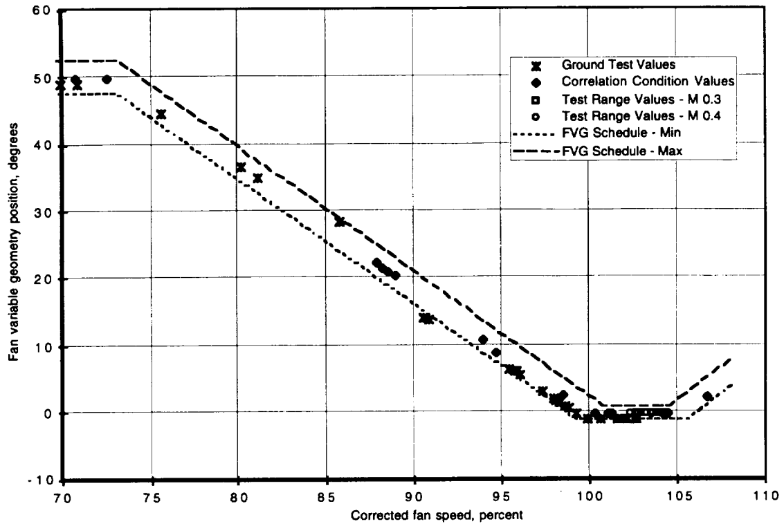
Figure 31. Fan variable geometry tracking for ground test, correlation, and fixed aerodynamic attitude conditions.
