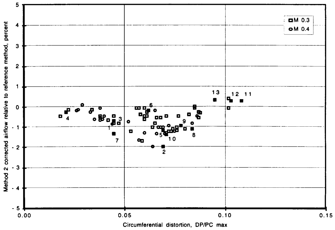
Figure 33. Method 2 corrected airflow relative to reference method as a function of circumferential distortion level.
