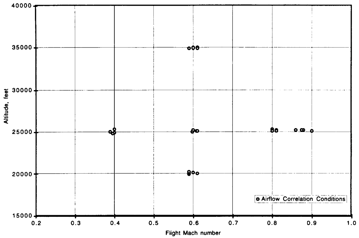
Figure 6. Mach number-altitude airflow correlation conditions.
