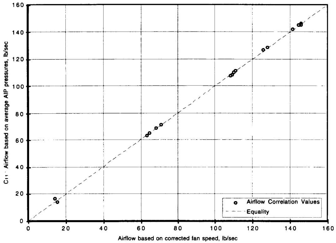
Figure 20. Method 1 calculated airflow as a function of reference method airflow.
