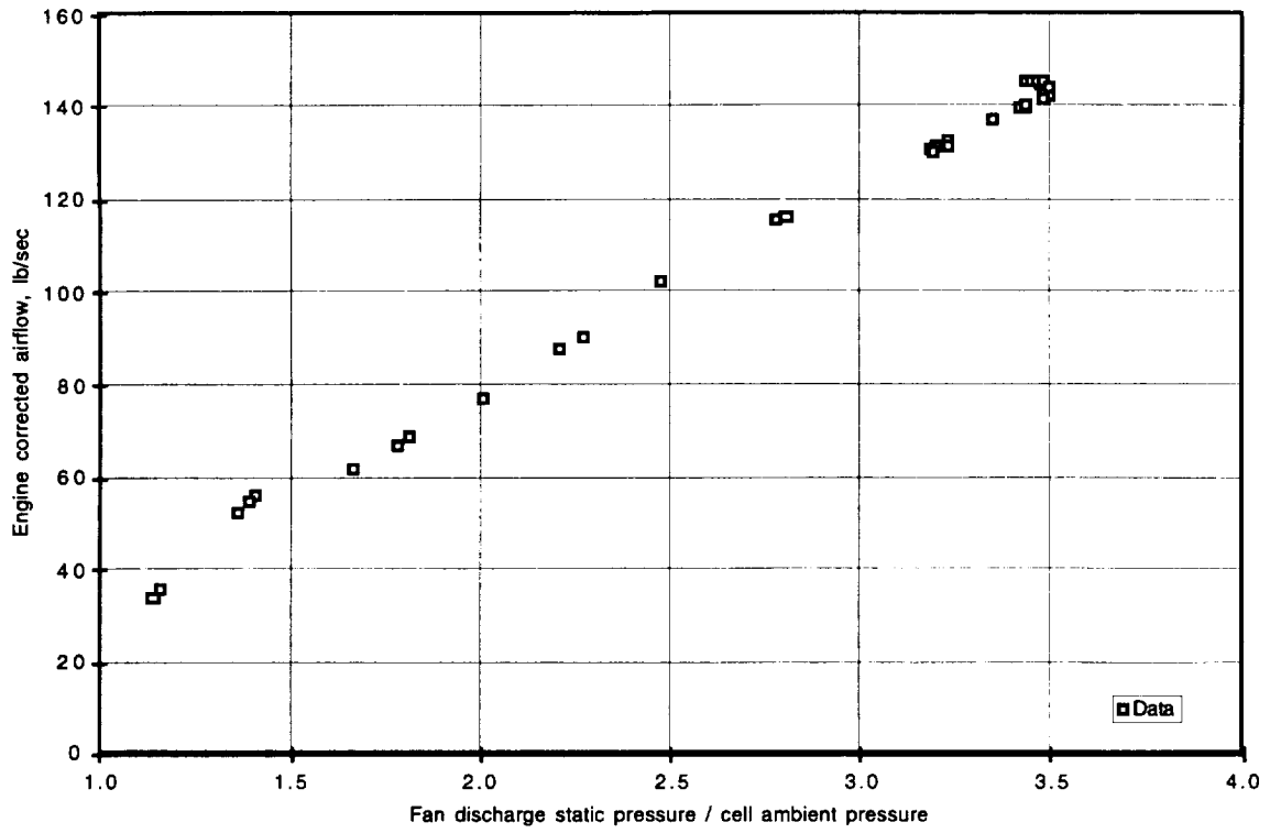
Figure 3. Ground test corrected flow to fan discharge static pressure / cell ambient pressure ratio correlation.
