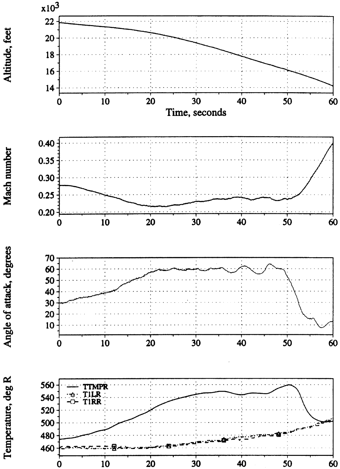
Figure B1. Illustration of temperature probe differences during angle-of-attack-change.
