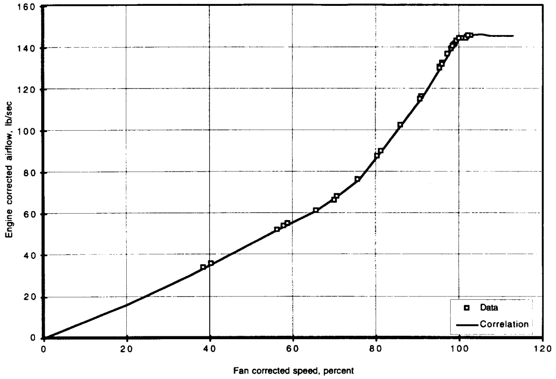
Figure 2. Ground test corrected flow to corrected speed data and correlation.
