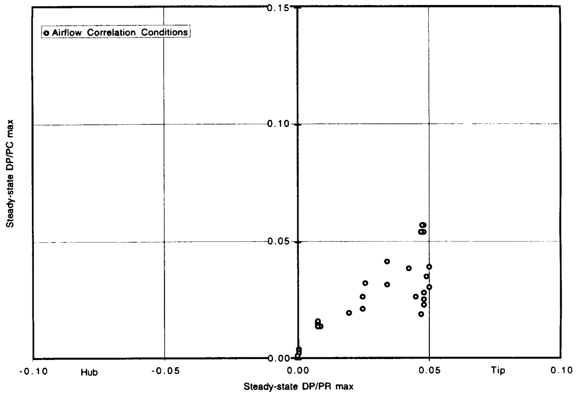
Figure 9. Steady-state circumferential and radial distortion levels for airflow correlation conditions.
