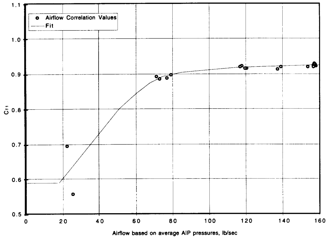
Figure 14. Method 1 flow coefficient relationship.
