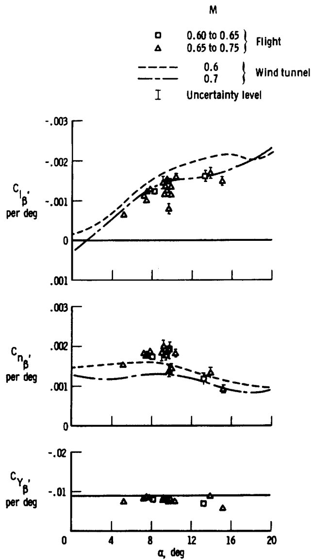
(b) C_{l_\beta} , C_{n_\beta} , C_{Y_\beta} for transonic configuration.
