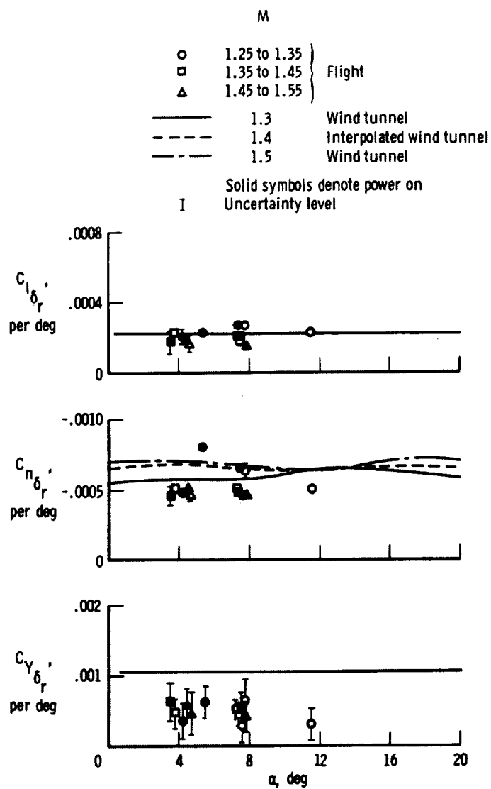
(b) C_{l_{\delta_r}} , C_{n_{\delta_r}} , C_{Y_{\delta_r}} .
