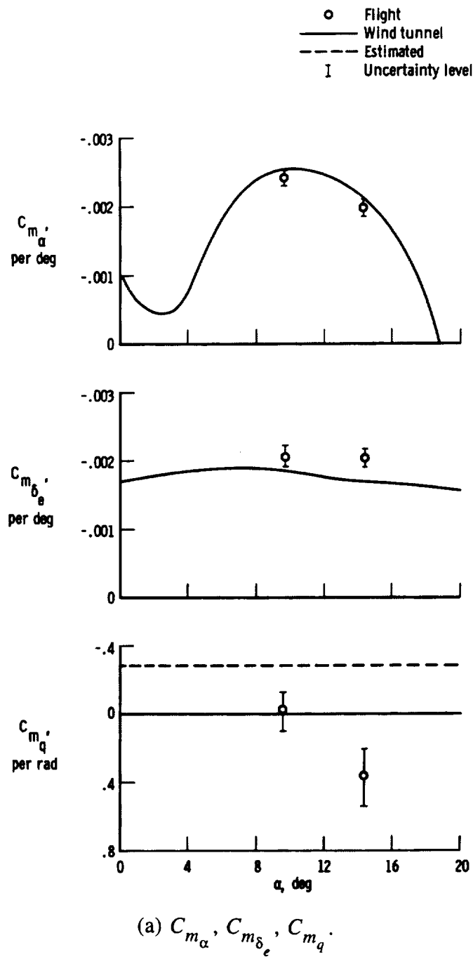
Figure 7. Comparison of longitudinal derivatives obtained from flight data with wind-tunnel results. M = 0.95 ; transonic configuration; center of gravity = 0.66\bar{c} .
