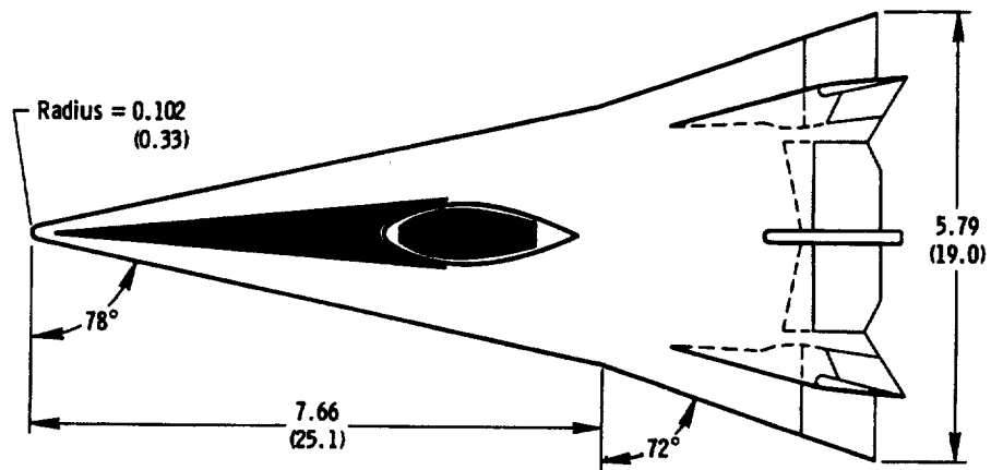
Figure 2. X-24B research aircraft dimensions (in meters (feet)).
