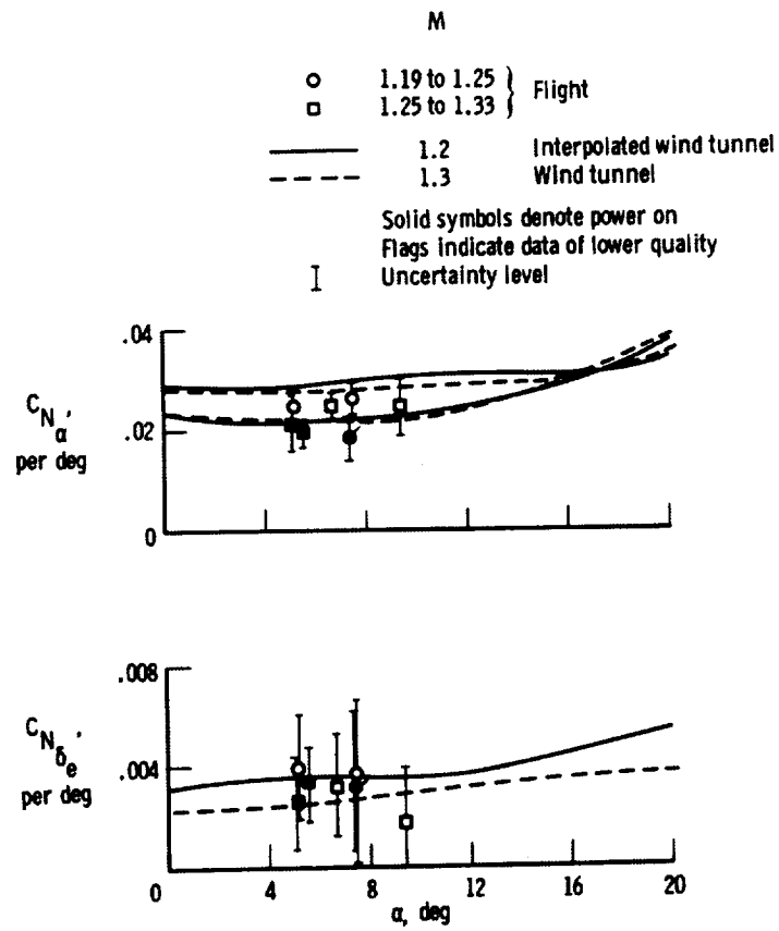
(b) C_{N_\alpha} , C_{N_{\delta_e}}
