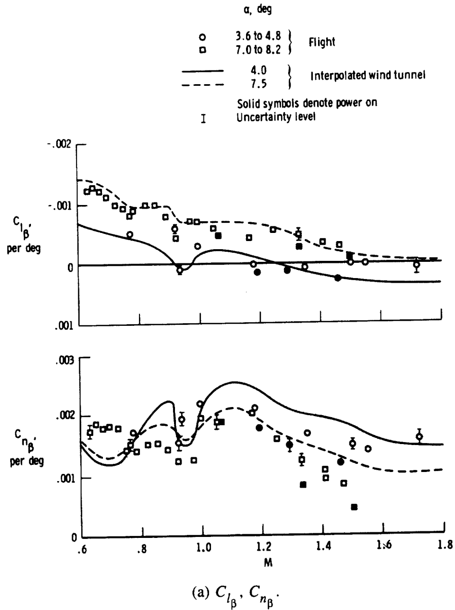
Figure 17. Comparison of lateral-directional derivatives obtained from flight data with wind-tunnel results for angles of attack near 4^{\circ} and 7.5^{\circ} . Transonic configuration; center of gravity = 0.65\bar{c} .
