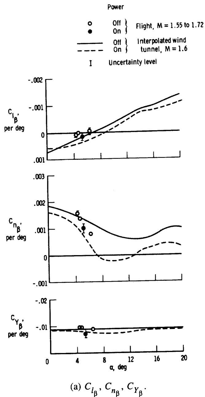
Figure 16. Comparison of lateral-directional derivatives obtained from flight data with wind-tunnel results. M = 1.55 to 1.72 ; transonic configuration; center of gravity = 0.65\bar{c} .
