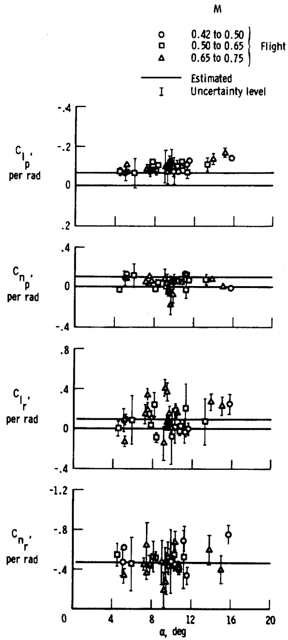
(f) C_{l_p} , C_{n_p} , C_{l_r} , C_{n_r} for subsonic and transonic configurations.
