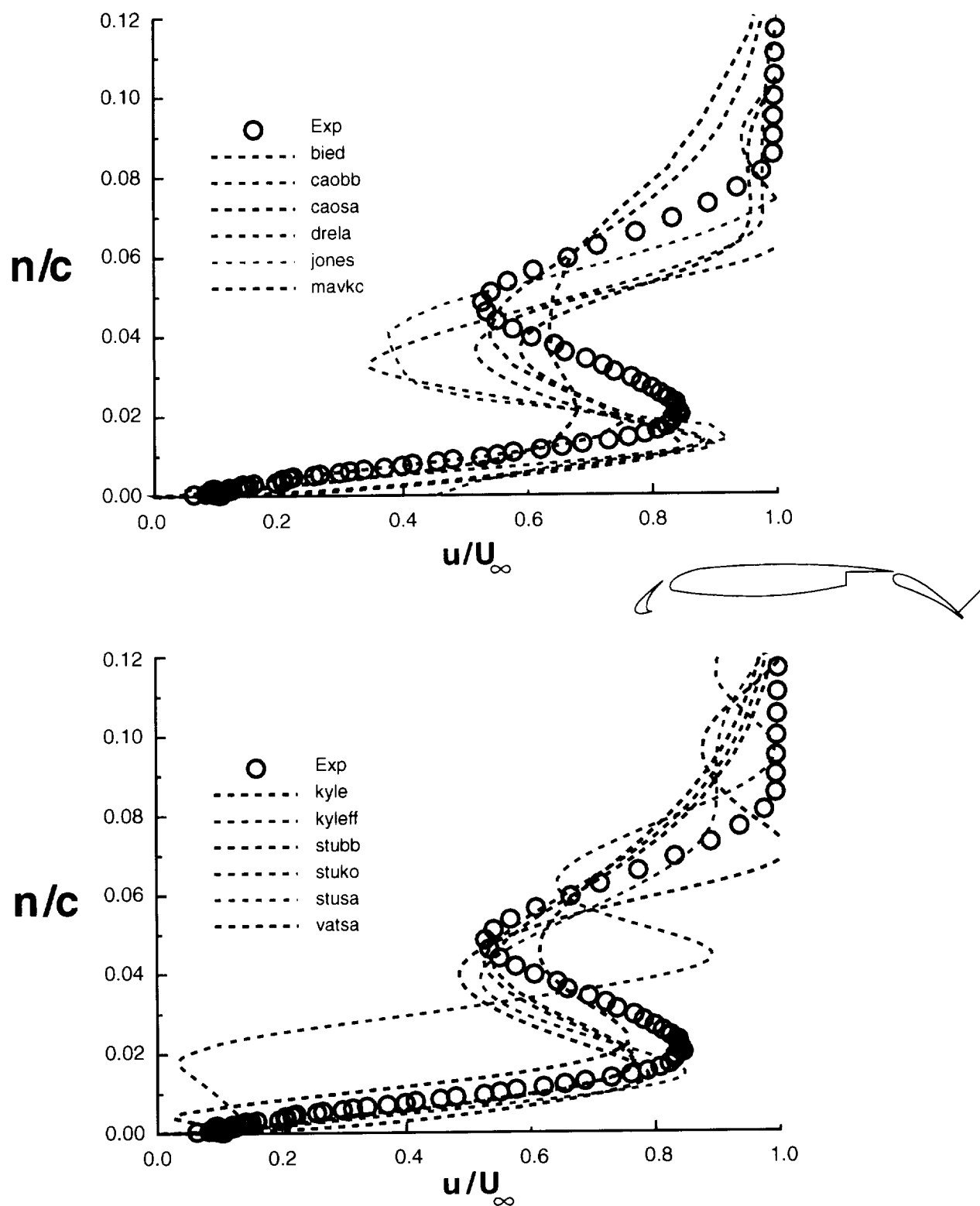
Figure 27. Velocity profiles on the flap -- Geometry A ( x/c=1.112 , \alpha=8.12^\circ , Re=5 million)
