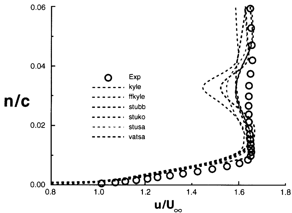
Figure 24. Velocity profiles on the main element -- Geometry A ( x/c=.45 , \alpha=8.12^\circ , Re=5 million)
