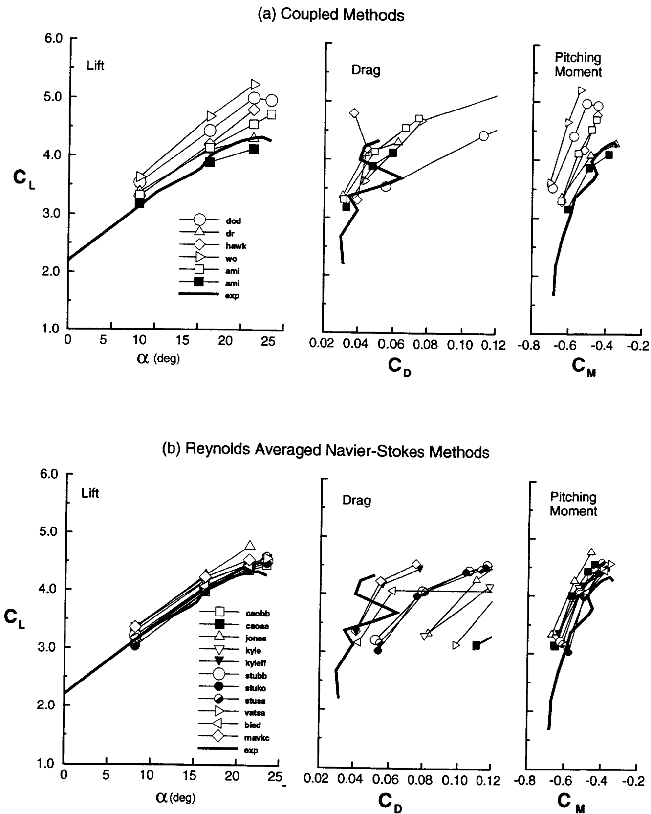
Figure 4. Force and moment coefficients for Geometry B, Re=9,000,000
