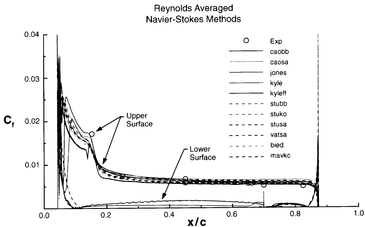
Figure 19. Main-element skin-friction distribution -- Geometry A (\alpha=8.12^\circ, Re=5 \text{ million})
