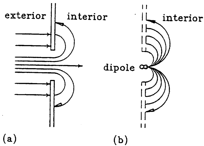
Fig. 12.1 Development of equivalent electric field dipole.
