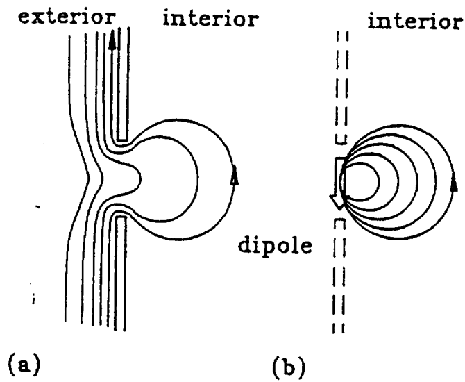
Fig. 12.2 Development of equivalent magnetic field dipole.
