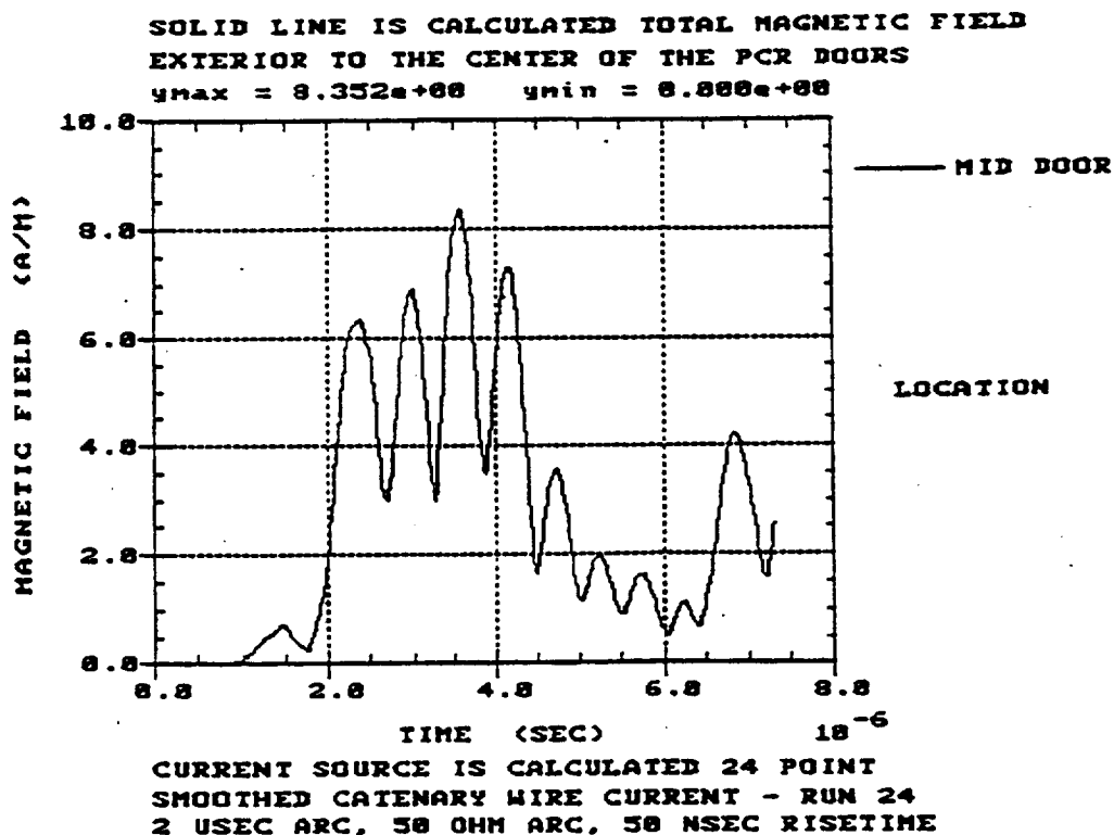
Figure 4.5 Total Magnetic Field Comparisons at the PCR Door Center
