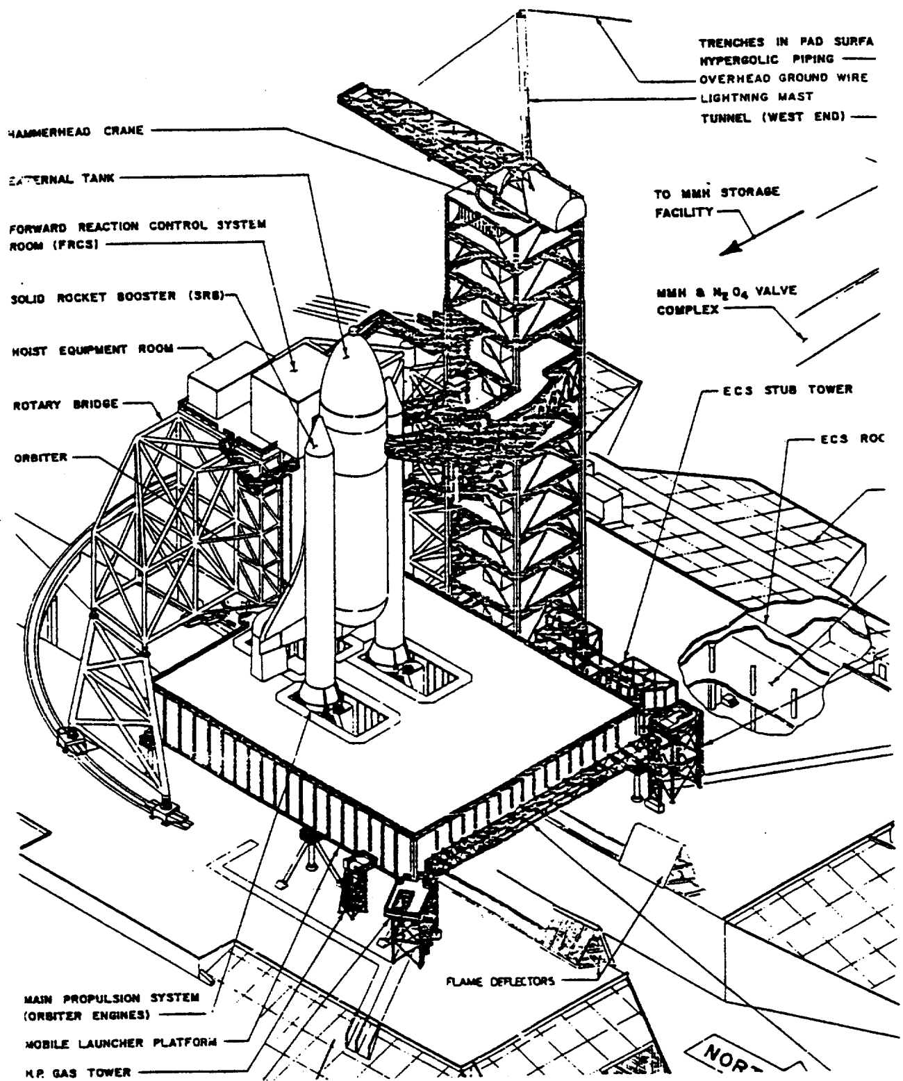
Figure 6.1 PCR and Orbiter in the Mate Position
