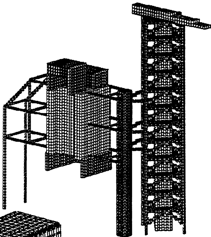
Figure 4.1 Launch Pad Structure in the Park Position
