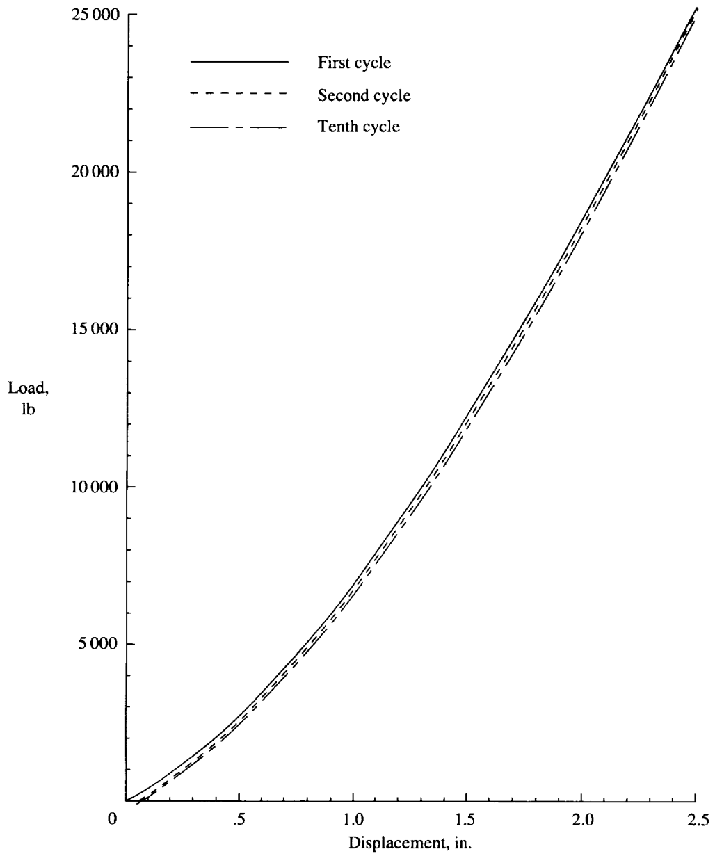
Figure 14. Least-squares approximation of hysteresis loops for cyclic loading test.
