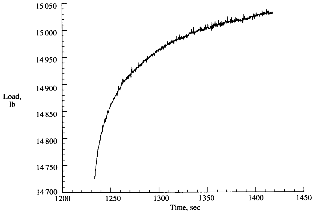
(b) Load rebound.
