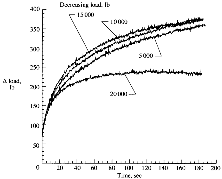
Figure 10. Stair-step test with decreasing load viscoelastic results.
