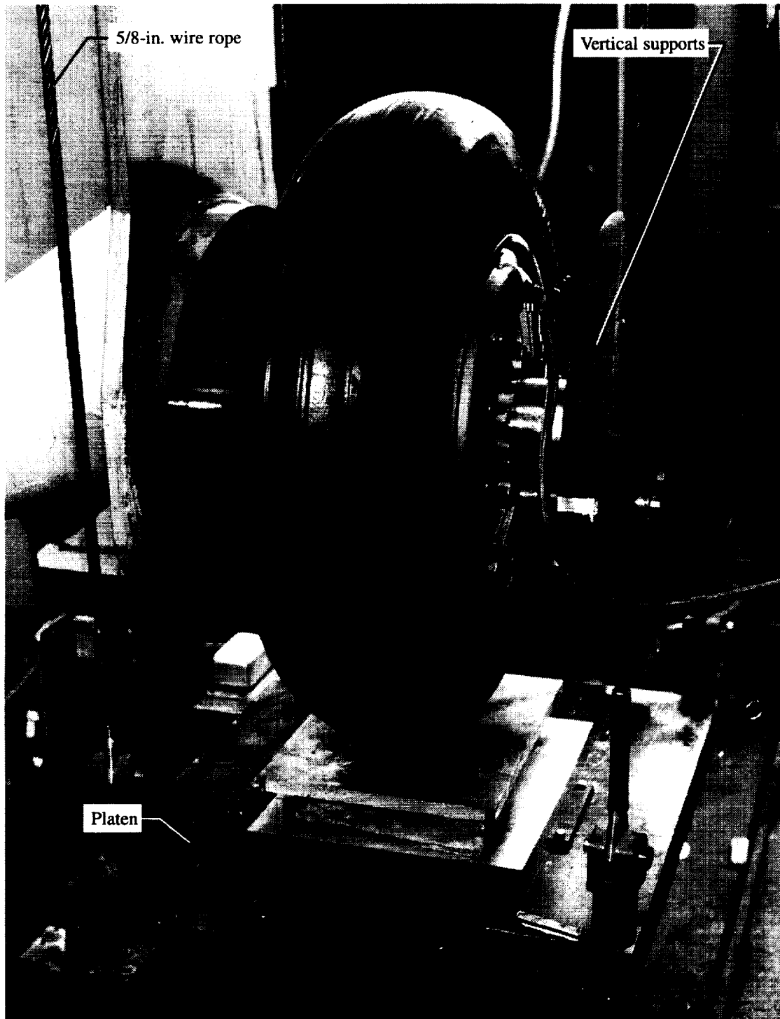
Figure 2. Tire vibration stand.
