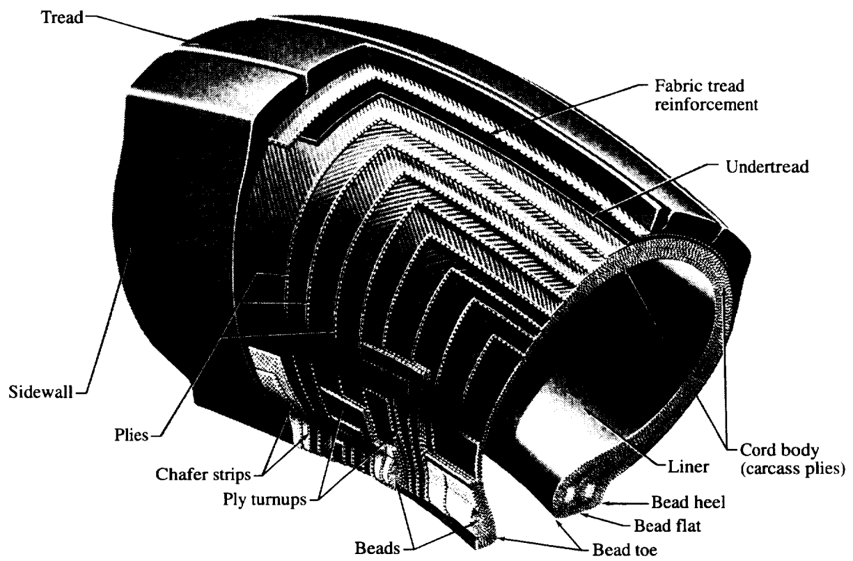
Figure 1. Aircraft tire construction.
