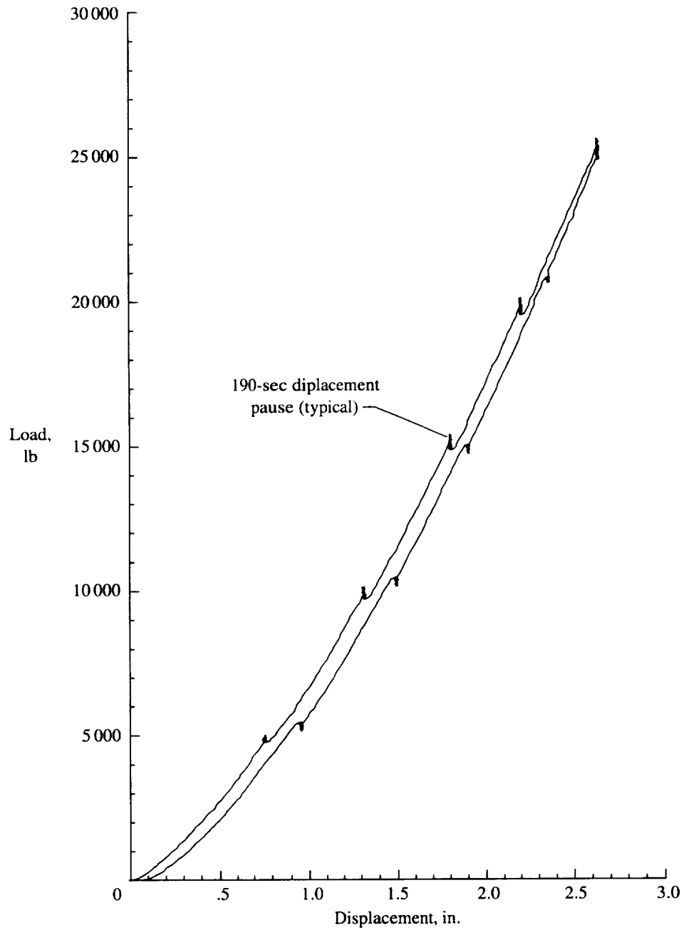
Figure 11. Load-deflection curve associated with stair-step test.
