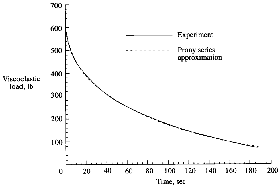
Figure 17. Prony series approximation of tire relaxation characteristics.
