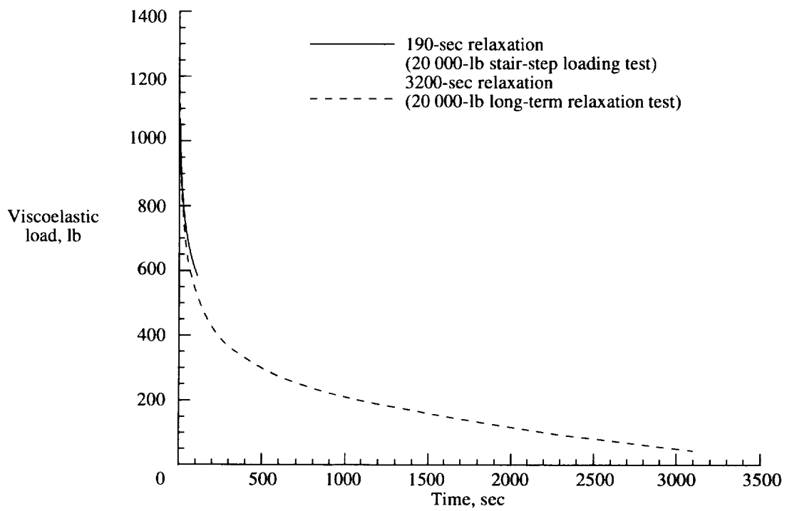
Figure 16. Long-term relaxation and stair-step tests results.
