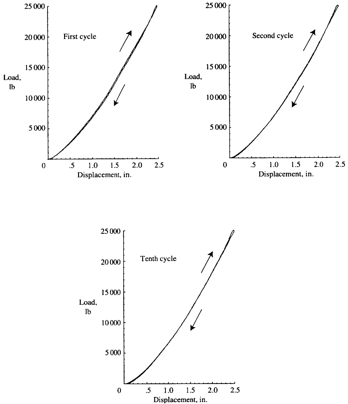
Figure 13. Typical load-deflection curves for cyclic loading test.
