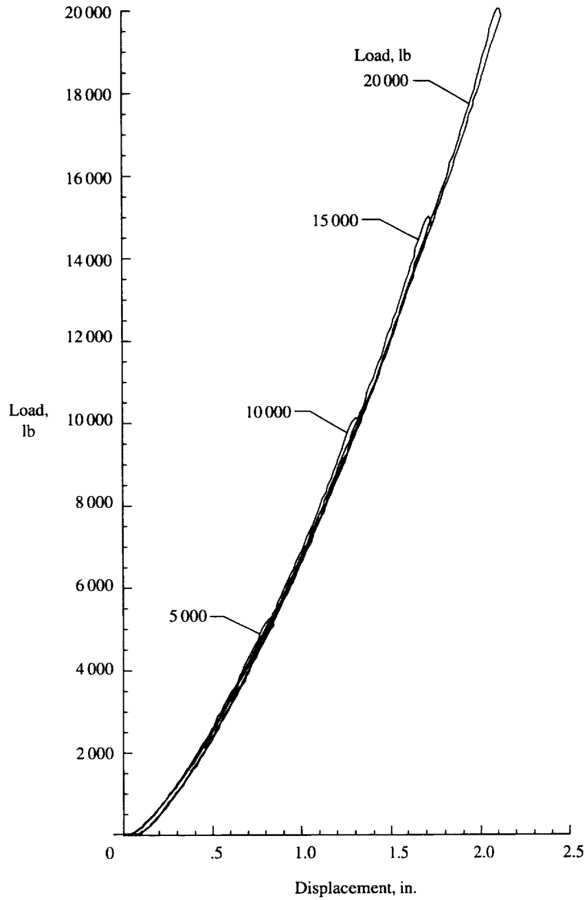
Figure 15. Hysteresis curves for loads from 5000 through 20 000 lb.
