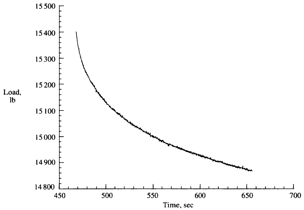
(b) Load relaxation.
