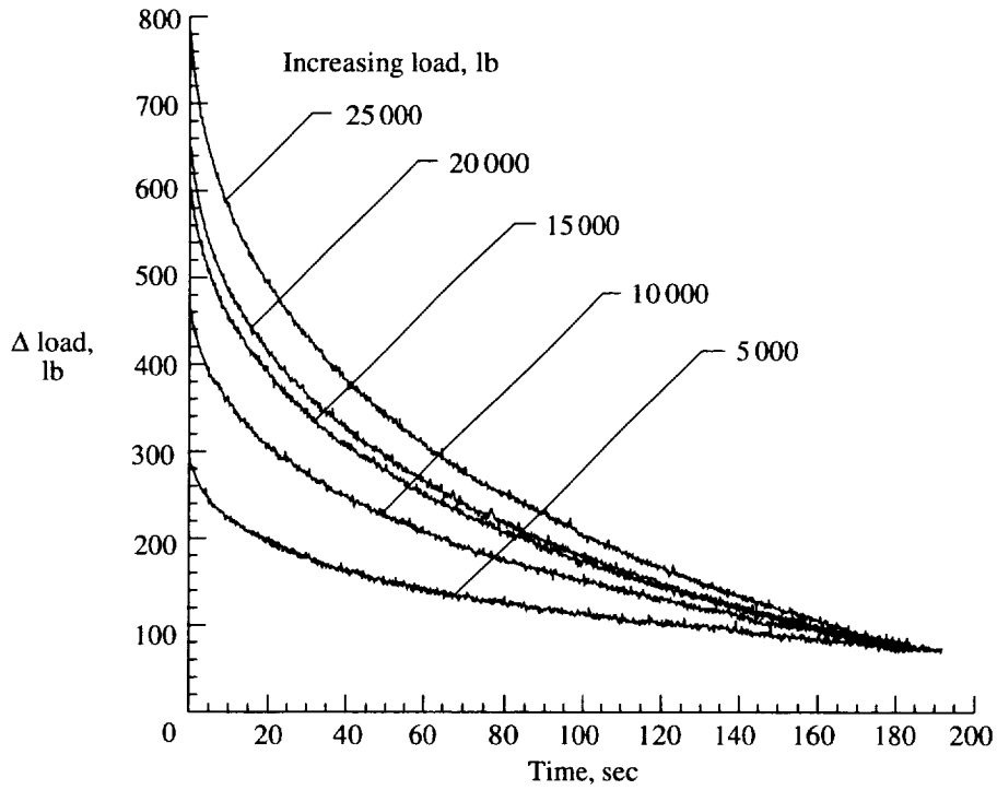
Figure 9. Stair-step test with increasing load viscoelastic results.
