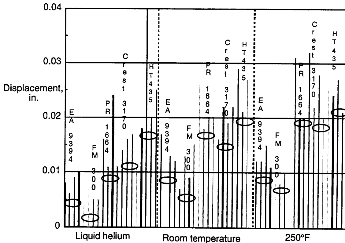
Figure 8: Displacement at failure of HRP honeycomb drill core bonded to Gr/Ep with five different adhesives and three different pre-conditionings tested at room temperature.
