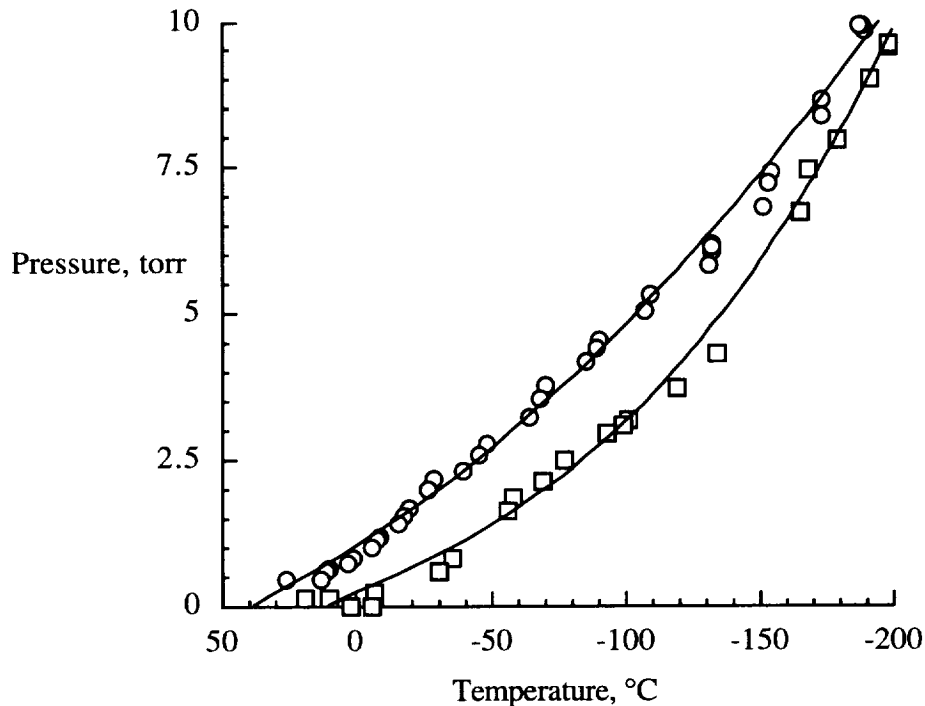
Figure 2: Pressure versus temperature for specimen #6.
