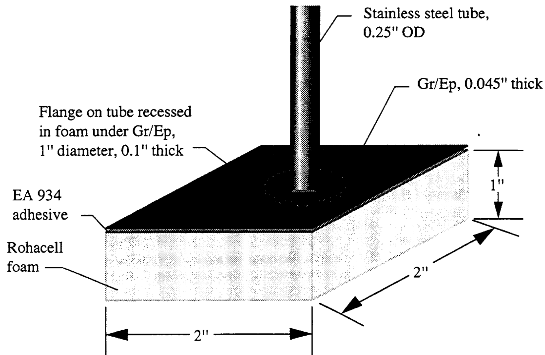
Figure 1: Schematic diagram of test specimen with stainless steel tube embedded between Gr/Ep and Rohacell foam.
