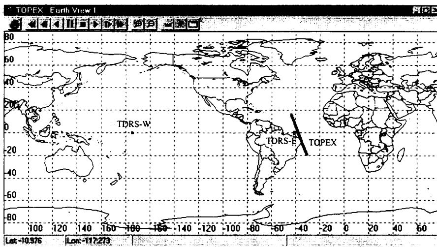
Figure 3 - TOPEX ground track for day 174 and access to TDRS-W.
