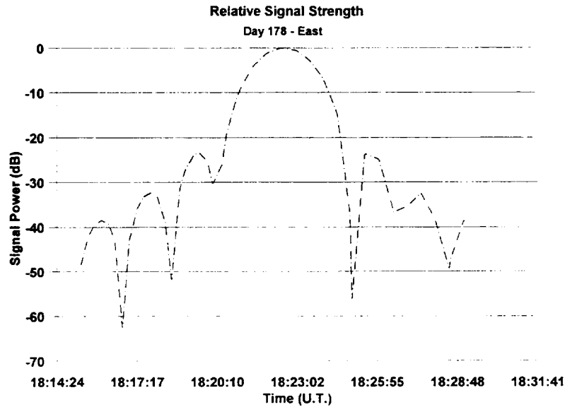
Figure 27 - Pointing loss and space loss for day 178 and TDRS East.
