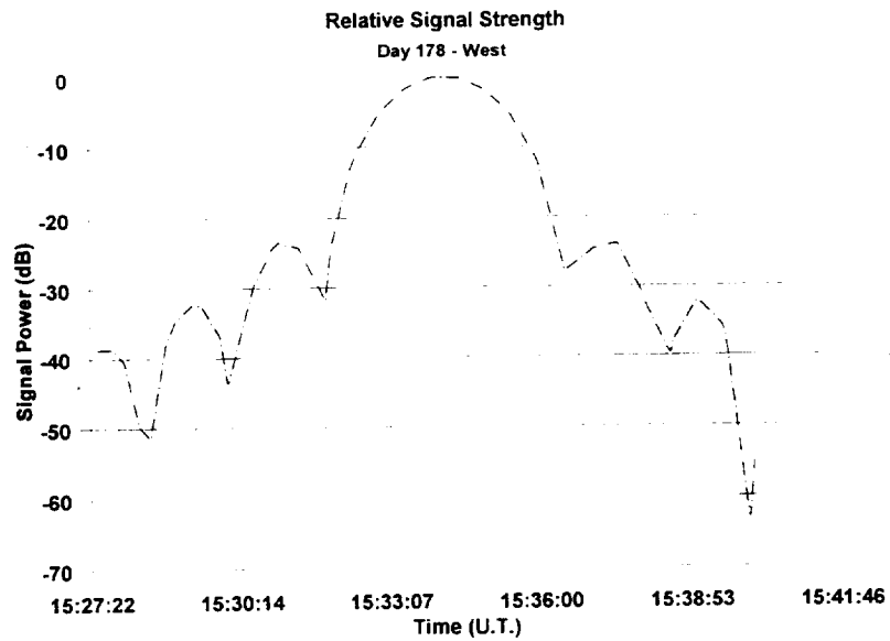
Figure 26 - Pointing loss and space loss for day 178 and TDRS West.
