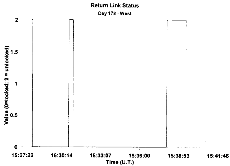
Figure 16 - Receiver lock status at the WSC for day 178 and TDRS West.
