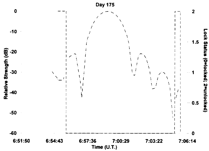
Figure 29 - Correlation of the signal strength with the receiver lock status for day 175
