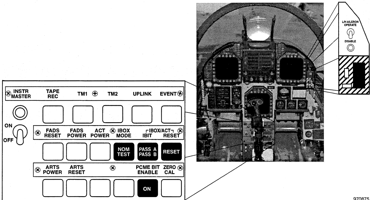
Figure 10. Electro-hydraulic actuator disable switch and control panel in cockpit.
