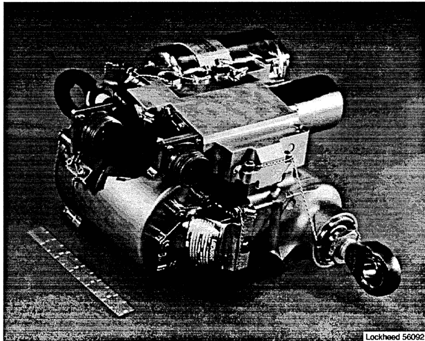
Figure 2. Electro-hydrostatic actuator (EHA).
