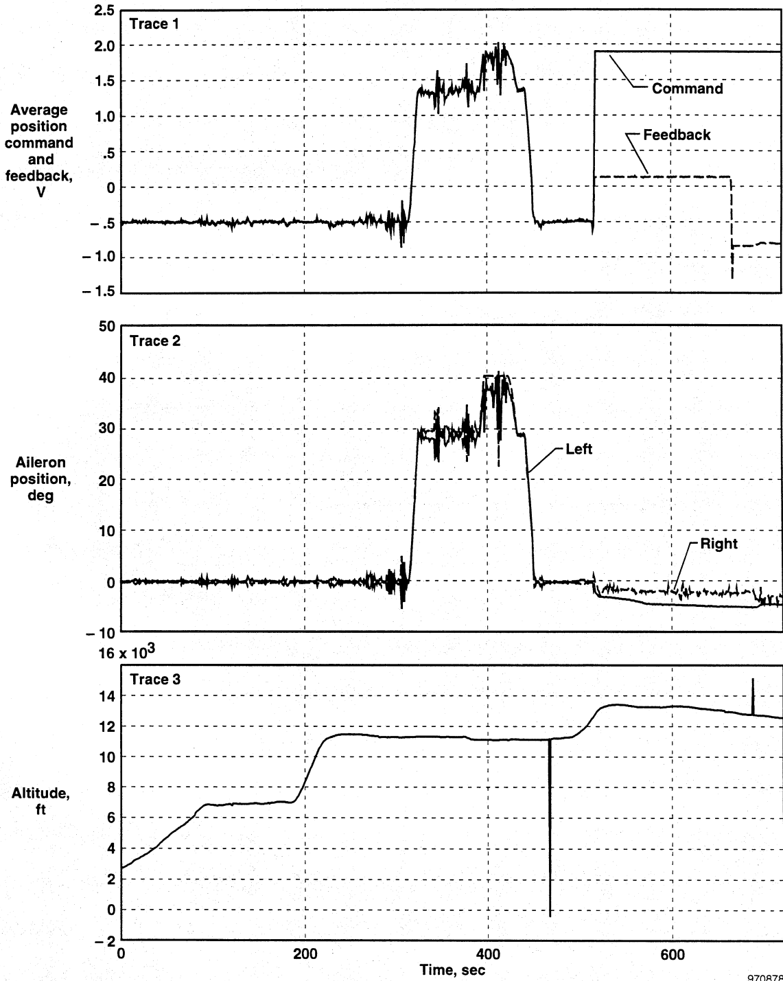
Figure 13. In-flight failure, January 16, 1996, flight 564.
