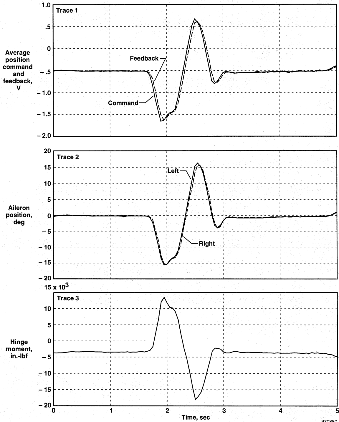
Figure 15. Abrupt roll doublet—full stick (left). M=0.72 , altitude=25,000 ft, q\text{-bar}=284 \text{ lbf/ft}^2 .
