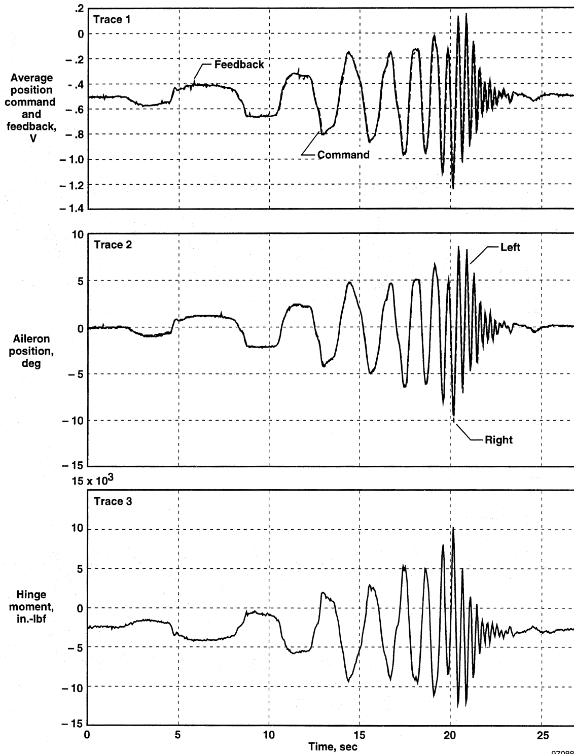
Figure 16. Slow—fast lateral frequency sweep. M=0.83 , altitude=25,000 ft, q\text{-bar}=376 \text{ lbf/ft}^2 .
