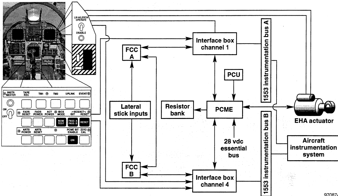
Figure 5. Systems Research Aircraft system architecture.
