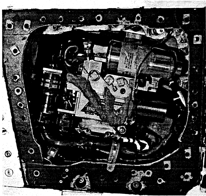
Figure 4. Electro-hydrostatic actuator installed in SRA.
