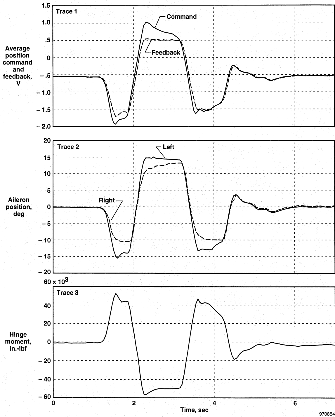
Figure 19. Aileron reversal—half stick (left). M=1.58 , altitude=34,000 ft, q\text{-bar}=890 lbf/ft 2 .
