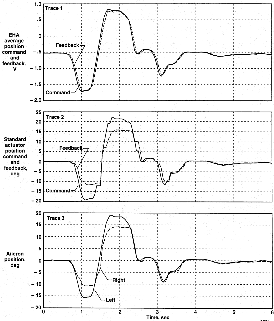
Figure 21. Abrupt aileron reversal—full stick (left).
