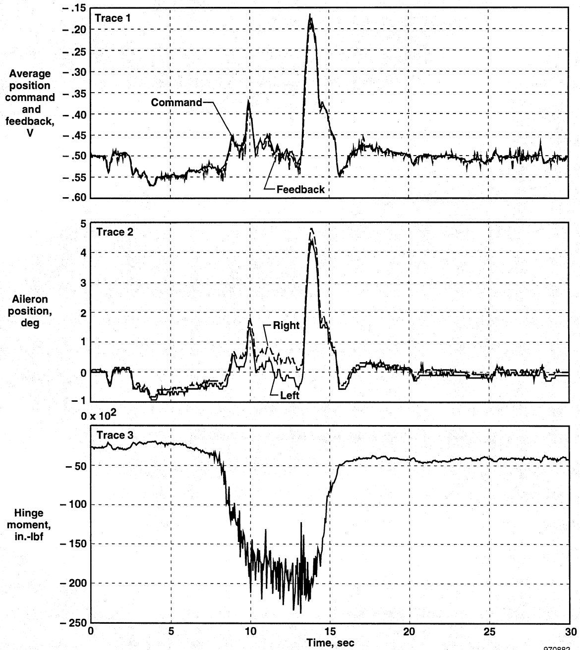
Figure 17. Windup turn to 20^\circ \alpha . M=0.83 , altitude=25,000 ft, q\text{-bar}=376 \text{ lbf/ft}^2 .
