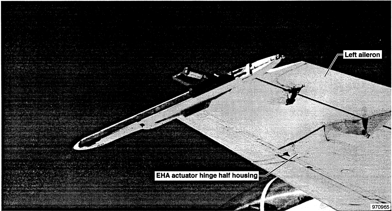
Figure 3. Hinge half housing.
