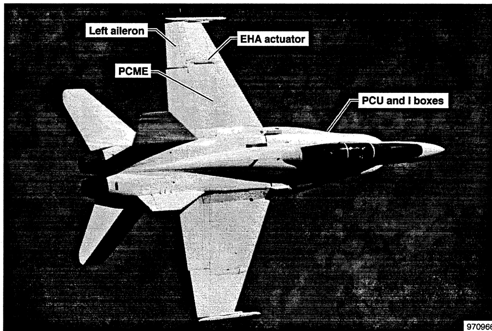
Figure 6. Electro-hydrostatic actuator system component locations on SRA.
