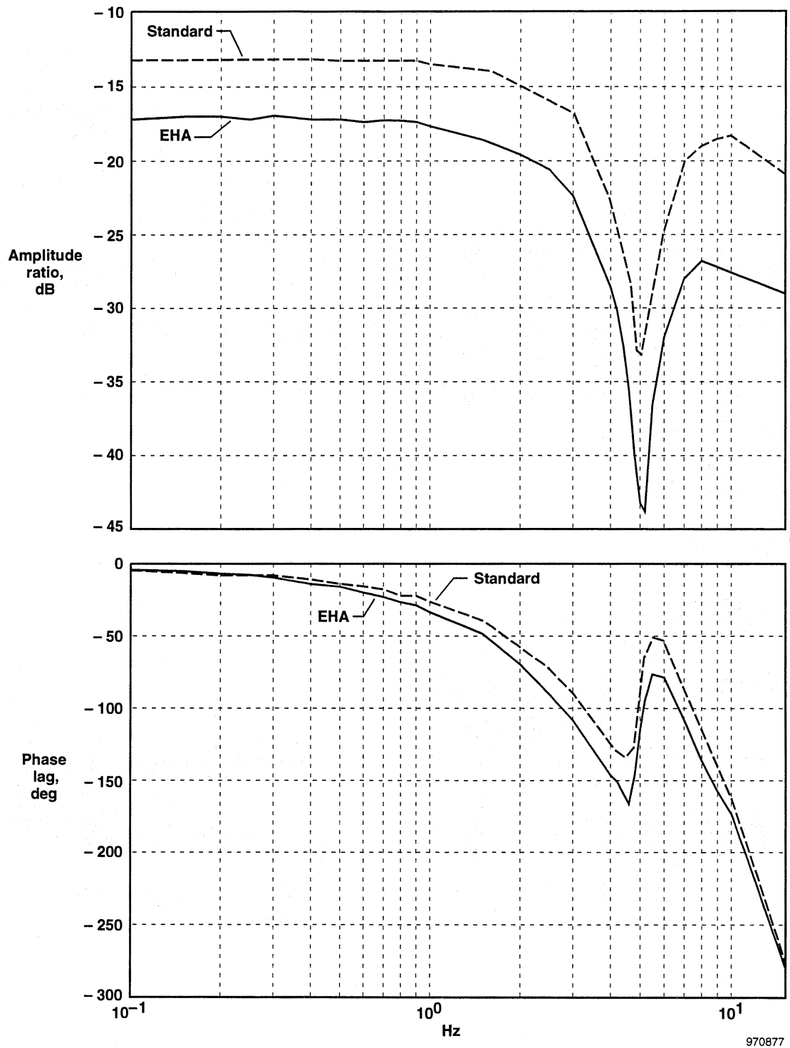
Figure 12. Electro-hydrostatic actuator and standard actuator closed-loop small amplitude frequency response.
