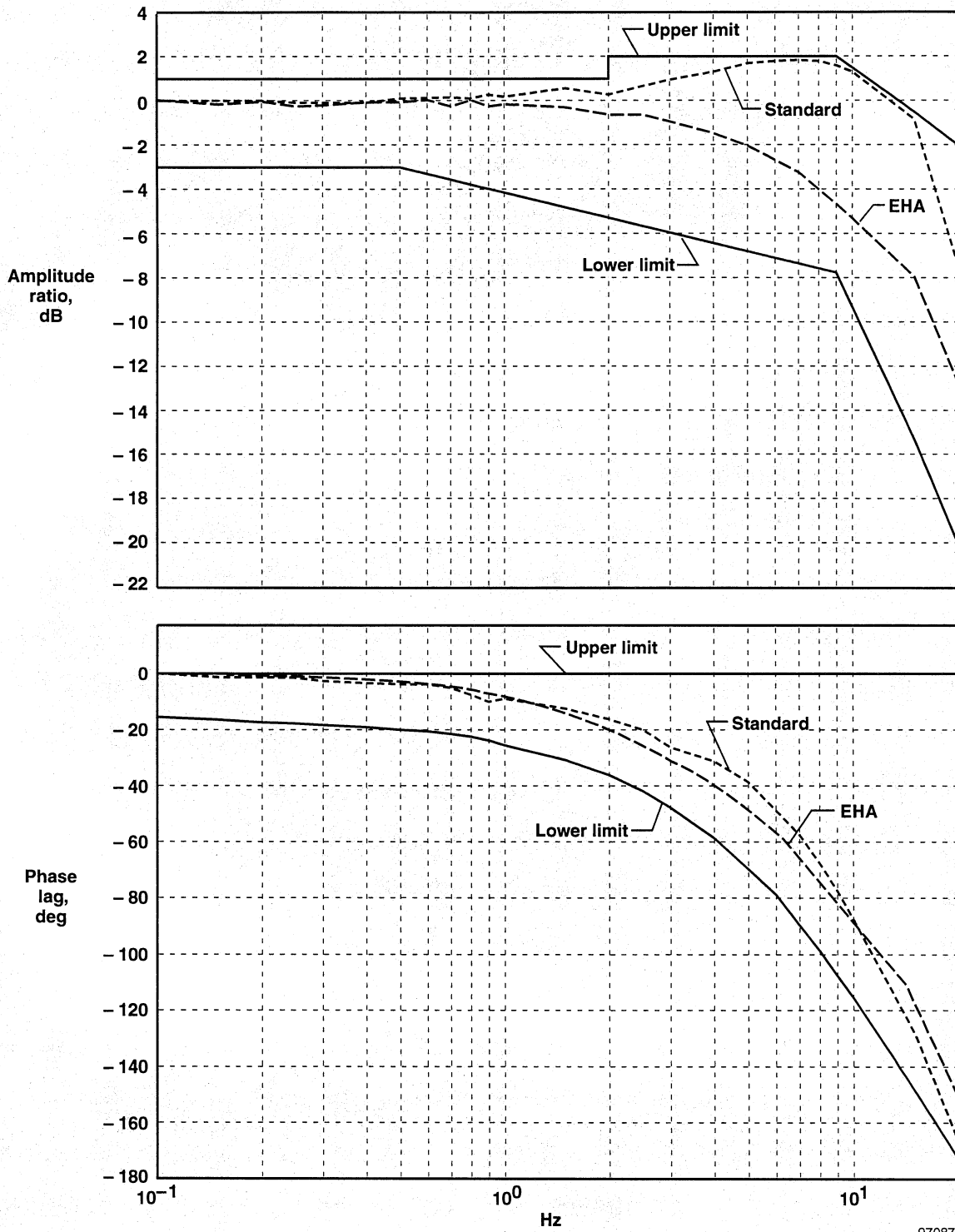
Figure 11. Electro-hydrostatic actuator and standard actuator open-loop small amplitude frequency response.
