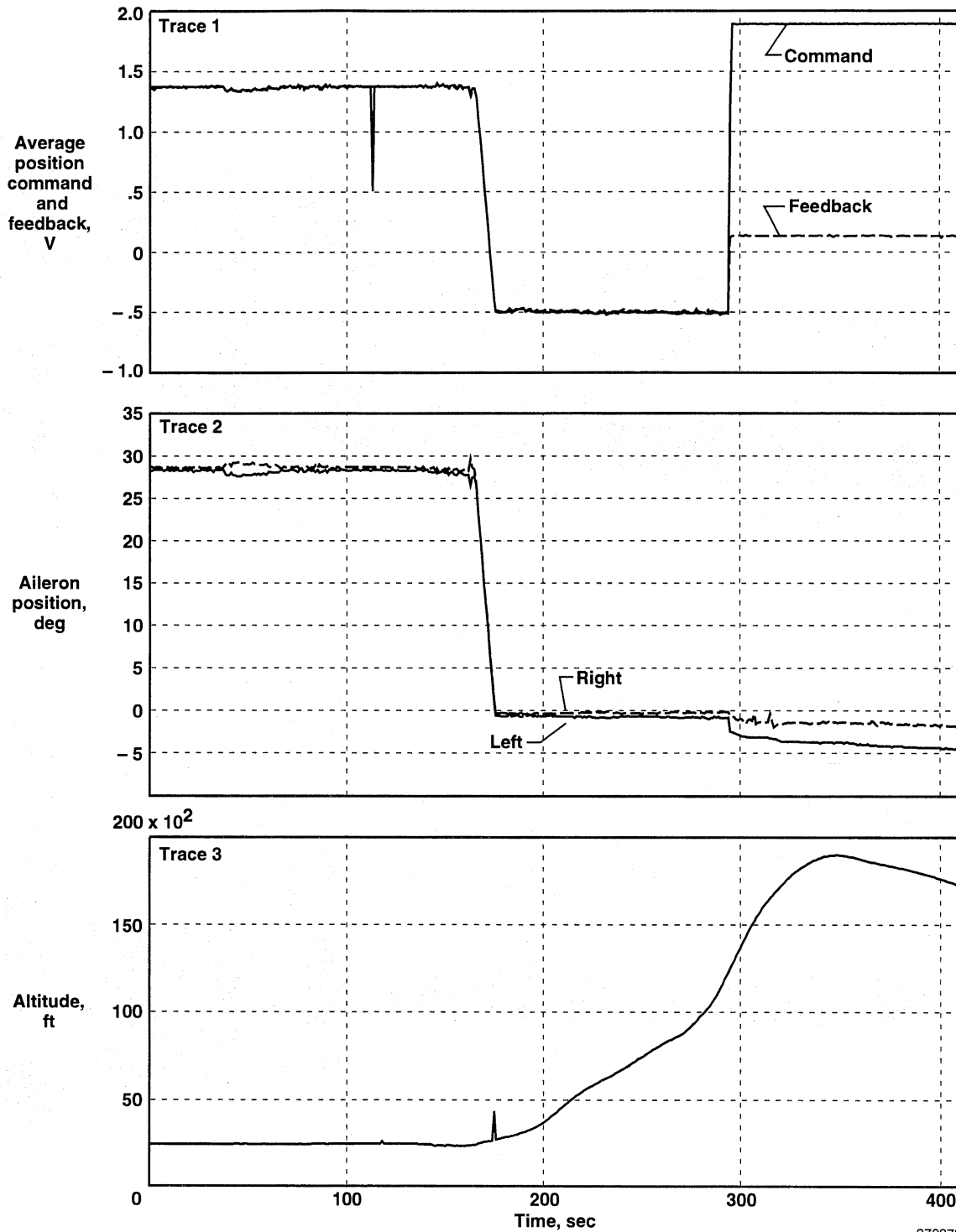
Figure 14. In-flight failure, January 10, 1997, flight 585.
