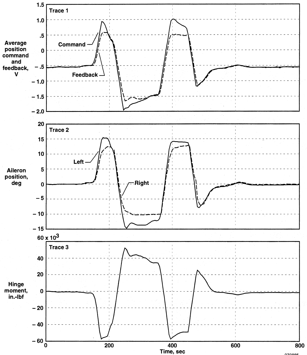
Figure 20. Abrupt aileron reversal—full stick (right).
