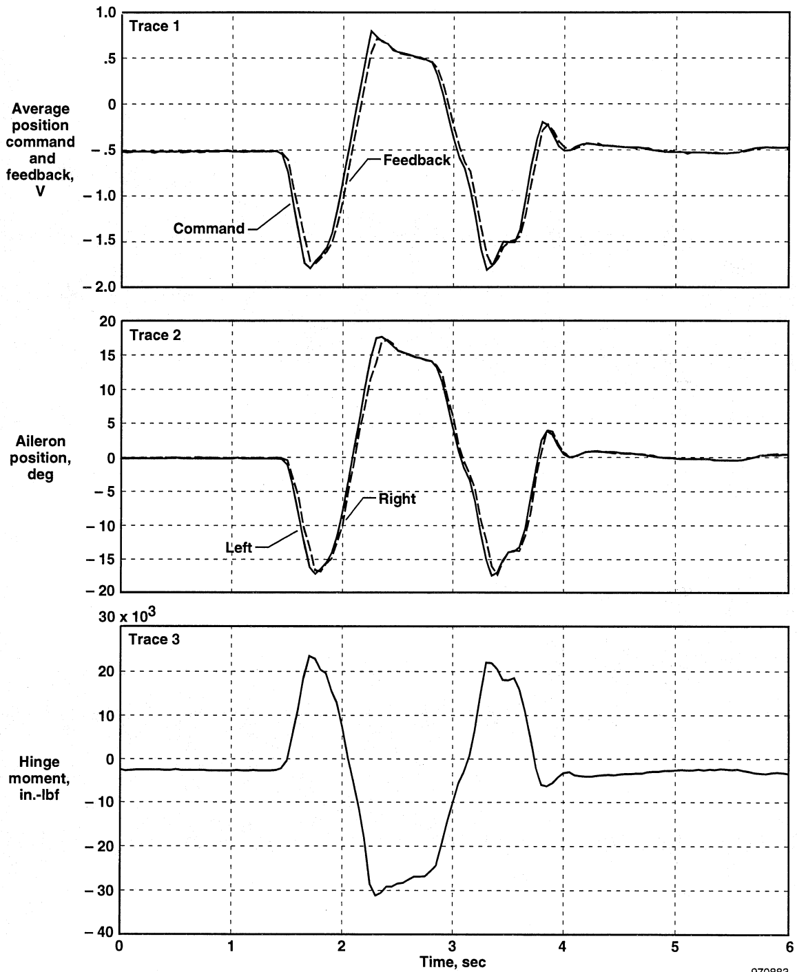
Figure 18. Abrupt aileron reversal—full stick (left).
