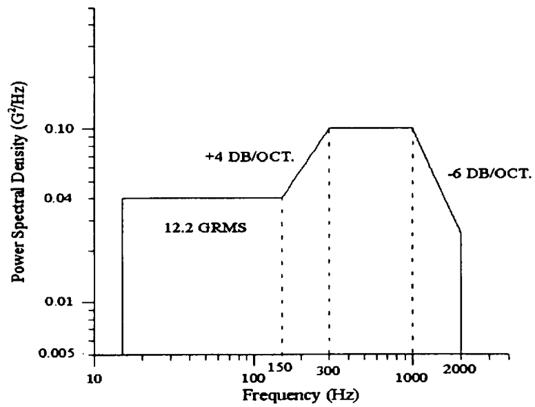
Figure 4: NASA ADFRF process specification No. 21-2.
