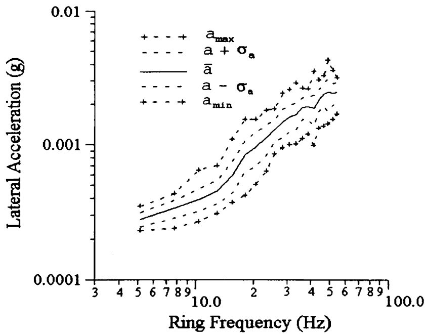
Figure 18: Statistical lateral response spectra of the circular ring without concentrated mass under random base excitation.
