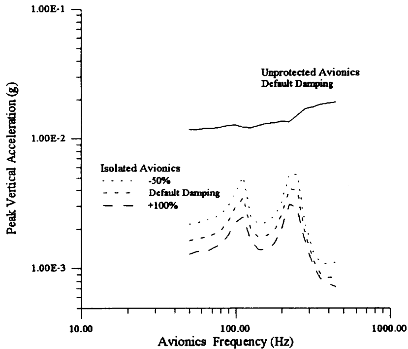
Figure 22: Vertical response spectra of an isolated avionics system with circular ring damping ratio variations as compared to unprotected avionics under random base excitation.
