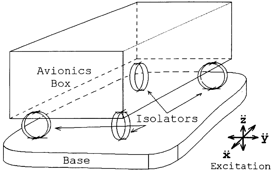
Figure 1: Circular ring isolation system for generic avionics equipment. .
