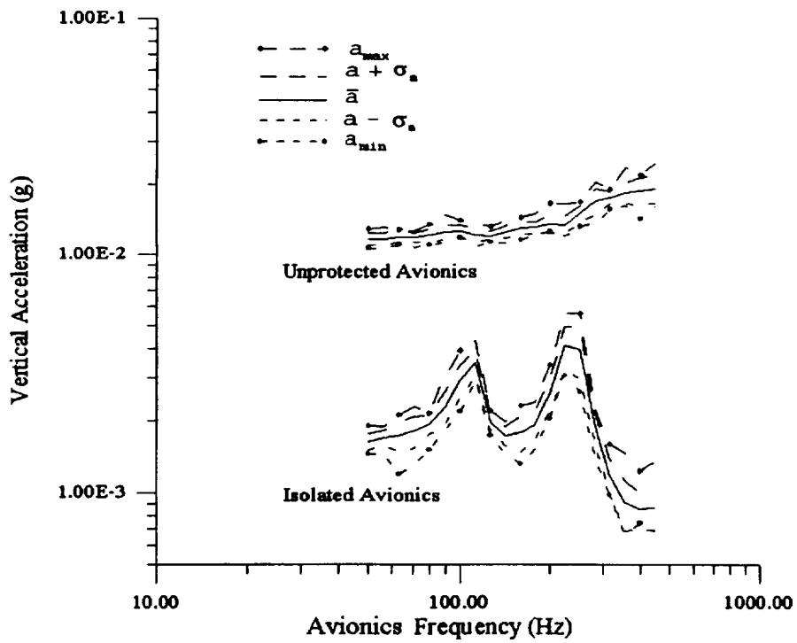
Figure 20: Comparison of vertical response spectra of avionics system with and without the circular ring under random base excitation - rigid mass avionics model.
