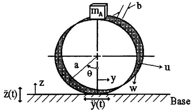
Figure 2: Circular ring structure.
