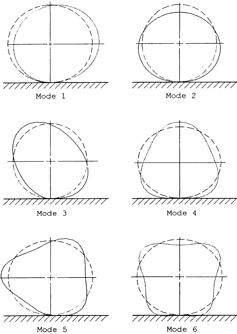
Figure 3: Circular ring mode shapes.
