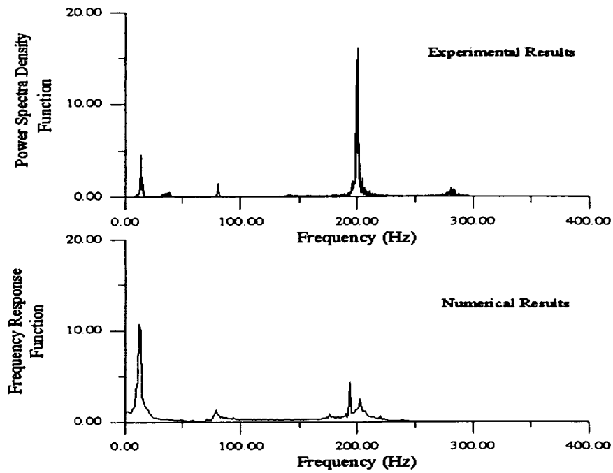
Figure 11: Comparison of analytical and experimental results for the circular steel ring for lateral excitation.
