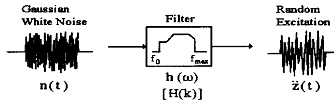
Figure 5: Random excitation model.
