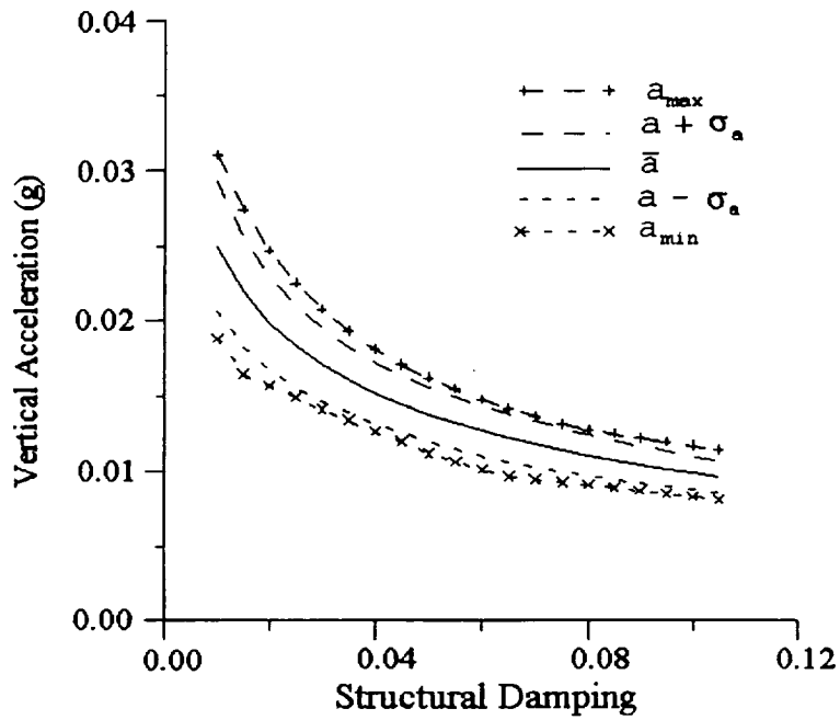
Figure 19: Statistical vertical response spectra of the circular ring as a function of damping under random base excitation.
