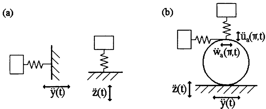
Figure 14: Single degree of freedom system configurations: (a) SDOF system exposed to random excitation without ring, (b) SDOF system exposed to transmitted vibration at top of ring.
