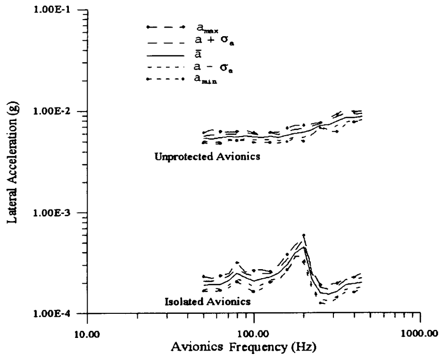
Figure 21: Comparison of lateral response spectra of avionics system with and without the circular ring under random base excitation - rigid mass avionics model.
