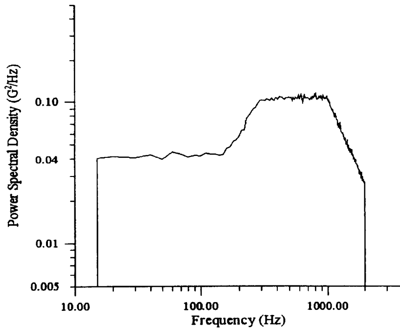
Figure 8: Frequency response of an ensemble average of 1000 time samples.
