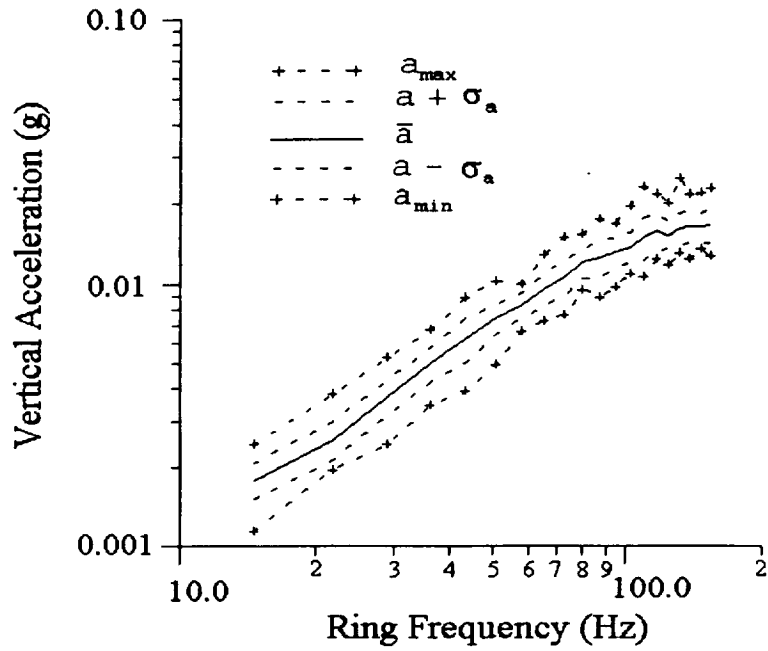
Figure 17: Statistical vertical response spectra of the circular ring without concentrated mass under random base excitation.
