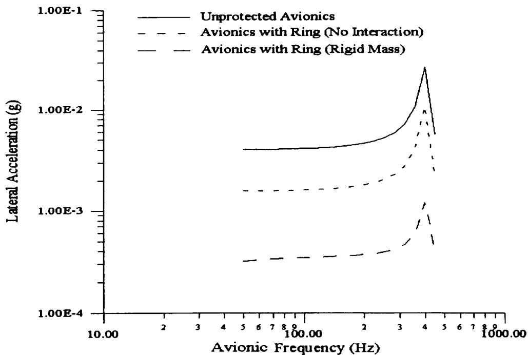
Figure 16: Comparison of lateral response spectra of an avionics system with and without the circular ring under sinusoidal base excitation.
