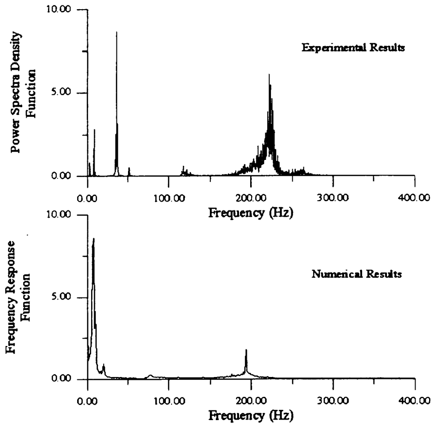
Figure 13: Comparison of analytical and experimental results for the circular steel ring with a 0.45 kg concentrated mass under lateral random base excitation.
