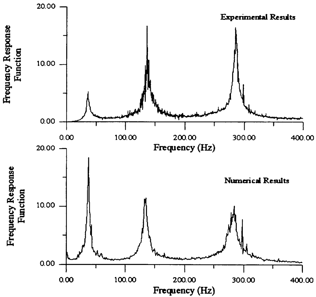
Figure 10: Comparison of analytical and experimental frequency response functions for the circular steel ring for vertical excitation.
