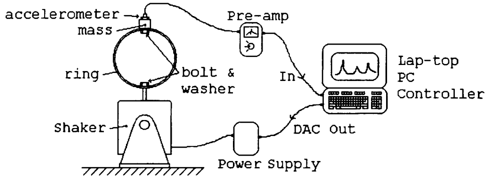
Figure 9: Experiment set-up for circular ring vibration.
