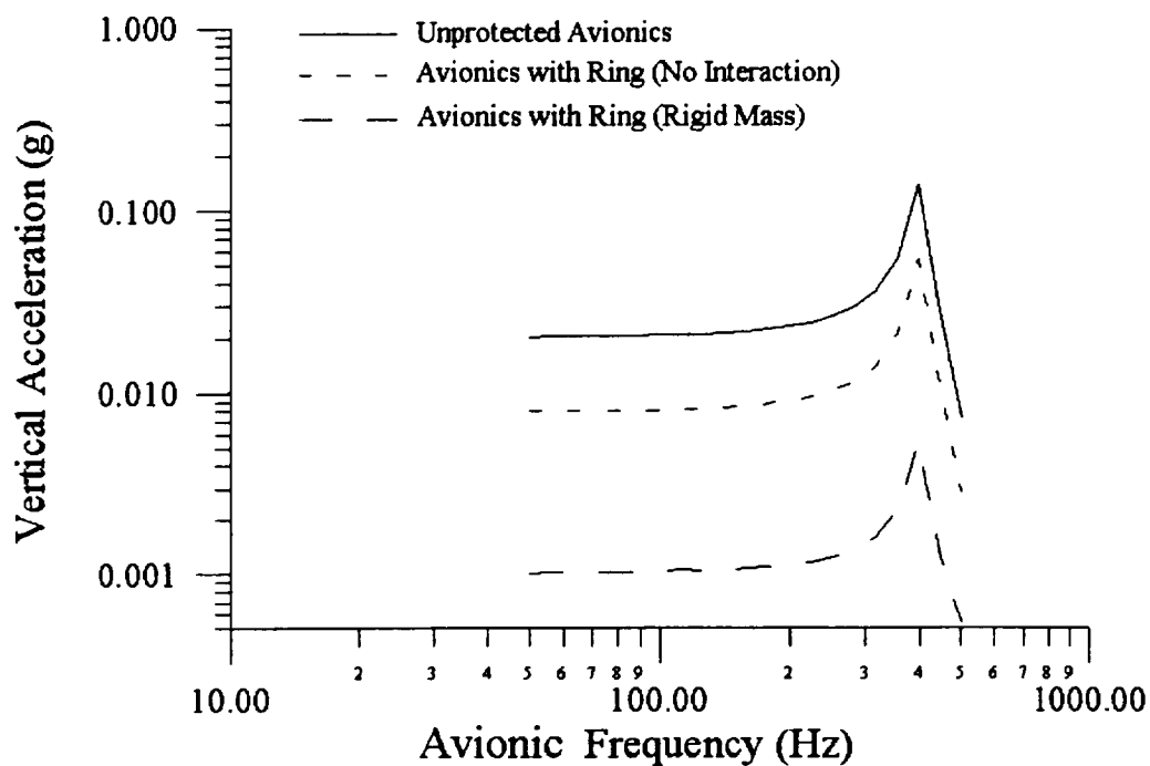
Figure 15: Comparison of vertical response spectra of an avionics system with and without the circular ring under sinusoidal base excitation.
