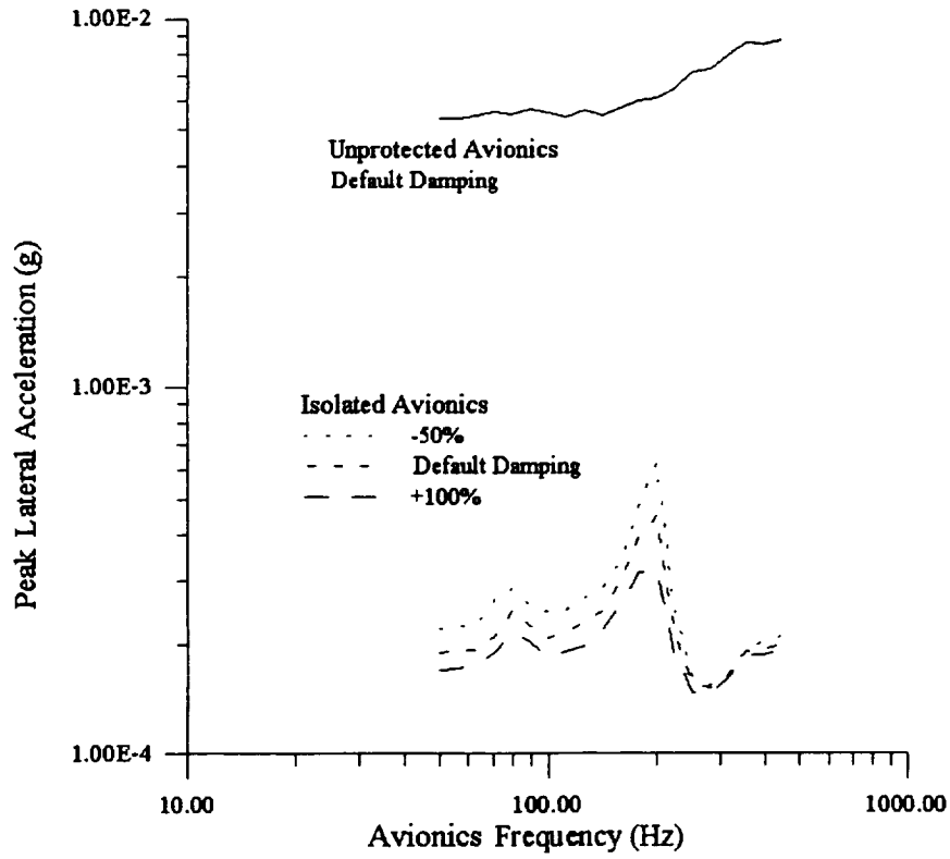
Figure 23: Lateral response spectra of an isolated avionics system with circular ring damping ratio variations as compared to unprotected avionics under random base excitation.
