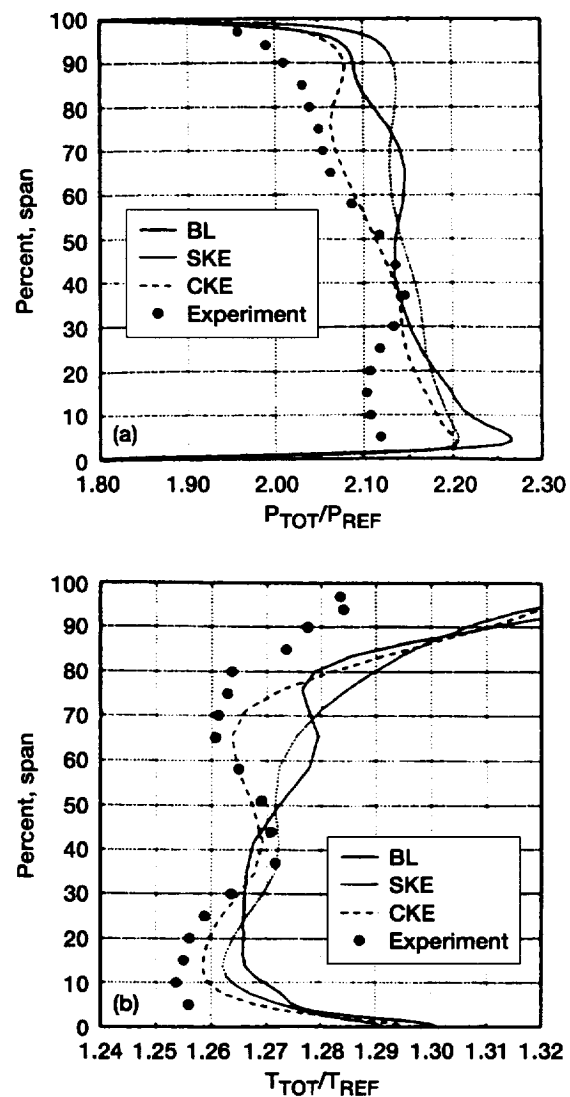
Figure 9.—The axisymmetric profiles of (a) normalized total pressure and (b), normalized total temperature, at station 4 (Shabbir, ref. 8).
