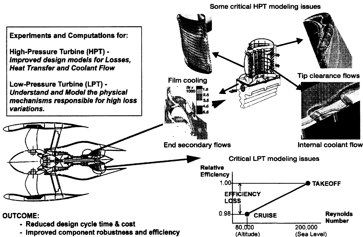
Figure 16.—Aerodynamics and heat transfer research for turbines (Gaugler).
