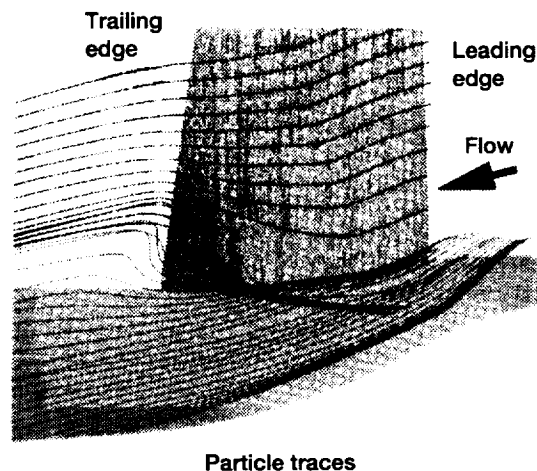
Figure 15.—Calculated flow near hub (Hah, ref. 10).
