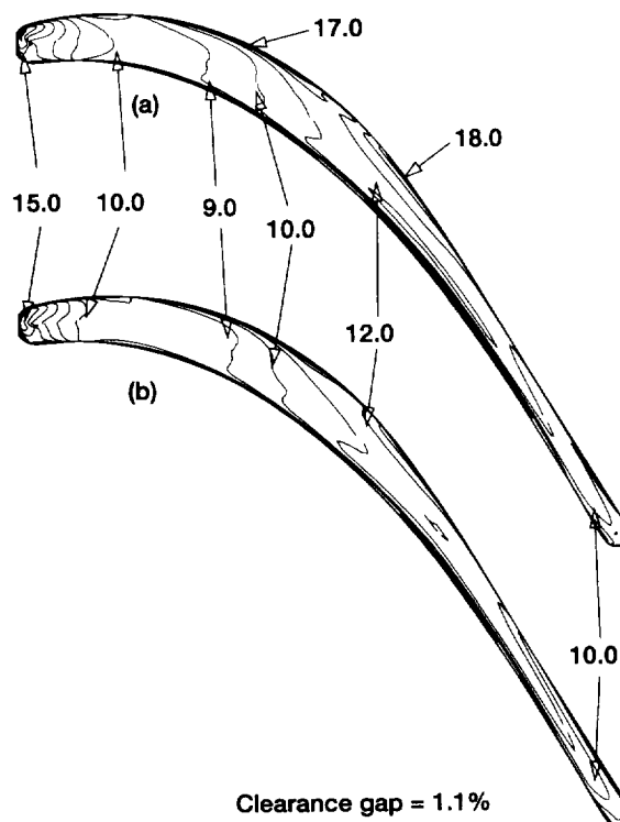
Figure 31.—Effect of grid density on the predicted tip heat transfer (Stx 1000). (a) 32 and (b) 40 radial cells in the tip clearance (Ameri & Steinthorsson, ref. 17).
