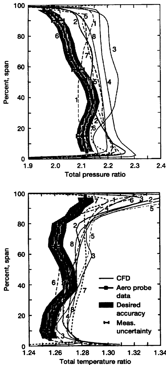
Figure 8.—CFD blind test case results: radial distribution of total pressure and total temperature ratio (Suder, ref. 5).
