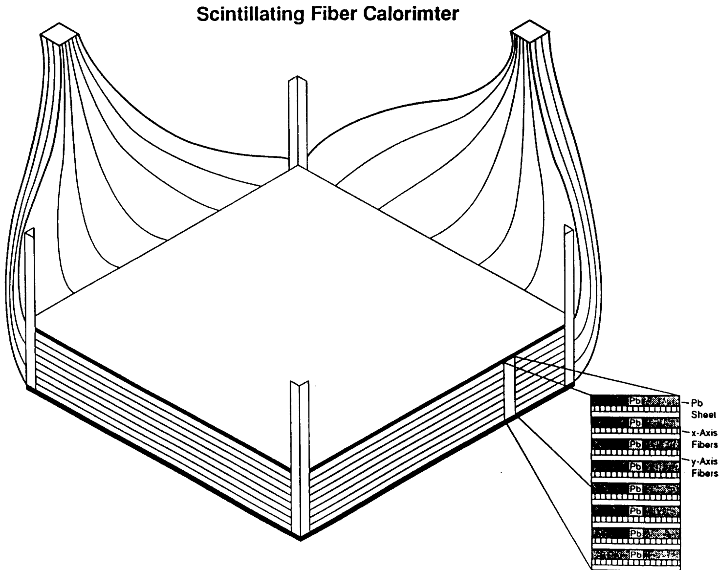
Fig. 2. Geometry of Scintillating Fiber Calorimeter (SOFICAL).
