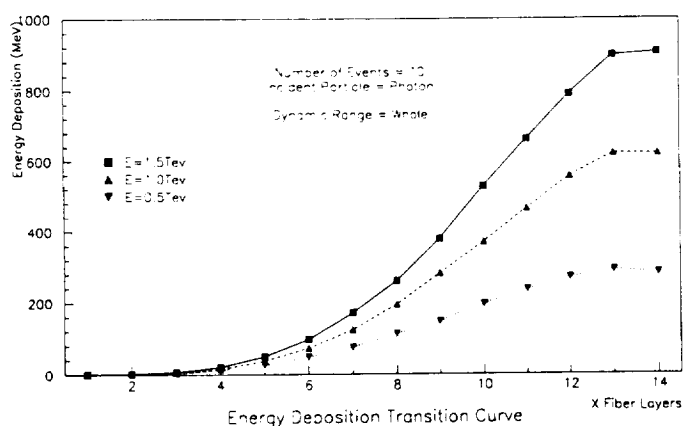
Fig. 4. The energy transition curve of a photon with energies of 0.5 TeV, 1 TeV, and 1.5 TeV.
