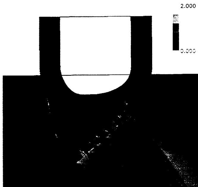
Figure 5: Mach number contours: final configuration - NPR = 2.5, midsection fore-aft cut, 30-degree vector
