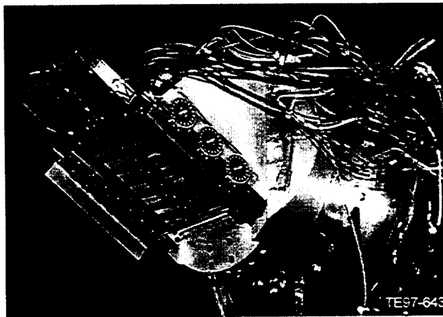
Figure 11: TEVEN nozzle model setup: 30-degree vectoring - 40-degree turning using hoods and 20-degree vectoring using guide vanes
