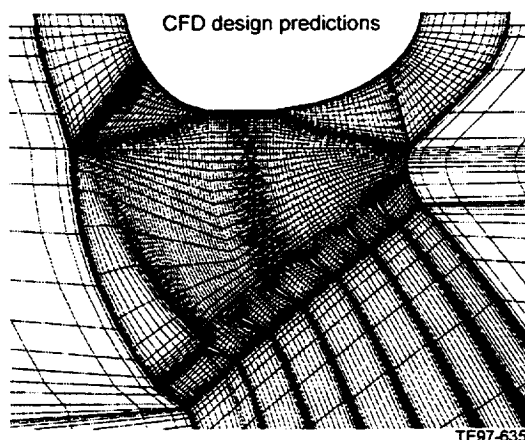
Figure 3: Typical LiftFan™ nozzle analysis grid: grid generation using GRIDGEN code
