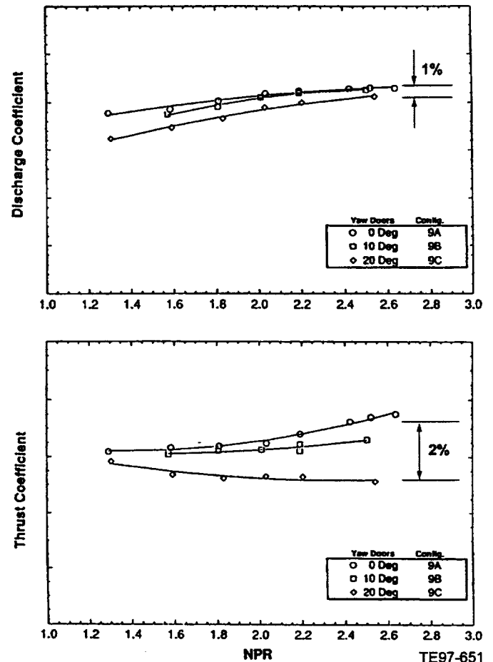
Figure 19: Effect of post-exit yaw doors on vaned nozzle performance, 70-degree vector
