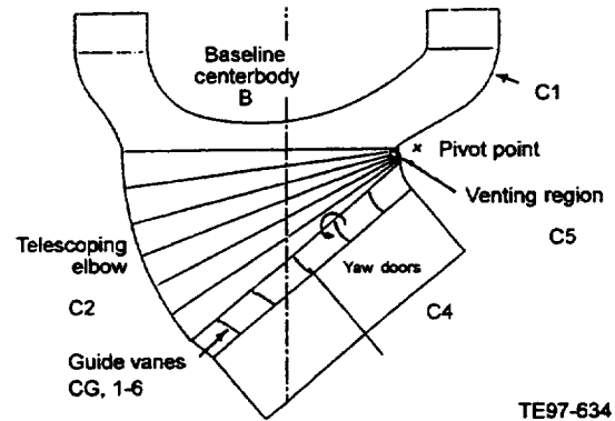
Figure 2: Schematic of TEVEN nozzle design
