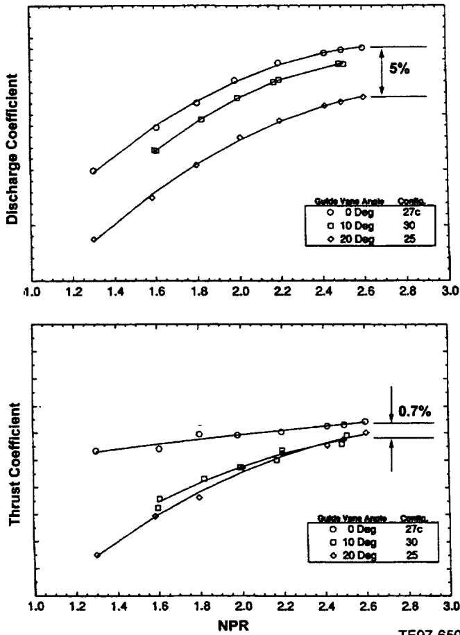
Figure 18: Effect of aft vectoring of guide vanes on nozzle performance, over/HP venting, 50-degree vector
