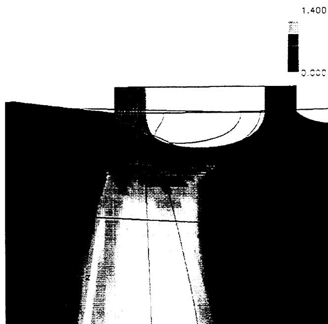
Figure 4: Mach number contours: initial configuration - NPR = 2.5, midsection fore-aft cut, 90-degree vector
