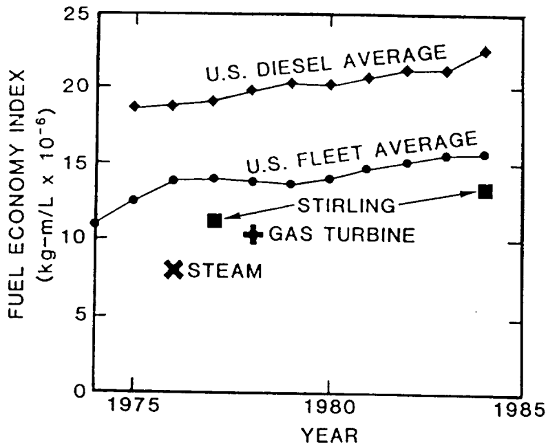
FIG. 7: FUEL ECONOMY INDEX FOR VARIOUS ENGINE TYPES
