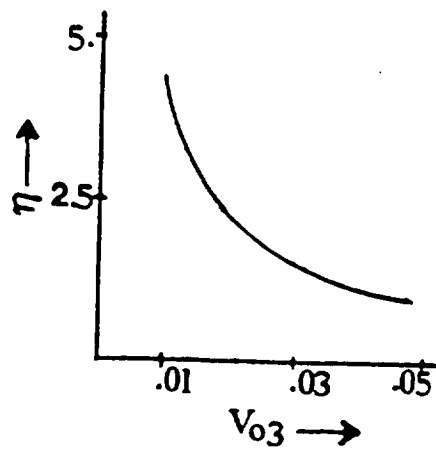
FIG. 22: RATIO ( \eta ) AS FUNCTION OF THIRD HARMONIC VOLTAGE
