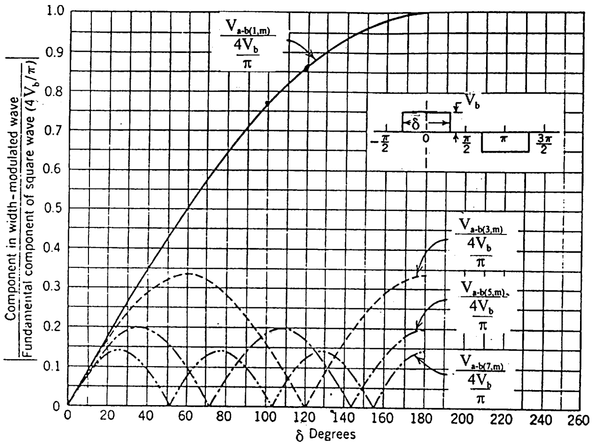
FIG. 14: RESONANT INVERTER OUTPUT CHARACTERISTICS WITH DELTA ANGLE
