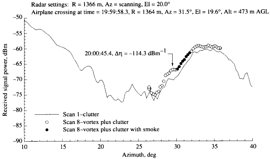
Figure A10. Total signal level vs. antenna azimuth angle compared with clutter scan for pass 54, azimuth scan 8, on 01-09-95.
