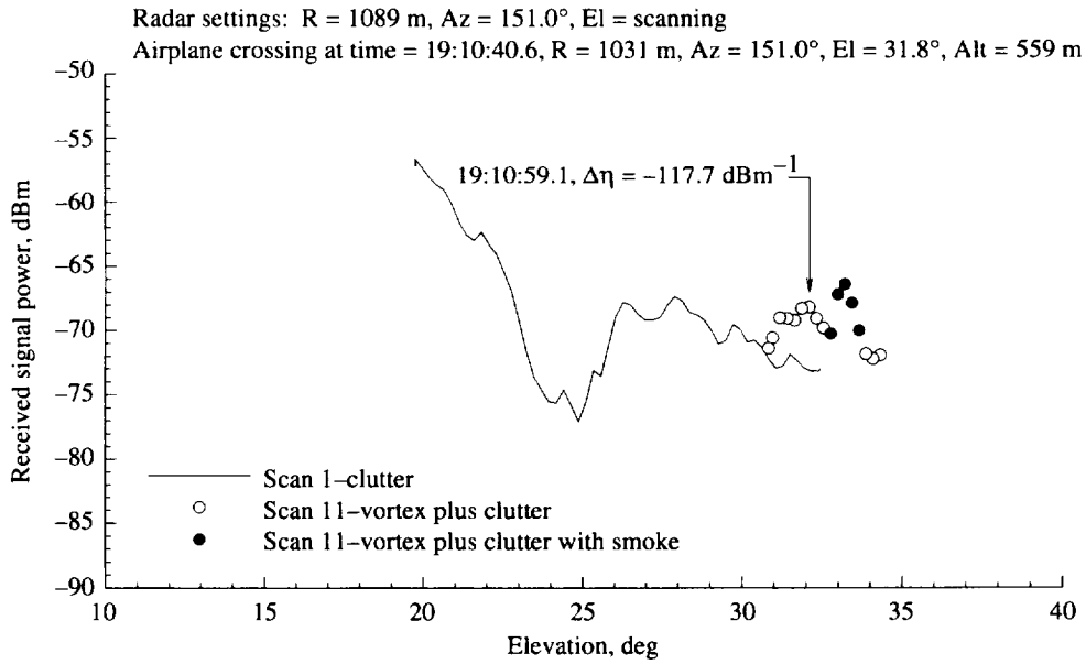
Figure A69. As for figure A68, except for elevation scan 11.
