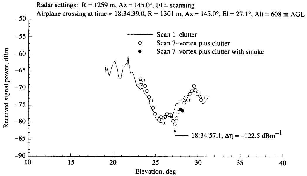
Figure A63. Total signal level vs. antenna elevation angle compared with clutter scan for pass 132, elevation scan 7, on 01-11-95.
