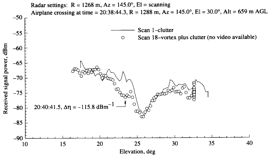
Figure A3. As for figure A1, except for elevation scan 18.
