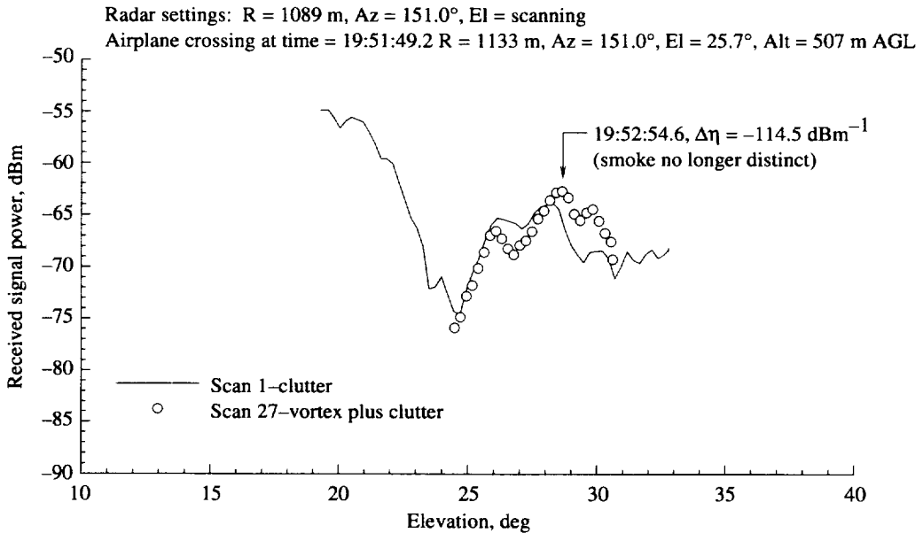
Figure A77. As for figure A76, except for elevation scan 27.
