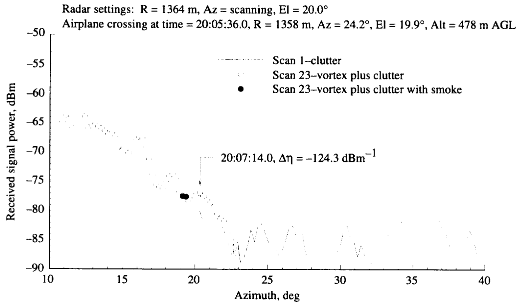
Figure A27. As for figure A25, except for azimuth scan 23.
