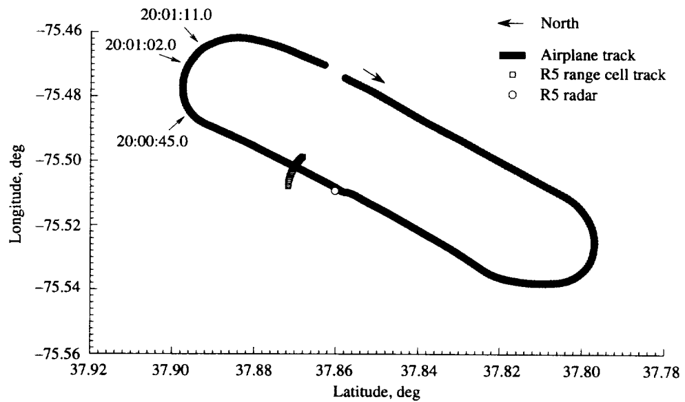
Figure A13. Pass 54 airplane and Radar 5 ground tracks; tail-on radar view of airplane wake.
