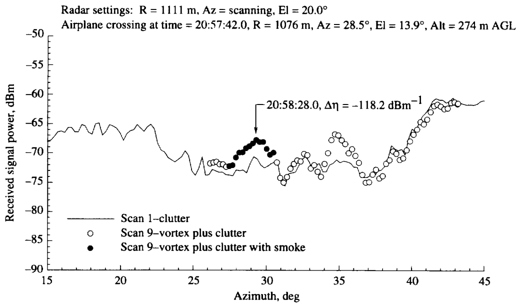
Figure A16. Total signal level vs. antenna azimuth angle compared with clutter scan for pass 64, azimuth scan 9, on 01-09-95.
