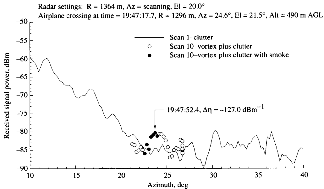
Figure A19. As for figure A18, except for azimuth scan 10.
