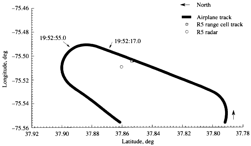
Figure A78. Pass 143 airplane and Radar 5 ground tracks; lateral radar view of airplane wake.
