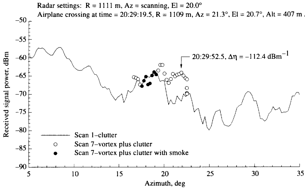
Figure A41. Total signal level vs. antenna azimuth angle compared with clutter scan for pass 108, azimuth scan 7, on 01-10-95.
