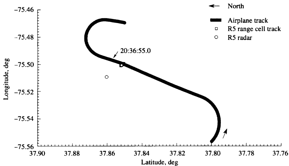
Figure A80. Pass 149 airplane and Radar 5 ground tracks; lateral radar view of airplane wake.
