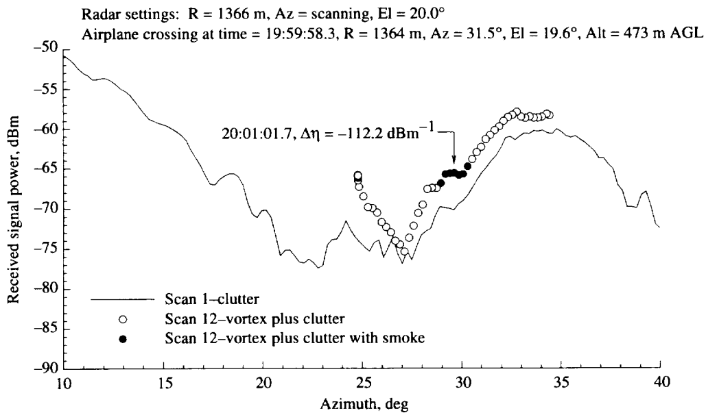
Figure A11. As for figure A10, except for azimuth scan 12.
