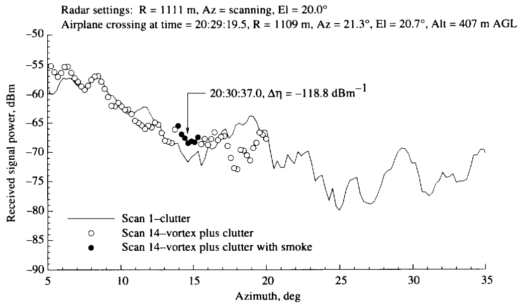
Figure A42. As for figure A41, except for azimuth scan 14.
