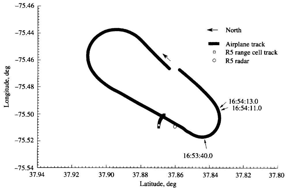
Figure A50. Pass 117 airplane and Radar 5 ground tracks; head-on radar view of airplane wake.
