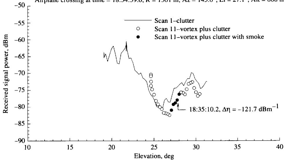
Figure A66. As for figure A63, except for elevation scan 11.
