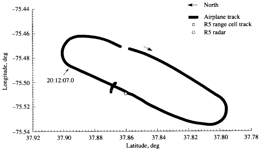
Figure A15. Pass 56 airplane and Radar 5 ground tracks; tail-on radar view of airplane wake.
