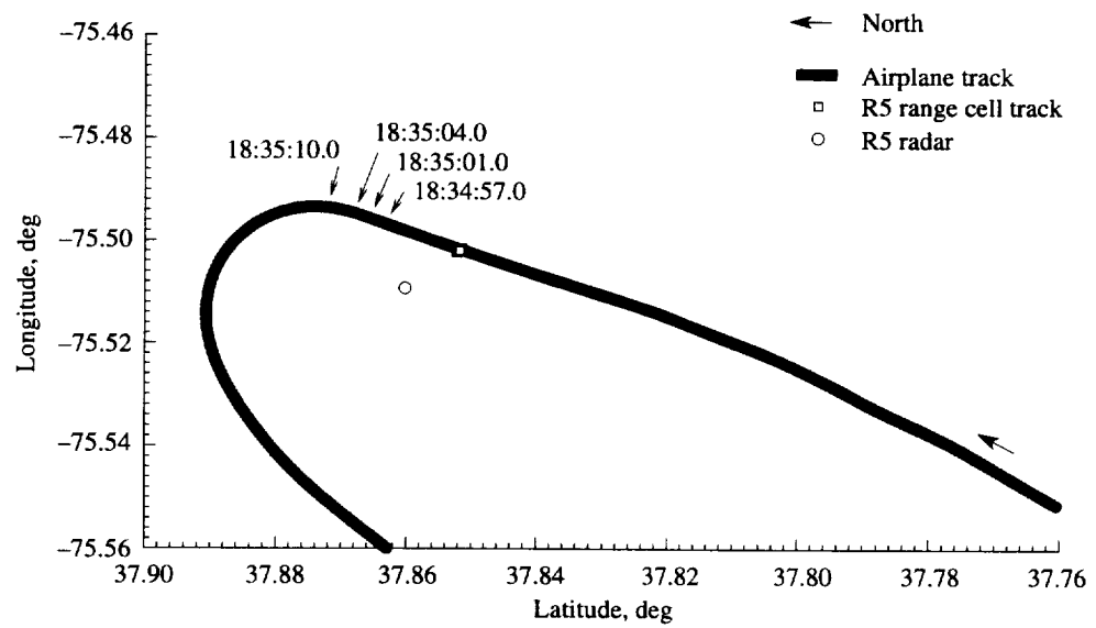
Figure A67. Pass 132 airplane and Radar 5 ground tracks; lateral radar view of airplane wake.
