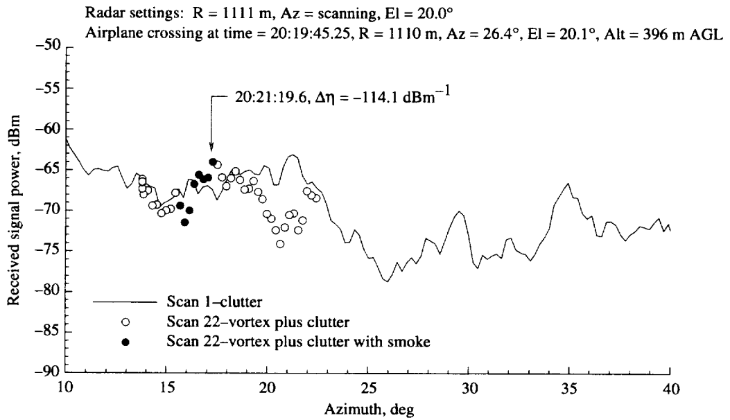
Figure A35. As for figure A33, except for azimuth scan 22.
