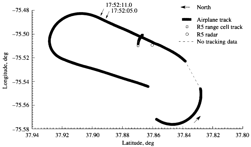
Figure A62. Pass 127 airplane and Radar 5 ground tracks; tail-on radar view of airplane wake.
