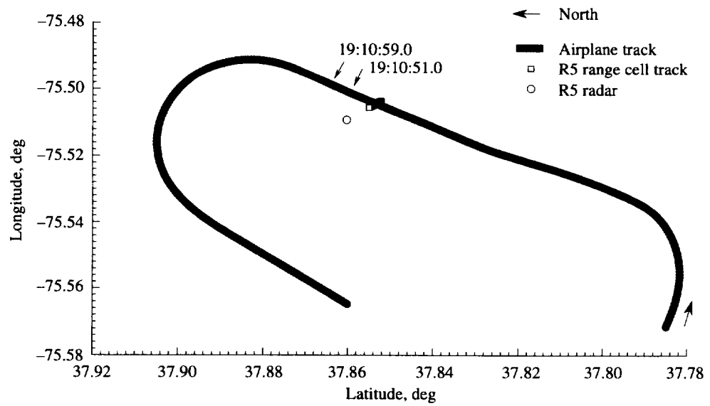
Figure A70. Pass 137 airplane and Radar 5 ground tracks; lateral radar view of airplane wake.
