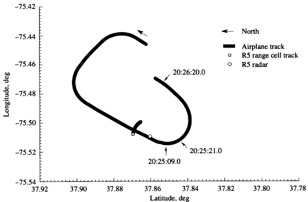
Figure A40. Pass 107 airplane and Radar 5 ground tracks; head-on radar view of airplane wake.
