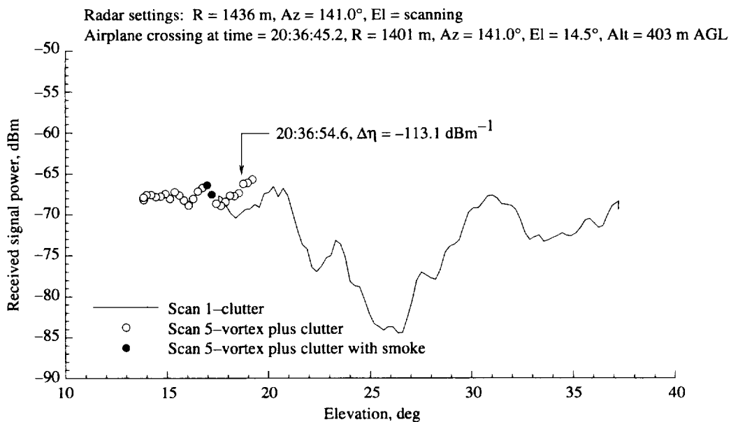
Figure A79. Total signal level vs. antenna elevation angle compared with clutter scan for pass 149, elevation scan 5, on 01-11-95.
