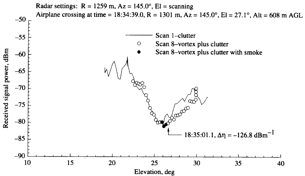
Figure A64. As for figure A63, except for elevation scan 8.
