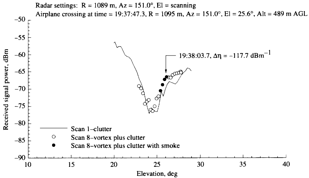
Figure A72. As for figure A71, except for elevation scan 8.
