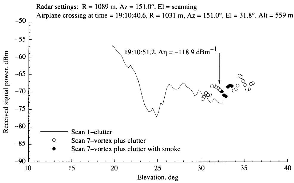
Figure A68. Total signal level vs. antenna elevation angle compared with clutter scan for pass 137, elevation scan 7, on 01-11-95.
