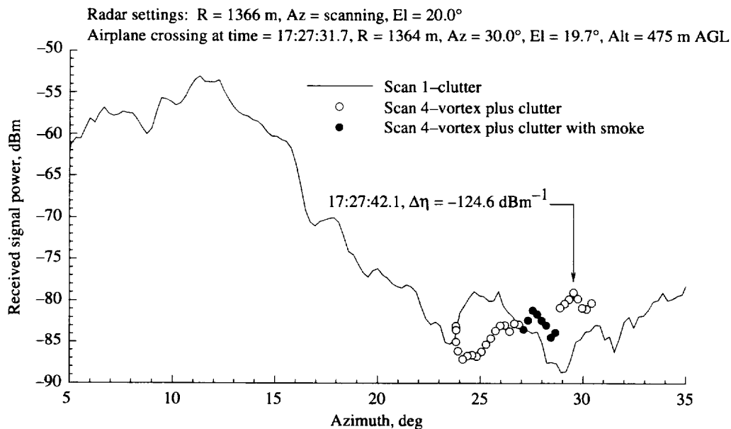
Figure A56. Total signal level vs. antenna azimuth angle compared with clutter scan for pass 123, azimuth scan 4, on 01-11-95.
