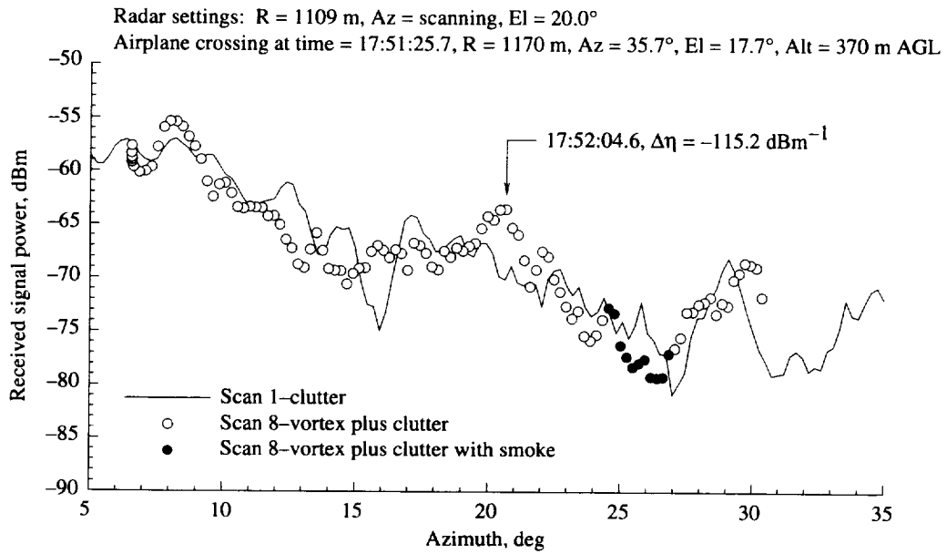
Figure A60. Total signal level vs. antenna azimuth angle compared with clutter scan for pass 127, azimuth scan 8, on 01-11-95.
