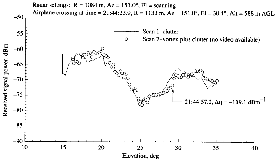
Figure A5. Total signal level vs. antenna elevation angle compared with clutter scan for pass 21, elevation scan 7, on 01-05-95.
