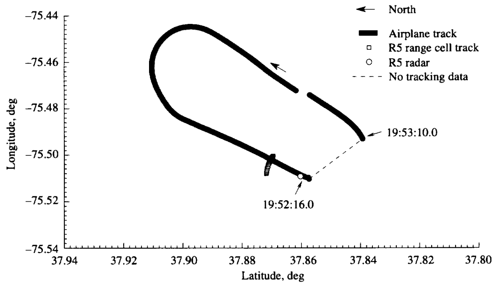
Figure A24. Pass 100 airplane and Radar 5 ground tracks; head-on radar view of airplane wake.
