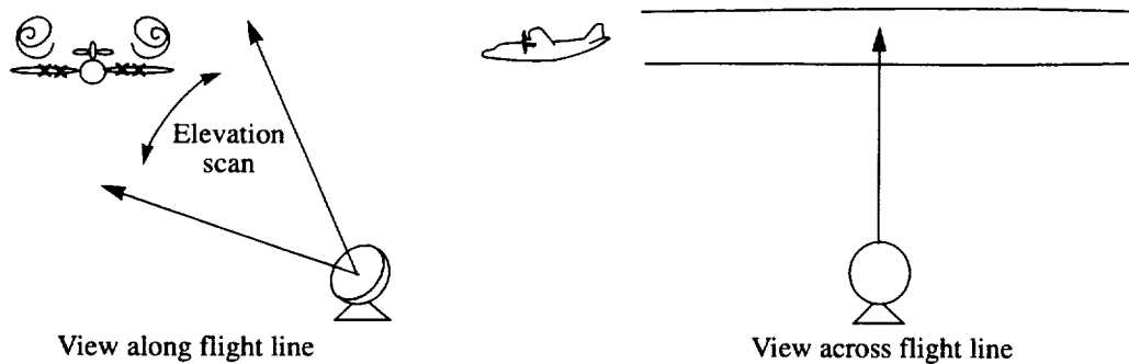
Figure 3. Elevation-scan configuration for airplane flying along side and past radar.
