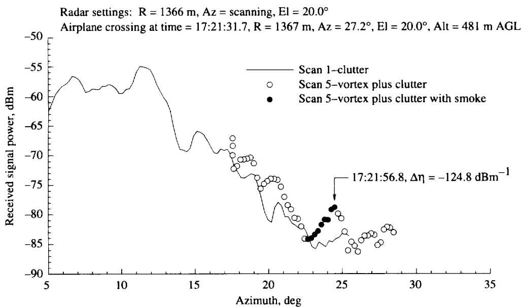
Figure A52. As for figure A51, except for azimuth scan 5.
