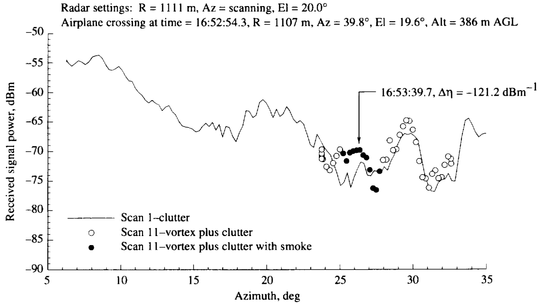
Figure A47. Total signal level vs. antenna azimuth angle compared with clutter scan for pass 117, azimuth scan 11, on 01-11-95.
