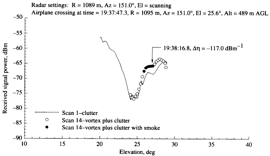
Figure A73. As for figure A71, except for elevation scan 14.
