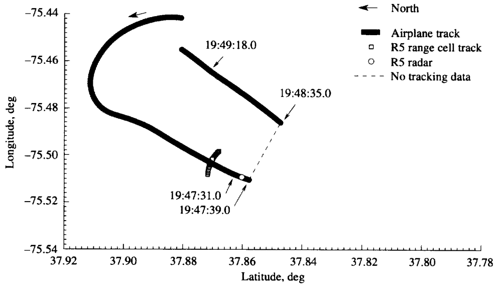
Figure A21. Pass 99 airplane and Radar 5 ground tracks; head-on radar view of airplane wake.
