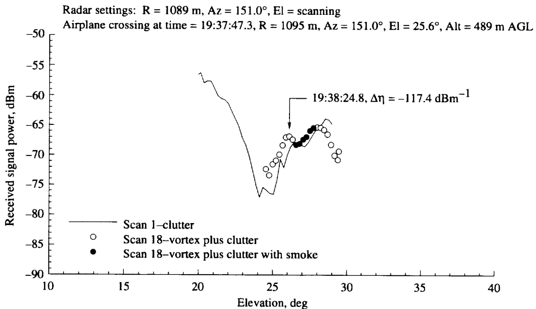
Figure A74. As for figure A71, except for elevation scan 18.
