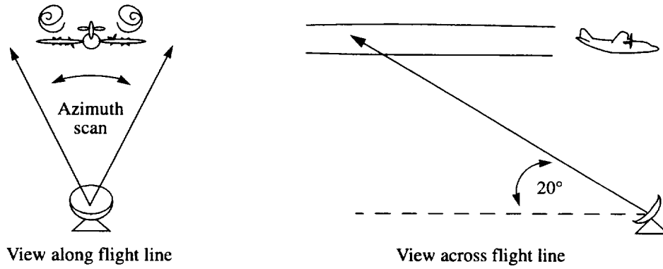
Figure 1. Head-on azimuth-scan configuration for airplane flying toward and over radar beam.
