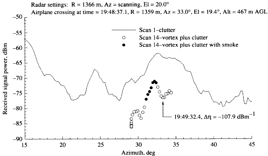
Figure A8. As for figure A7, except for azimuth scan 14.
