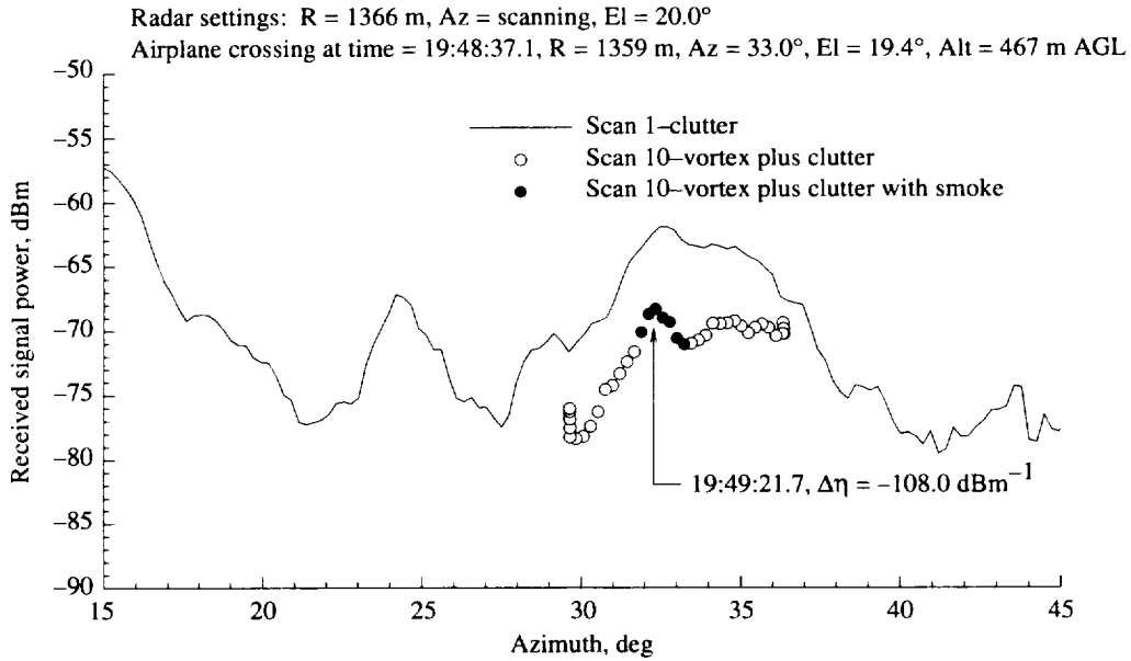
Figure A7. Total signal level vs. antenna azimuth angle compared with clutter scan for pass 52, azimuth scan 10, on 01-09-95.
