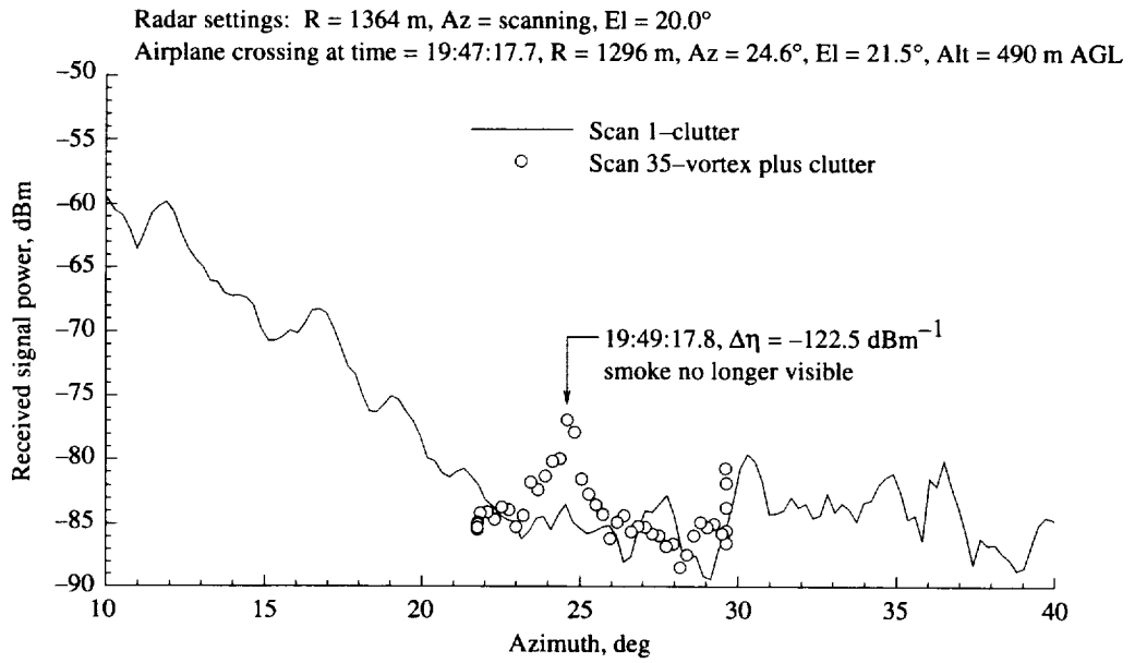
Figure A20. As for figure A18, except for azimuth scan 35.
