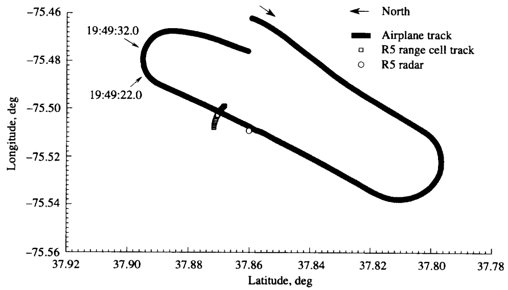
Figure A9. Pass 52 airplane and Radar 5 ground tracks; tail-on radar view of airplane wake.
