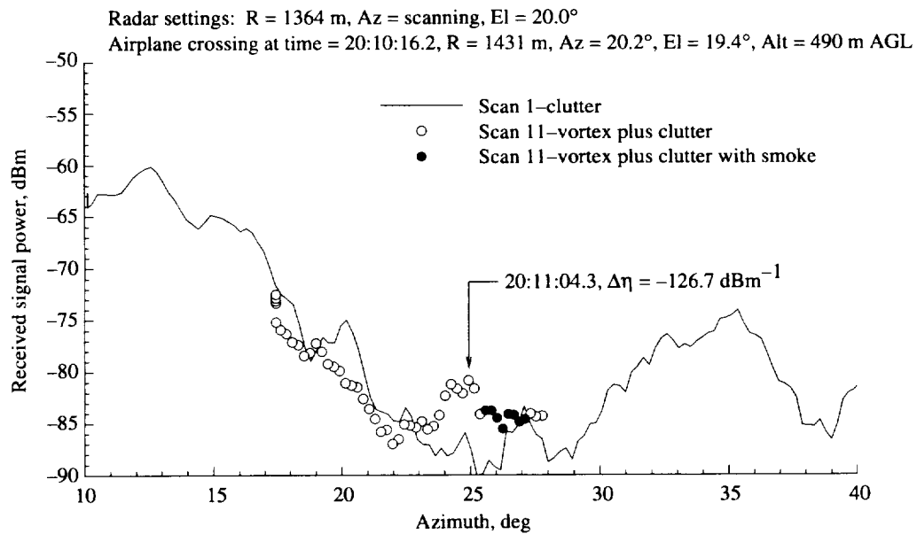
Figure A30. As for figure A29, except for azimuth scan 11.
