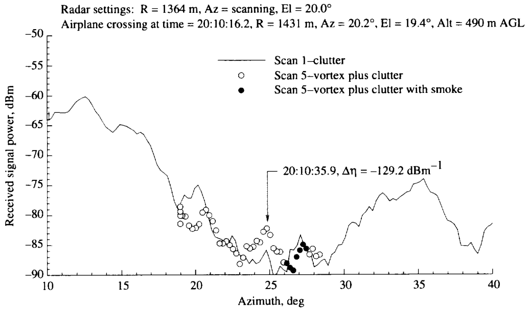
Figure A29. Total signal level vs. antenna azimuth angle compared with clutter scan for pass 104, azimuth scan 5, on 01-10-95.
