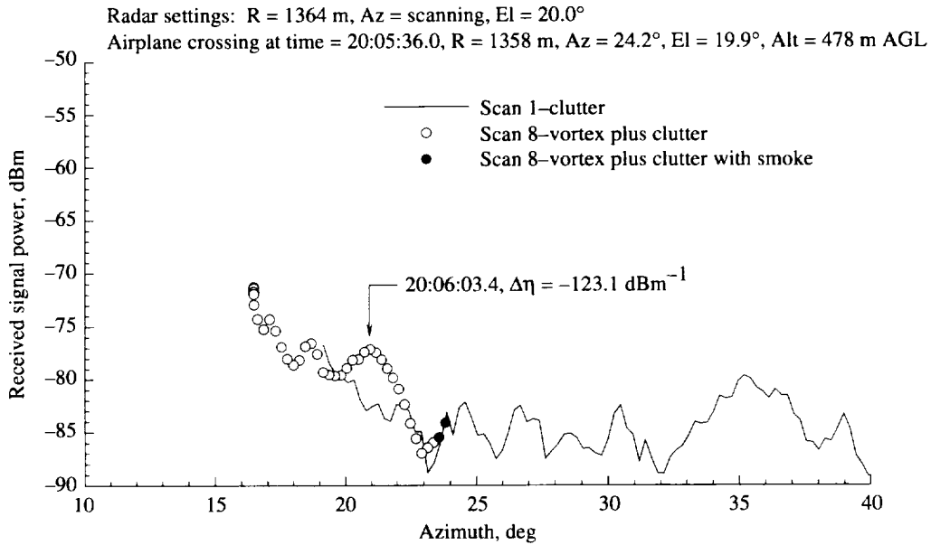
Figure A25. Total signal level vs. antenna azimuth angle compared with clutter scan for pass 103, azimuth scan 8, on 01-10-95.
