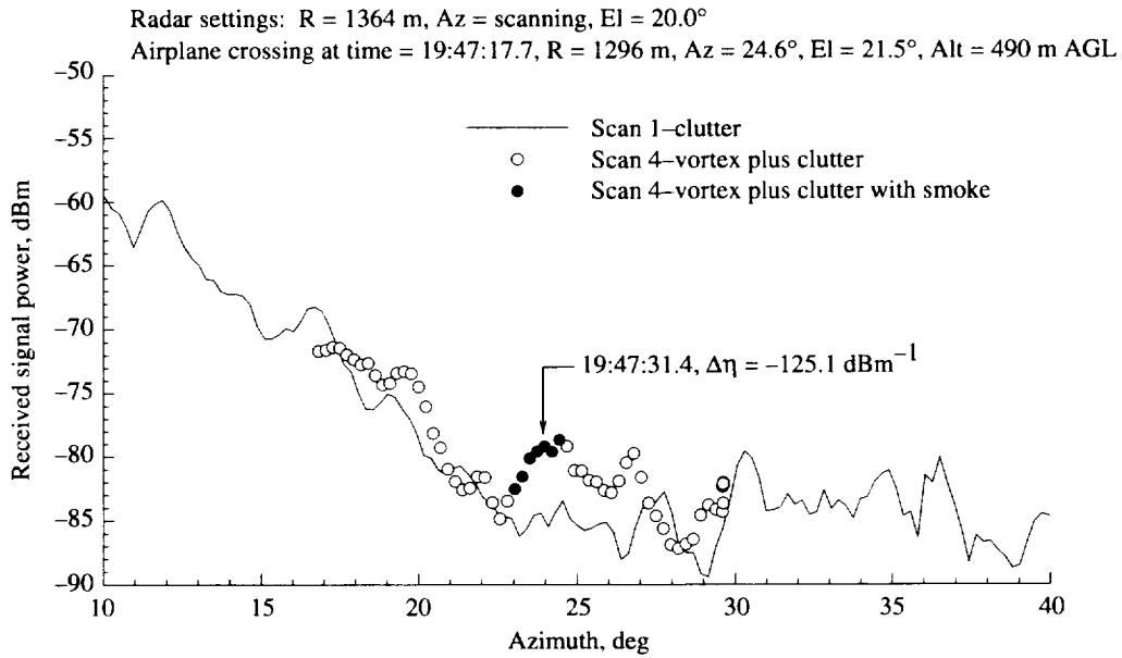
Figure A18. Total signal level vs. antenna azimuth angle compared with clutter scan for pass 99, azimuth scan 4, on 01-10-95.
