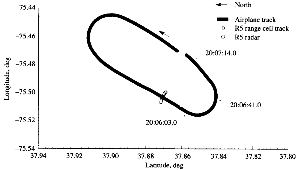
Figure A28. Pass 103 airplane and Radar 5 ground tracks; head-on radar view of airplane wake.
