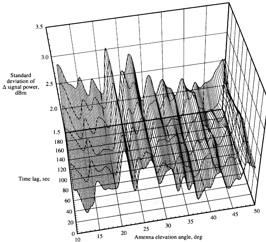
Figure 6. Variability of received clutter power with elevation direction; Wallops R5 at azimuth = 141° on 11/28/85 (data smoothed). At any given angular position and time lag, mean signal level change was negligible. Standard deviation of signal level change varied from 1.5 to 3.6 dBm before smoothing.
