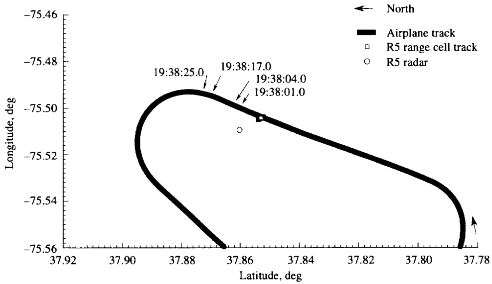
Figure A75. Pass 141 airplane and Radar 5 ground tracks; lateral radar view of airplane wake.
