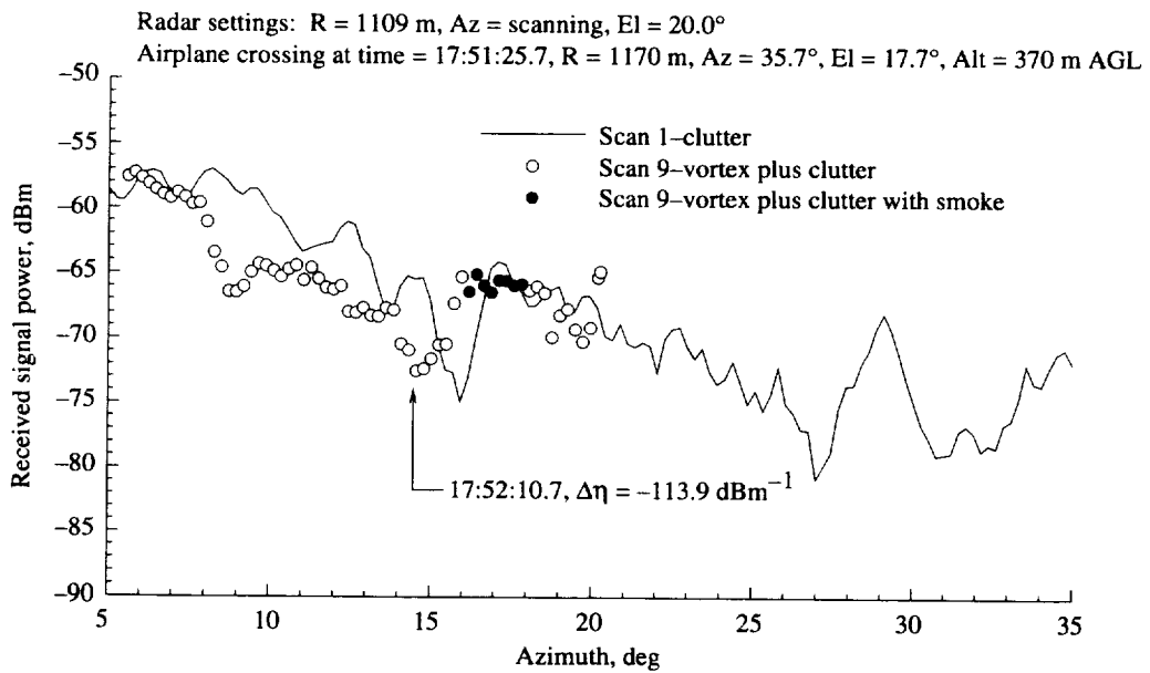
Figure A61. As for figure A60, except for azimuth scan 9.
