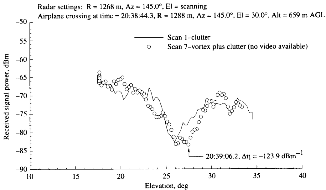
Figure A1. Total signal level vs. antenna elevation angle compared with clutter scan for pass 14, elevation scan 7, on 01-05-95.
