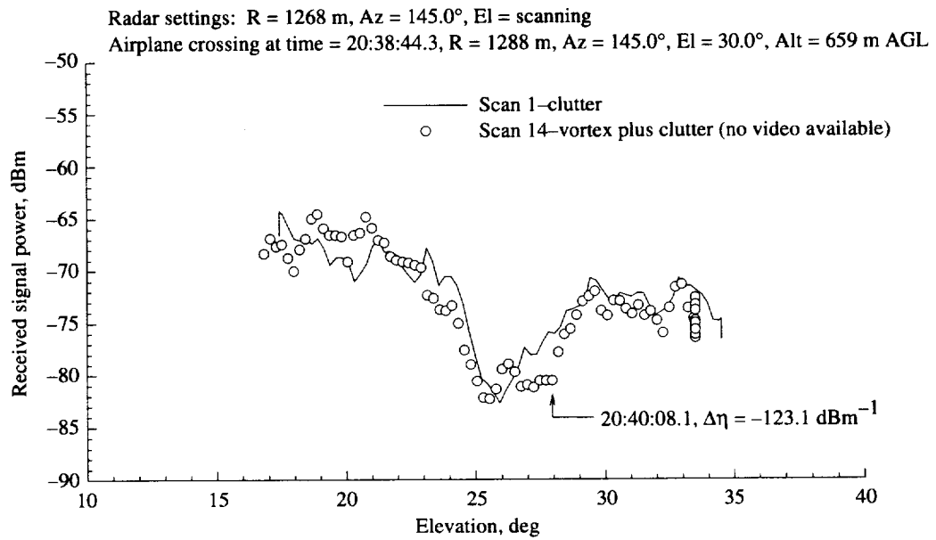
Figure A2. As for figure A1, except for elevation scan 14.
