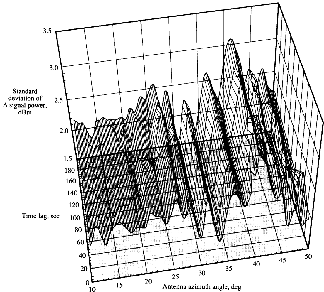
Figure 5. Variability of received clutter power with azimuth direction; Wallops R5 elevation = 20° on 11/28/95 (data smoothed). At any given angular position and time lag, mean signal level change was negligible. Standard deviation of signal level change varied from 1.4 to 3.7 dBm before smoothing.
