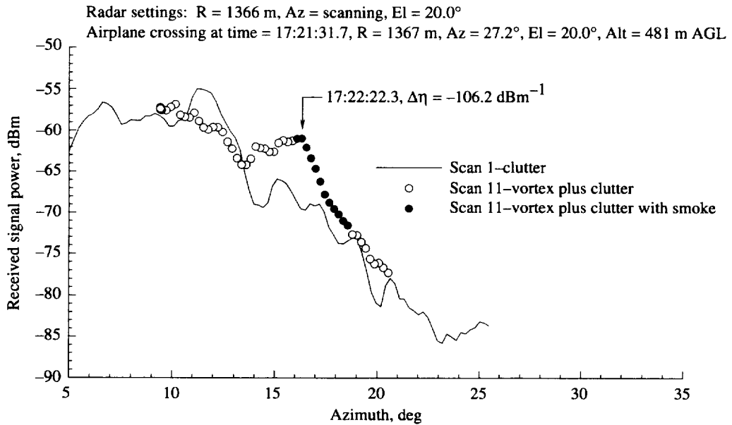
Figure A54. As for figure A51, except for azimuth scan 11.
