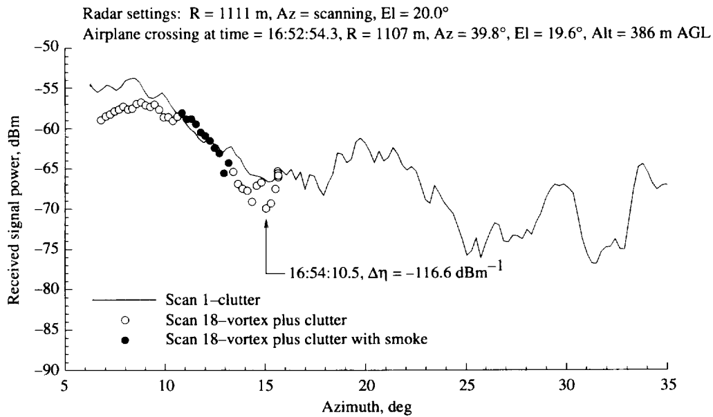
Figure A48. As for figure A47, except for azimuth scan 18.
