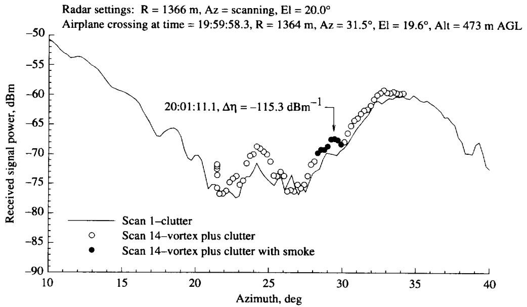
Figure A12. As for figure A10, except for azimuth scan 14.
