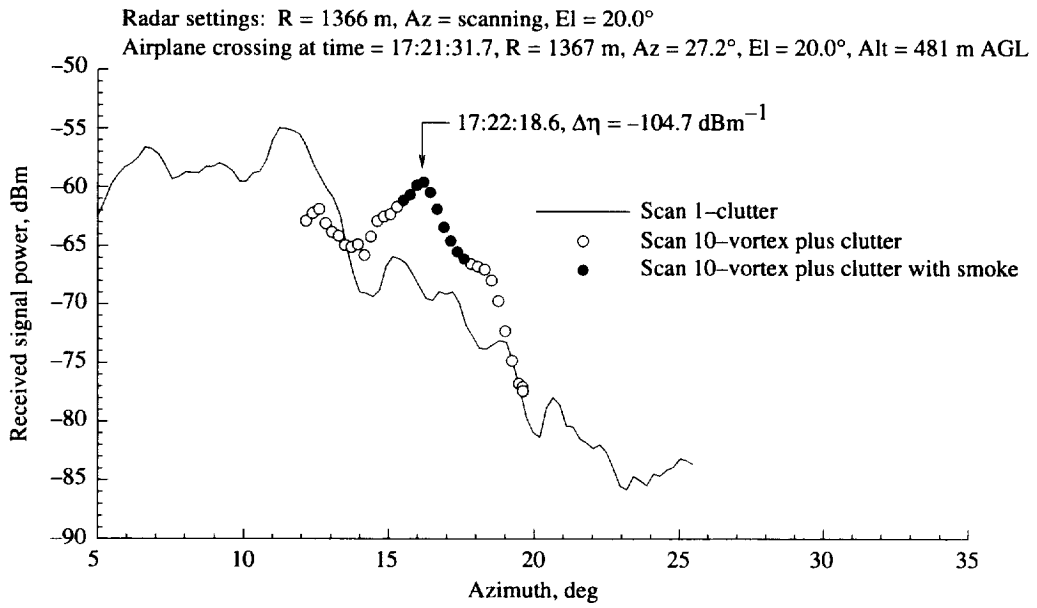
Figure A53. As for figure A51, except for azimuth scan 10.
