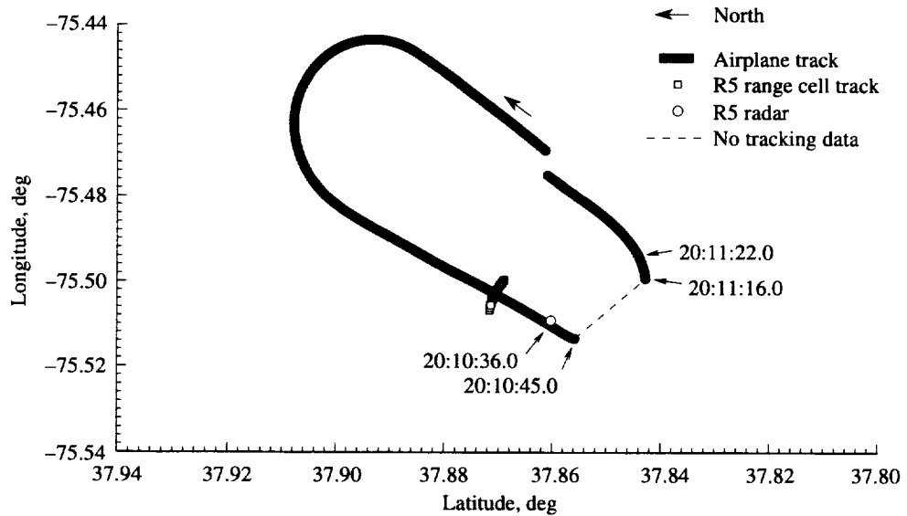
Figure A32. Pass 104 airplane and Radar 5 ground tracks; head-on radar view of airplane wake.
