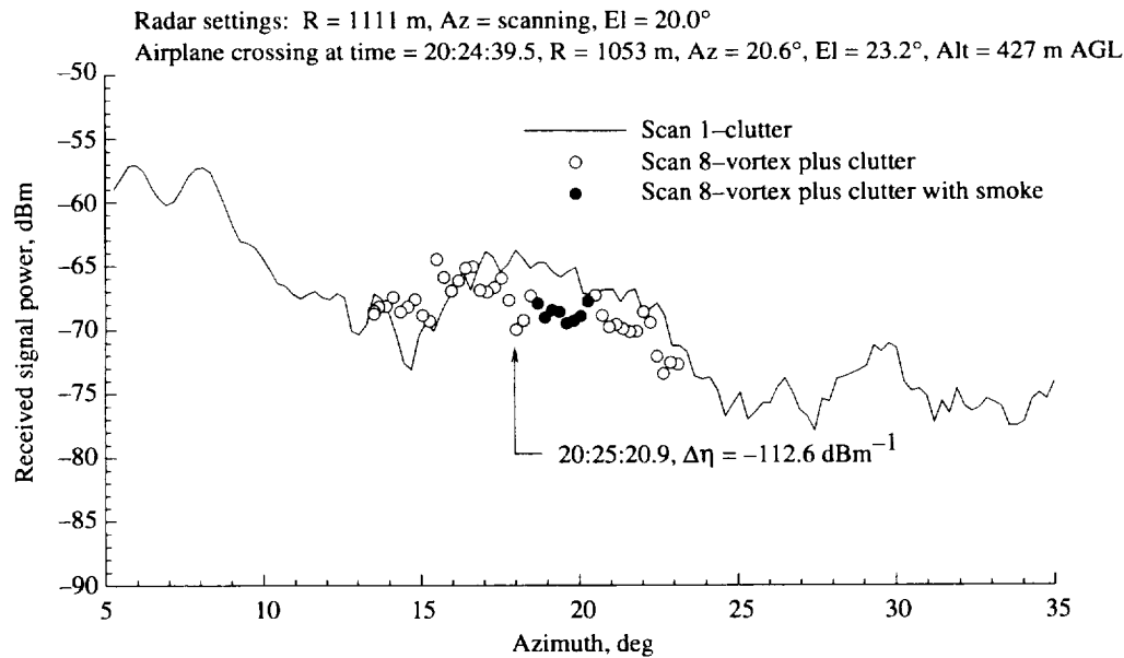
Figure A38. As for figure A37, except for azimuth scan 8.
