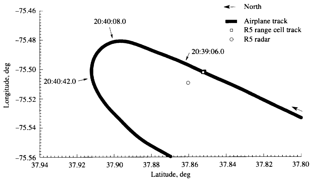
Figure A4. Pass 14 airplane and Radar 5 ground tracks; lateral radar view of airplane wake.
