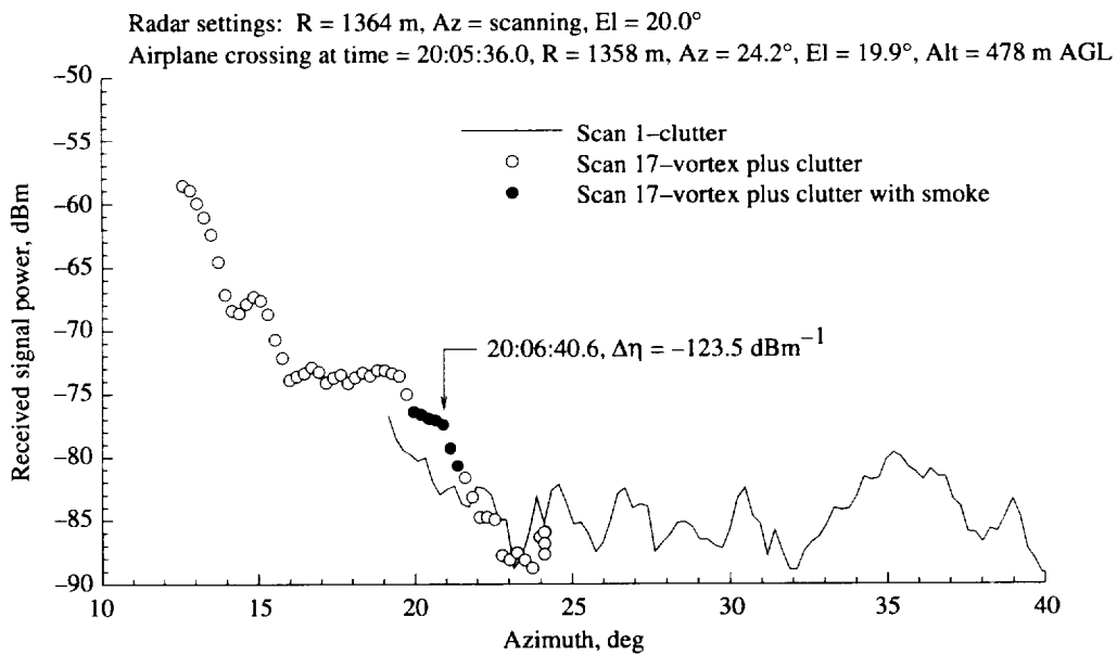
Figure A26. As for figure A25, except for azimuth scan 17.
