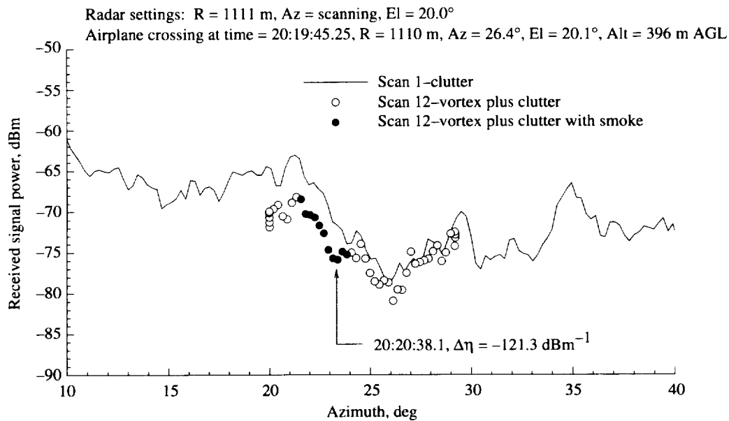
Figure A34. As for figure A33, except for azimuth scan 12.
