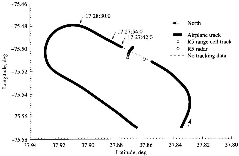
Figure A59. Pass 123 airplane and Radar 5 ground tracks; tail-on radar view of airplane wake.
