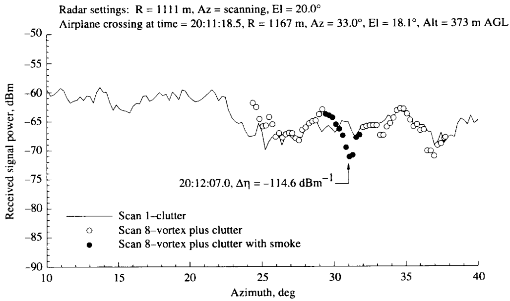
Figure A14. Total signal level vs. antenna azimuth angle compared with clutter scan for pass 56, azimuth scan 8, on 01-09-95.
