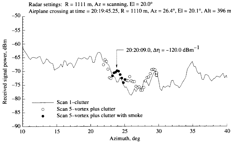
Figure A33. Total signal level vs. antenna azimuth angle compared with clutter scan for pass 106, azimuth scan 5, on 01-10-95.
