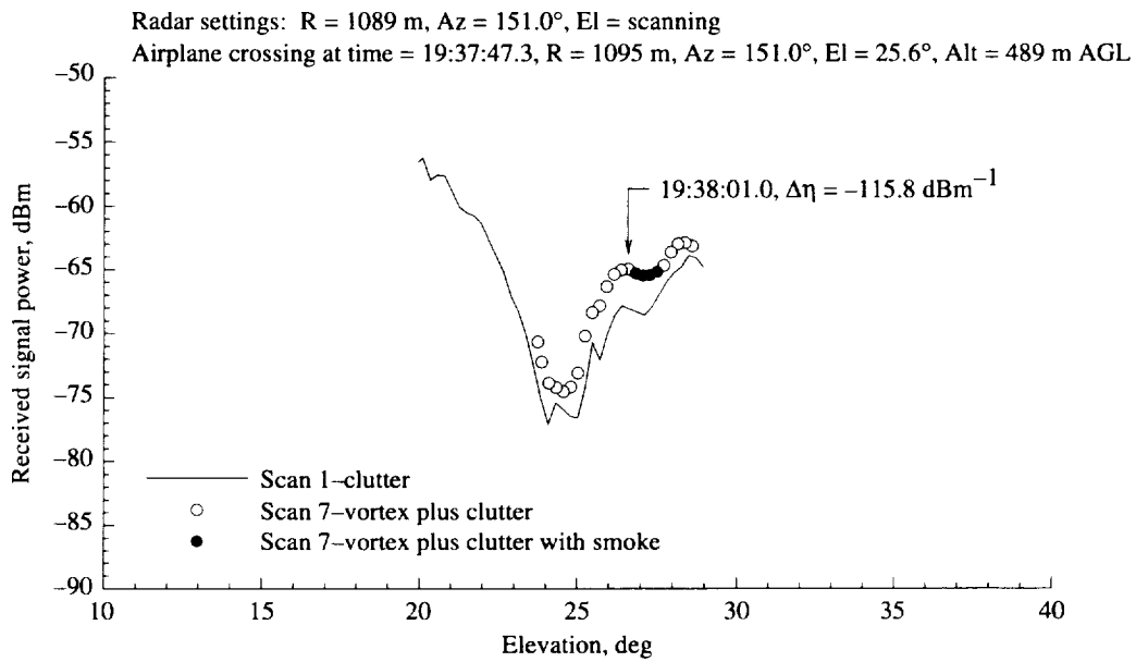
Figure A71. Total signal level vs. antenna elevation angle compared with clutter scan for pass 141, elevation scan 7, on 01-11-95.
