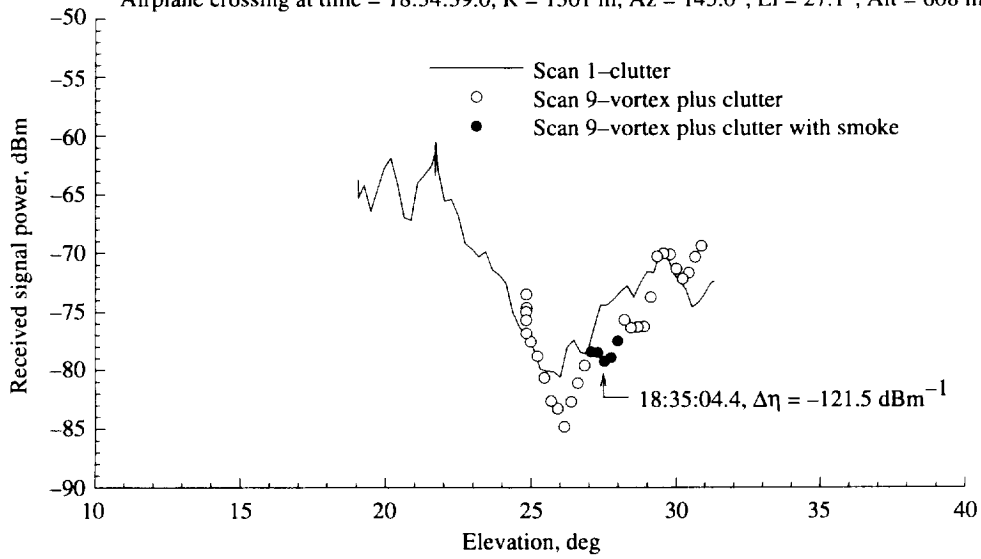
Figure A65. As for figure A63, except for elevation scan 9.
