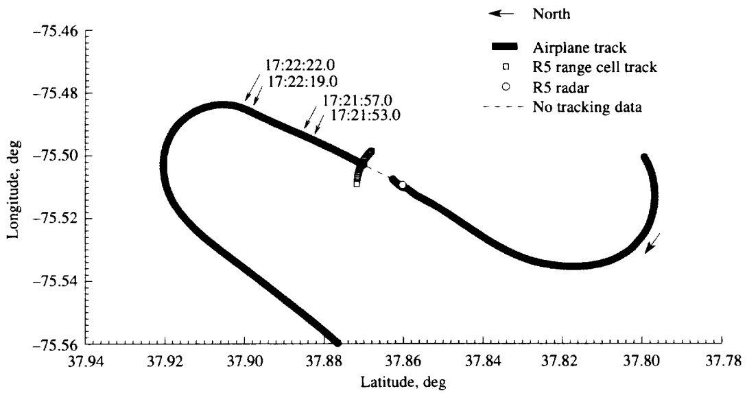
Figure A55. Pass 122 airplane and Radar 5 ground tracks; tail-on radar view of airplane wake.
