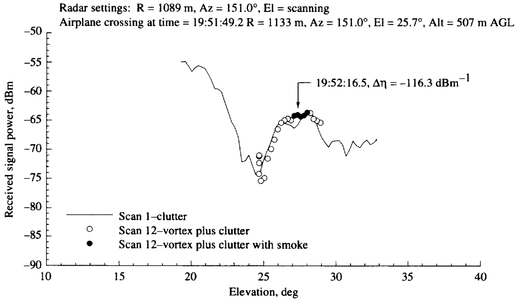
Figure A76. Total signal level vs. antenna elevation angle compared with clutter scan for pass 143, elevation scan 12, on 01-11-95.
