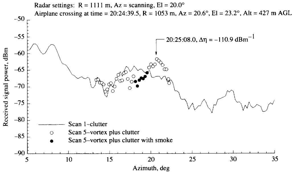
Figure A37. Total signal level vs. antenna azimuth angle compared with clutter scan for pass 107, azimuth scan 5, on 01-10-95.
