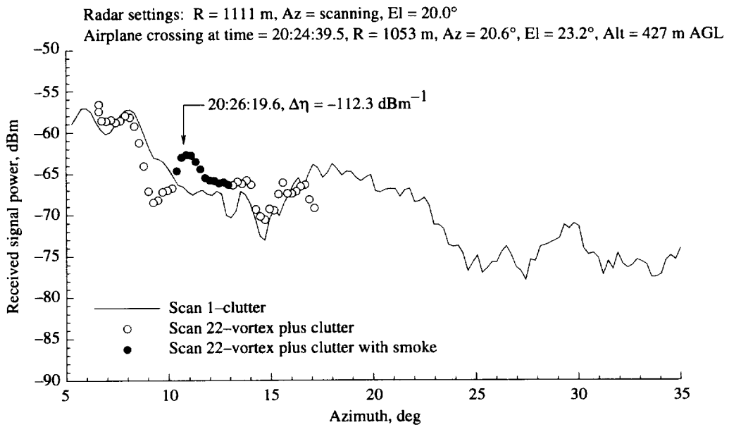
Figure A39. As for figure A37, except for azimuth scan 22.
