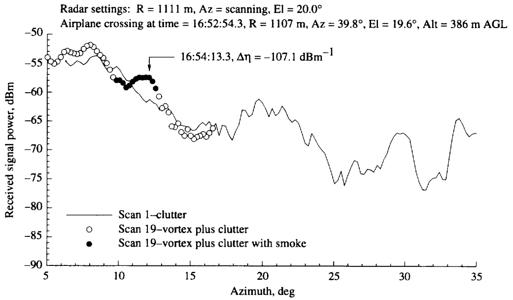
Figure A49. As for figure A47, except for azimuth scan 19.
