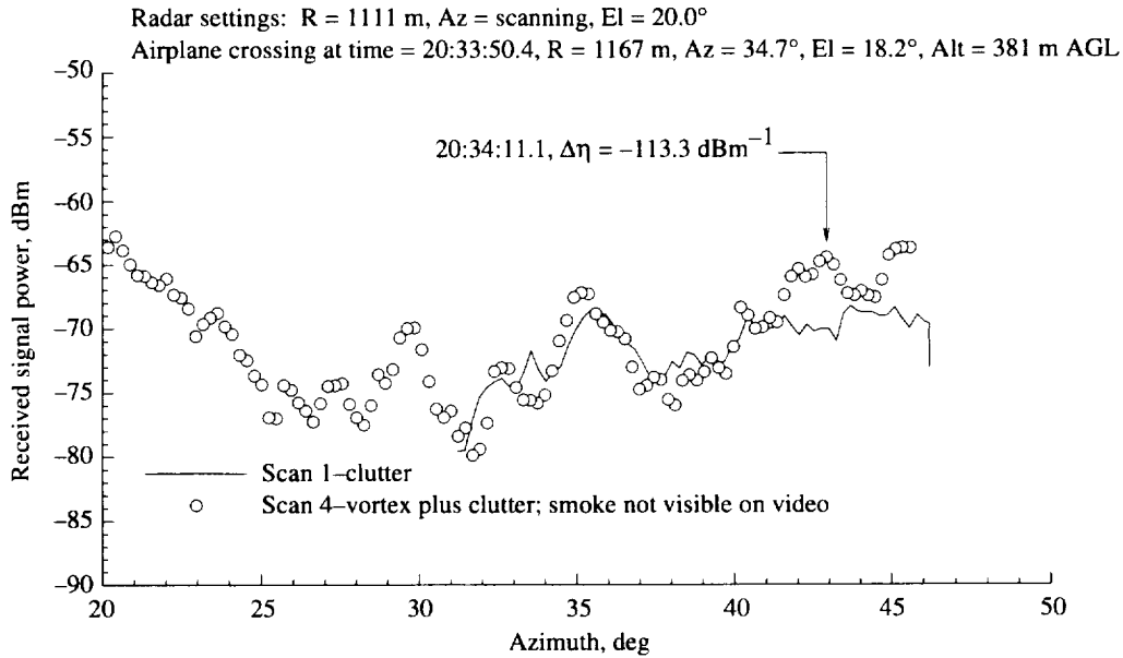
Figure A44. Total signal level vs. antenna azimuth angle compared with clutter scan for pass 109, azimuth scan 4, on 01-10-95.
