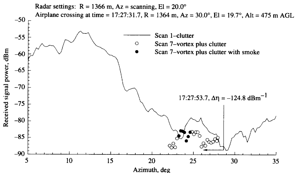
Figure A57. As for figure A56, except for azimuth scan 7.
