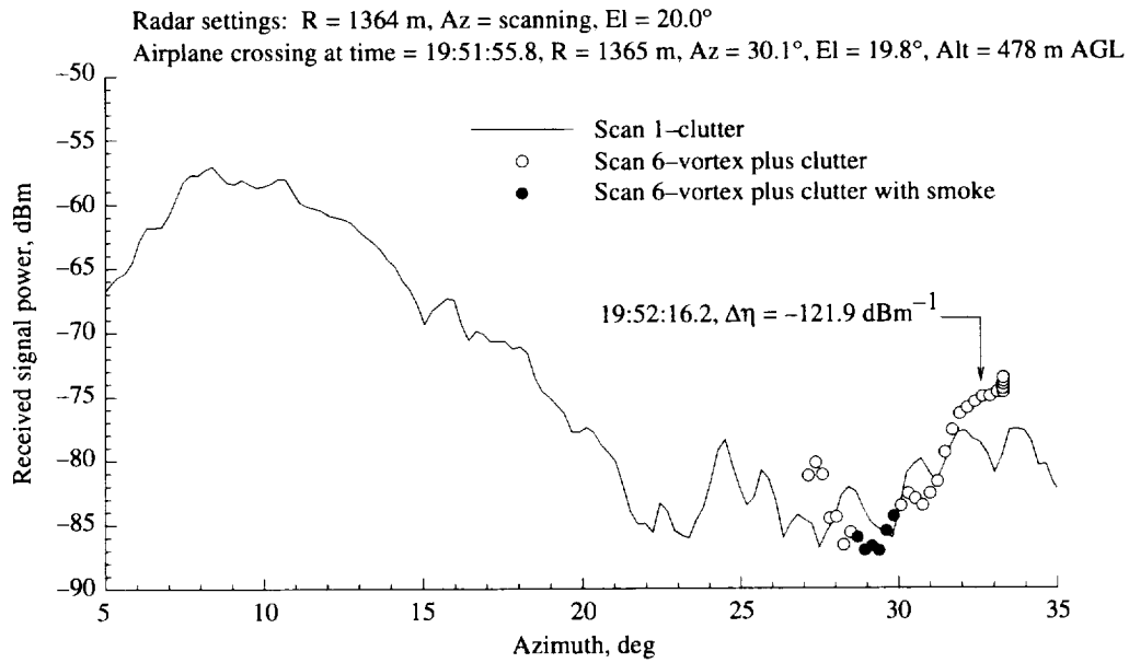
Figure A22. Total signal level vs. antenna azimuth angle compared with clutter scan for pass 100, azimuth scan 6, on 01-10-95.
