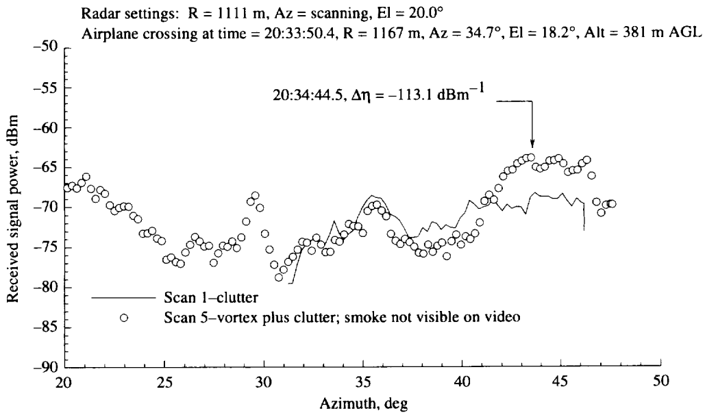
Figure A45. As for figure A44, except for azimuth scan 5.
