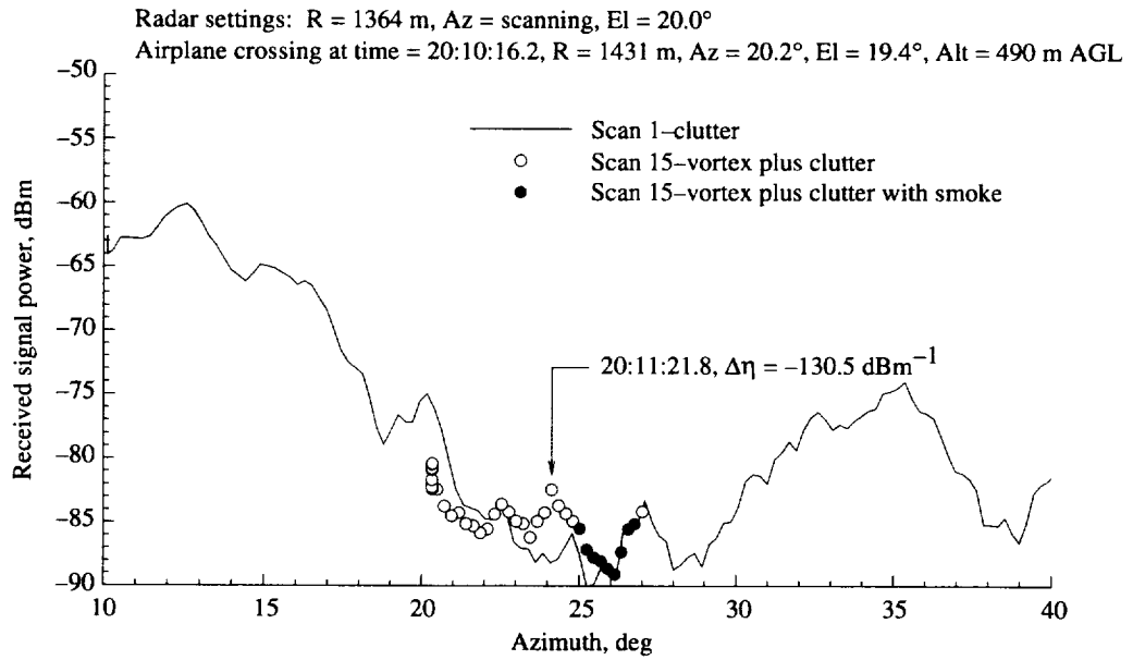
Figure A31. As for figure A29, except for azimuth scan 15.
