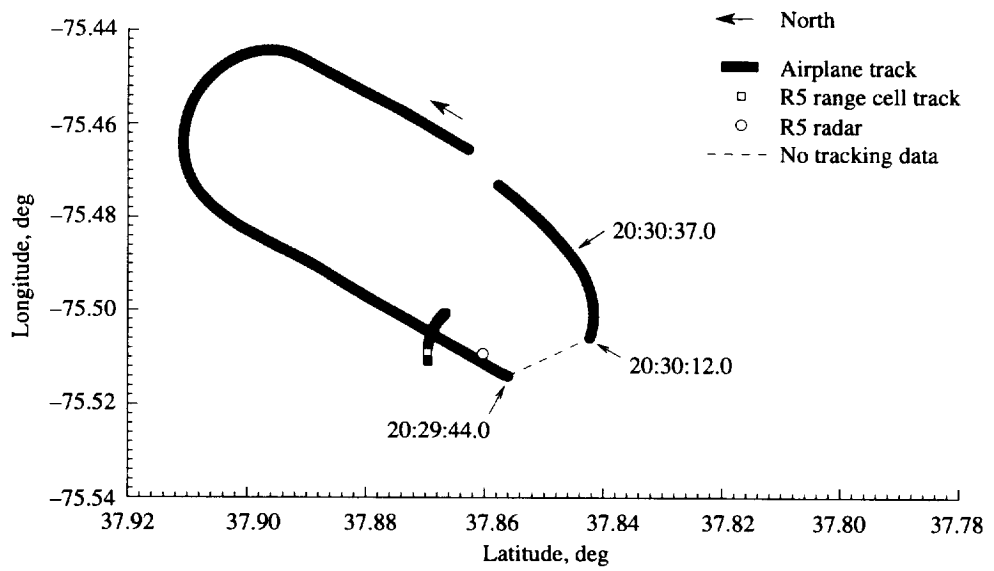
Figure A43. Pass 108 airplane and Radar 5 ground tracks; head-on radar view of airplane wake.
