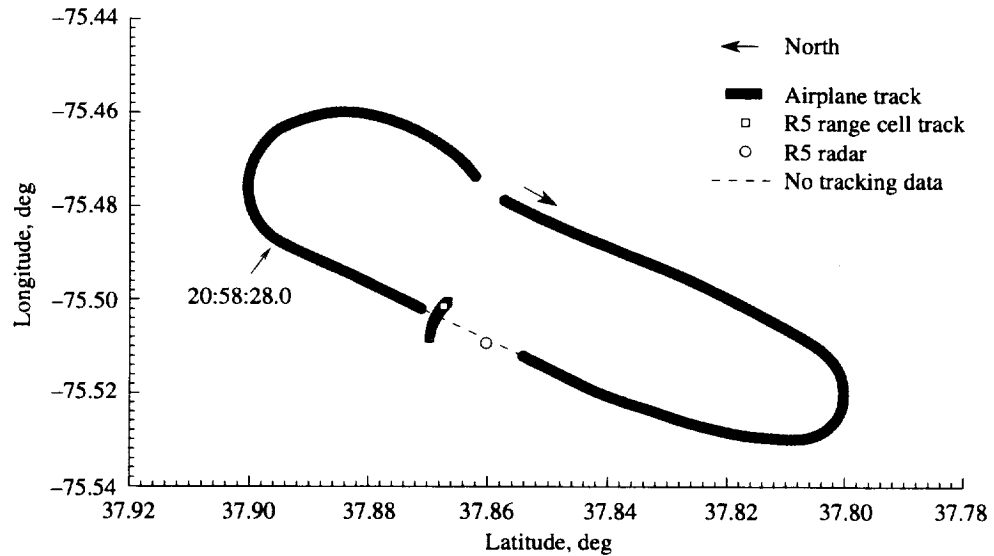
Figure A17. Pass 64 airplane and Radar 5 ground tracks; tail-on radar view of airplane wake.
