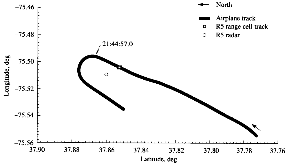
Figure A6. Pass 21 airplane and Radar 5 ground tracks; lateral radar view of airplane wake.
