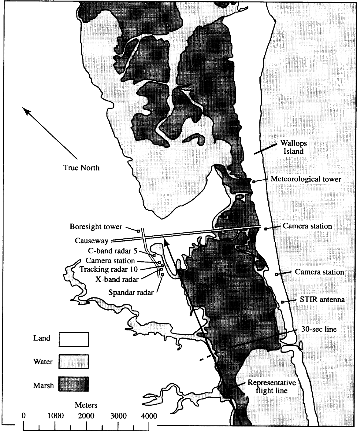
Figure 4. Map of experiment site at Wallops Flight Facility, Wallops Island, Virginia. C-band Radar 5 is situated in a row of radars which include tracking Radar 10 and the X-band radar that operated in conjunction with R5 during the experiment. This group of radars is about 6 miles south of the airfield and tracking Radar 18 (not pictured). During azimuth-scan passes, the C-130 flew directly over the radars; during elevation-scan passes, the aircraft flew past the radars as pictured.
