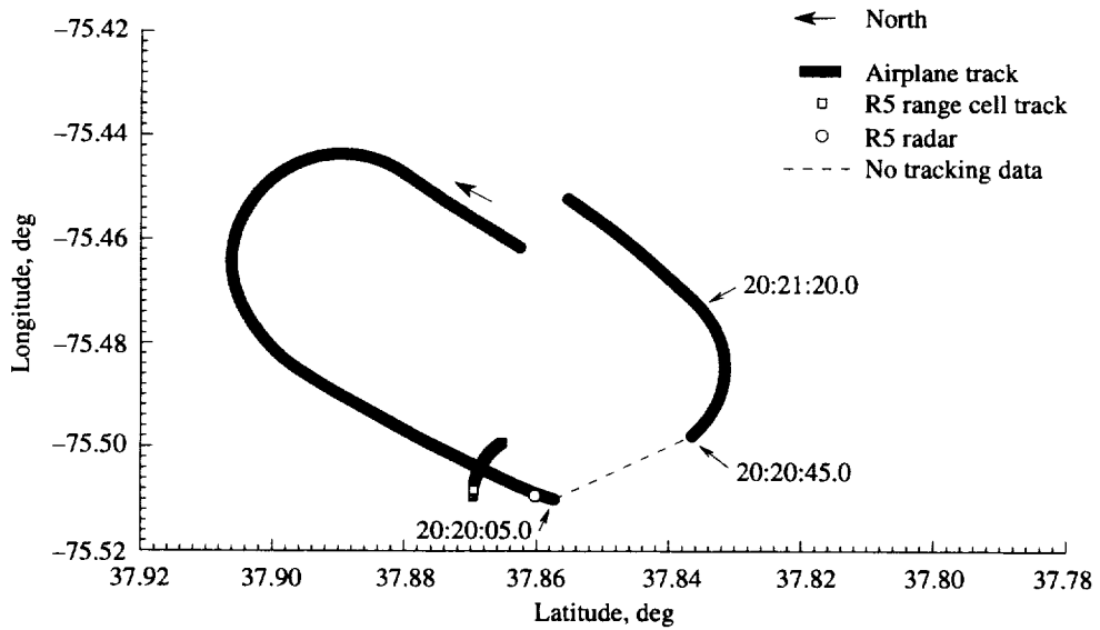
Figure A36. Pass 106 airplane and Radar 5 ground tracks; head-on radar view of airplane wake.
