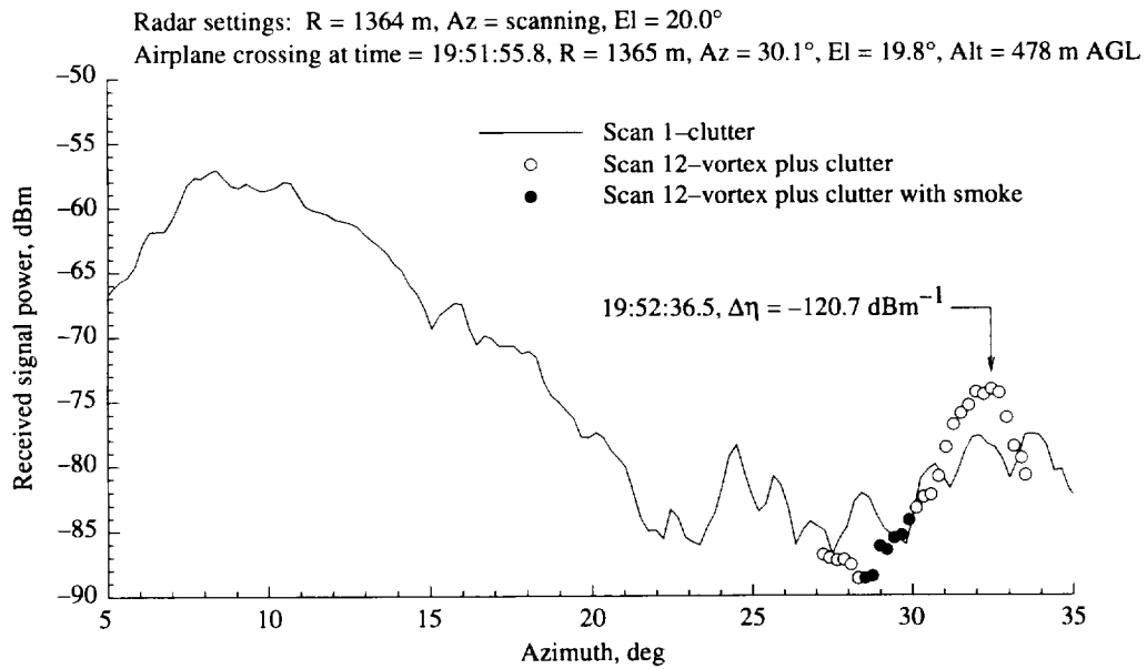
Figure A23. As for figure A22, except for azimuth scan 12.
