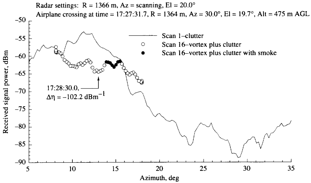
Figure A58. As for figure A56, except for azimuth scan 16.
