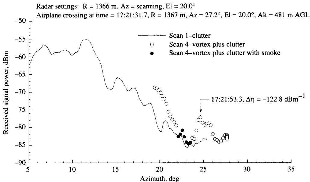
Figure A51. Total signal level vs. antenna azimuth angle compared with clutter scan for pass 122, azimuth scan 4, on 01-11-95.
