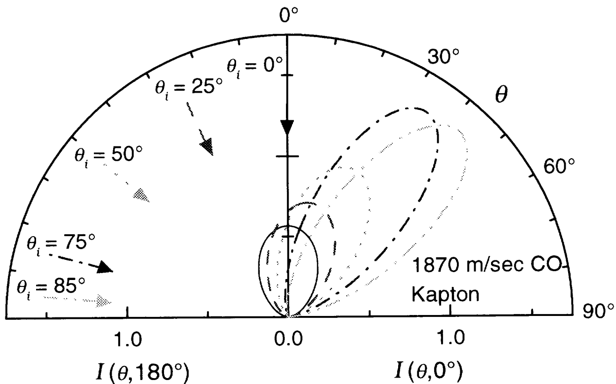
Figure 43: The angular distribution functions for 1870 m/s CO incident upon Kapton.
