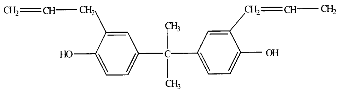
o,o'-Diallyl bisphenol A (DABA)
