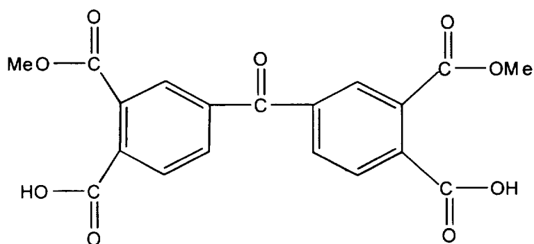
b.) Dimethyl ester of 3,3', 4,4'-benzophenone-tetracarboxylic acid (BTDE)
