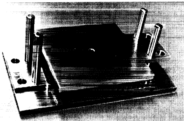
Figure 5: Photograph of a specimen in the bonding fixture between two load plates.
