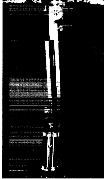
Figure 6: Photograph of specimen in test machine with plumb line showing load path through the corner of the specimen as stated in ASTM C 273.
