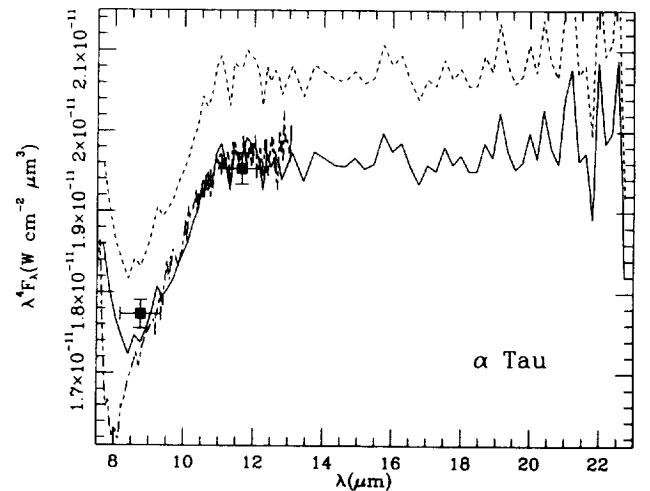
FIG. 2. A single-sided splice of the IRAS LRS spectrum of \alpha Tau with the higher resolution UKIRT CGS3 spectrum (long-dashed–short-dashed line), which was previously “locked” to photometry from UKIRT ([8.7], [11.7]). The short-dashed line is the original LRS fragment; the solid line is the LRS scaled by 0.95. Note the close accord of the shapes of the rescaled LRS spectrum and the ground-based CGS3 spectrum. Deacon’s (1991) photometry is included (along with the \pm HWHMs of the passbands).
