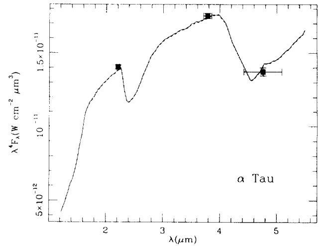
FIG. 1. Strecker et al. (1979) 1.2–5.5 \mu\text{m} KAO fragment for \alpha Tau located with respect to photometry (Kn, Ln, M). The \pm HWHMs of the relevant passbands are plotted. The short dashed line (barely distinguishable from the solid) is the SEW fragment; the solid line is the result of scaling it by 1.003 to fit this photometry.
