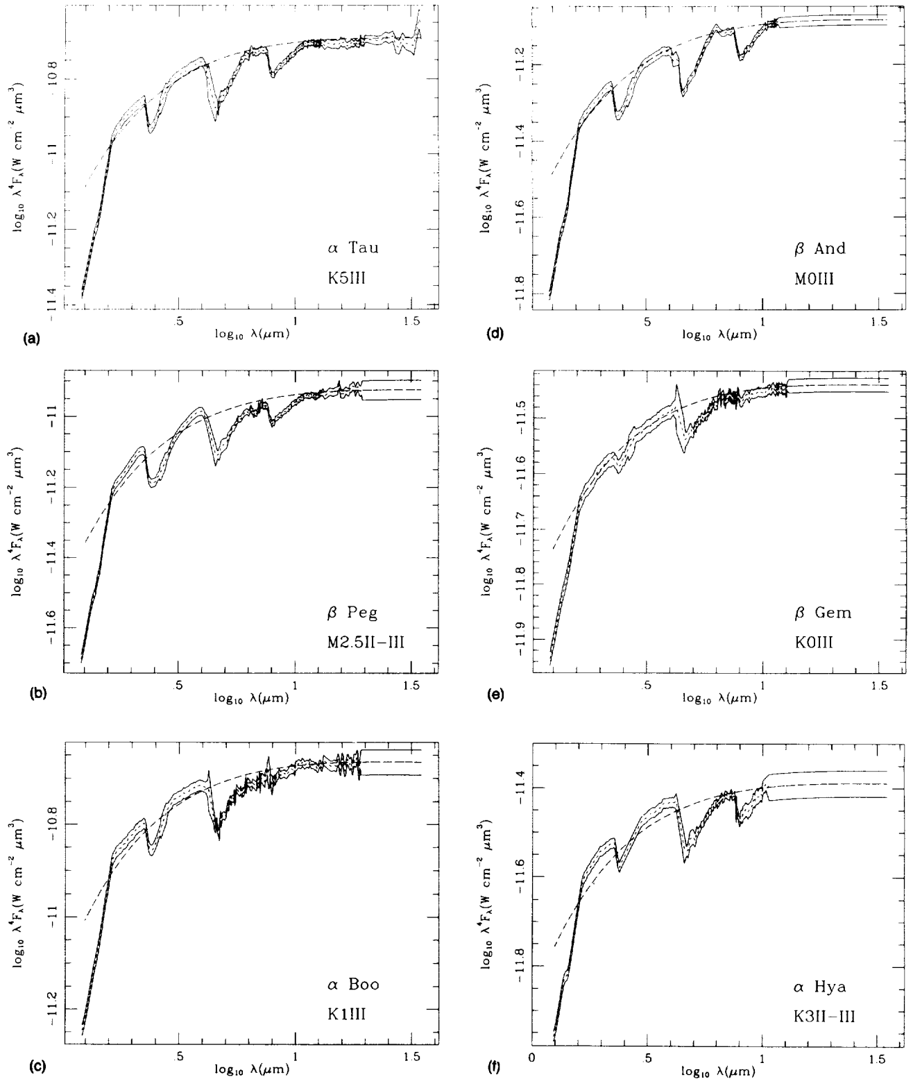
FIG. 4. All six cool stellar composites in the form of logarithmic plots of absolute \lambda^4 F_\lambda against \lambda . In each spectrum, the \pm 1\sigma error bars are indicated by the pair of solid lines, with the mean spectrum represented by the short-dashed line. The long-dashed line is the best-fitting Engelke approximation. (a) \alpha Tau; (b) \beta Peg; (c) \alpha Boo; (d) \beta And; (e) \beta Gem; and (f) \alpha Hya.
