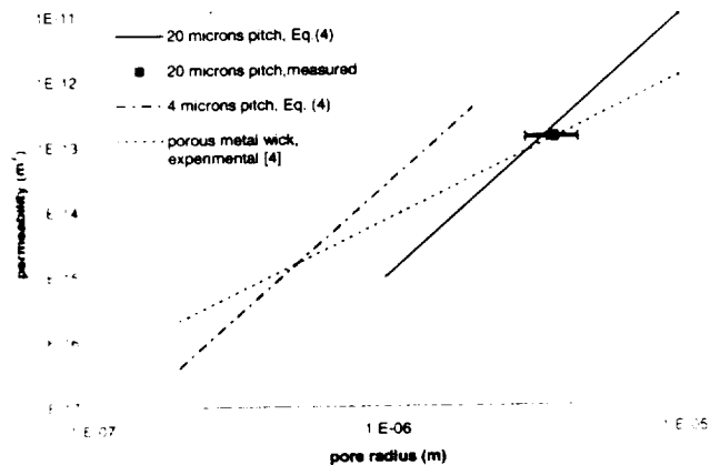
Figure 8. Permeability vs. pore radius for two different pore initiation patterns (masks), as well as conventional porous metal wicks. The theoretical and test results match well.
