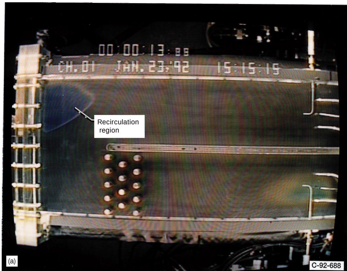
Figure 11.—Surface color-temperature patterns ( Re_{\text{entrance}} = 45\,000 ). (a) Low heat input, main section. (b) Medium heat input. (c) High heat input.
