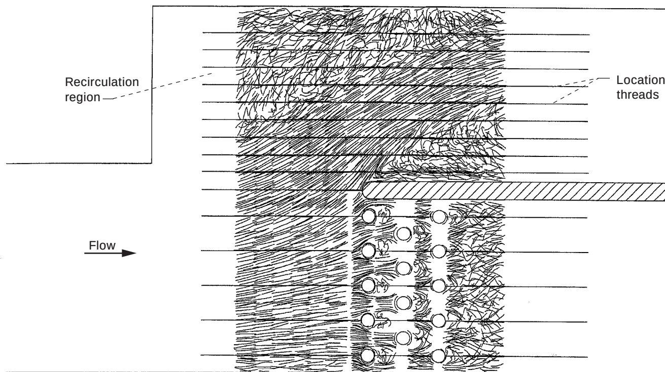
Figure 16.—Composite of digitized video data showing streamlines (300 video frames combined ( Re_{entrance} = 45\,000 )).
