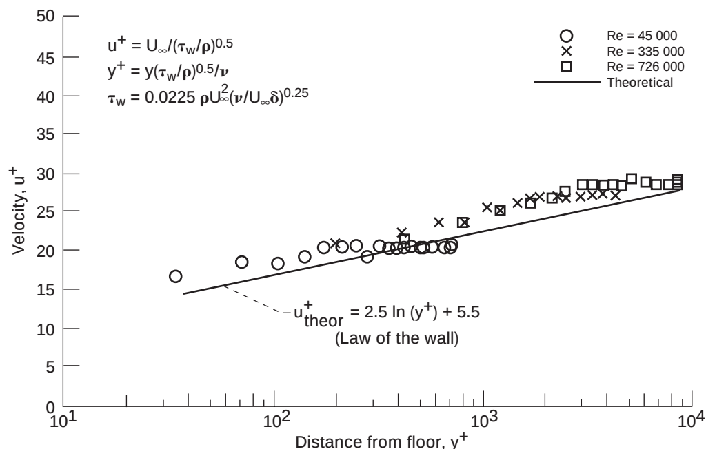
Figure 10.—Dimensionless boundary-layer profile.
