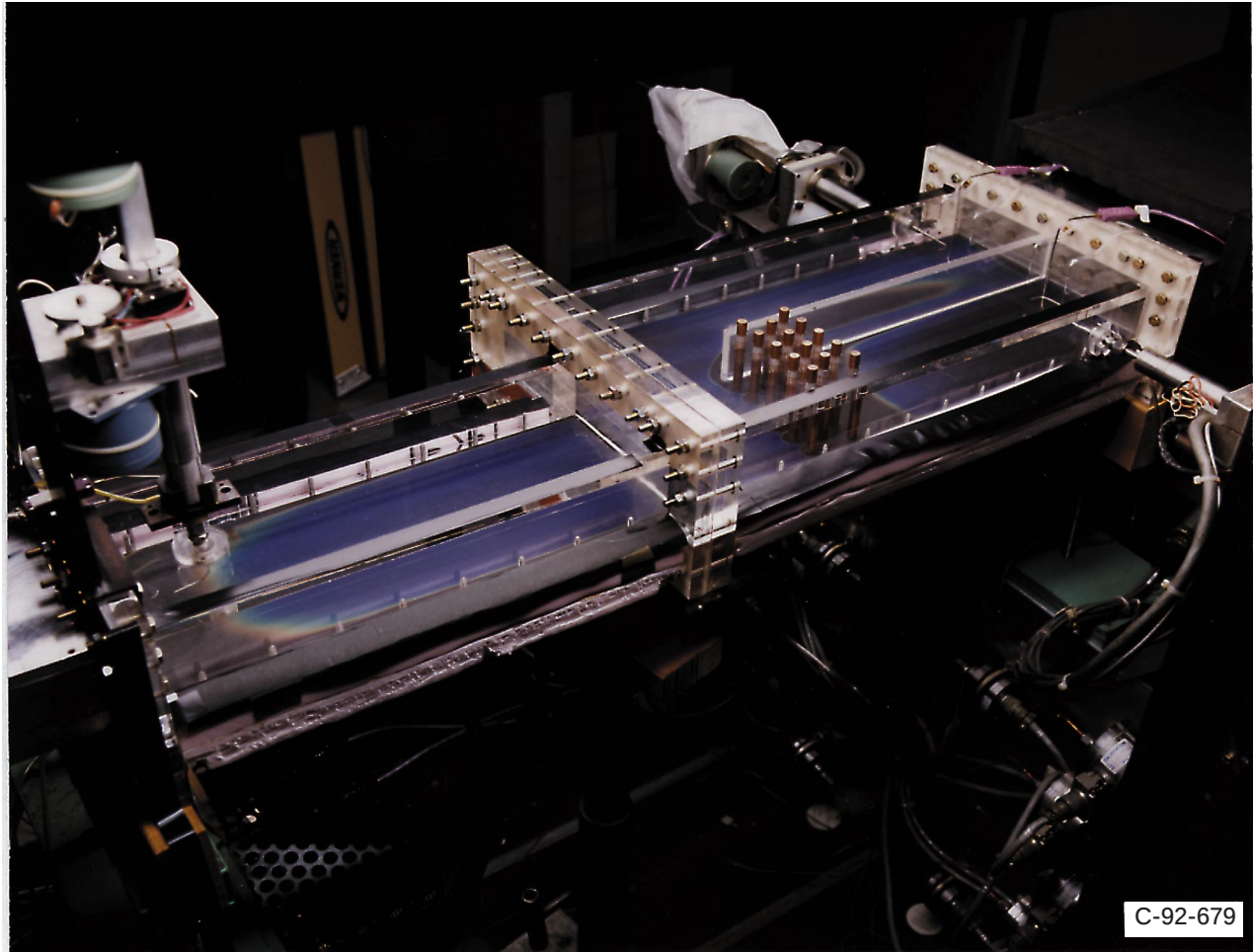
Figure 7.—Test section under flow conditions ( Re_{entrance} = 45\,000 ).
