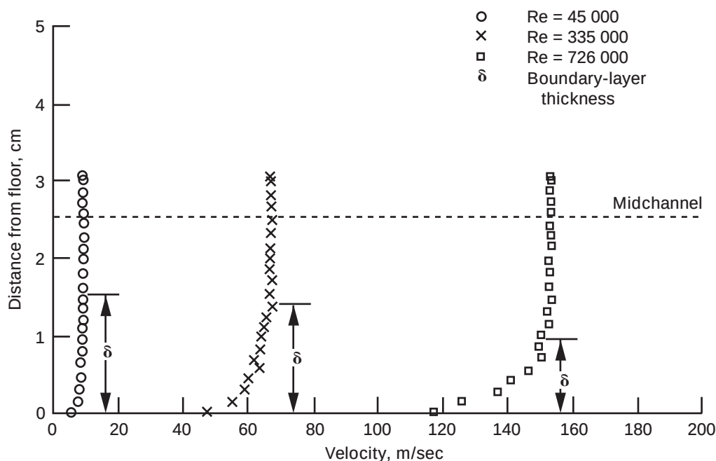
Figure 9.—Entrance velocity profiles.
