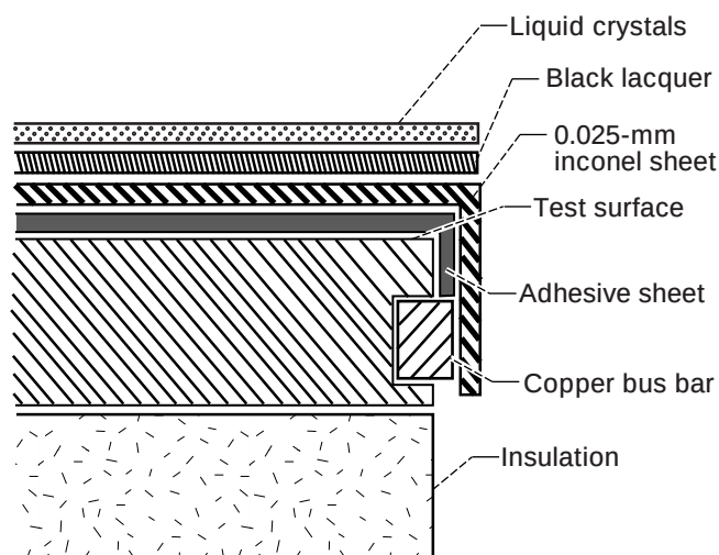
Figure 4.—Cross section of test surface.
