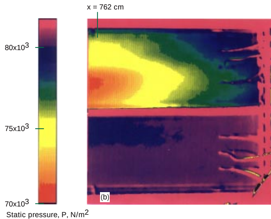
Figure 20.—Experimental floor static pressure maps from pressure sensitive paint technique ( Re_{\text{entrance}} = 726\,000 ). (a) Flow split region. (b) Downstream end of test section.
