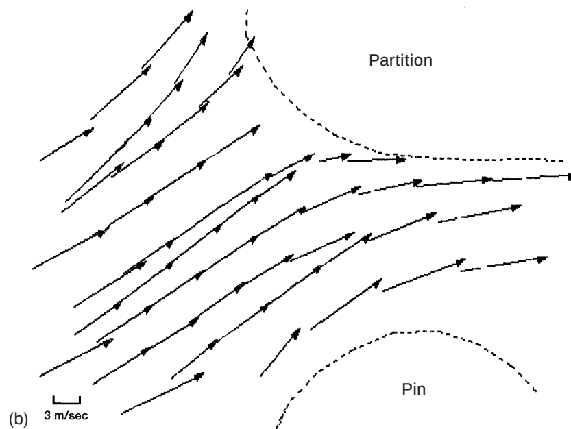
Figure 15.—Particle trajectories ( Re_{entrance} = 45\,000 ). (a) Video picture. (b) Velocity vector diagram.
