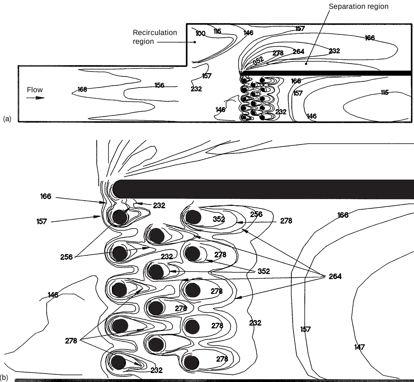
Figure 13.—Experimental heat transfer coefficients ( Re_{entrance} = 335\,000 ). (Coefficients given in W/m^2-K .) (a) Entire test surface. (b) Closeup of area.
