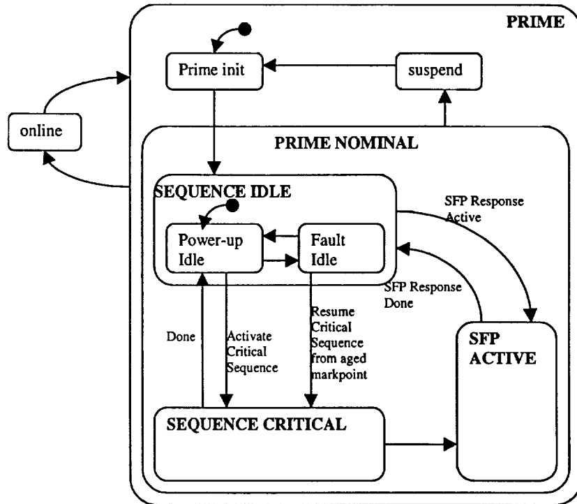
Figure 1: A partial statechart for the DRS prime string
