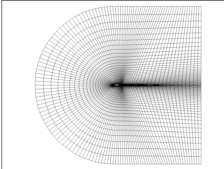
Figure 12: Entire Level 2 Computational Mesh of the Eppler 387 Airfoil
