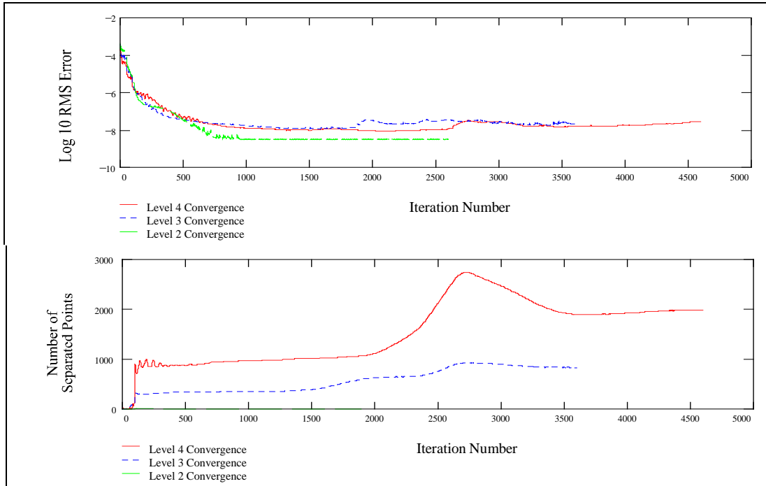
Figure 24: Comparison of the Convergence Histories, Re = 200,000 M = 0.2
