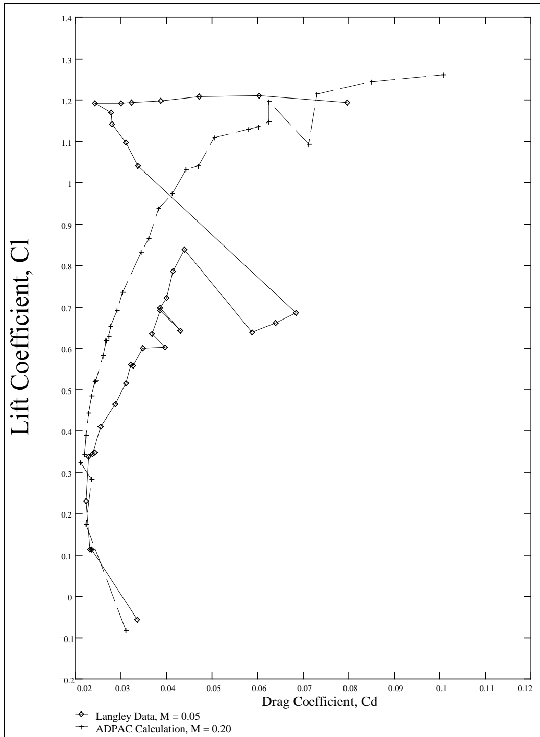
Figure 38: Comparison of Measured and Calculated Drag Coefficient versus Lift Coefficient for Re = 60,000
