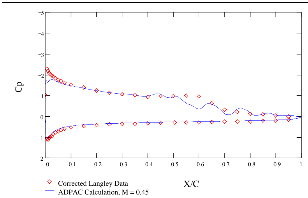
Figure 56: Pressure Coefficient vs. Non-dimensional Chordwise Position, Re = 60,000 \alpha = 7.00^\circ
