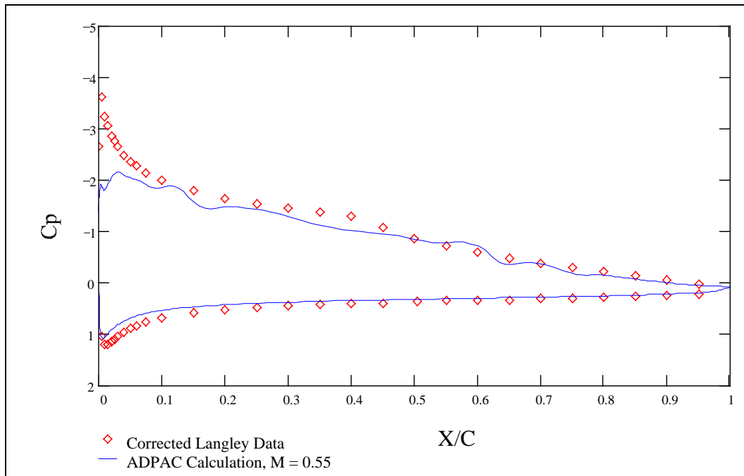
Figure 69: Pressure Coefficient vs. Non-dimensional Chordwise Position, Re = 100,000 \alpha = 8.00^\circ
