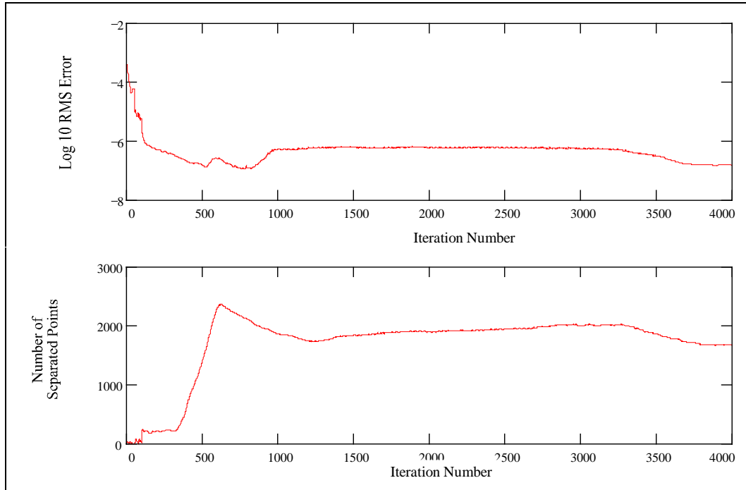
Figure 71: ADPAC Convergence History, Re = 100,000 M = 0.55 \alpha = 4.00^\circ
