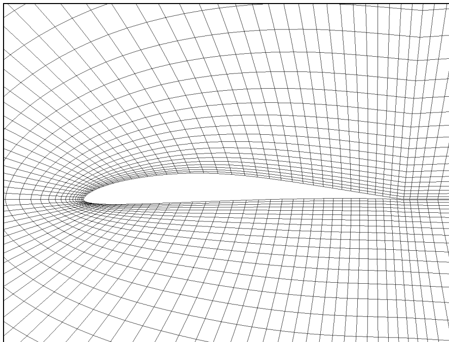
Figure 15: Portion of Level 2 Mesh Close to the Airfoil Surface
