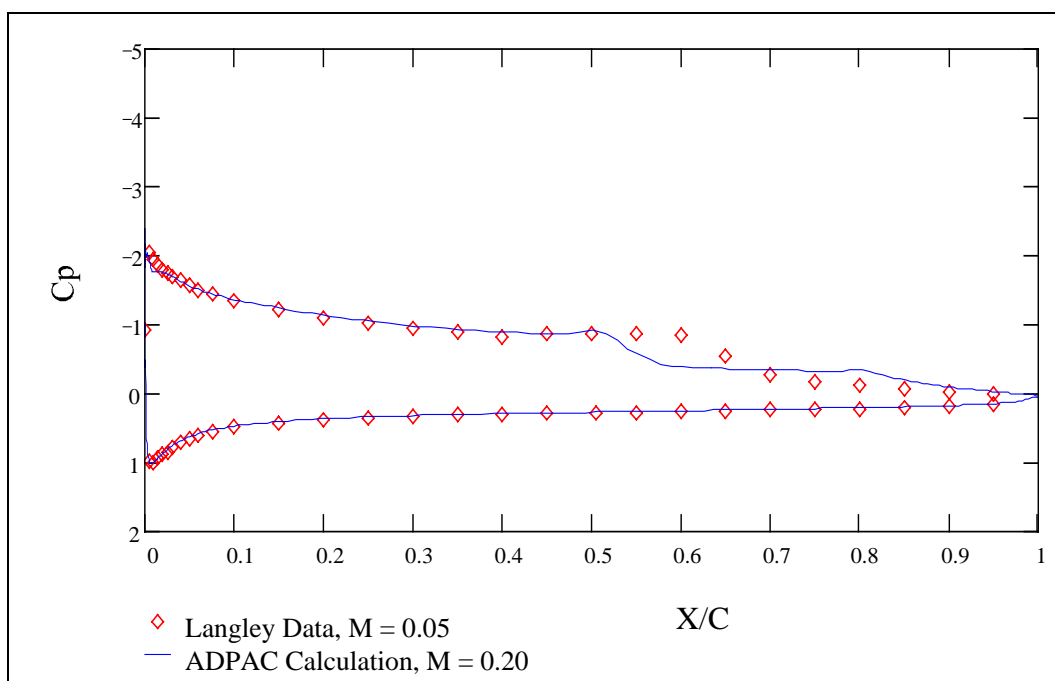
Figure 29: Pressure Coefficient vs. Non-dimensional Chordwise Position, Re = 60,000 \alpha = 7.00^\circ
