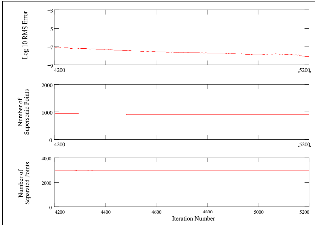
Figure 95: ADPAC Convergence History, Re = 60,000 M = 0.75 \alpha = 4.00^\circ
