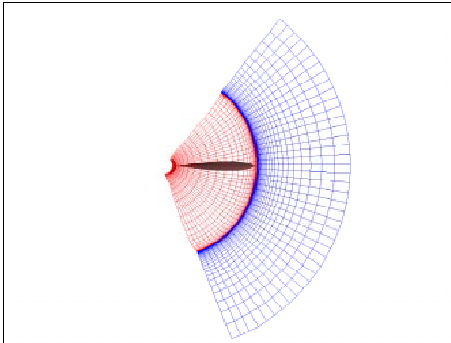
Figure 123: View of Computational Mesh Upstream and Above the Blade Tip— Forward Looking Aft
