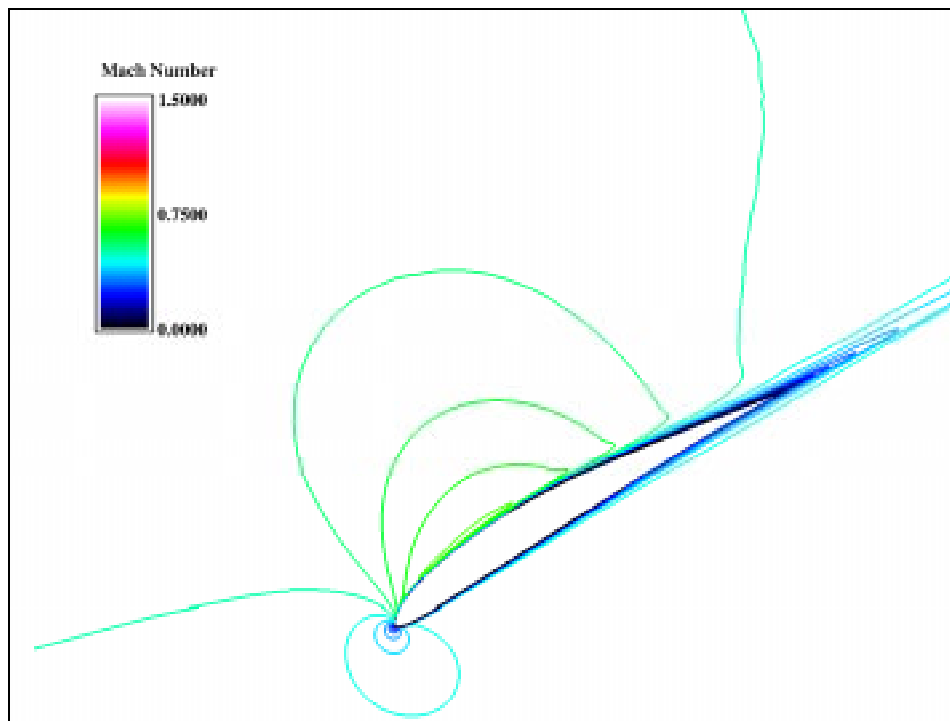
Figure 127: Mach Number Contours for r/R_{tip} = 0.0406
