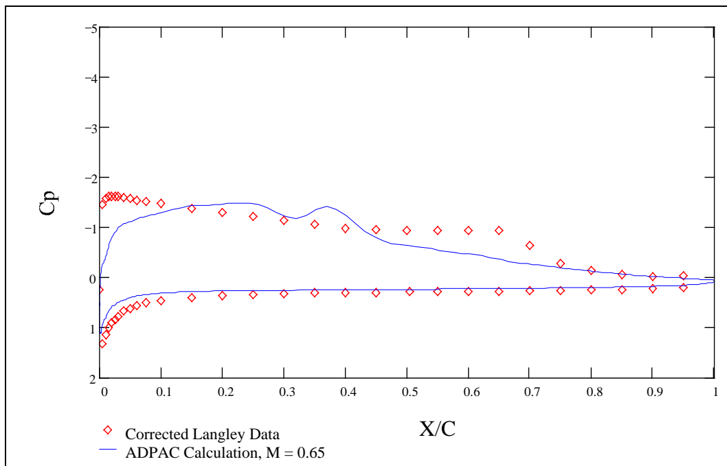
Figure 78: Pressure Coefficient vs. Non-dimensional Chordwise Position, Re = 100,000 \alpha = 5.01^\circ
