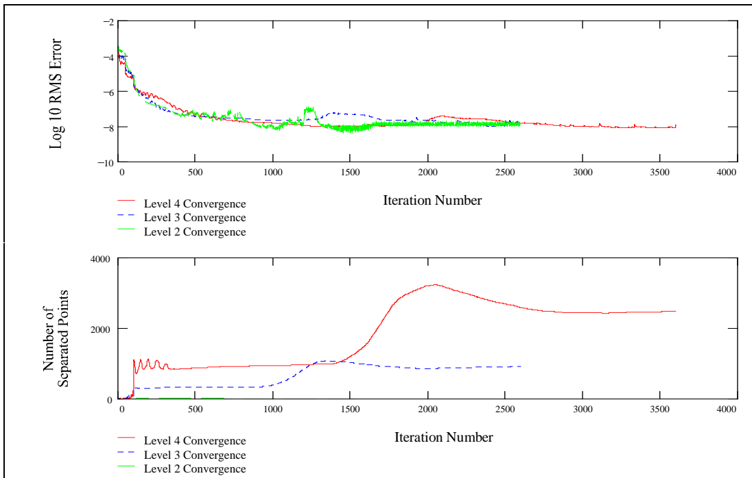
Figure 23: Comparison of the Convergence Histories, Re = 100,000 M = 0.2
