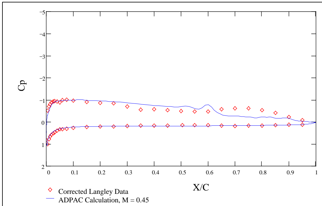
Figure 53: Pressure Coefficient vs. Non-dimensional Chordwise Position, Re = 60,000 \alpha = 4.00^\circ
