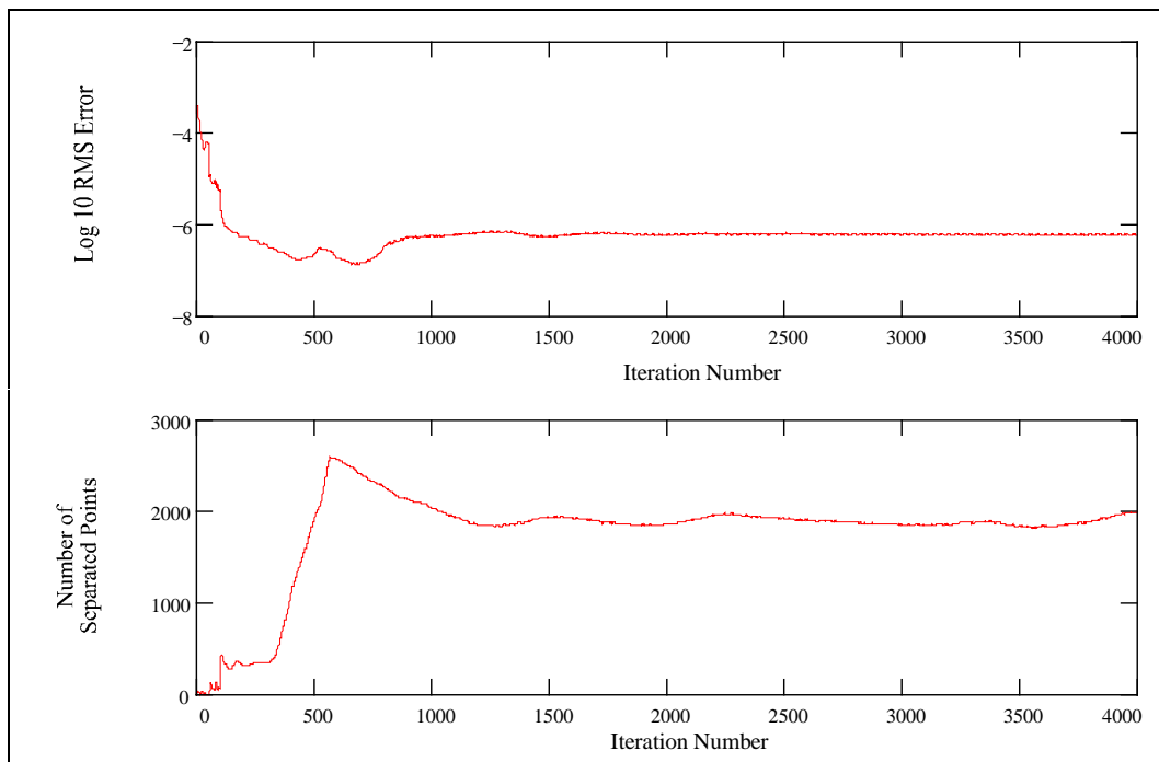
Figure 72: ADPAC Convergence History, Re = 100,000 M = 0.55 \alpha = 5.01^\circ
