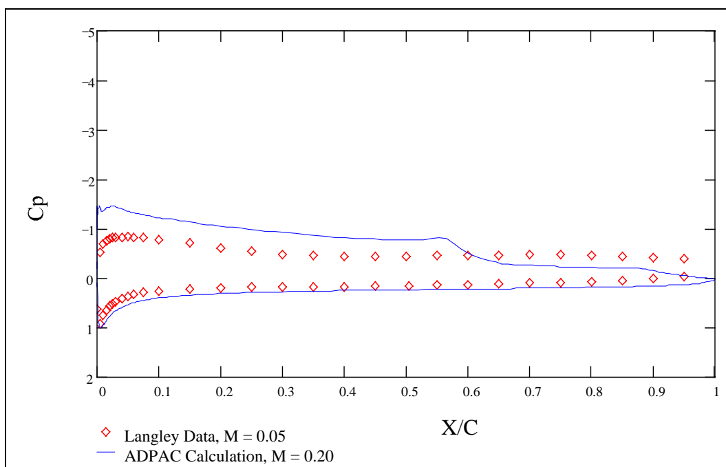
Figure 28: Pressure Coefficient vs. Non-dimensional Chordwise Position, Re = 60,000 \alpha = 6.01^\circ
