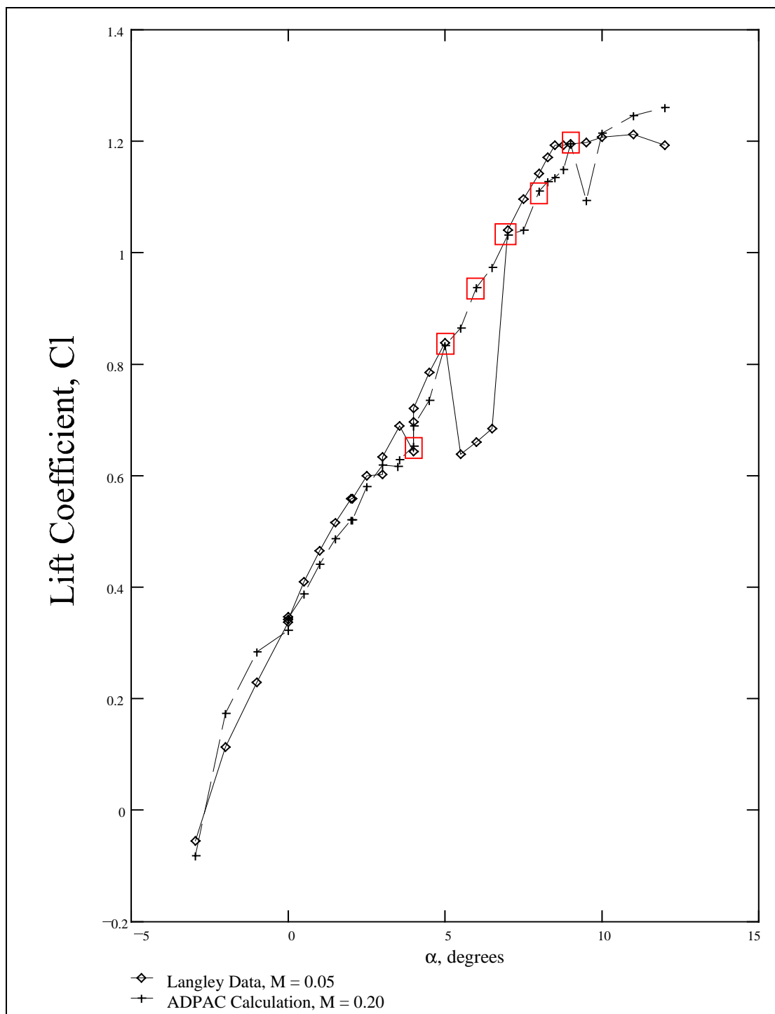
Figure 25: Comparison of Measured and Calculated Lift Coefficient versus Angle of Attack for Re = 60,000
