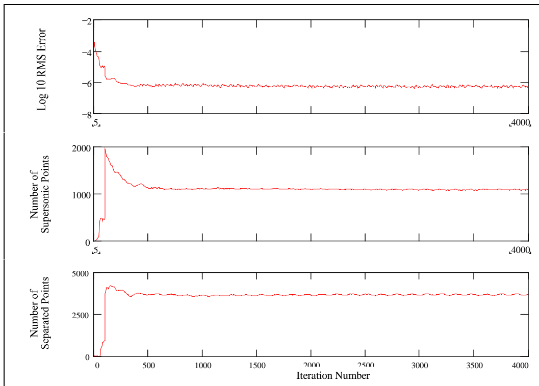
Figure 98: ADPAC Convergence History, Re = 60,000 M = 0.75 \alpha = 7.00^\circ
