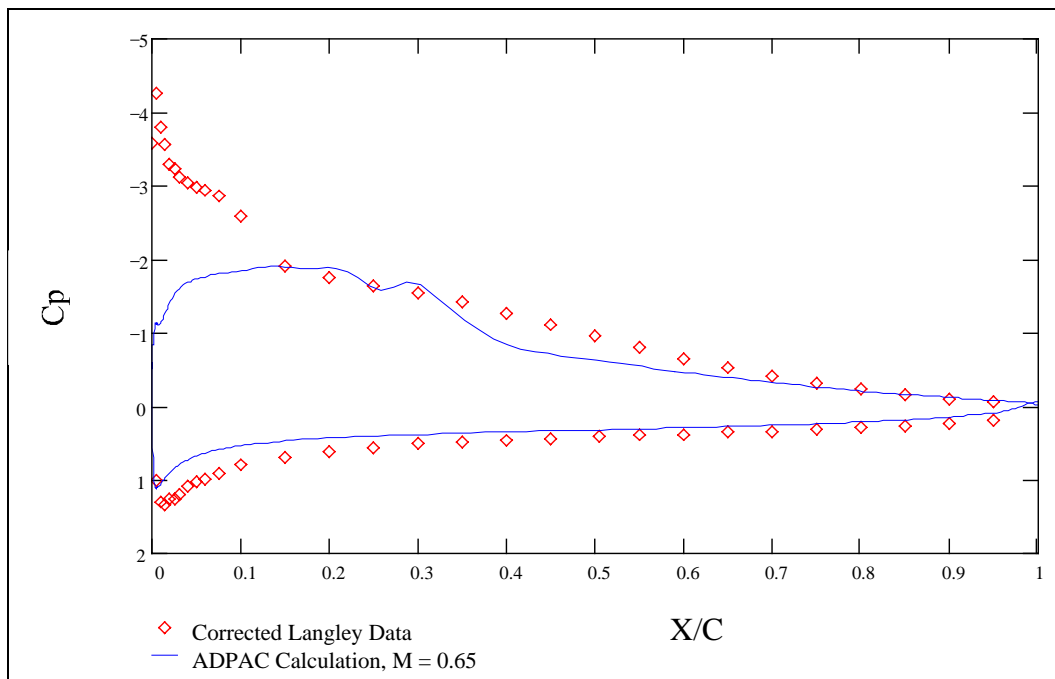
Figure 82: Pressure Coefficient vs. Non-dimensional Chordwise Position, Re = 100,000 \alpha = 9.00^\circ
