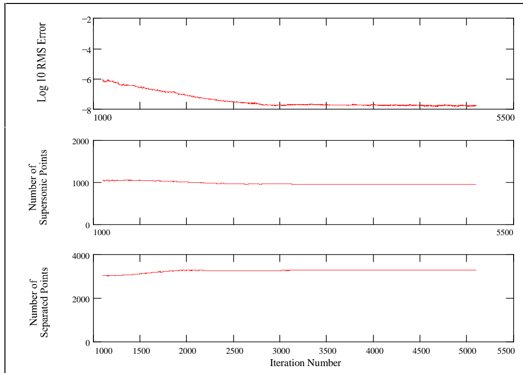
Figure 96: ADPAC Convergence History, Re = 60,000 M = 0.75 \alpha = 4.99^\circ
