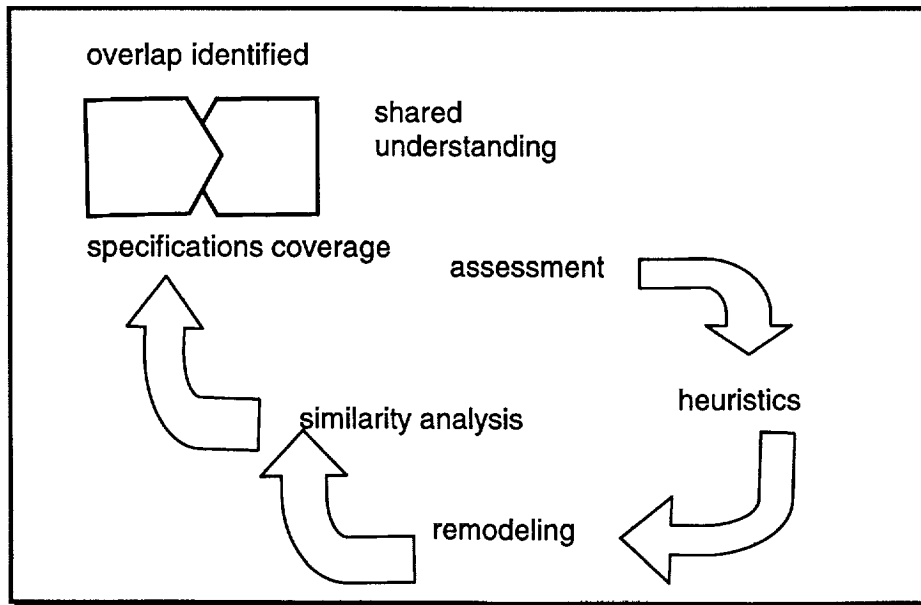
Figure 4. Reconciliation Approach to Interference Management.
