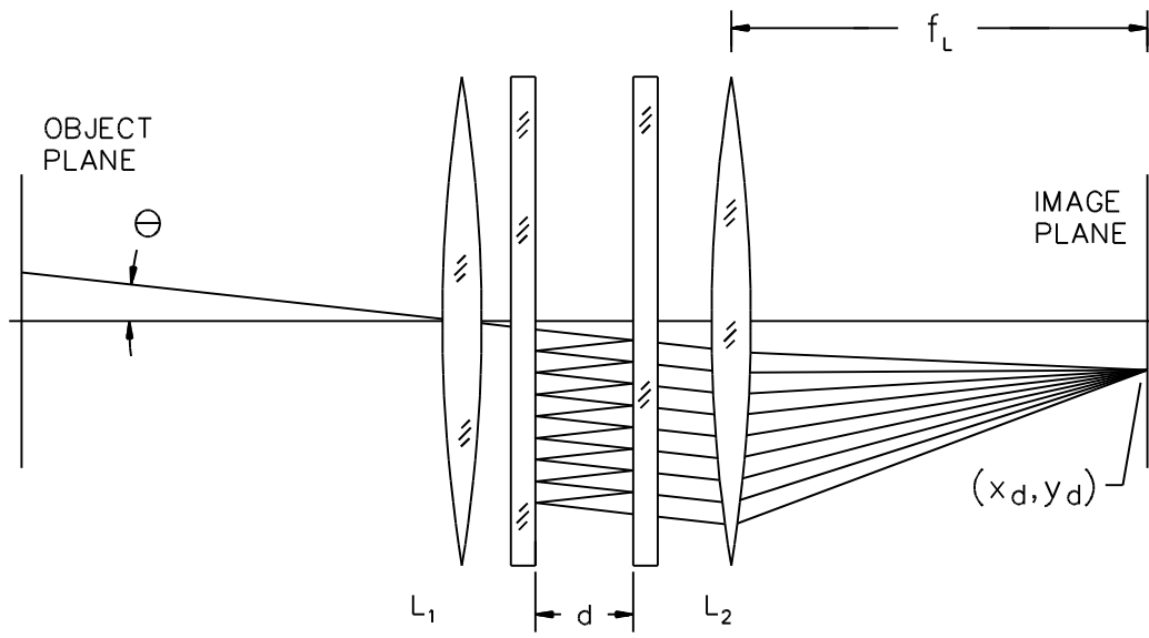
Fig. 5 - Fabry-Perot interferometer
