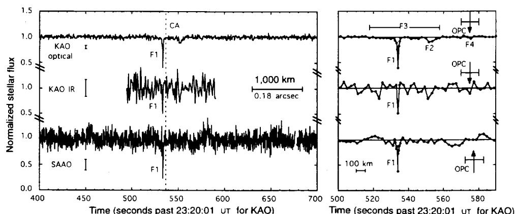
FIG. 1 Chiron occultation light curves. Portions of the stellar flux (normalized to 1.0 for the unocculted star) from Ch08 have been plotted versus ut for an interval that includes Chiron's closest approach to Ch08 (shown by the dotted line labelled "CA"). The left-hand panel is at full resolution. The right-hand panel includes only data near closest approach; to enhance the signal-to-noise ratio, data outside the sharp drop (feature 1, F1) have been averaged to 2.0 s. The segment of the light curves comprising F1 have been left at full resolution for the KAO data, whereas the SAAO data have been averaged to 0.4 s (two integration times and two deadtimes). In the left-hand panel the error bars are \pm 1\sigma , and the 1,000-km spatial scale at Chiron (for the KAO shadow velocity of 18.32 \text{ km s}^{-1} ) is approximately the resolution of the Hubble Space Telescope. The orbit-plane crossing (OPC) time is indicated in the right-hand panel. A sharp drop and recovery (F1) is evident in all three light curves. As the paths of the KAO and SAAO were separated in Chiron's shadow plane by only 1.4 km at closest approach (107.8 km for the KAO and 106.4 km for SAAO), we have assumed that F1 was
