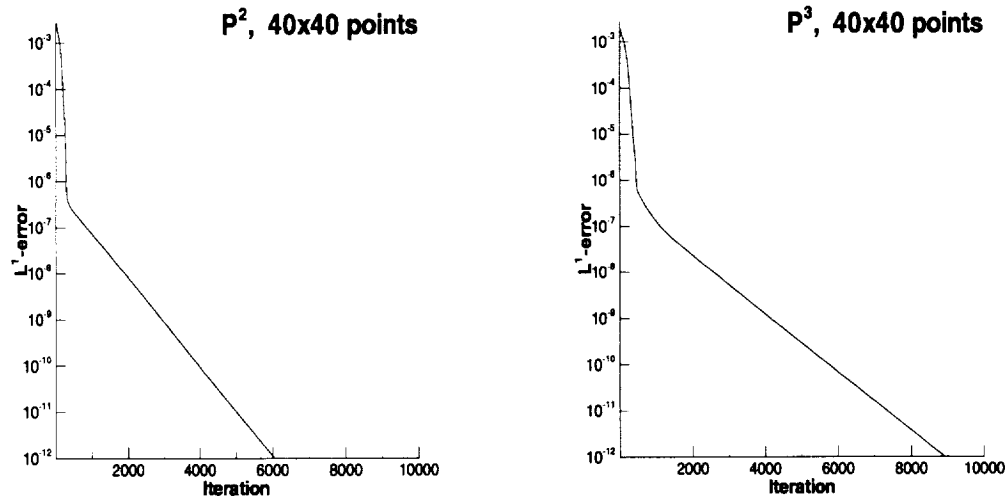
FIG. 4.21. Computer vision problem, history of iterations.
