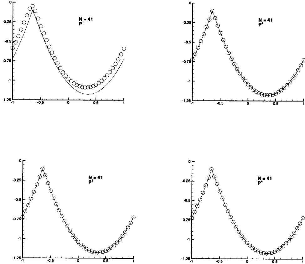
FIG. 4.1. One-dimensional Burgers' equation, t = 3.5/\pi^2 .
