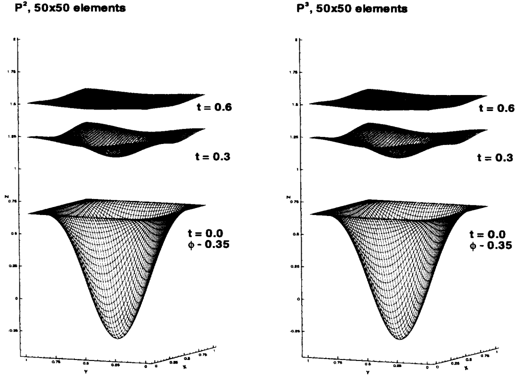
FIG. 4.11. Propagating surfaces, rectangular mesh, \varepsilon = 0.1 .
