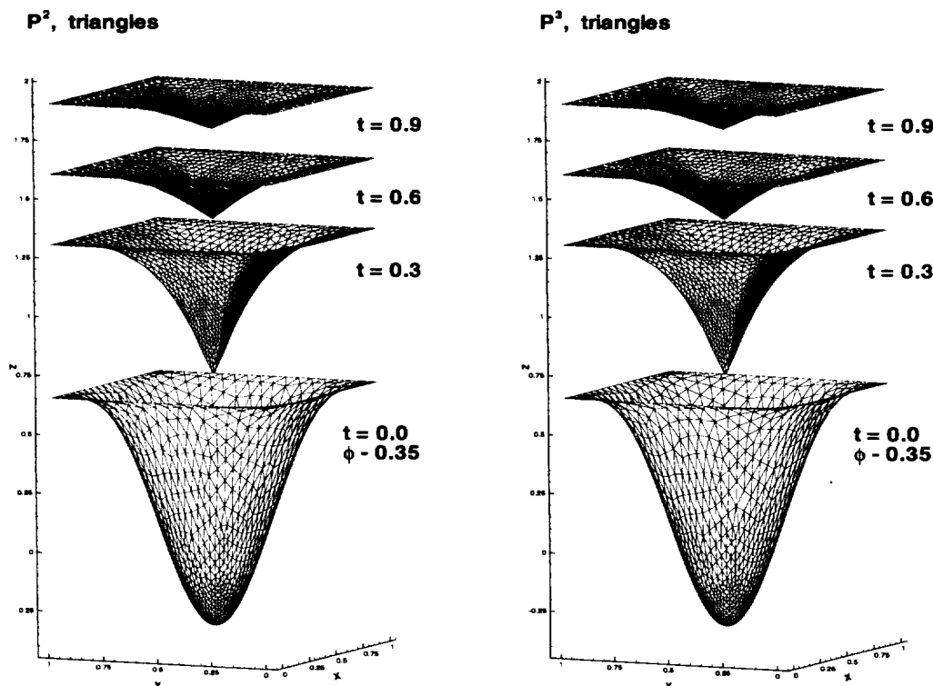
FIG. 4.13. Propagating surfaces, triangular mesh, \epsilon = 0 .
