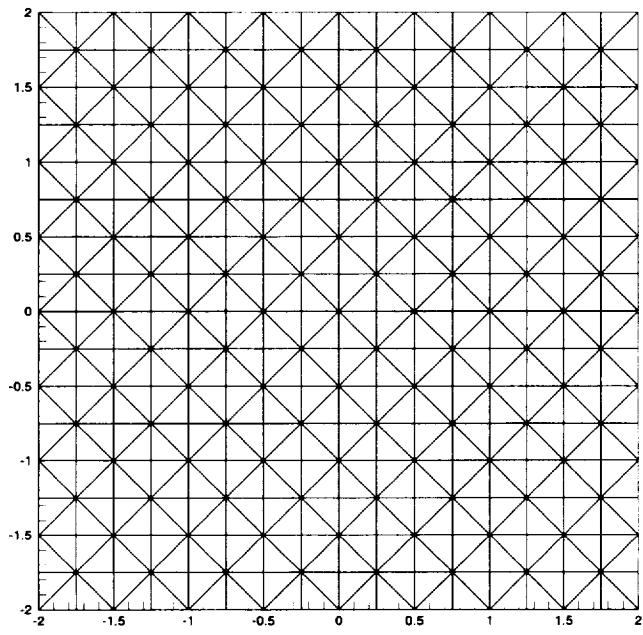
FIG. 4.6. Triangulation for two dimensional Burgers equation, h = \frac{1}{4} .
