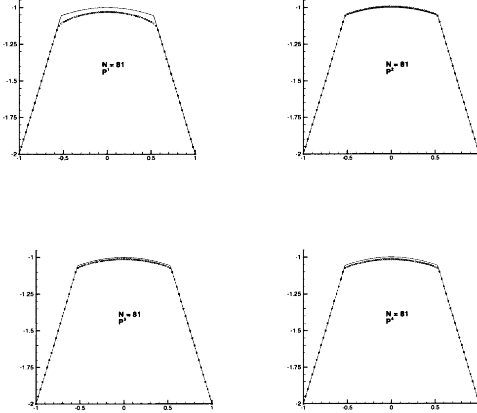
FIG. 4.3. One dimension Riemann problem, local Lax-Friedrichs flux, H(u) = \frac{1}{4}(u^2 - 1)(u^2 - 4) , t = 1 .
