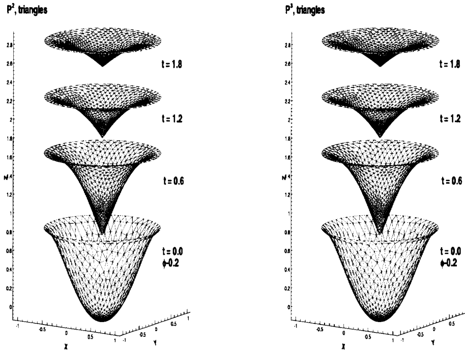
FIG. 4.16. Propagating surfaces on a disk, triangular mesh, \epsilon = 0 .
