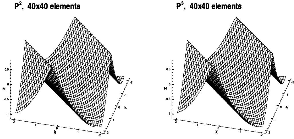
FIG. 4.5. Two dimension Burgers' equation, rectangular mesh, t=1.5/\pi^2 .
