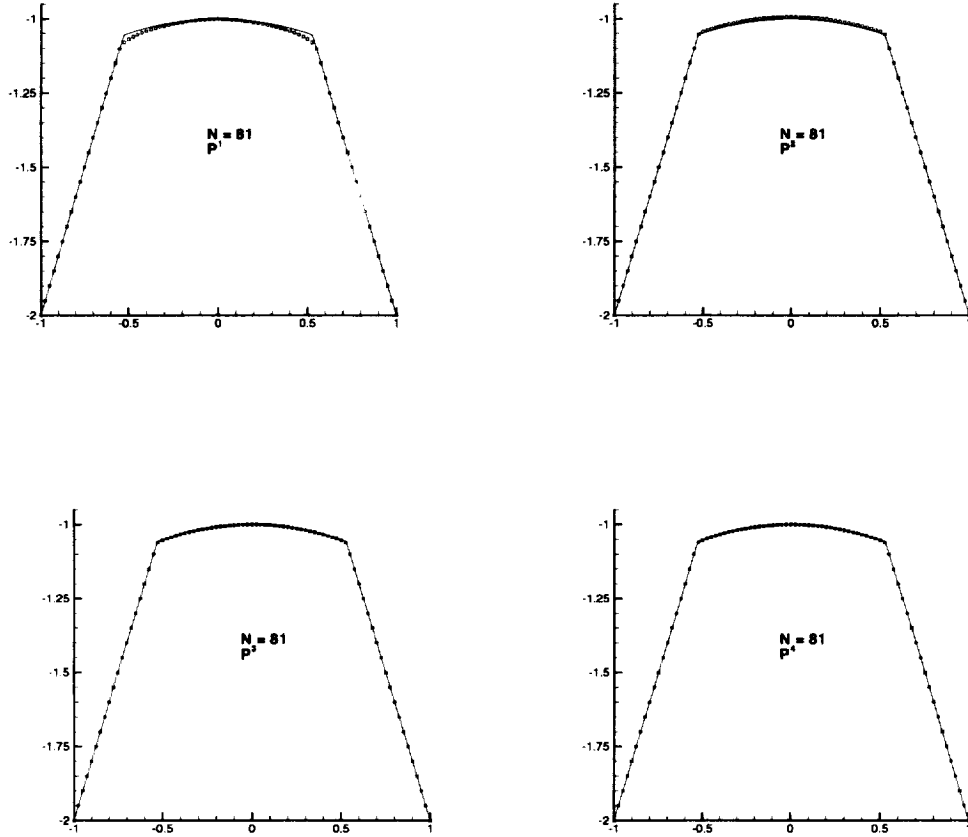
FIG. 4.4. One dimension Riemann problem, Godunov flux, H(u) = \frac{1}{4}(u^2 - 1)(u^2 - 4) , t = 1 .
