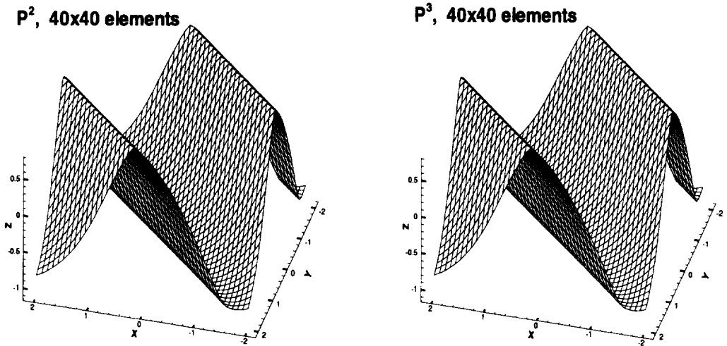
FIG. 4.7. Two dimension Burgers' equation, triangular mesh, t=1.5/\pi^2 .
