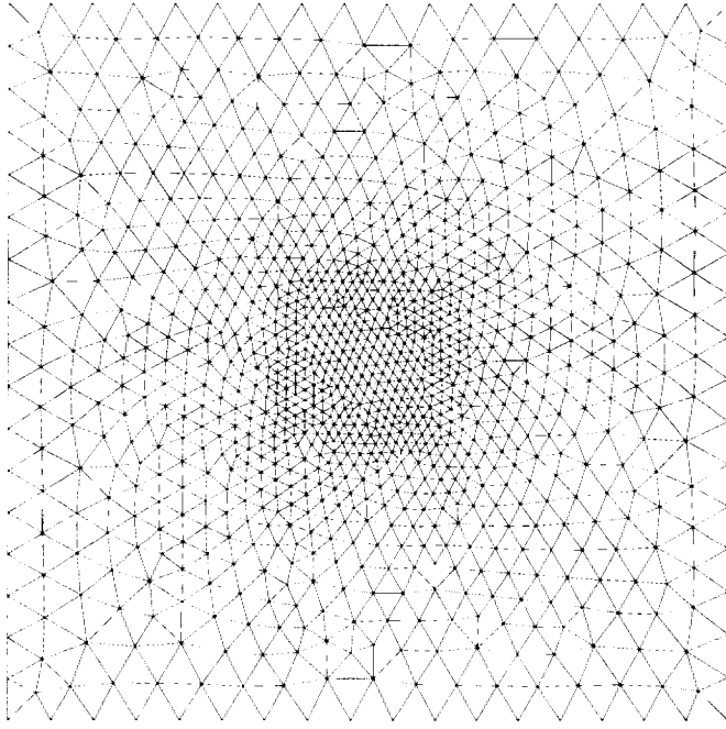
FIG. 4.12. Triangulation used for the propagating surfaces.
