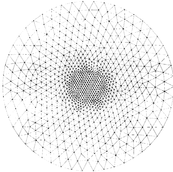
FIG. 4.15. Triangulation for the propagating surfaces on a disk.
