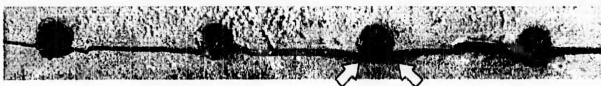
(a) Crack Located in Upper Rivet Row in Precorroded Specimen. Arrows Indicate Crack Initiation Sites.
