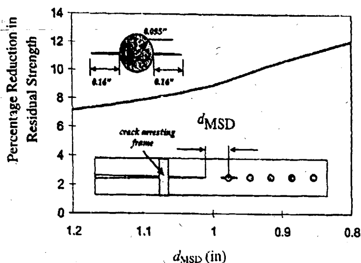
Figure 8. The Influence of d_{MSD} , the Distance Between the Lead Crack Tip and the Center of the First Rivet Hole, on the Reduction in Residual Strength.
