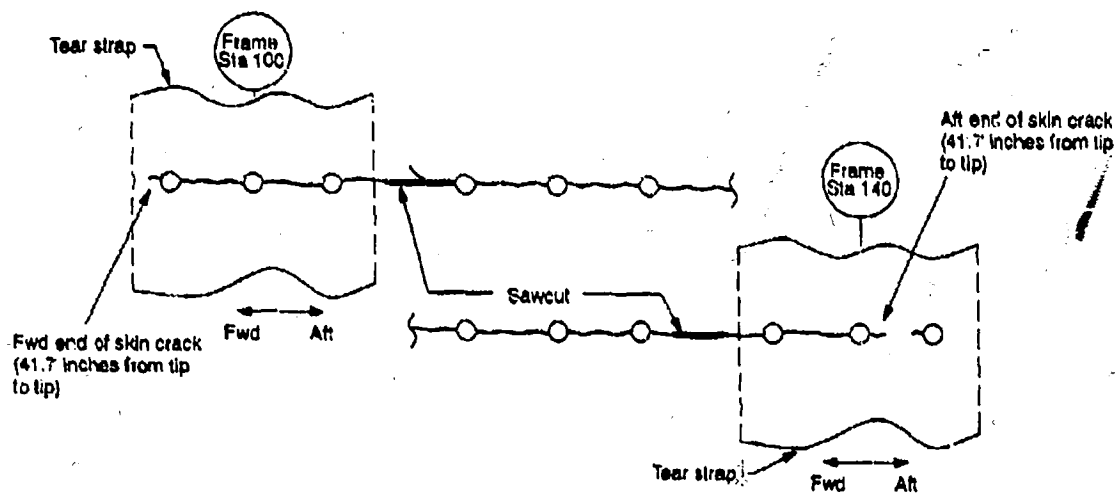
Figure 6. Crack Configuration Prior to Panel Failure (FAA 2-Test 1).
