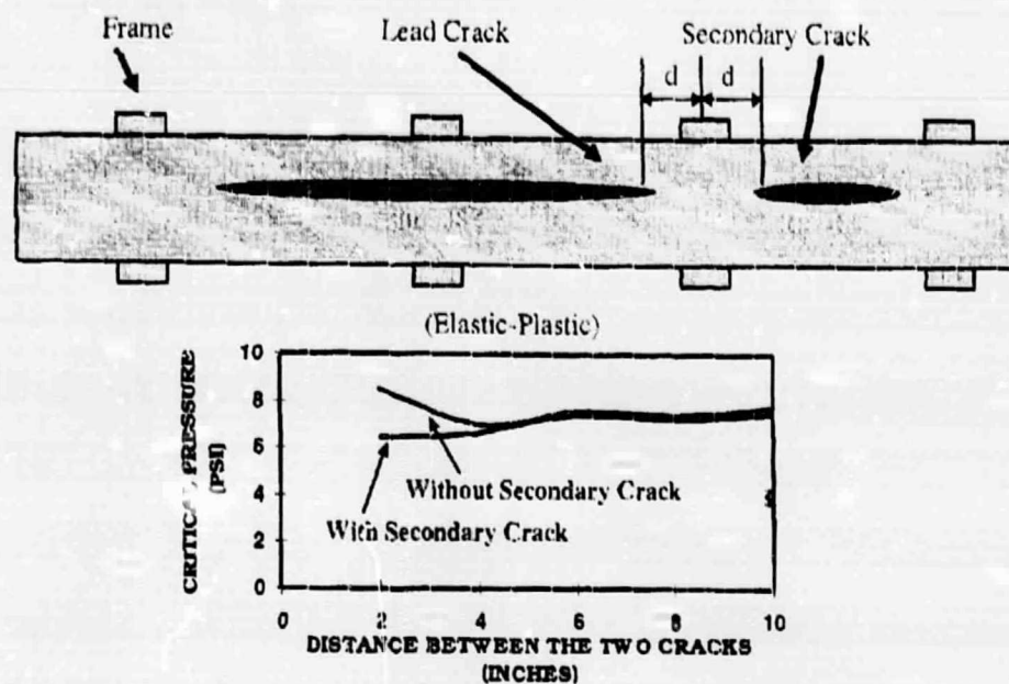
Figure 7. Interaction Between Two Large Cracks.
