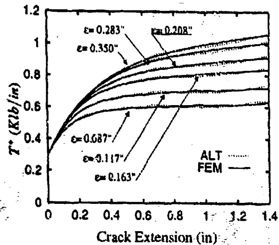
Figure 8. The T^* for NIST-90 MSD-3 Using EPFEM and Classical FEM.
