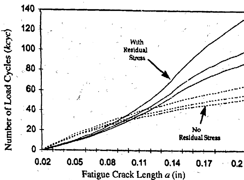
Figure 11. Fatigue Crack Growth With and Without the Effects of Residual Stress.
