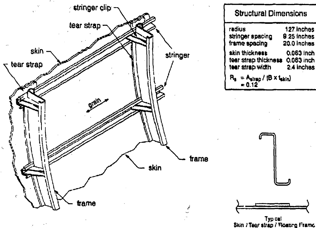
Figure 2. Structural Details of Panels FAA 1 and FAA 2.
