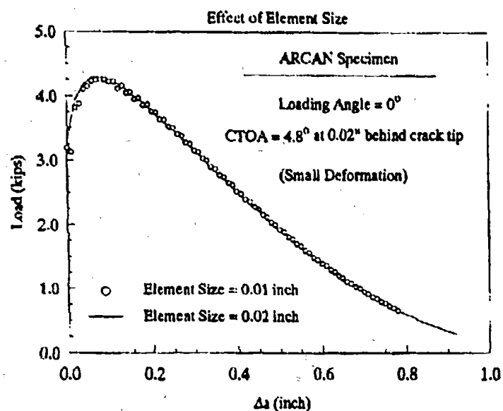
Figure 7. Effect of Finite Element Size on Crack Growth Simulation.
