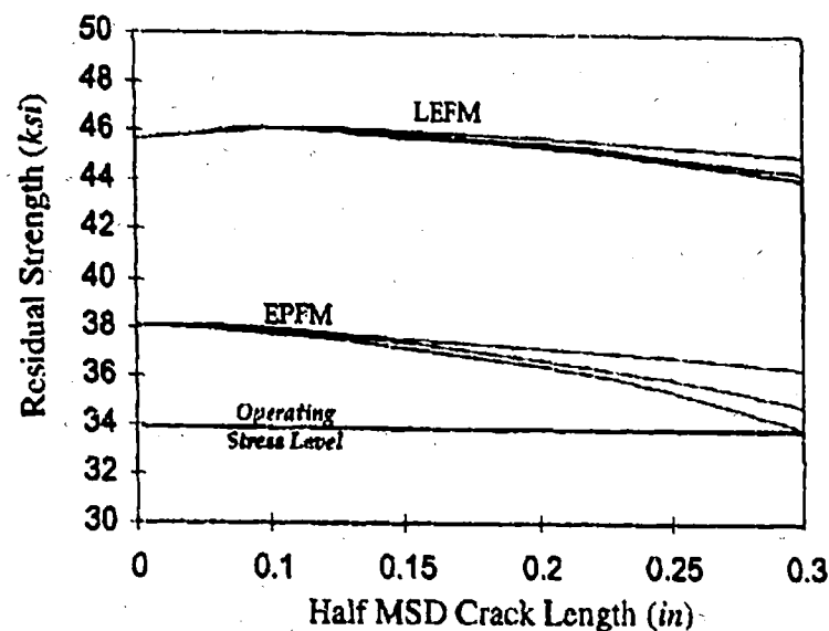
Figure 10. Residual Strength in the Presence of MSD Cracks and a Lead Crack With a Half-Crack Length of 8 Inches.
