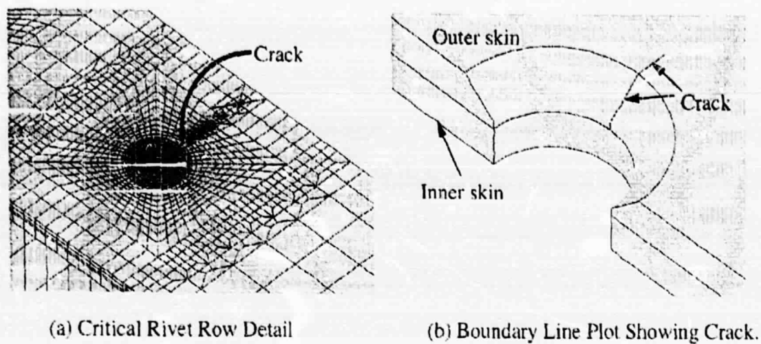
Figure 3. Fracture Mechanics Finite Element Model.
