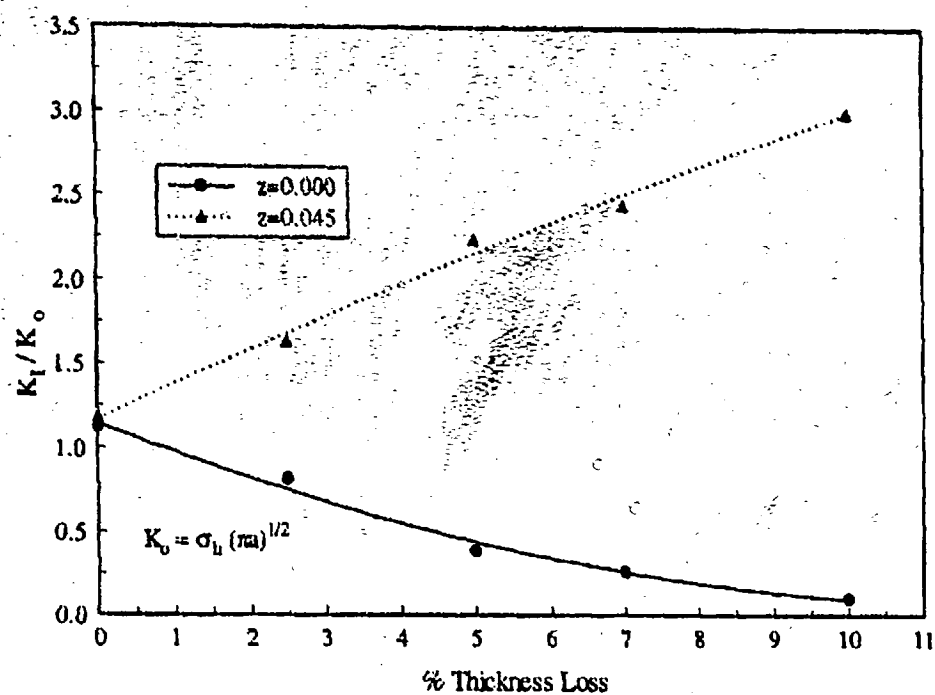
Figure 8. Nondimensional Stress Intensity Plot of Outer Skin ( z=0.000 ) and Inner Skin ( z=0.045 ) Crack Edges Where \sigma_h is the Applied Hoop Stress in Plate and a is the Crack Length From the Center of the Rivet Hole.
