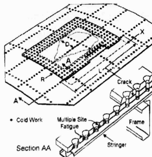
Figure 12. External Patch Repair of a Fuselage Skin.
