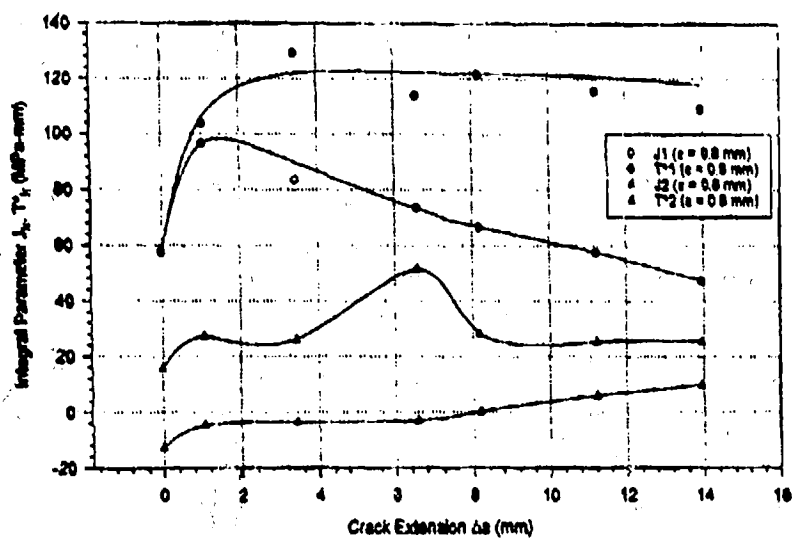
Figure 5. T^*_{ke} Variation With Crack Extension.
