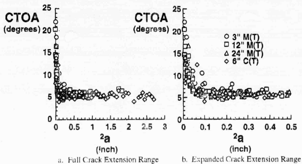
Figure 4. Surface CTOA Measurements for 2024-T3 Aluminum Alloy Fracture Tests.
