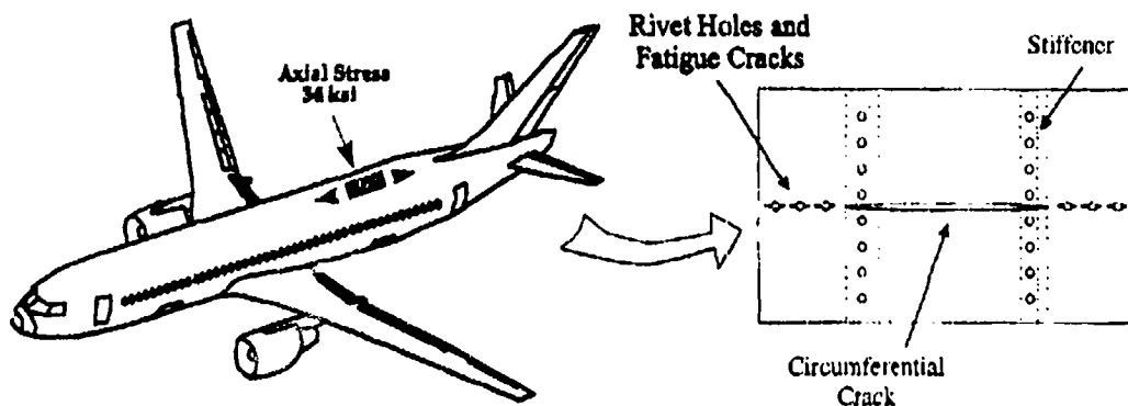
Figure 1. A Critical Location on the Aircraft Fuselage for Circumferential Damage.
