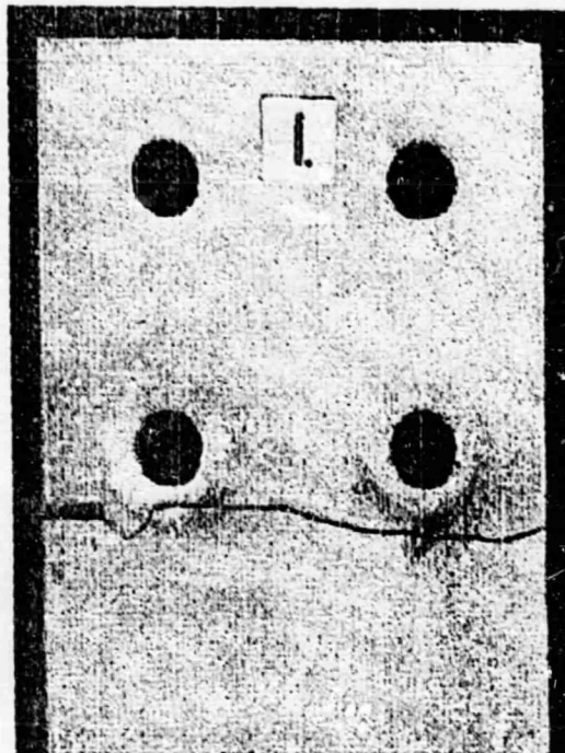
Figure 1. Fatigue Failure of a Lap Splice Attributed to Fretting (Ref. 3).
