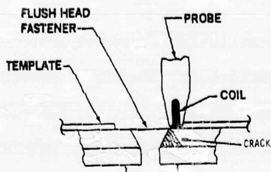
Figure 1. Short Fatigue Crack Under Flush-Head Fastener.
