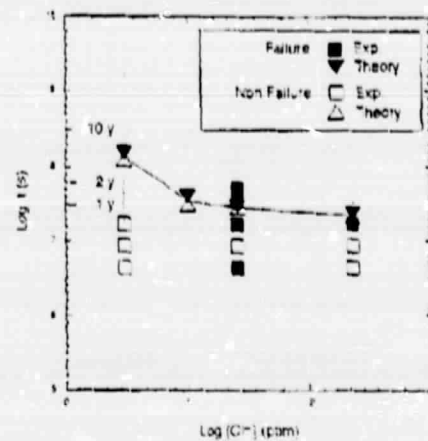
Figure 8. The Measured and Calculated Service Life for Type 304L SS Heat Exchanger Tubes as a Function of [Cl^-] . Parameters are Identical to Those for Figure 7.
