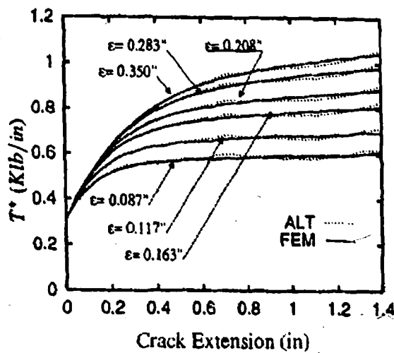
Figure 7. The T^* for NIST-90 MSD-2 Using EPFEM and Classical FEM.
