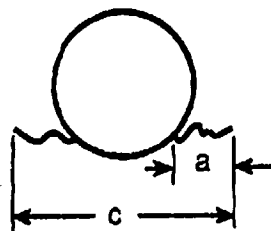
Figure 3. Drawing of Top Panel Surface With Rivet Head Defining a and c .
