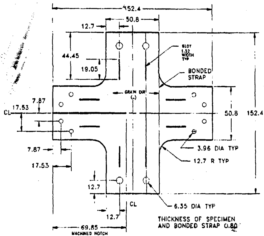
Figure 2. Biaxially Loaded SEN Specimen.
