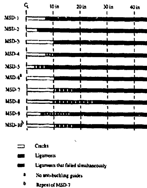
Figure 4. Experimental Results Illustrating the MSD Linkup Behavior for Each of the NIST-90 MSD Tests.
