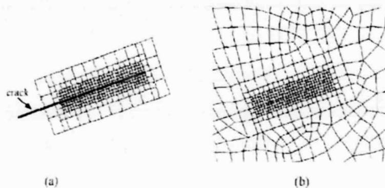
Figure 13. (a) A Template Inserted Along the Tearing Path and (b) the Final Mesh Generated By the all-Quadrilateral Element Meshing Algorithm.
