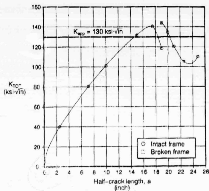
Figure 10. Stress-Intensity Factor Predictions at Operating Pressure.
