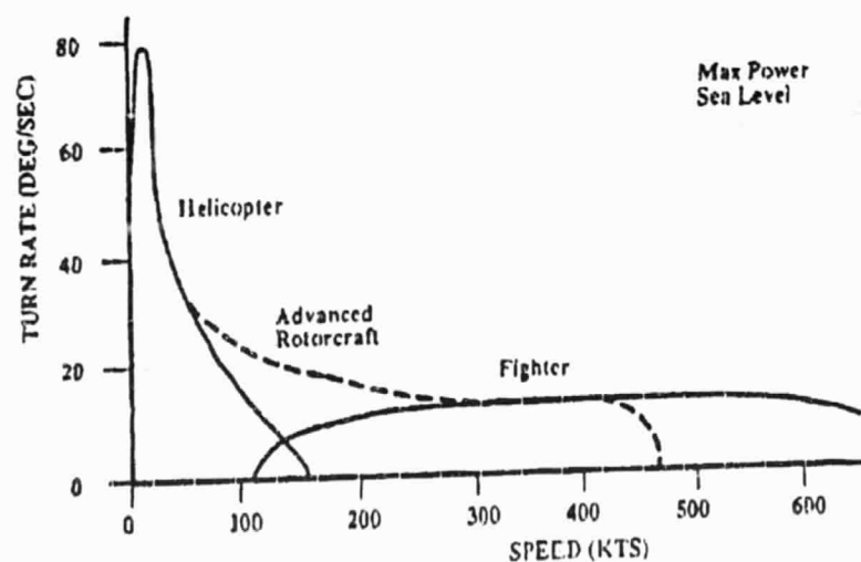
Figure 4. Rotorcraft are Agile Machines in Terms of Turning Rate.
