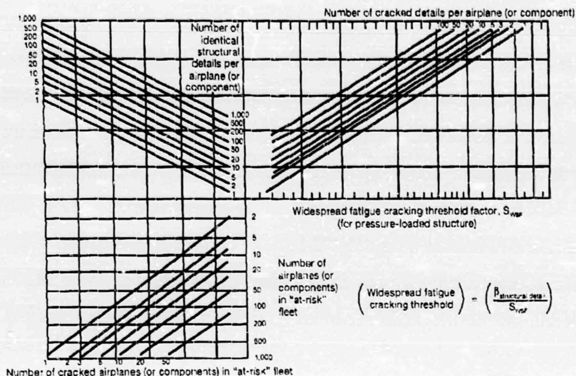
Figure 5. Nomograph for Estimating WFD Threshold Factor for Pressurized Structures.
