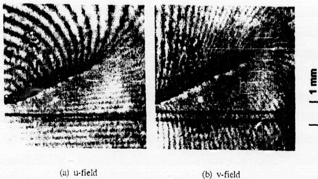
Figure 3. Moiré Fringe Patterns of a Biaxially Loaded 2024-T3 Aluminum SEN Specimen.
