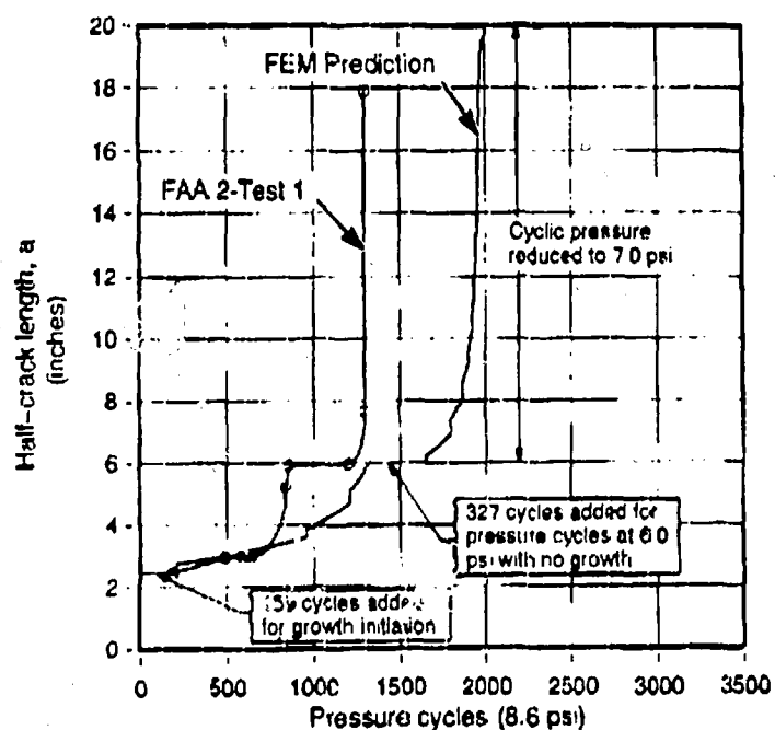
Figure 13. Crack Growth Predictions Versus Test Results for FAA 2-Test 1 (varied MSD).
