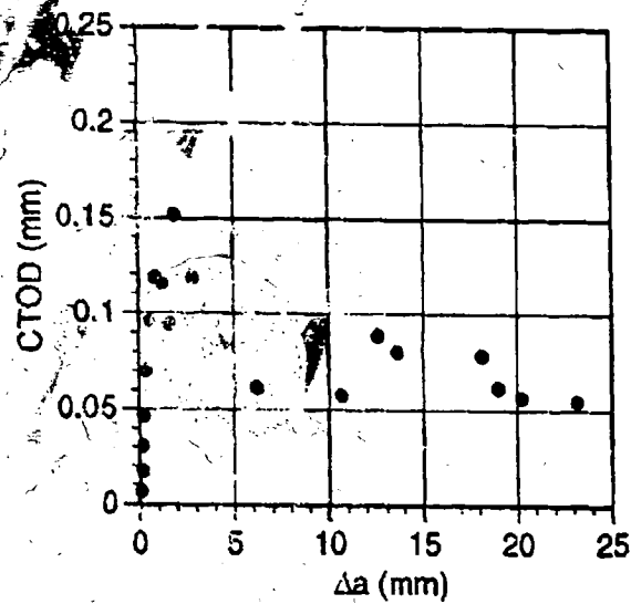
\Phi=0^\circ , TL Specimen
