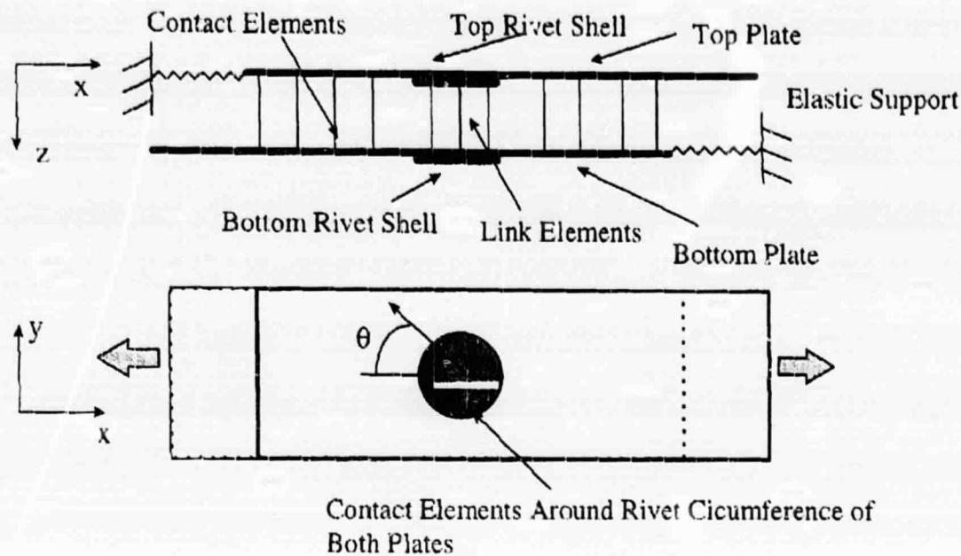
Figure 7. Schematic of Shell Model.
