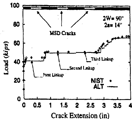
Figure 12. Load and Crack Growth Predictions for NIST-90 MSD-4 Compared With Experimental Results.
