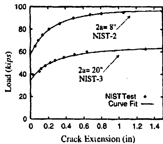
Figure 6. Experimental Data for NIST-90 MSD-2 and MSD-3.
