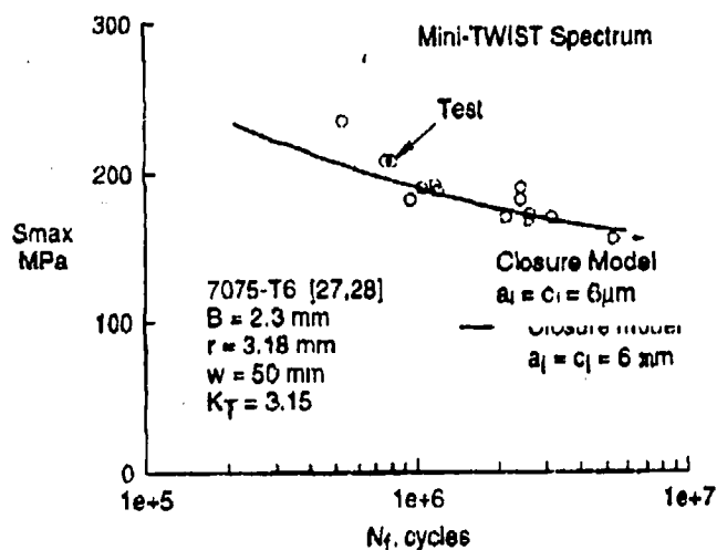
Figure 13. Measured and Predicted Fatigue Lives for 7075-T6 Aluminum Alloy SENT Specimens Under Mini-TWIST Spectrum Loading.
