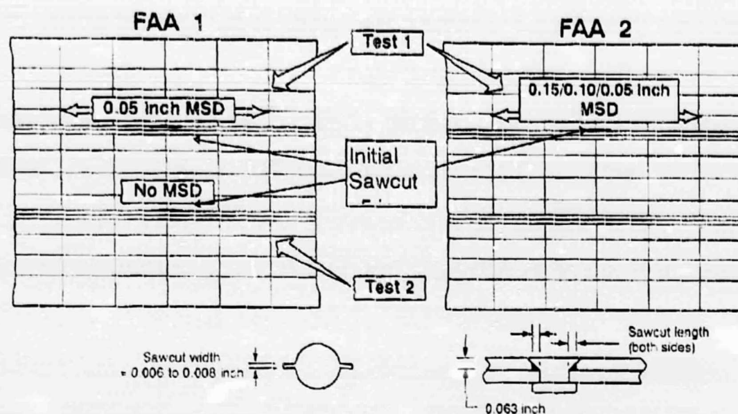
Figure 3. Simulated MSD Regions.
