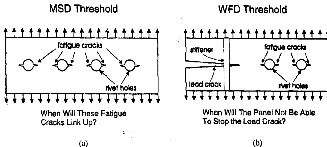
Figure 1. MSD Threshold Approach and WFD Threshold Approach.
