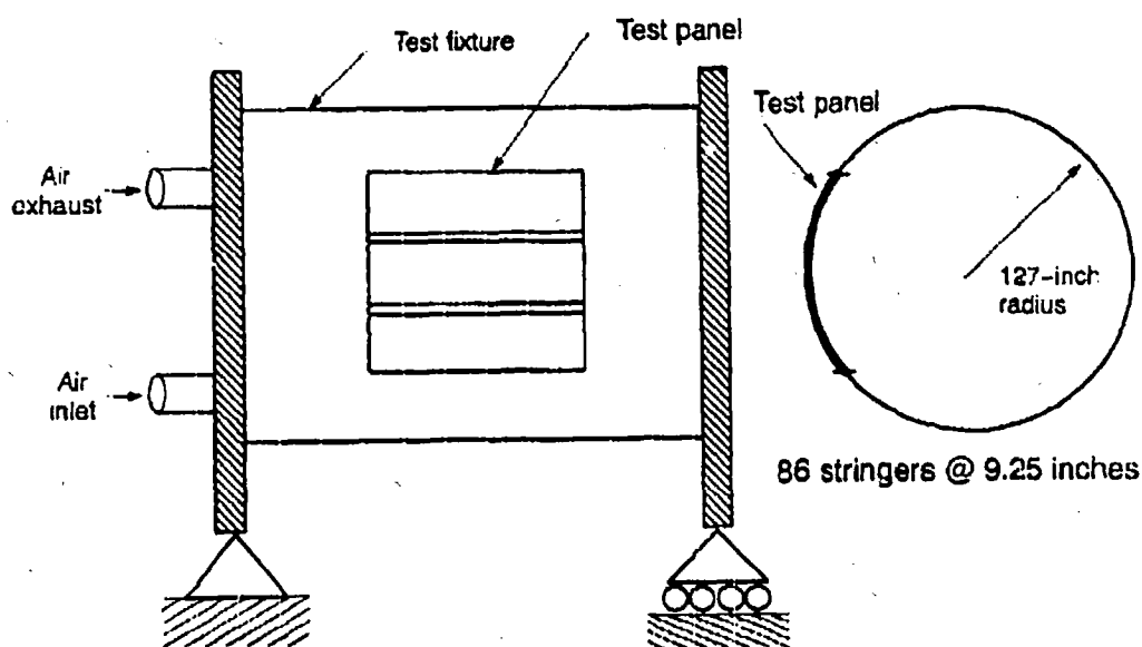
Figure 1. Wide-Body Pressure Test Fixture.
