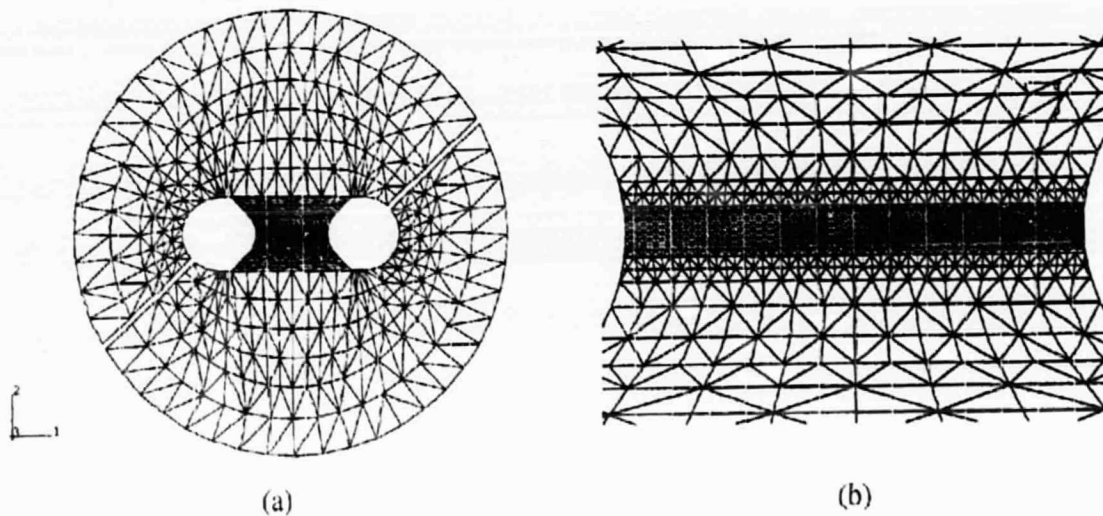
Figure 6. Finite Element Mesh used in Mode I ARCAN Test Simulations: (a) Global Mesh, (b) Refined Local Mesh Along Crack Growth Path.
