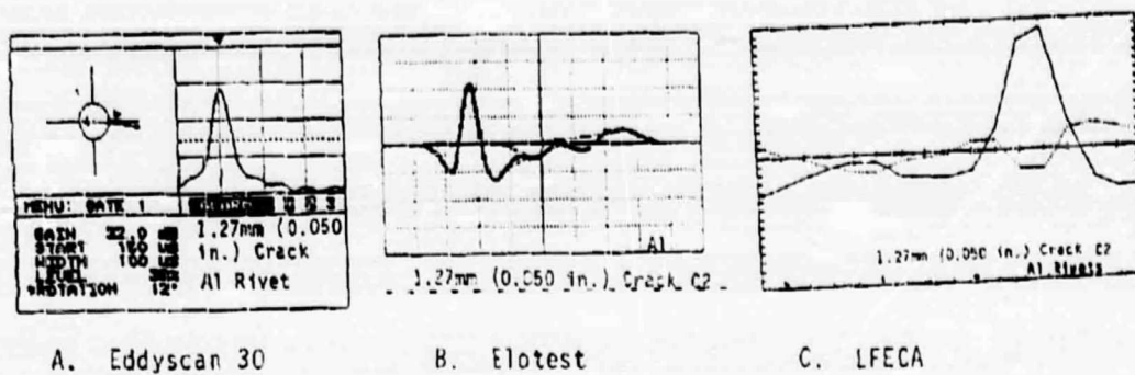
Figure 3. Detection of 1.27-mm (0.050-in.) Crack Under Flush-Head Aluminum Fastener.
