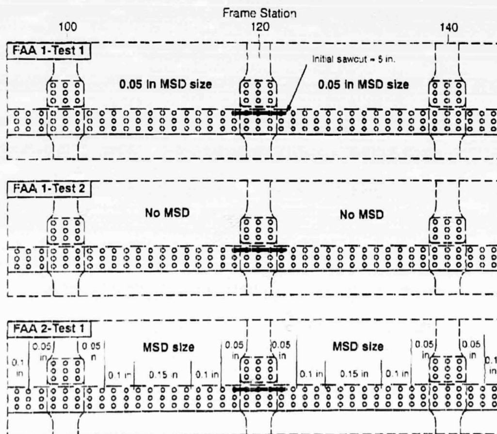
Figure 4. Initial Sawcut Installation and Simulated MSD Sizes.
