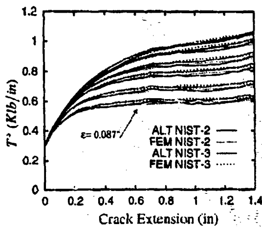
Figure 9. The T^* for NIST-90 MSD-2 and MSD-3 Using EPFEM and Classical FEM.
