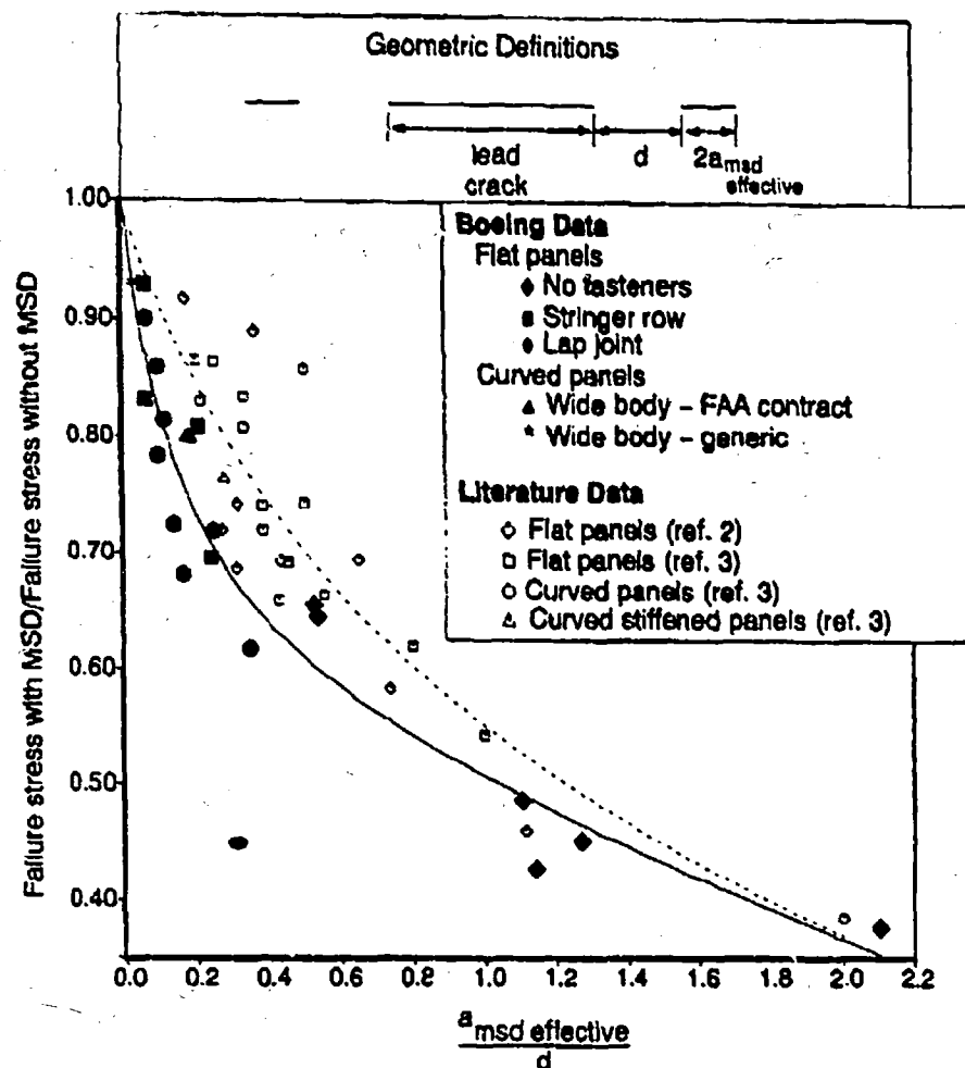
Figure 17. Comparison of MSD Test Data.
