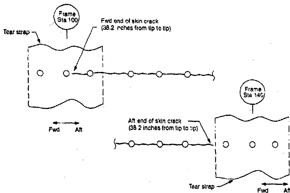
Figure 5. Crack Configuration Prior to Panel Failure (FAA 1-Test 2).
