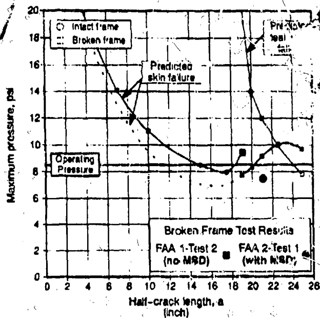
Figure 14. Residual Strength Test and Analysis Correlation.
