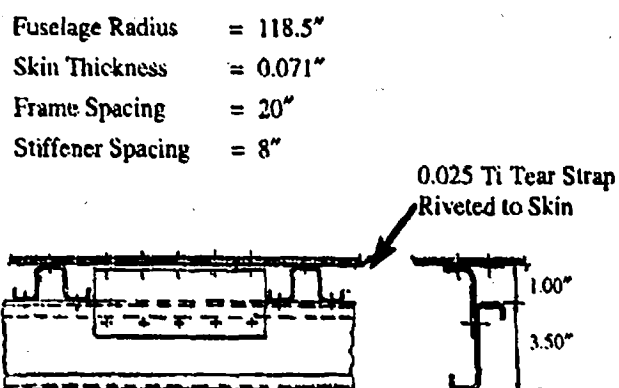
Figure 2. The Geometric Dimensions of the Fuselage Panel.
