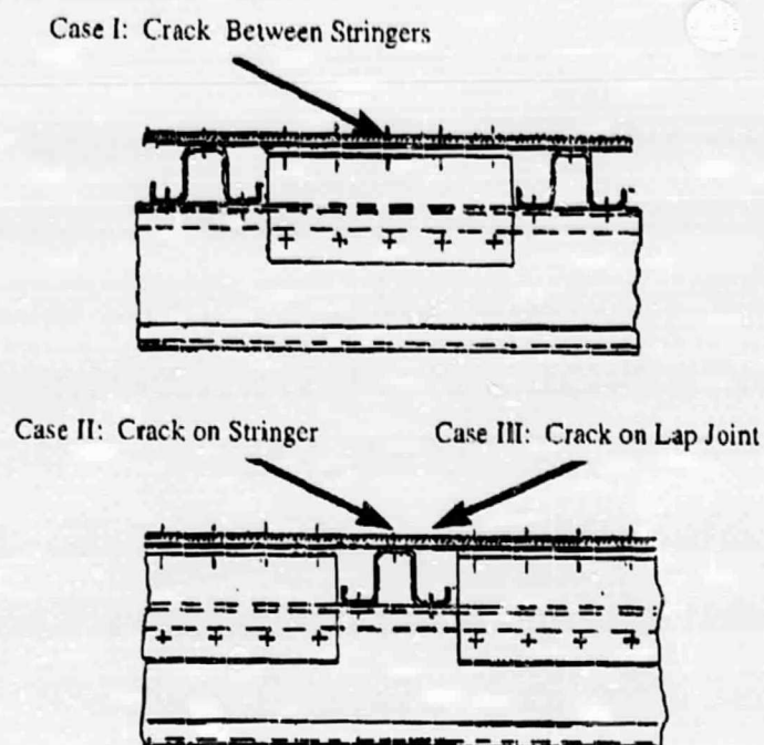
Figure 6. The Effect of Frame Design in the Residual Strength of a Two-Bay Crack.
