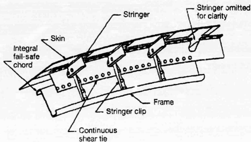
Figure 8. Frame With Shear Ties.
