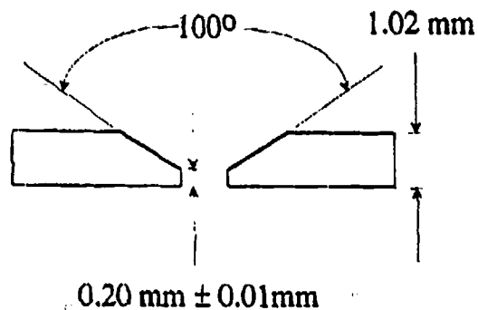
Figure 2. Section View of Sheet With Countersunk Hole.
