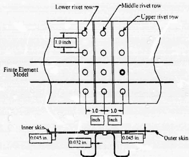
Figure 1. Lap Joint Configuration.
