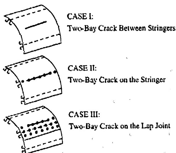
Figure 4. Locations of the Two-Bay Crack.
