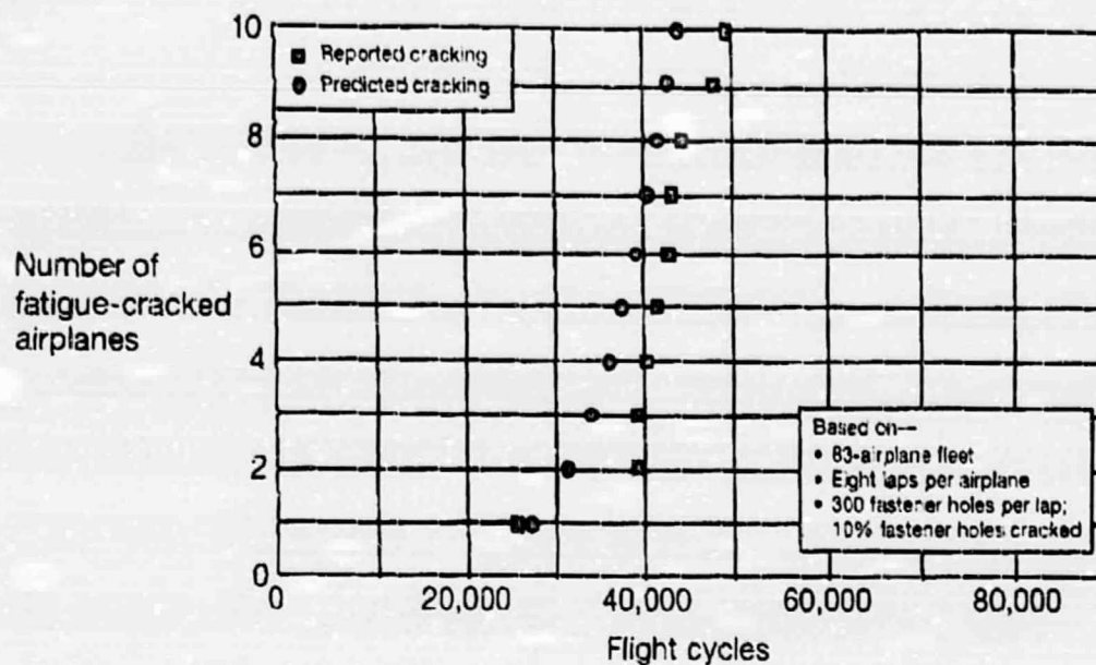
Figure 11. Comparison of Predicted and Actual Cracking Histories for Example Problem 3.
