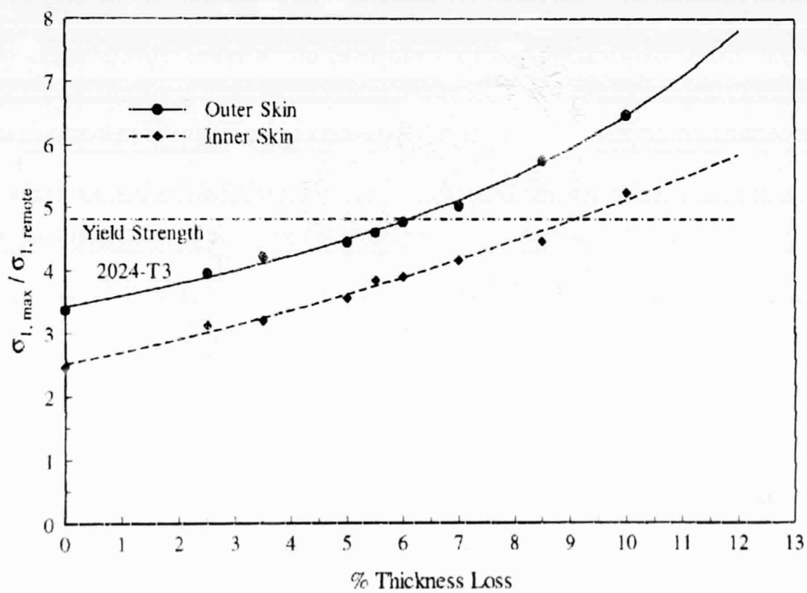
Figure 4. Effect of Increased Corrosion Pilling on Critical Rivet Row of Respective Skins.
