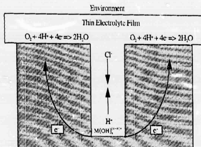
Figure 2. Schematic of Coupled Environment Pitting/Fracture Model Employed in the Deterministic Estimation of Pit and Crack Propagation Rates in Metals and Alloys Under Thin Electrolyte Films That Condense on a Surface.
