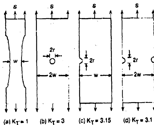
Figure 2. Fatigue Specimens Analyzed With Small-Crack Theory.
