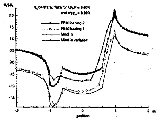
Figure 3. Tangential Stress, \sigma_{xx} , Along the Contact Surface FEM Loading 1 and the Mindlin Cases Involve no Bulk Stress While FEM Loading 2 and the Mindlin Variation Cases Incorporate the Bulk Stress \sigma_o . For the Given Set of Conditions ( Q/\mu P ) and ( \sigma_o/\mu P_o ), no Reversal of Microslip at the Contact Surface Occurs.
