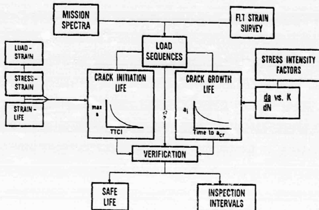
Figure 5. Flow Diagram of the Total Life Methodology.
