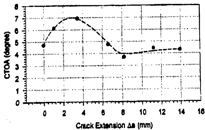
Figure 7. CTOA Variation With Crack Extension.
