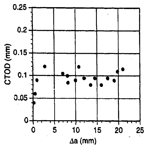
\Phi=15^\circ , LT Specimen
