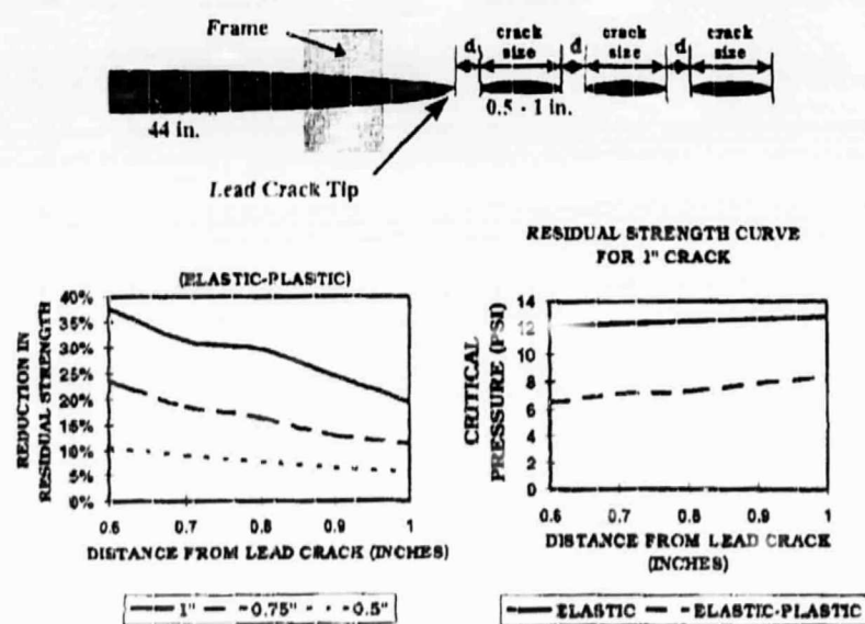
Figure 9. Interaction of a Lead Crack With Three Smaller Cracks.
