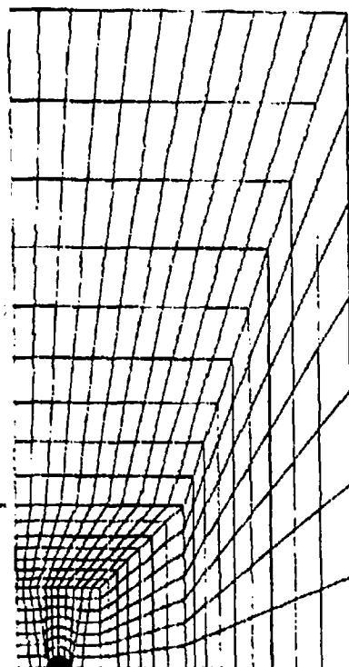
Figure 3. Typical Finite Element Mesh.
