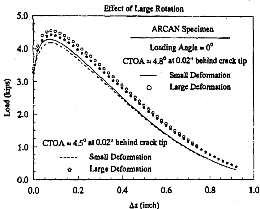
Figure 9. Effect of Large Specimen Rotation on Crack Growth Simulation.
