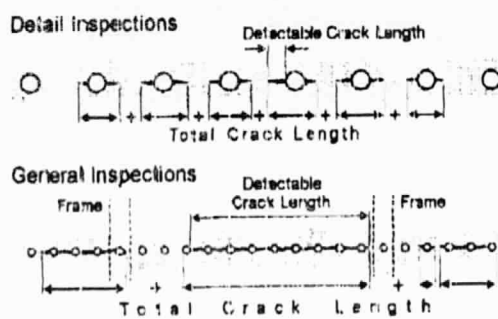
Figure 5. Detectable and Total Crack Lengths.
