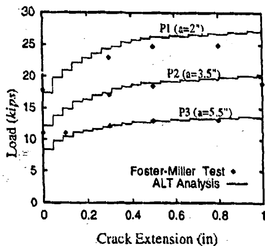
Figure 11. Load and Crack Growth Predictions for Foster-Miller Single Crack Panels P1, P2, and P3 Compared With Experimental Results.
