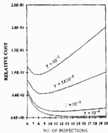
Figure 6. Relative Cost C_i Versus Number of Inspection.
