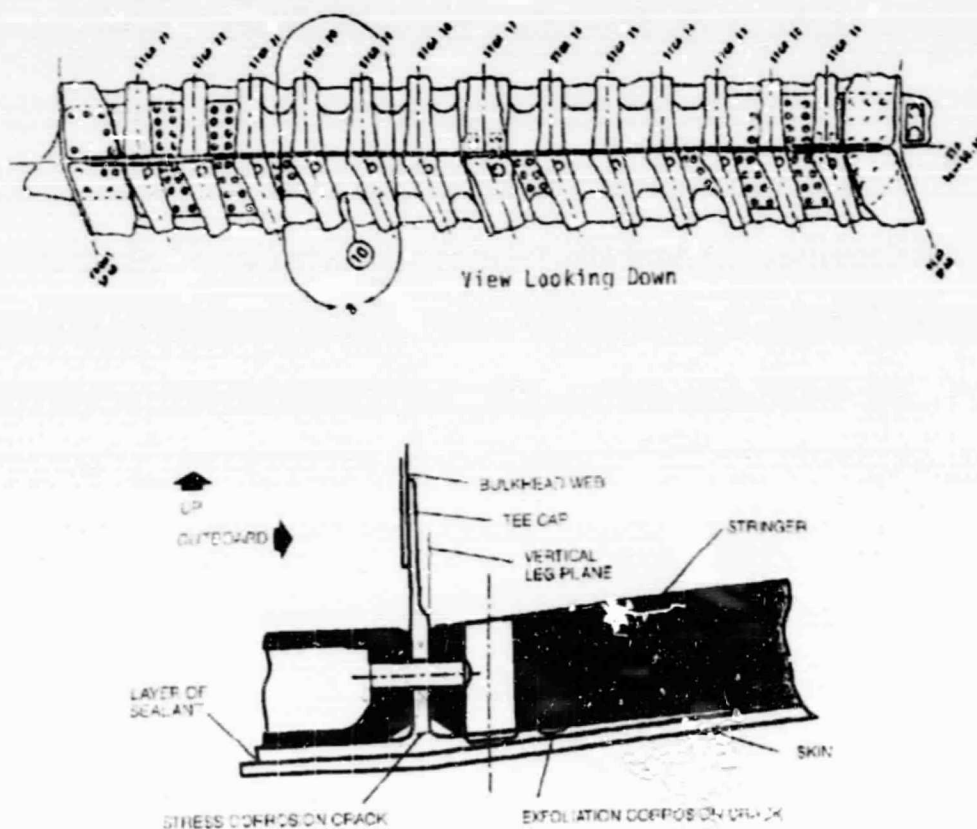
Figure 11. DC-11 Lower Wing Skin and Tee Cap and Stringers.
