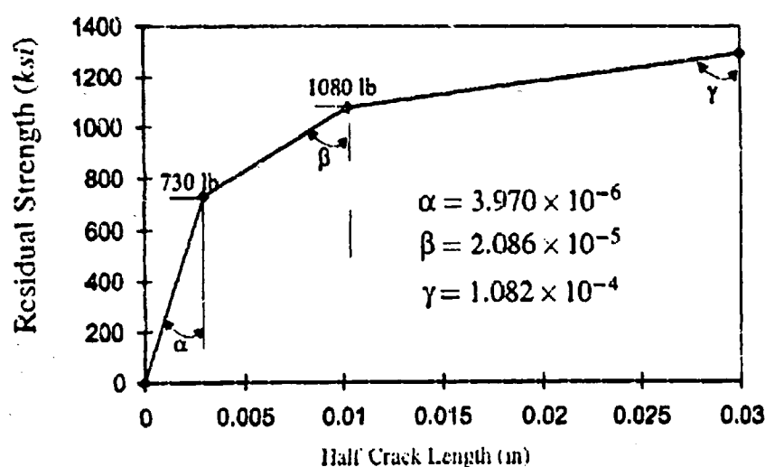
Figure 7. Nonlinear Rivet Flexibility Curve.
