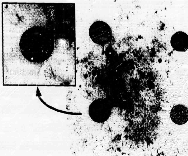
(a) Cracks in Area of Maximum Pillowing in Outer Skin.
