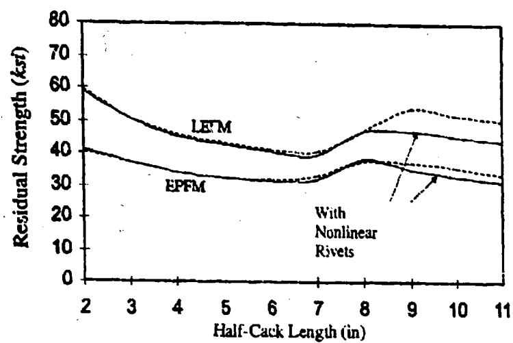
Figure 8. Effect of the Nonlinear Behavior of the Rivets.
