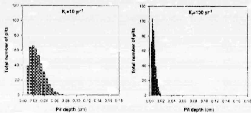
Figure 9. Differential Damage Functions for Carbon Steel in Oxygenated Pure Water ( T = 150^\circ C , pH = 5.82 , [O_2] = 7.5 ppm , t_{ex} = 2 yrs ) as a Function of the Delayed Repassivation Rate Constants. Note that the Pit Depths Were Calculated Using an Empirical Correlation Between Pit Depth and Time for Pits Grown Under Identical Conditions.
