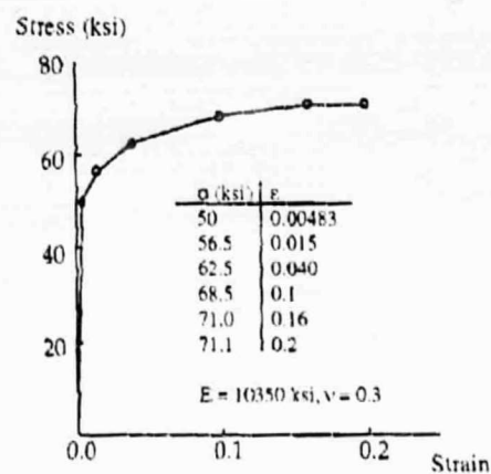
Figure 2. Piecewise Linear Representation of the Uniaxial Stress-Strain Curve for 2024-T3 Aluminum.
