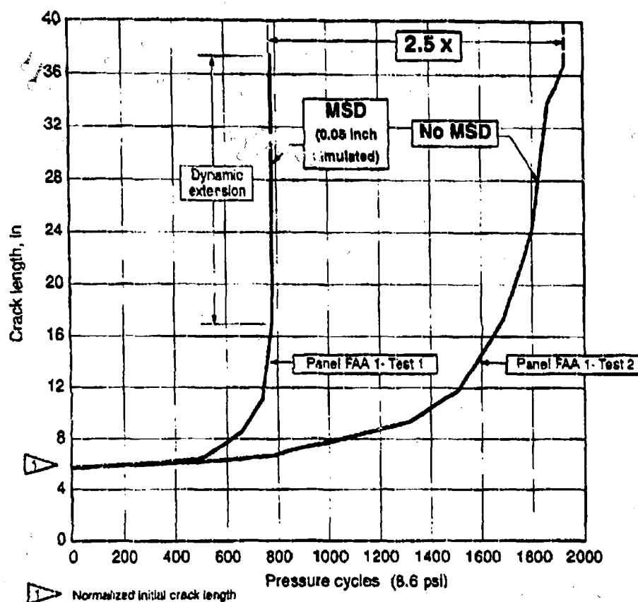
Figure 7. Crack Growth Comparison, MSD Versus Non-MSD.
