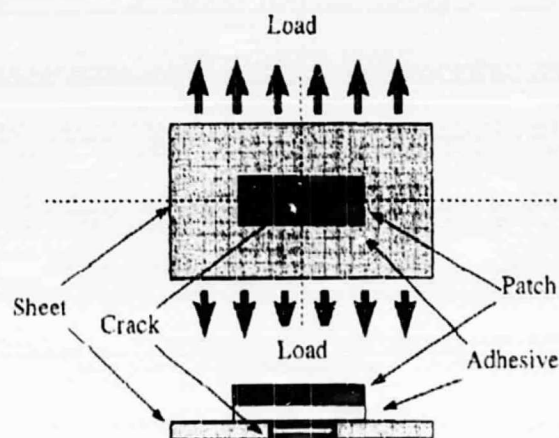
Figure 3. Composite Patch Repair Problem.
