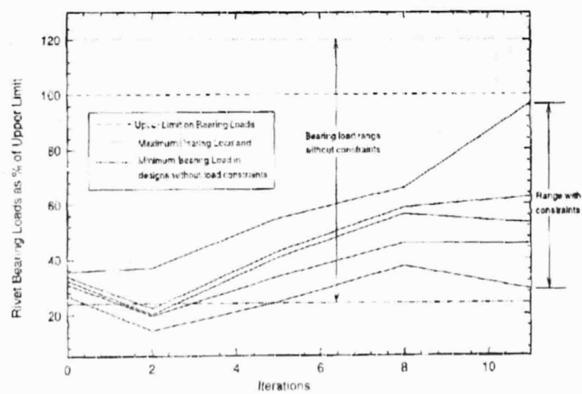
Figure 6. Iteration History of Bearing Load Constraints.
