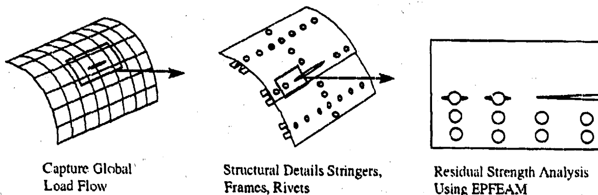
Figure 4. A Global-Intermediate-Local Hierarchical Approach for the Residual Strength Analysis of an Aircraft Fuselage.
