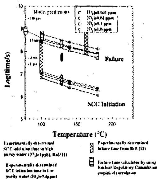
Figure 5. Calculated SCC Initiation and Total Failure Times as a Function of Oxygen Concentration and Temperature. ([NaCl] = 10^{-3} mol/cm 3 , [HCl] = 10^{-6} mol/cm 3 , \sigma = 3.0 \times 10^2 MPa, h = 1.0 \times 10^{-3} cm, a_0 = 5.0 \times 10^{-5} cm, L = 1.0 \times 10^{-3} cm, K_{ISCC} = 10 MPa m 1/2 , K_{IC} = 190 MPa m 1/2 ). See Liu and Macdonald 22 for a Discussion of the Experimental Data.
