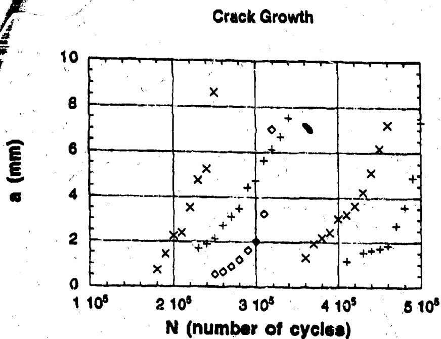
Figure 9. Crack Growth Data for Five Specimens. Note Wide Variation Among Specimens in the Number of Cycles Until a Dominant Crack is First Observed.
