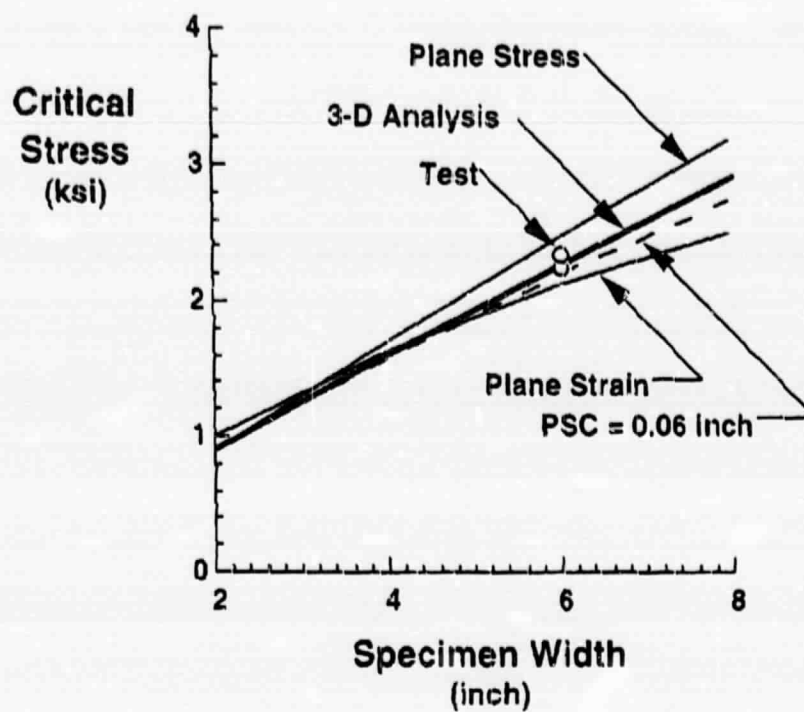
Figure 7. Critical Load Measured in the C(T) Fracture Tests, the Three-Dimensional Finite Element Simulations, and the Two-Dimensional Finite Element Predictions.
