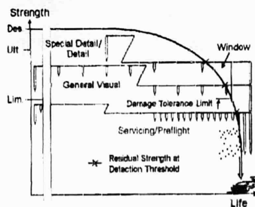
Figure 6. Inspection Opportunities With Widespread Fatigue Damage.
