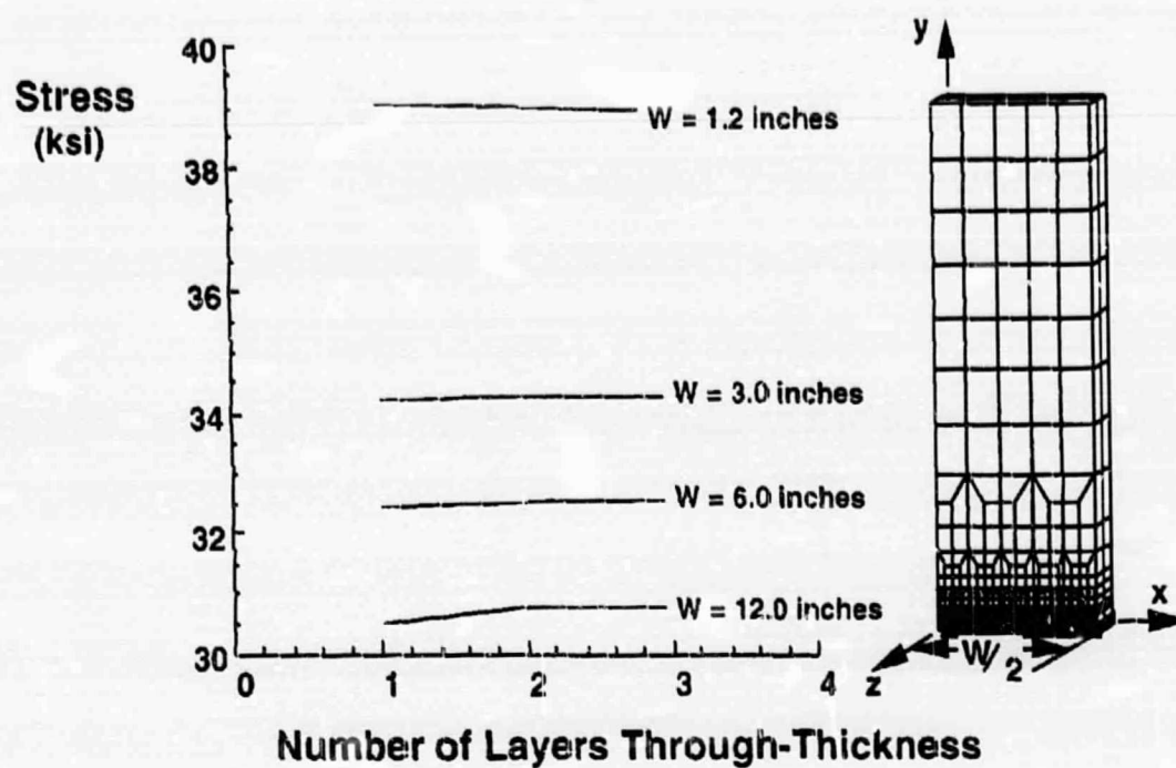
Figure 1. Three-Dimensional Finite Element Analysis Through-Thickness Convergence Study.
