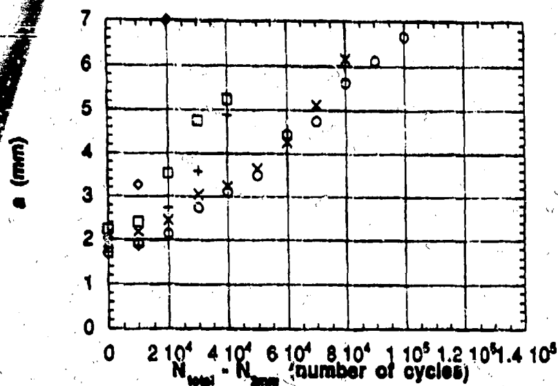
Figure 11. Crack Growth After Initiation, a vs. N_{total} - N_{2mm} . A Variation of 85,000 Cycles for Growth of an Approximate 2-mm Crack to 7 mm in Length Is Observed. Most of the Variation in the Total Cycles to 7 mm Is in the Number of Cycles for Crack Initiation.
