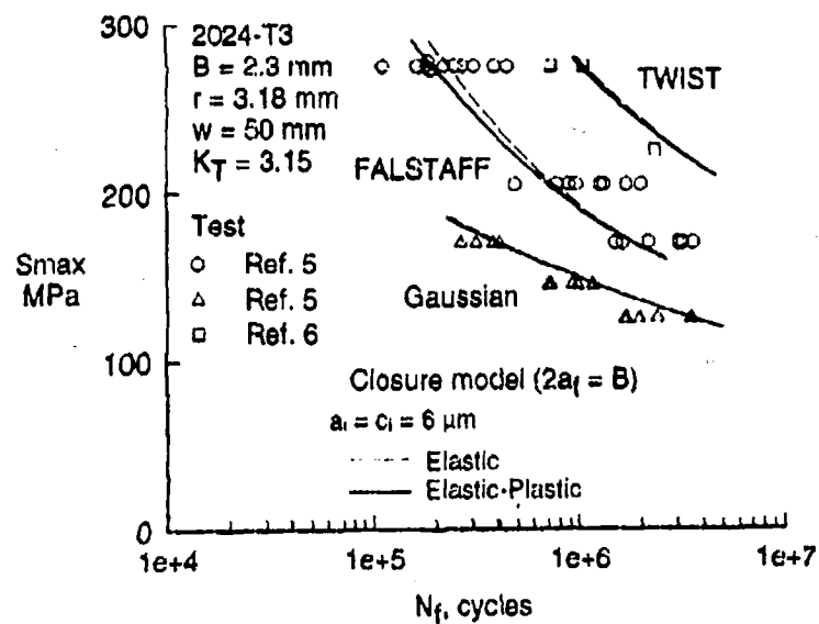
Figure 10. Measured and Predicted Fatigue Lives for 2024-T3 Aluminum Alloy SENT Specimens Under Various Spectrum Loading.
