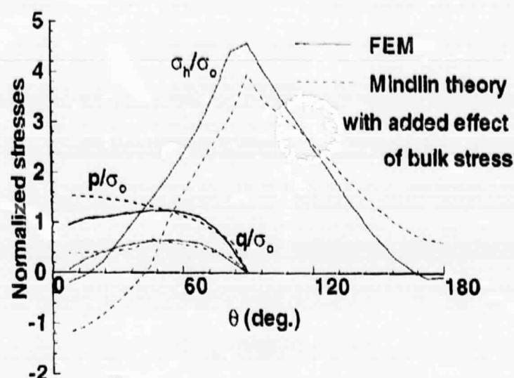
Figure 9. Normalized Contact Stresses at Fastener Hole at the Mid-Plane of the Top Plate. The Applied Clamping Force is 75 lb., and 40% of Applied Load is Transferred Through the Rivet Assembly. The Assumed Coefficient of Friction at the Fastener-Skin Interface is \mu = 0.5 .
