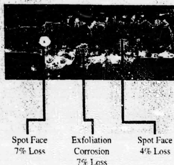
Figure 13. Second Layer Ultrasonic C-Scans Can Reveal Small Amounts of Material Loss
