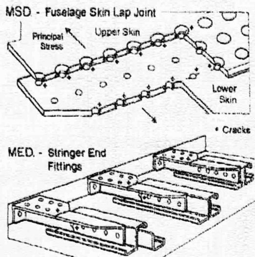
Figure 1. Examples of MSD and MED.
