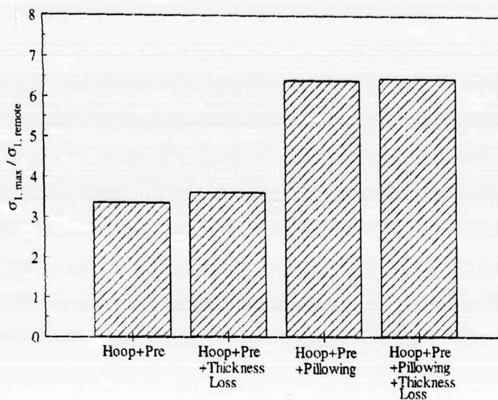
Figure 5. Effect on Stress Caused by Reduction of Outer Skin Thickness as Compared to Pillowing (10% thickness loss).
