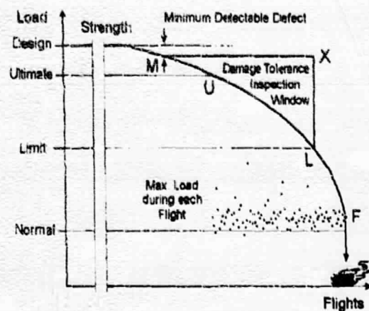
Figure 2. Damage Tolerance Inspection Window.
