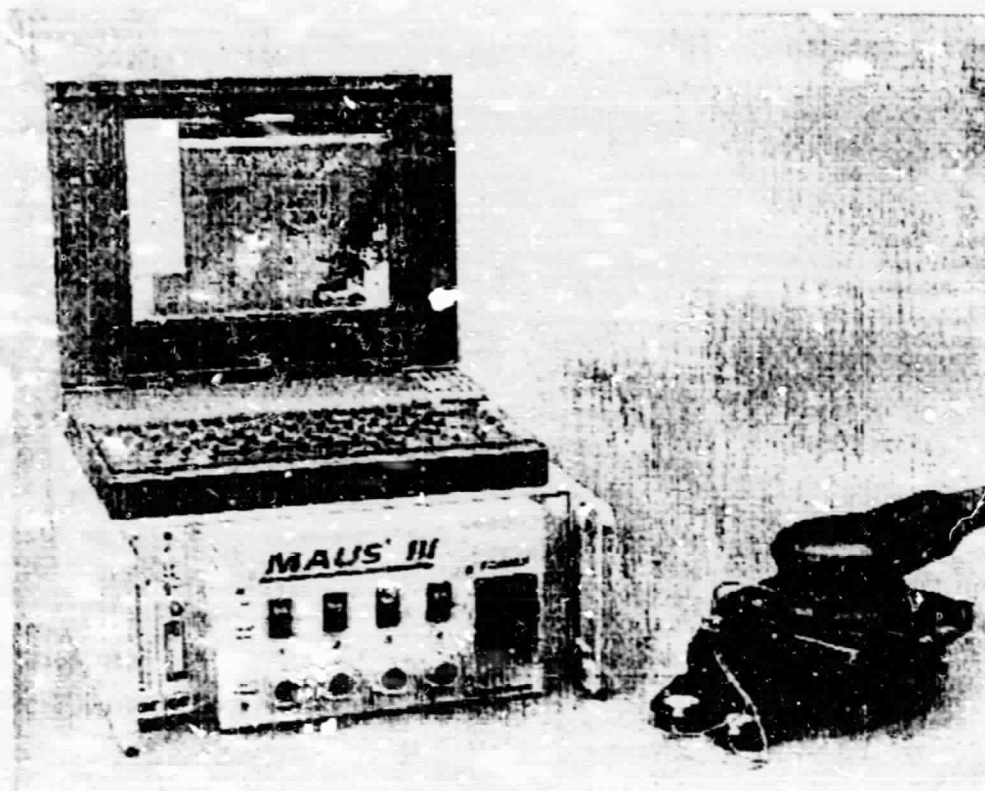
Figure 8. Mobile Automated Scanner (MAUS III).
