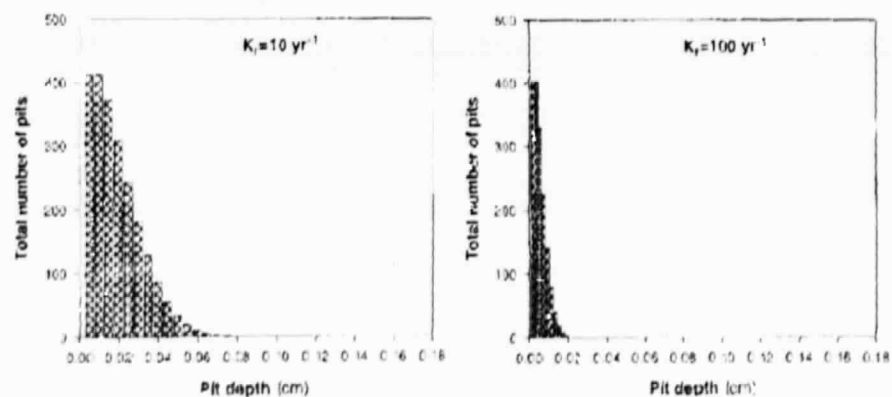
Figure 10. Integral Damage Functions for Carbon Steel in Oxygenated Pure Water ( T = 150^\circ C , pH = 5.82 , [O_2] = 7.5 ppm , t_{ex} = 2 yrs ) as a Function of the Delayed Repassivation Rate Constant.
