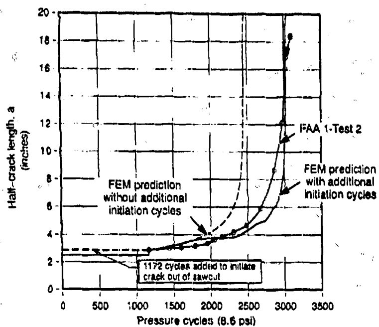
Figure 12. Crack Growth Predictions vs. Test Results for FAA 1-Test 2 (No MSD).
