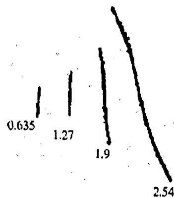
Figure 5. Hocking FastScan Results for Cracks Under Flush-Head Rivets (Millimeters)
