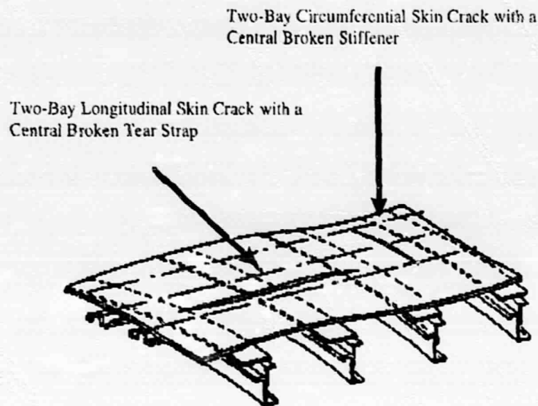
Figure 1. Damage Tolerance Requirement Based on Two-Bay Crack.
