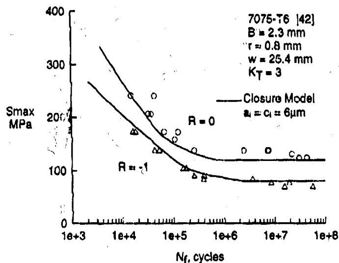
Figure 12. Measured and Calculated Fatigue Lives for 7075-T6 Aluminum Alloy Circular-Hole Specimens.
