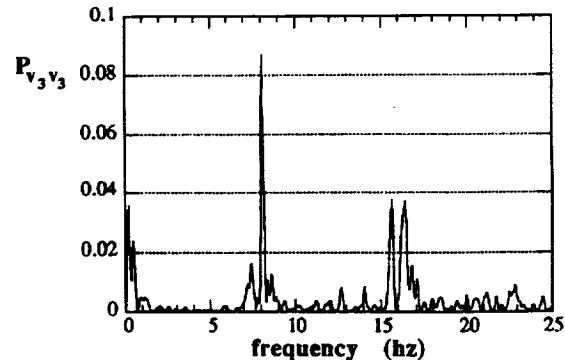
Fig. 4 Power spectrum of \alpha_z residuals, flight test run 1.
