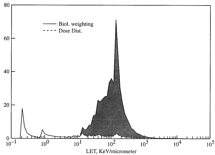
Figure 2. Dose equivalent and physical dose distributions for the galactic cosmic rays at solar minimum behind 1 g/cm 2 aluminum shielding. The shaded area denotes the difference between the distributions with and without the ICRP60 quality factor included.
