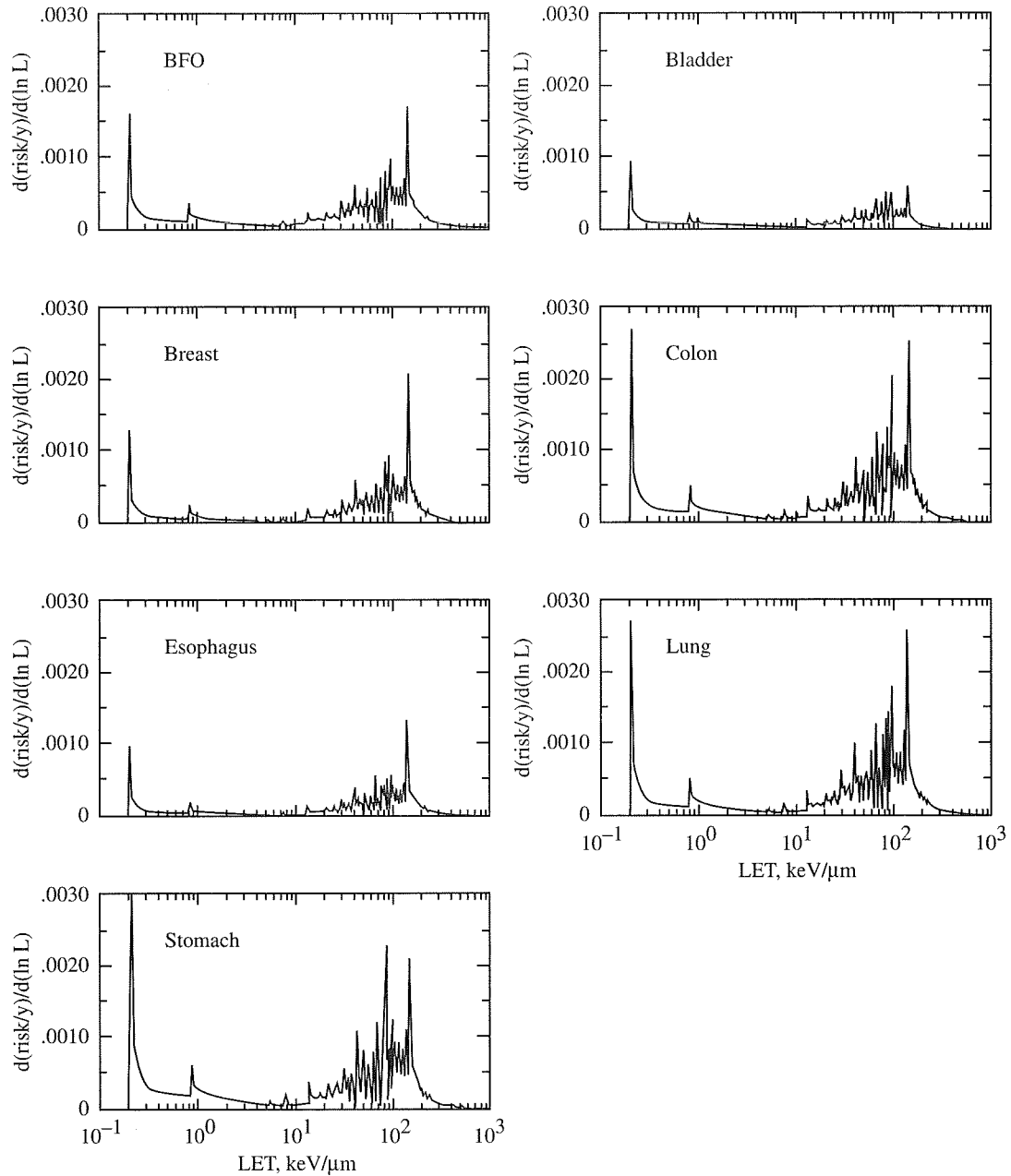
Figure 4. Differential risks per logarithmic interval of LET for one year's exposure to the galactic cosmic rays at solar minimum behind 10 \text{ g/cm}^2 aluminum shielding plotted semi-logarithmically against LET for seven radiation-sensitive organs. The plots show the relative importance of the various components of LET to the total risk (from [6]).
