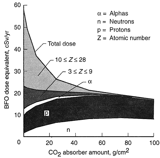
Figure 11. BFO annual dose-equivalent contributions from specified particle constituents as a function of carbon dioxide absorber amount for GCR at solar minimum conditions (Simonsen et al. 1990a).
