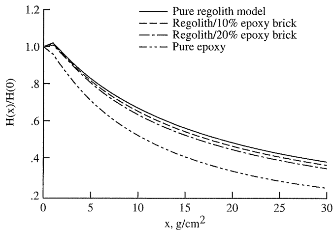
Figure 13. Attenuation of dose equivalent due to 1977 solar minimum GCR fluence behind regolith and regolith-epoxy shield as a function of areal density [27].
