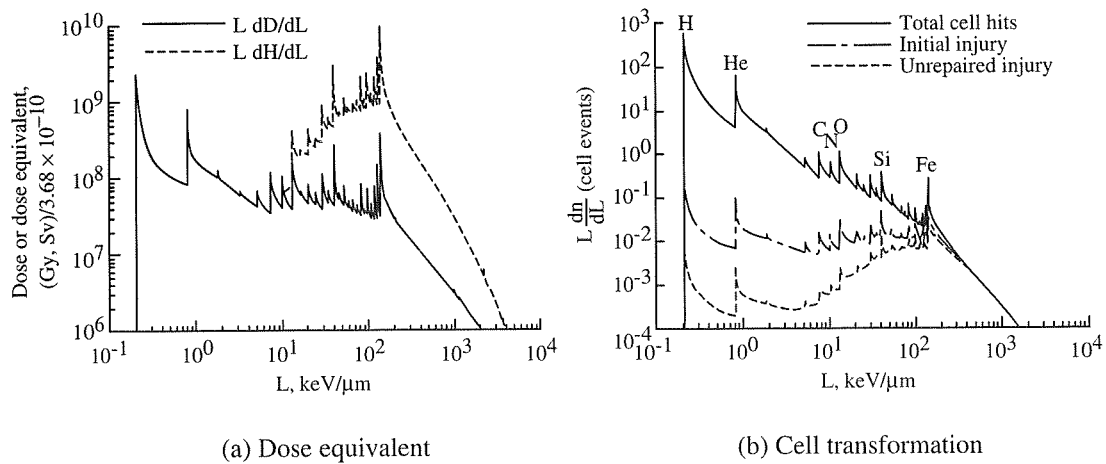
Figure 17. Distribution of biological injury behind 5 g/cm 2 of aluminum according to two biological models
