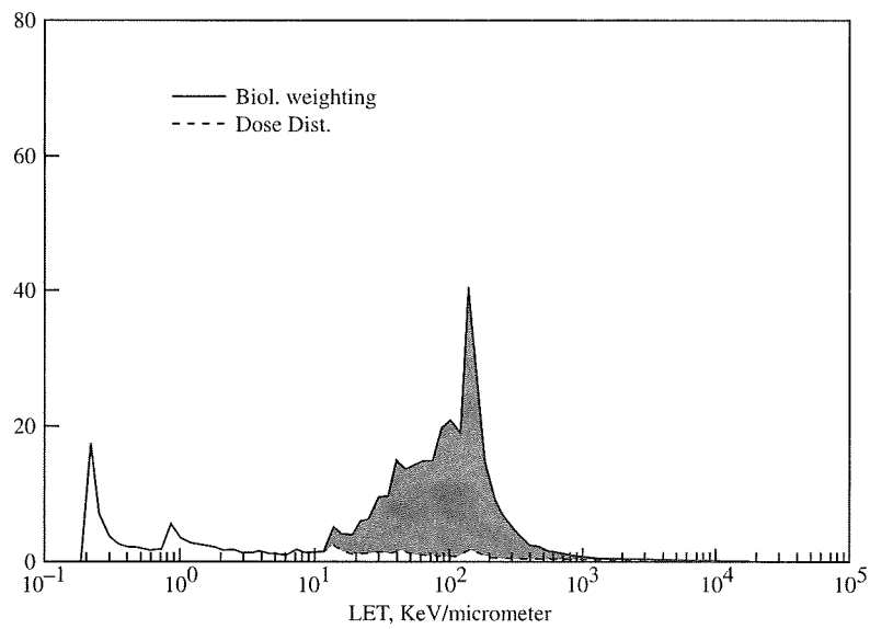
Figure 3. Dose equivalent and physical dose distributions for the galactic cosmic rays at solar minimum behind 10 \text{ g/cm}^2 aluminum shielding. The shaded area denotes the difference between the distributions with and without the ICRP60 quality factor included.
