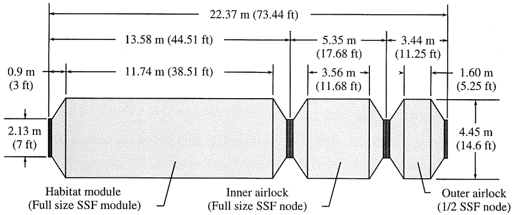
Figure 2. Lunar outpost habitat Concept 2 [2].
