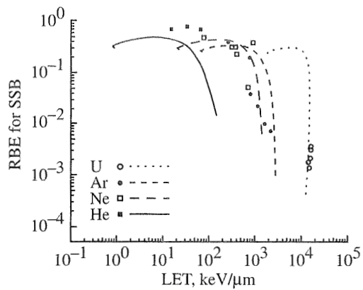
Figure 7a. Comparison of calculations (lines) in radial dose model and experiments (symbols) for RBE for SSB's in mammalian cells.
