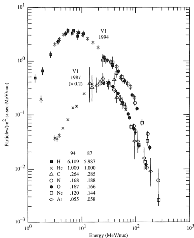
Figure 5. Energy spectra of anomalous cosmic rays.
