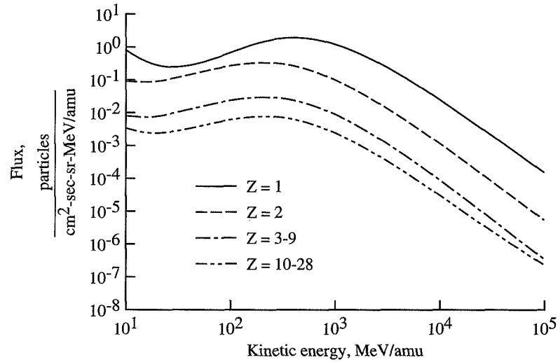
Figure 7. Galactic cosmic ray differential flux spectra at solar minimum for selected elemental groupings.
