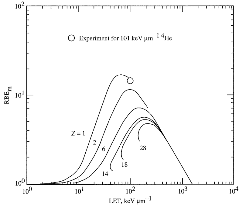
Figure 7. RBE_m for cell survival of a C3H10T1/2 exponential population. The ( \odot ) is the value measured by Bettega, et al. (1990) for low energy ^4\text{He} ions at 0.01 Gy.
