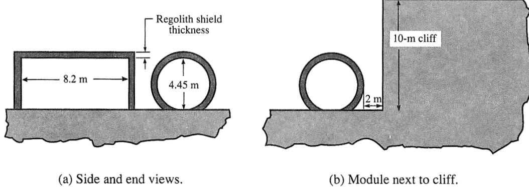
Figure 20. Cylindrical habitat module with regolith shielding for Mars (Simonsen et al. 1990b).
