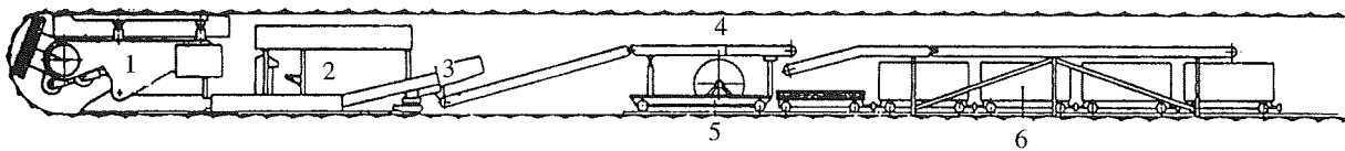
Figure 3. A tunnel boring machine with its support system (from Handewith and Dahmen [10]). 1 = tunneling machine, 2 = trailer with the motors, 3 = machines's muck removal system, 4 = transfer conveyor, 5 = skid frame, 6 = railcars for transporting muck out of the tunnel.
