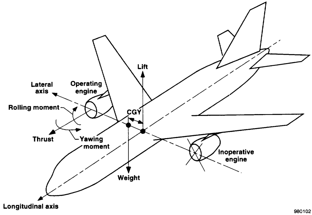
Figure 3. Forces and moments on an airplane with a wing engine inoperative and a CGY offset.
